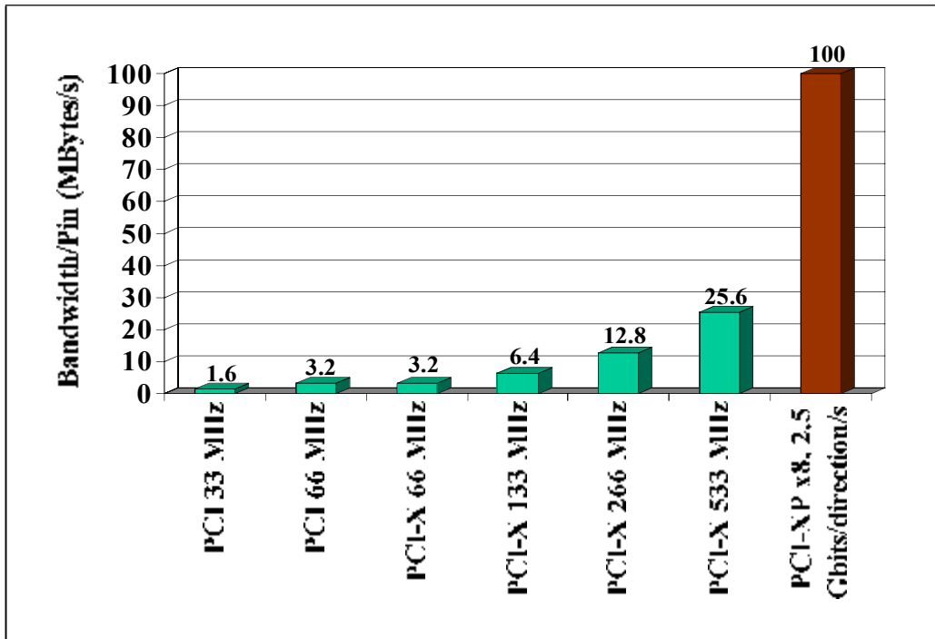
Figure 1-1: Comparison of Performance Per Pin for Various Buses
