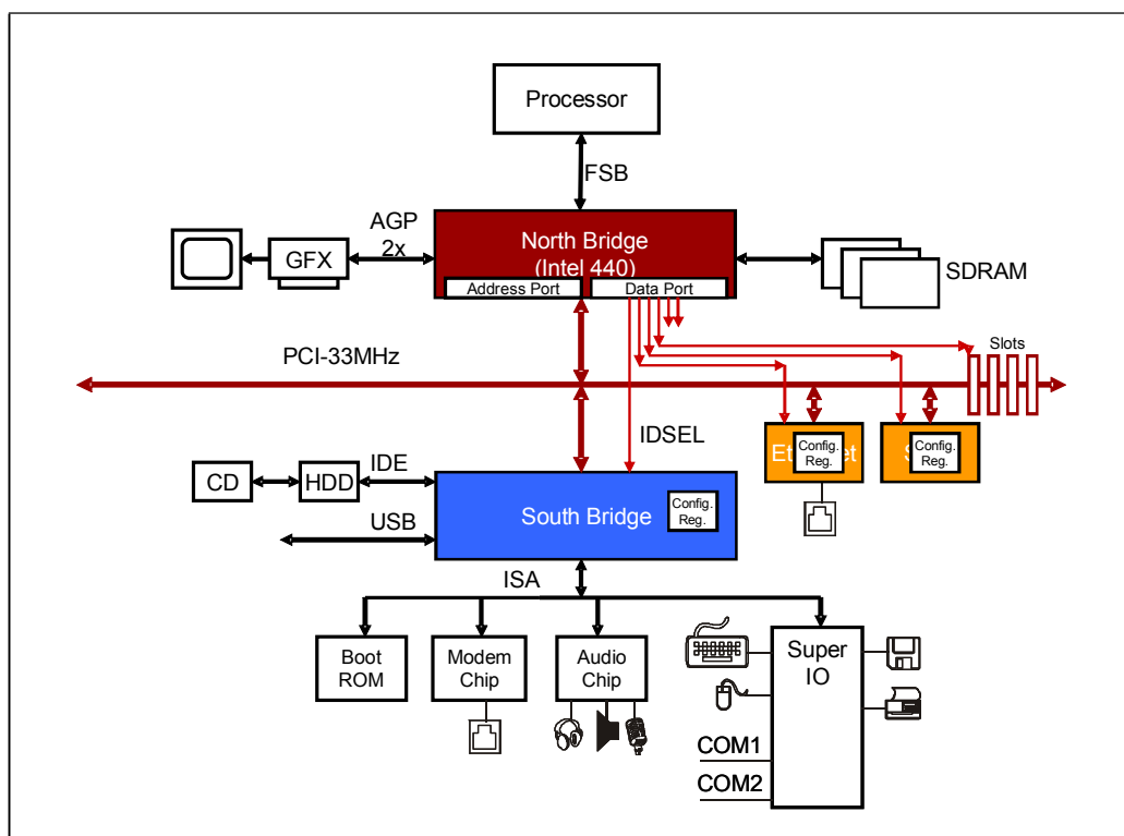
Figure 1-12: PCI Configuration Cycle Generation
