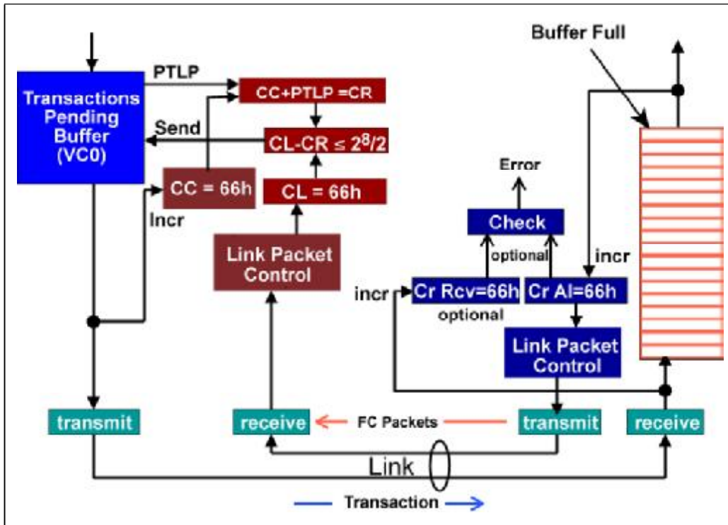
Figure 7-7: Flow Control Elements with Flow Control Buffer Filled
