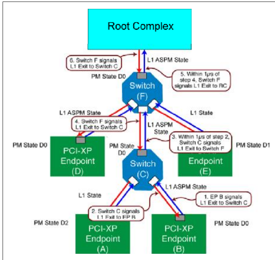
Figure 16-17: Switch Behavior When Downstream Component Signals L1 Exit
