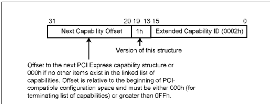
Figure 24-29: VC Enhanced Capability Header
