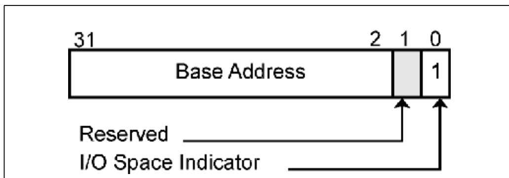
Figure 22-12: IO Base Address Register Bit Assignment
