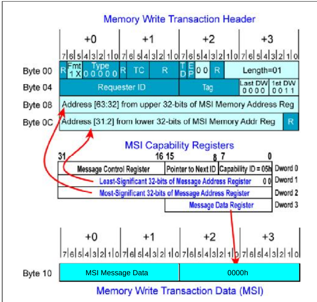
Figure 9-6: Format of Memory Write Transaction for Native-Drive MSI Delivery
