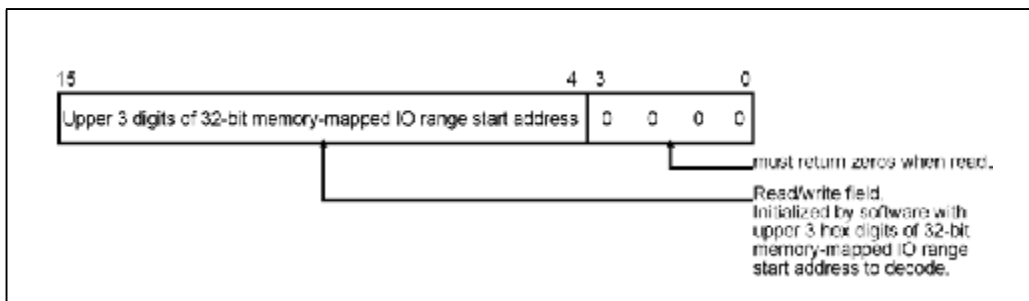
Figure 22-19: Memory-Mapped IO Base Register
