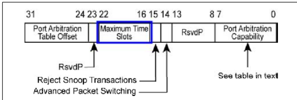
Figure 6-20: Maximum Time Slots Register
