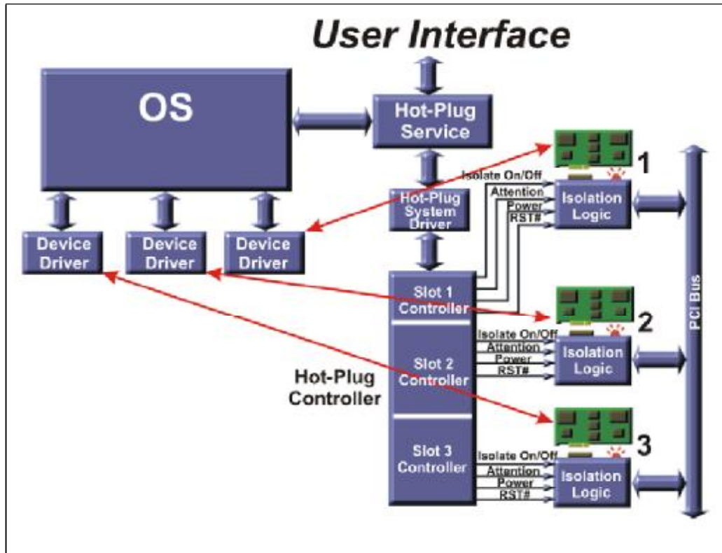
Figure 17-1: PCI Hot Plug Elements
