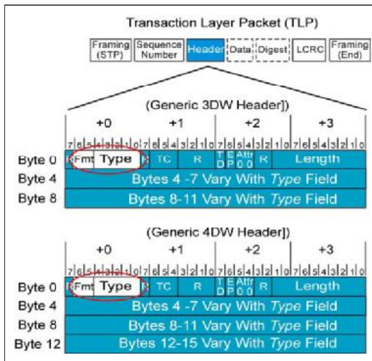
Figure 3-5: Transaction Layer Packet Generic 3DW And 4DW Headers
