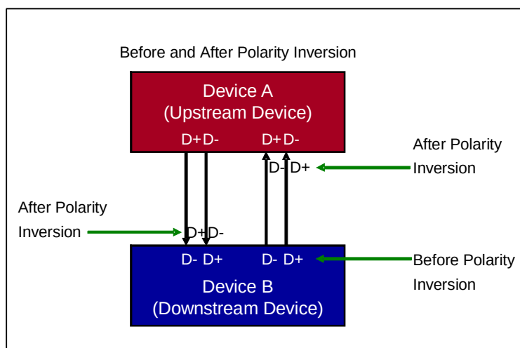
Figure 14-3: Example Showing Polarity Inversion
