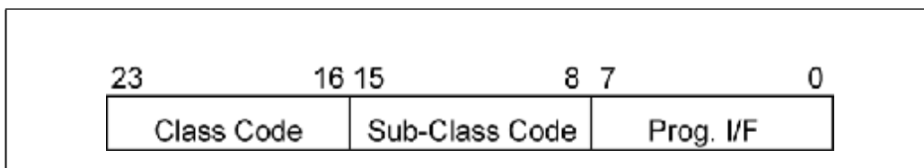
Figure 22-2: Class Code Register
