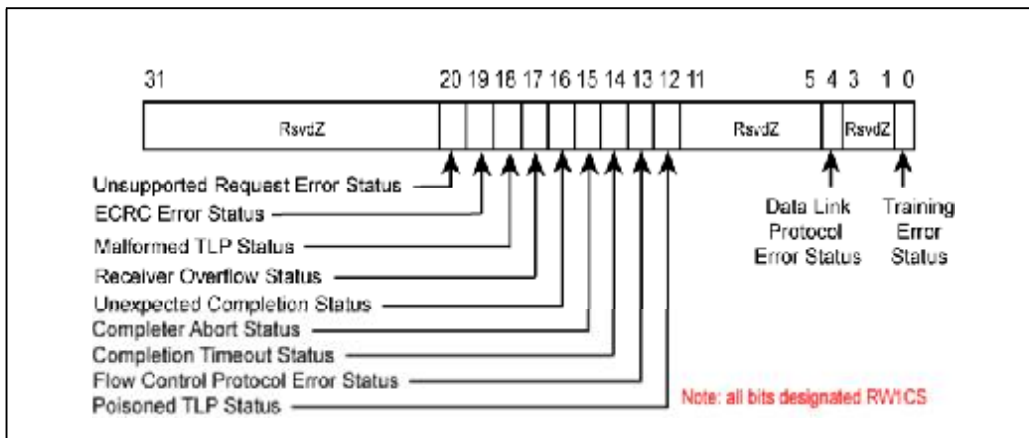
Figure 24-23: Advanced Error Uncorrectable Error Status Register
