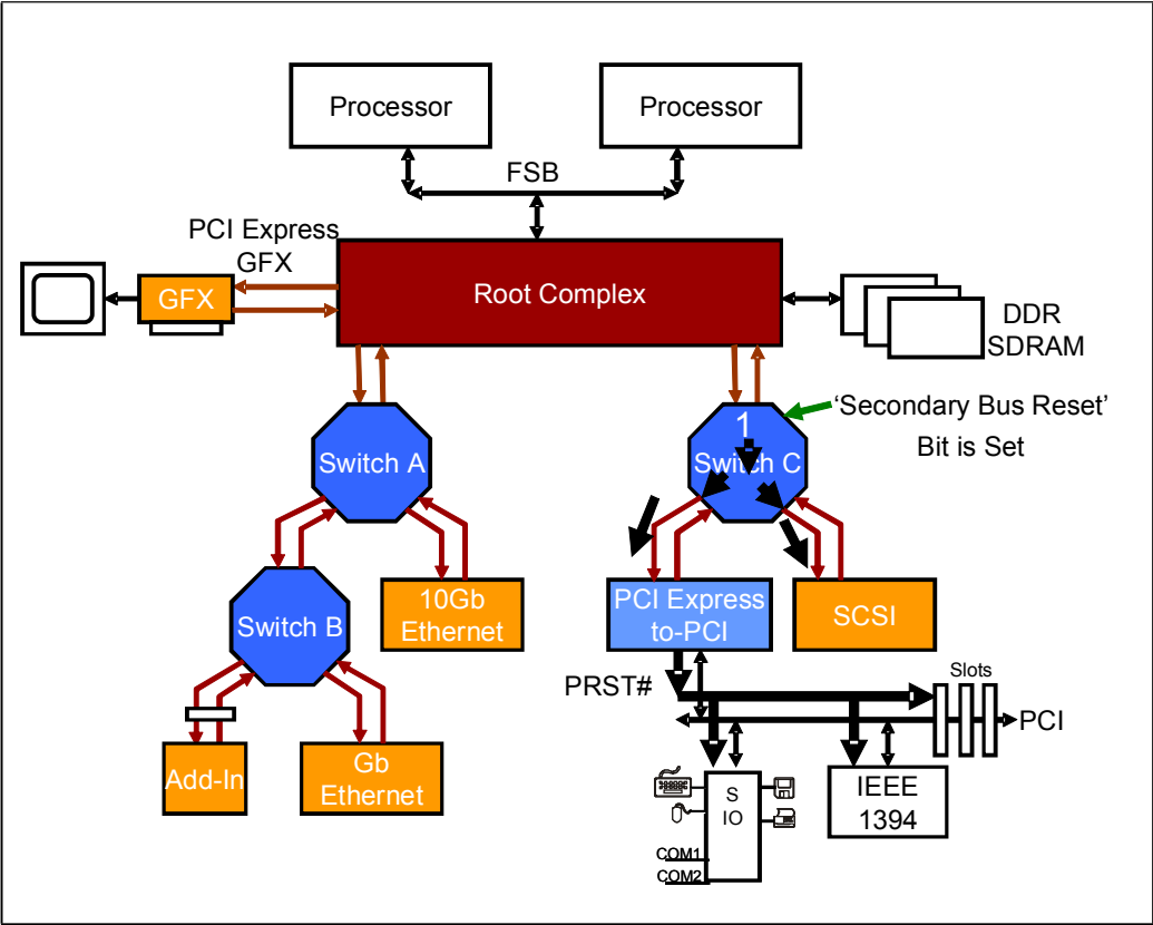
Figure 13-5: Switch Generates Hot Reset on All Downstream Ports
