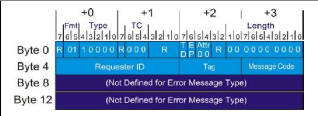
Figure 10-4: Basic Format of the Error Messages
