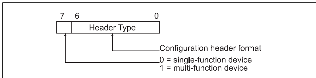
Figure 19-4: Header Type Register
