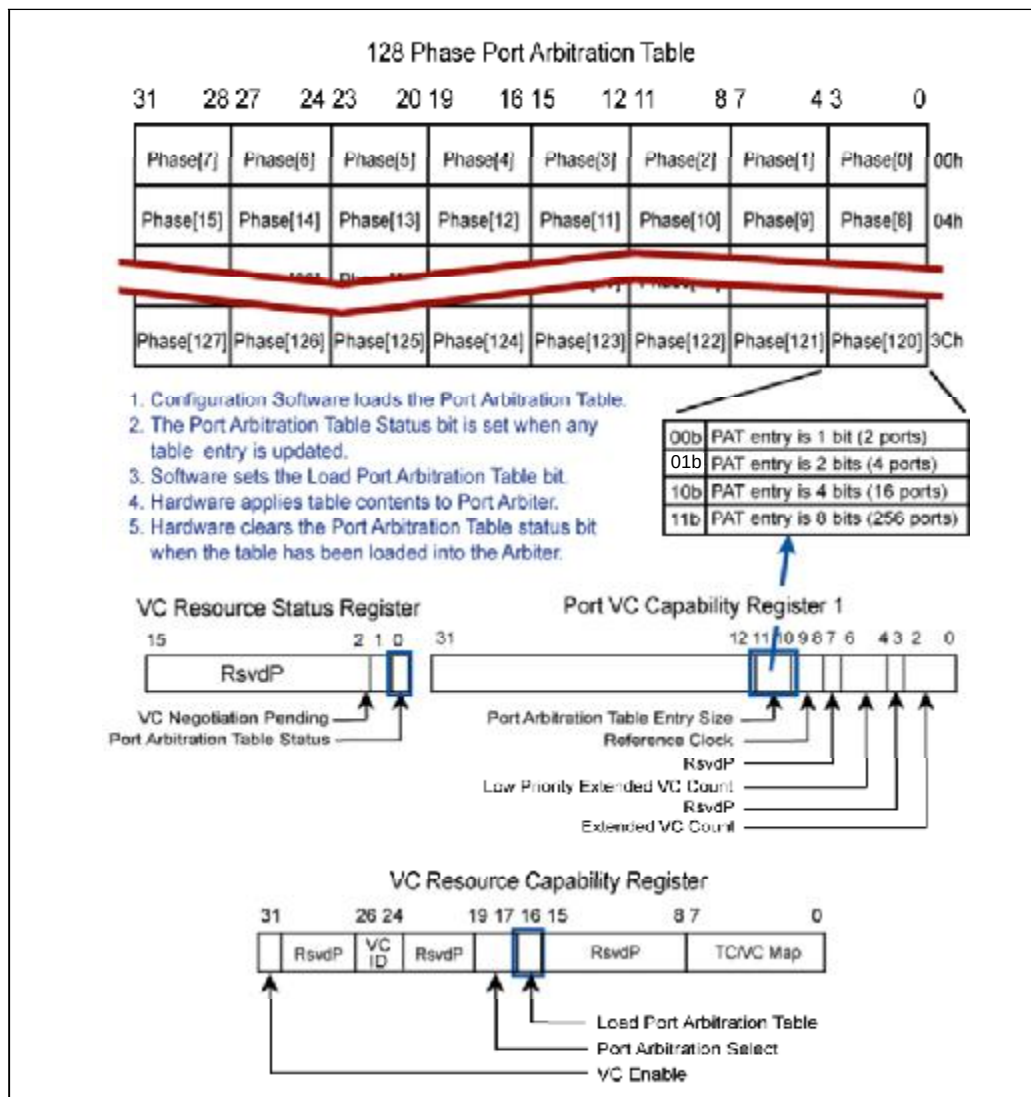
Figure 6-21: Format of Port Arbitration Table
