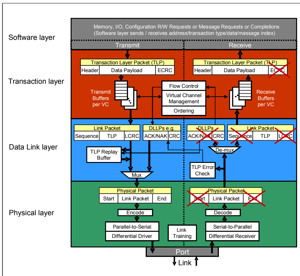
Figure 2-19: Detailed Block Diagram of PCI Express Device's Layers
