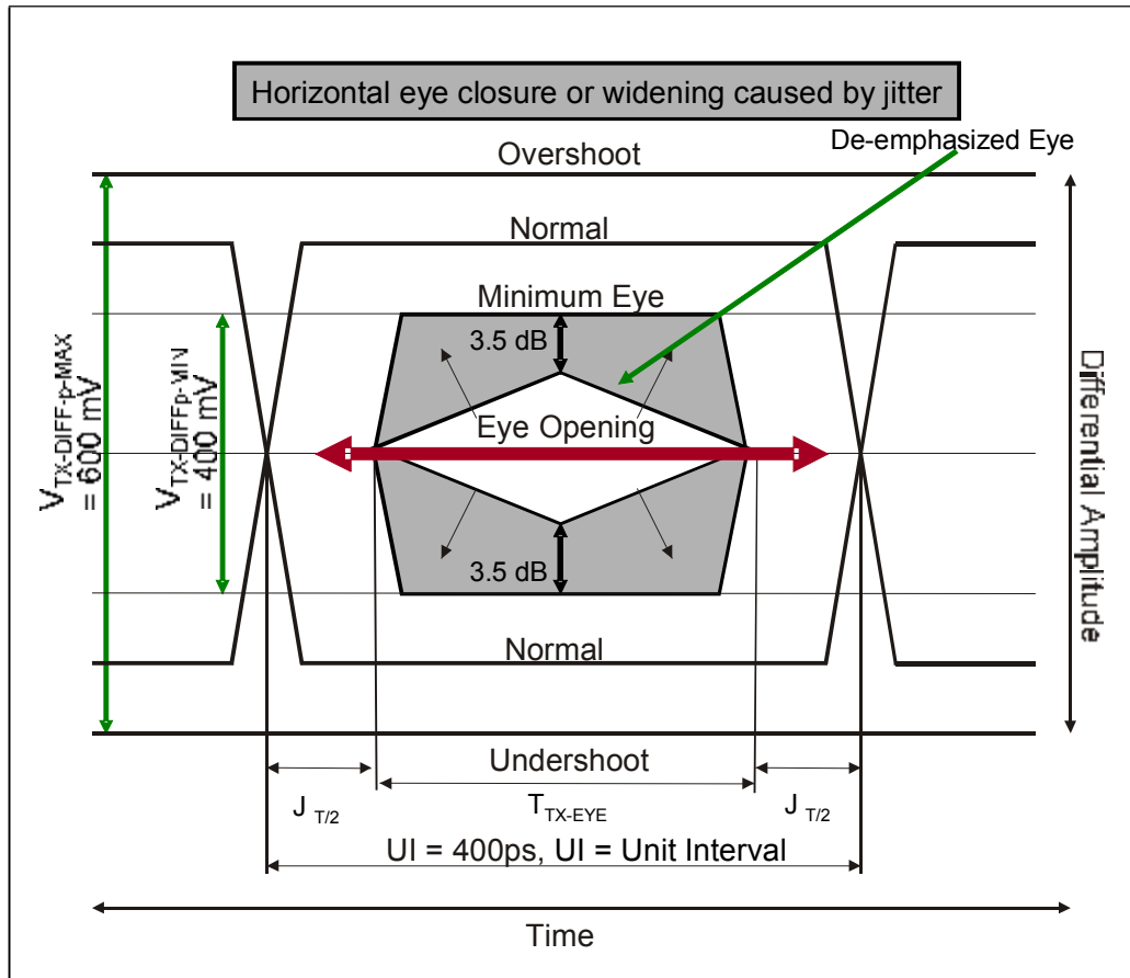
Figure 12-11: Transmitter Eye Diagram Jitter Indication
