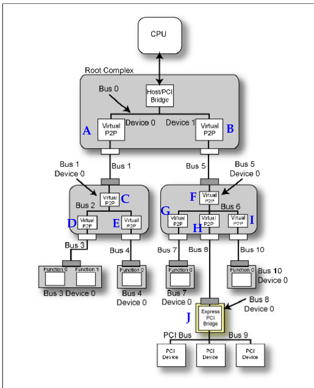
Figure 21-3: Example System After Bus Enumeration
