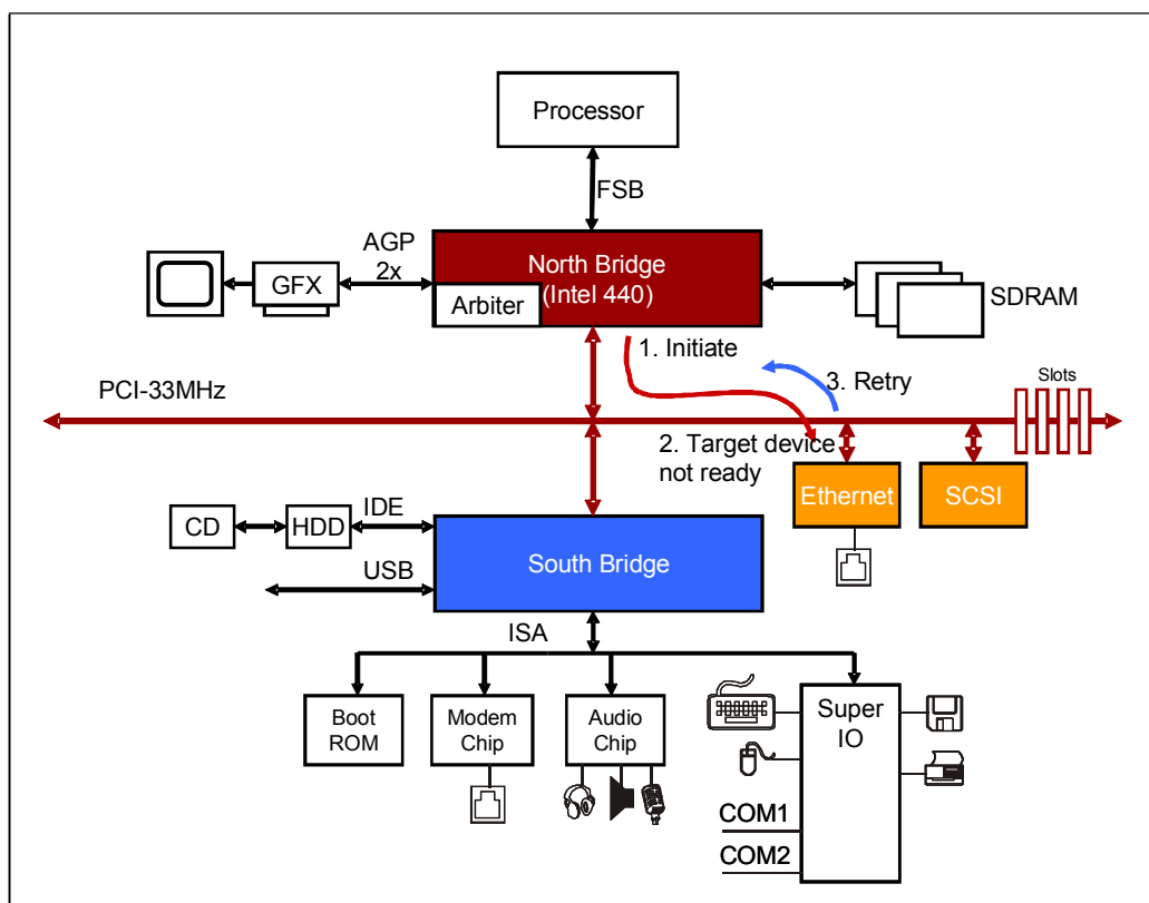
Figure 1-7: PCI Transaction Retry Mechanism
