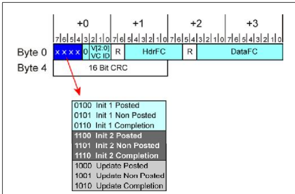
Figure 7-4: Types and Format of Flow Control Packets
