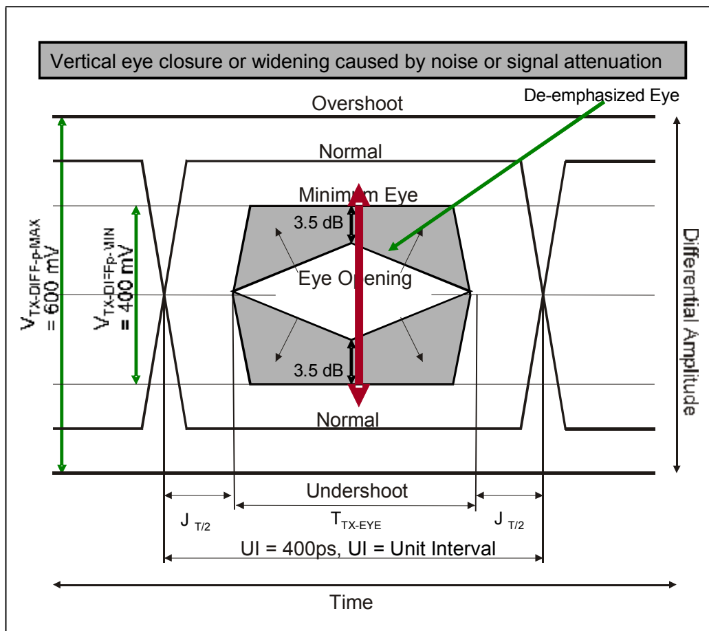
Figure 12-12: Transmitter Eye Diagram Noise/Attenuation Indication
