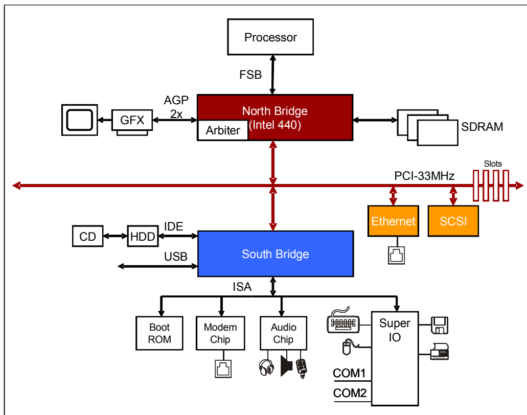
Figure 1-2: 33 MHz PCI Bus Based Platform
