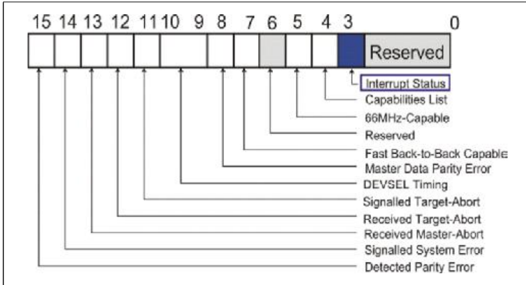
Figure 9-10: Configuration Status Register — Interrupt Status Field
