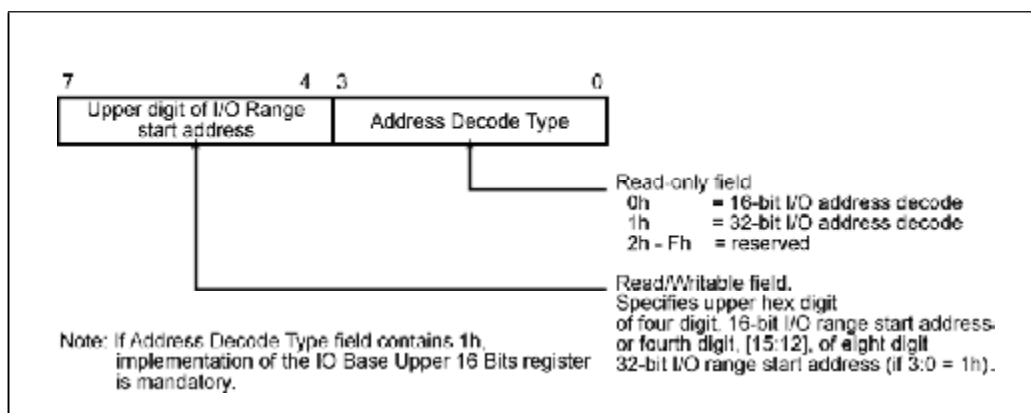
Figure 22-14: IO Base Register
