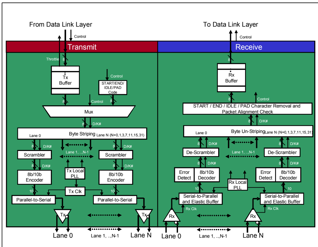
Figure 11-3: Physical Layer Details
