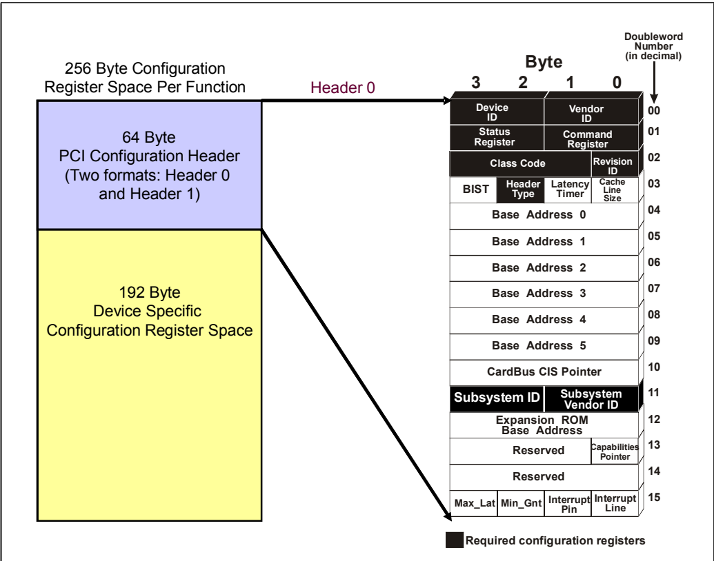
Figure 1-13: 256 Byte PCI Function Configuration Register Space
