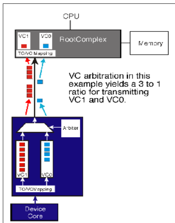
Figure 6-7: Conceptual VC Arbitration Example
