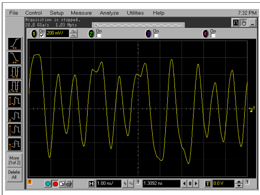
Figure A-2: PCI Express Serial Bit Stream
