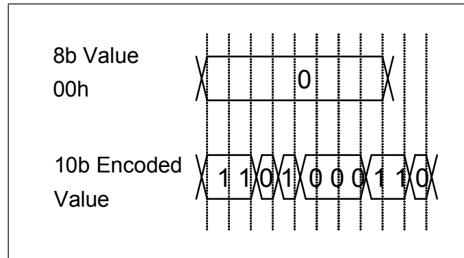
Figure 11-14: Example of 8-bit Character of 00h Encoded to 10-bit Symbol
