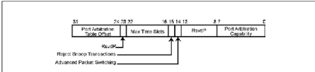
Figure 24-34: VC Resource Capability Register
