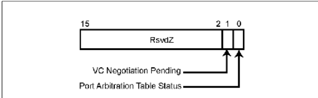
Figure 24-36: VC Resource Status Register (Read-Only)
