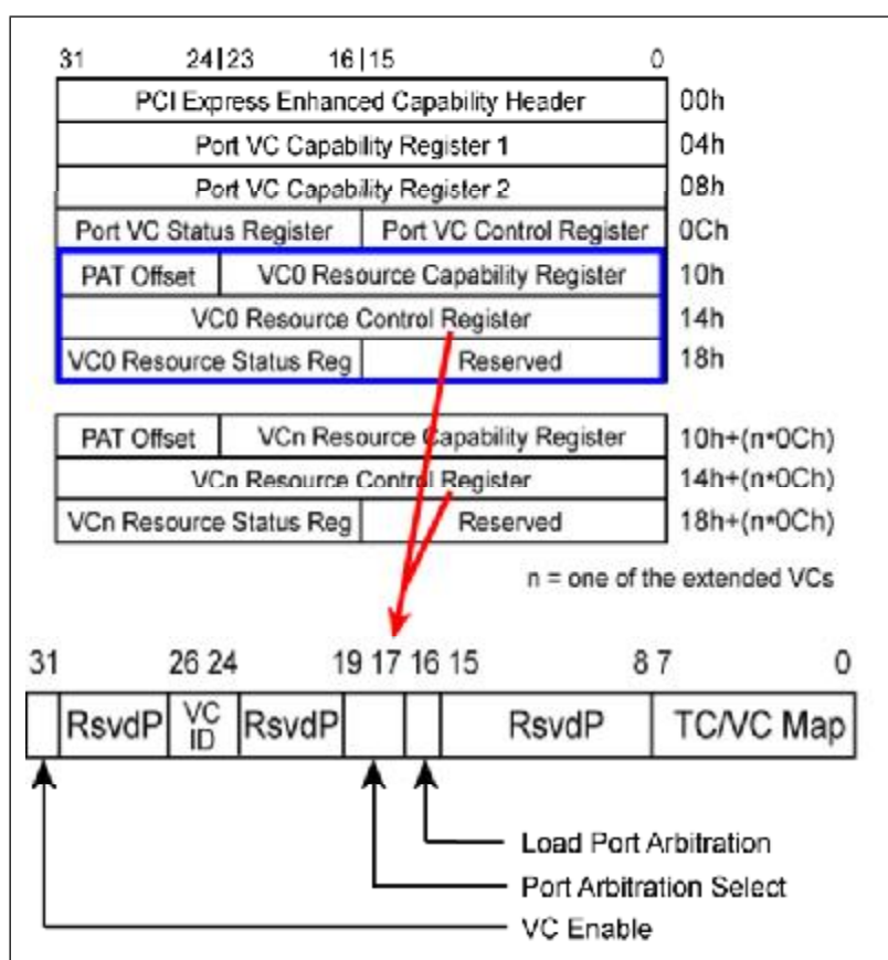
Figure 6-5: VC Resource Control Register
