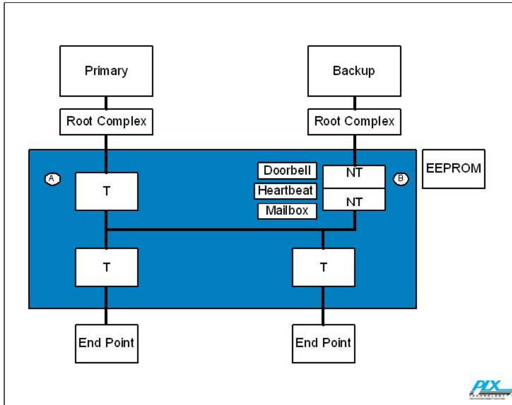
Figure C-5: Host Failover in PCI and PCI Express Systems
