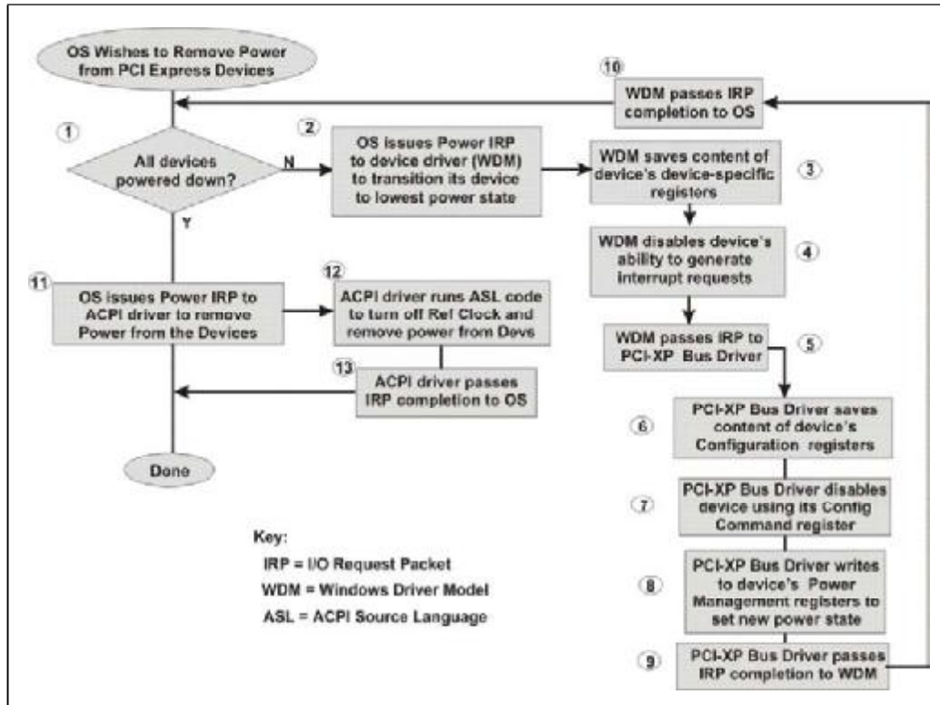
Figure 16-2: Example of OS Powering Down All Functions On PCI Express Links and then the Links Themselves
