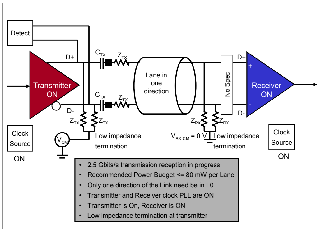
Figure 12-17: L0 Full-On Link State
