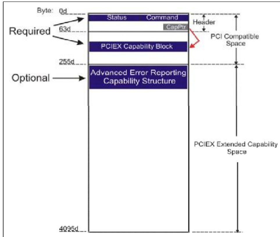
Figure 10-2: Location of PCI Express Error-Related Configuration Registers
