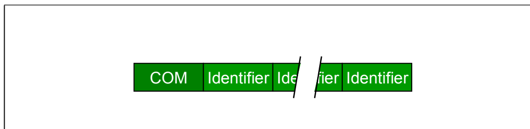
Figure 2-18: PLP or Ordered-Set Structure
