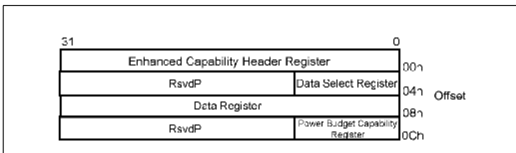
Figure 24-40: Power Budget Register Set
