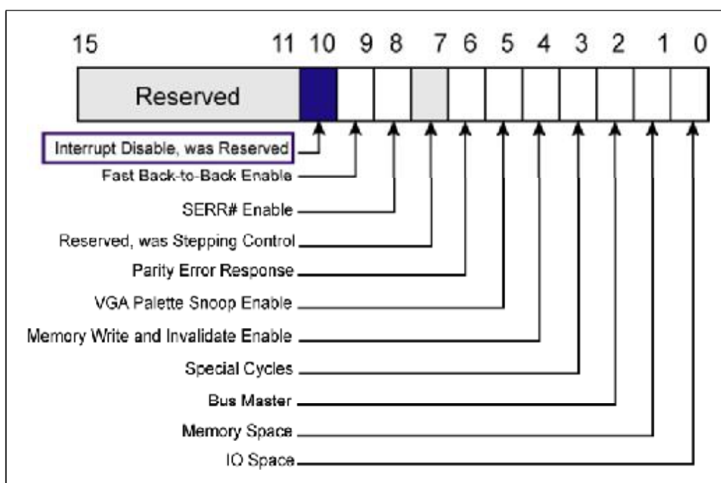
Figure 9-9: Configuration Command Register — Interrupt Disable Field
