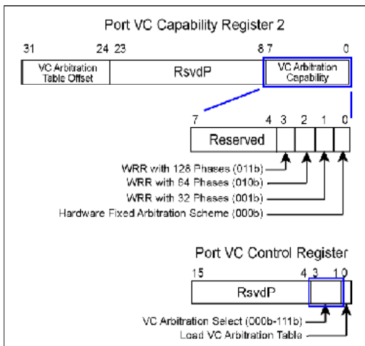
Figure 6-10: Determining VC Arbitration Capabilities and Selecting the Scheme
