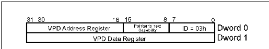
Figure 22-26: VPD Capability Registers
