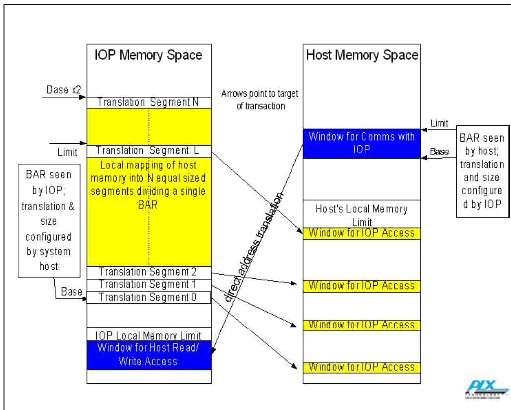
Figure C-3: Look Up Table Translation Creates Multiple Windows
