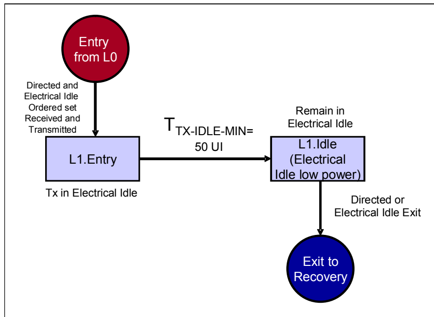
Figure 14-16: L1 State Machine
