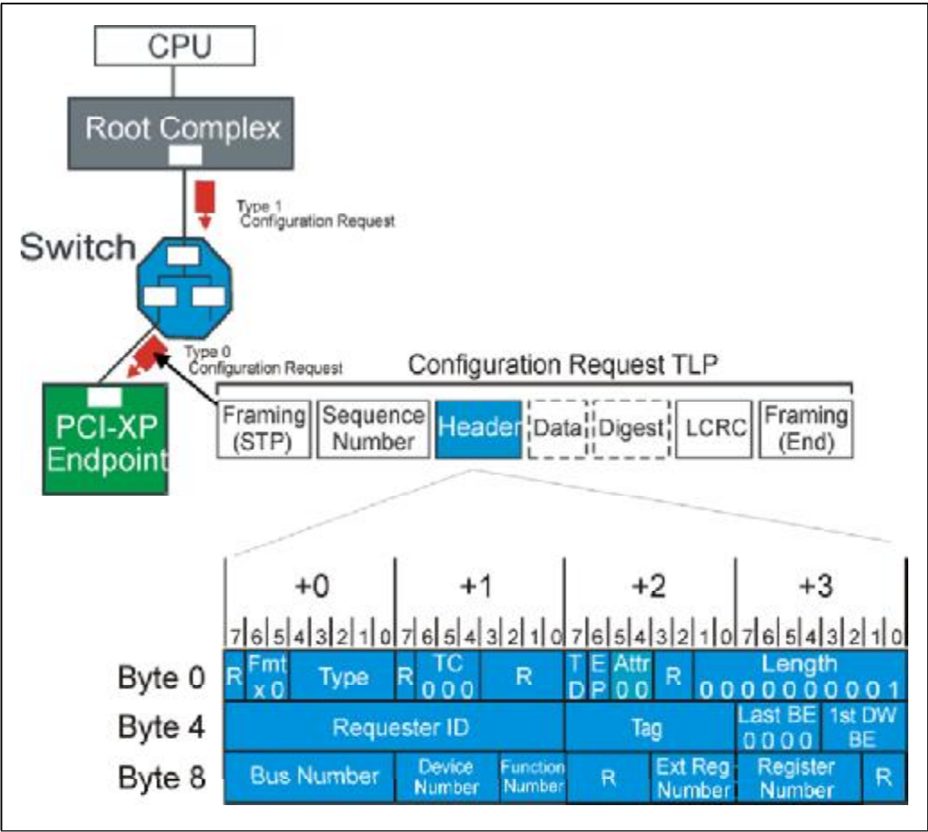
Figure 4-9: 3DW Configuration Request And Header Format
