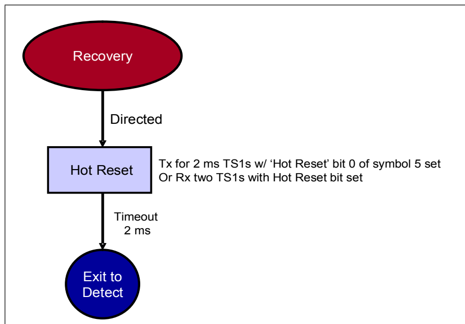
Figure 14-18: Hot Reset State Machine
