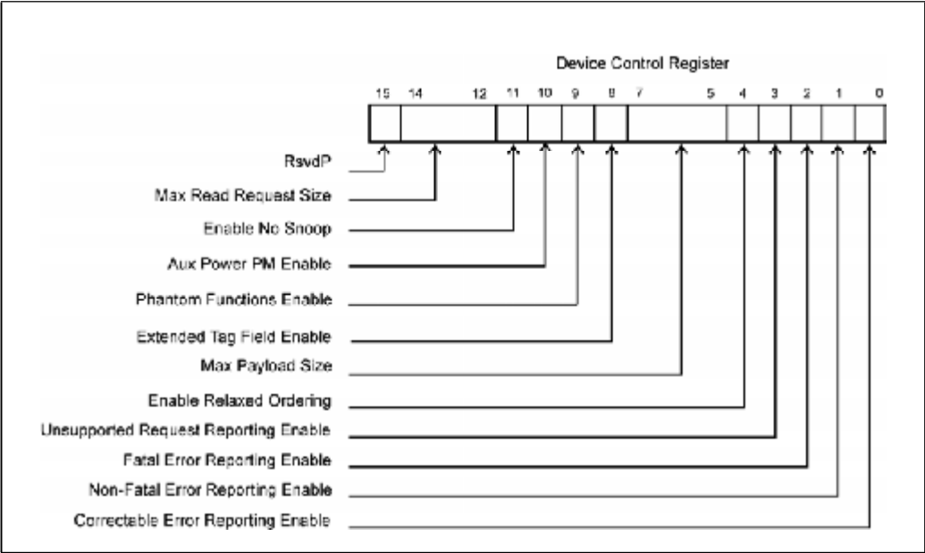
Figure 24-5: Device Control Register
