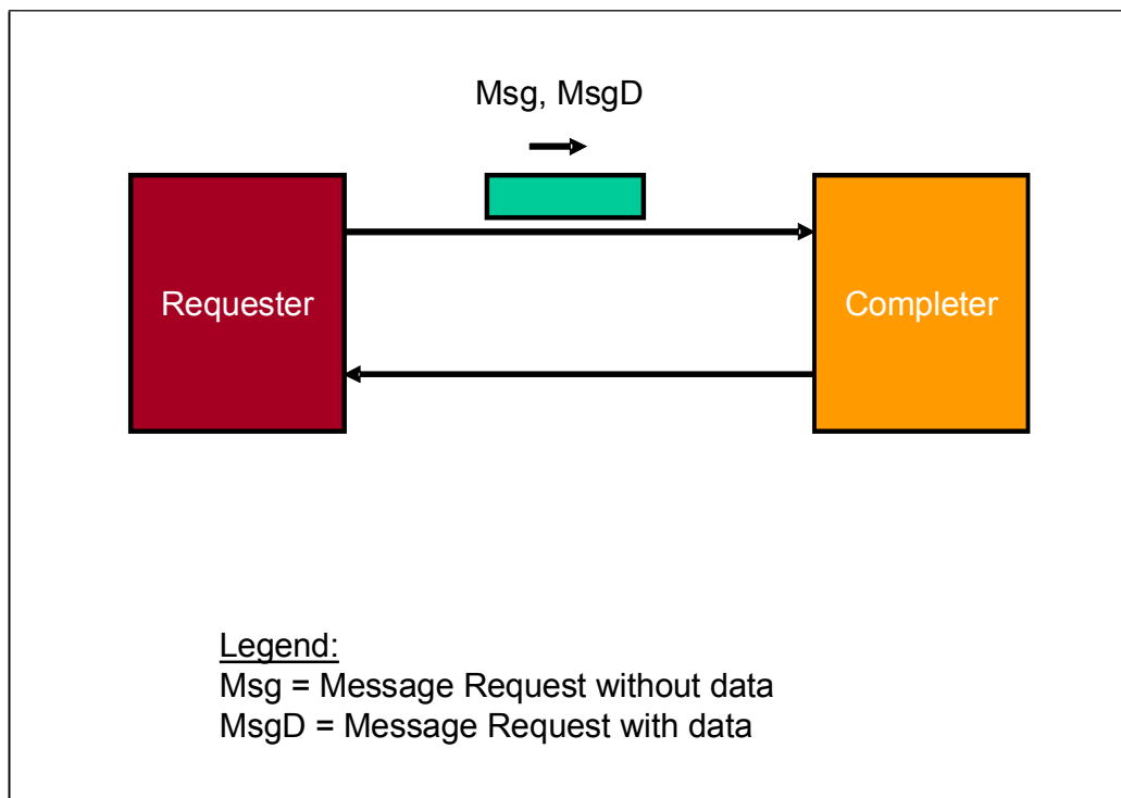
Figure 2-5: Posted Message Transaction Protocol
