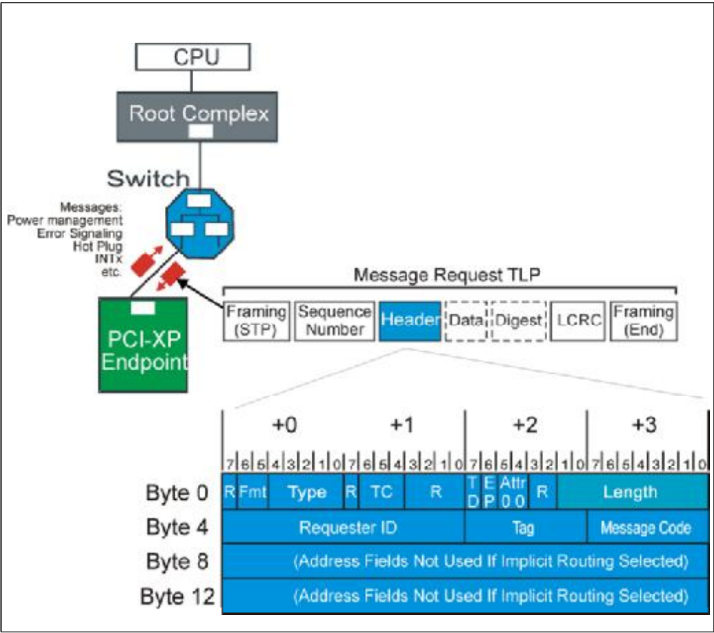
Figure 4-11: 4DW Message Request Header Format
