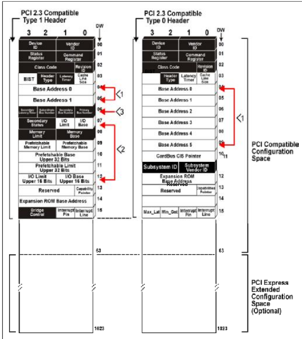
Figure 3-16: PCI Express Configuration Space Type 0 and Type 1 Headers
