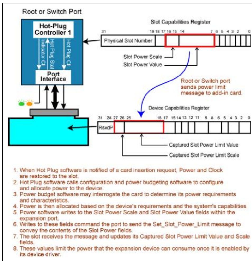
Figure 15-3: Slot Power Limit Sequence
