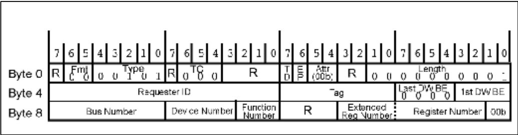
Figure 20-7: Type 1 Configuration Read Request Packet Header
