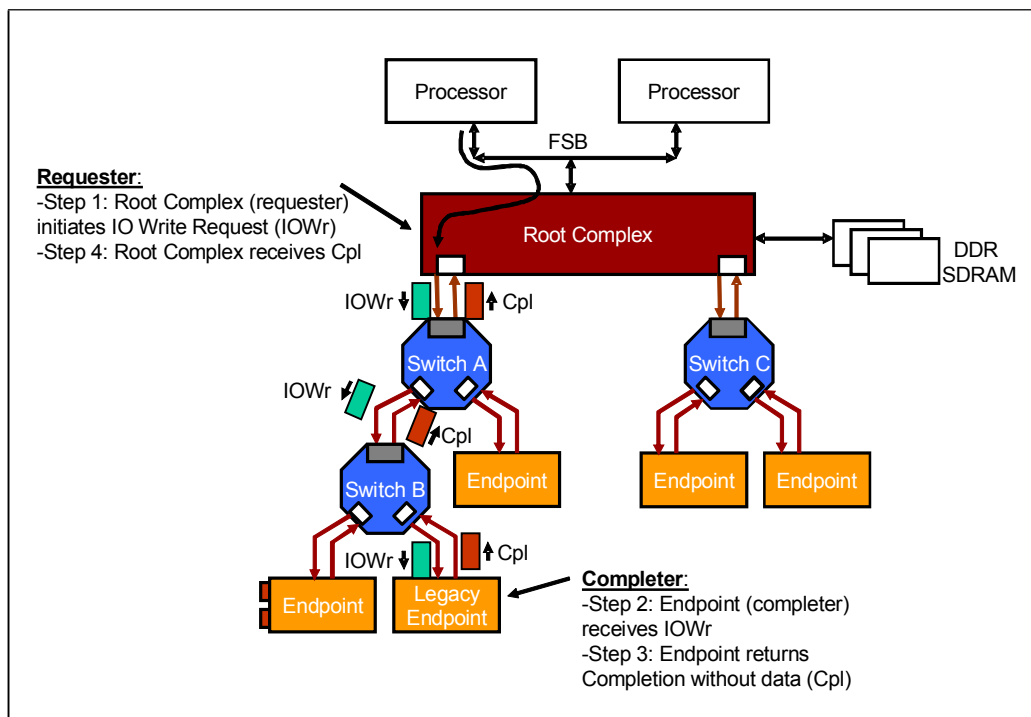
Figure 2-8: IO Write Transaction Originated by CPU, Targeting Legacy Endpoint
