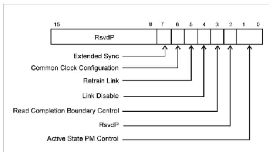
Figure 14-23: Link Control Register
