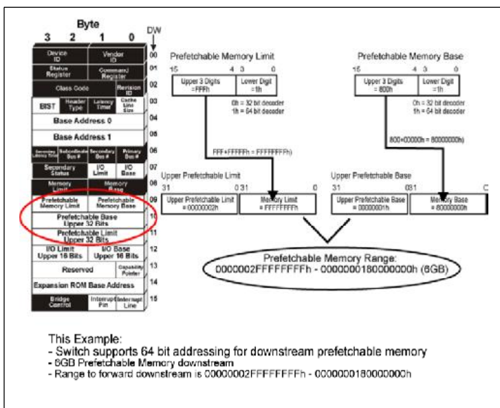
Figure 3-20: 6GB, 64-Bit Prefetchable Memory Base/Limit Register Set Up
