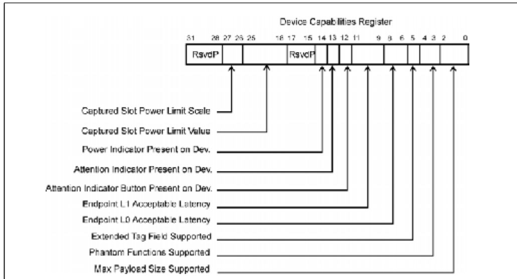
Figure 24-4: Device Capabilities Register
