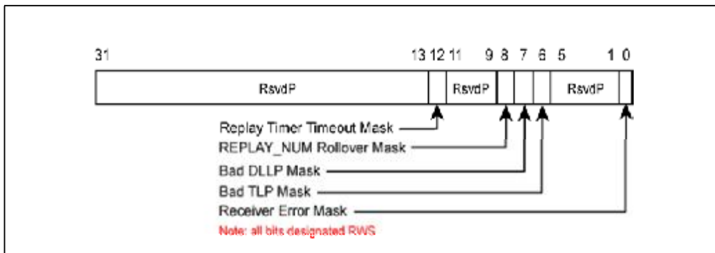
Figure 24-19: Advanced Error Correctable Error Mask Register
