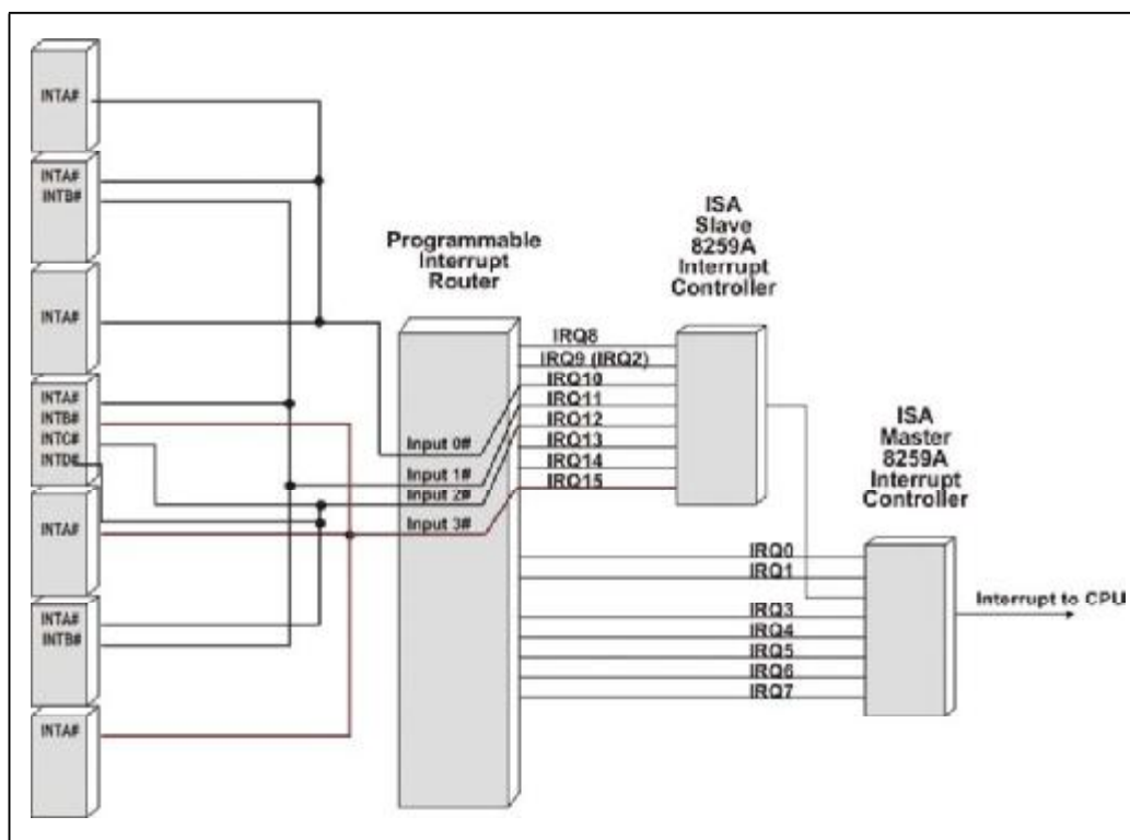
Figure 9-8: INTx Signal Routing is Platform Specific
