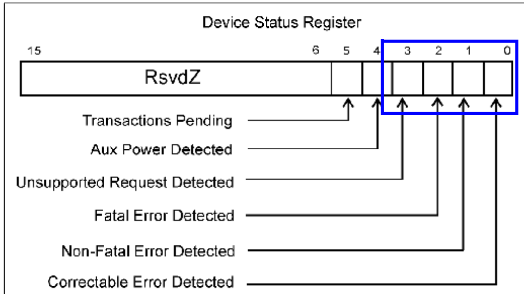
Figure 10-10: Device Status Register Bit Fields Related to Error Handling
