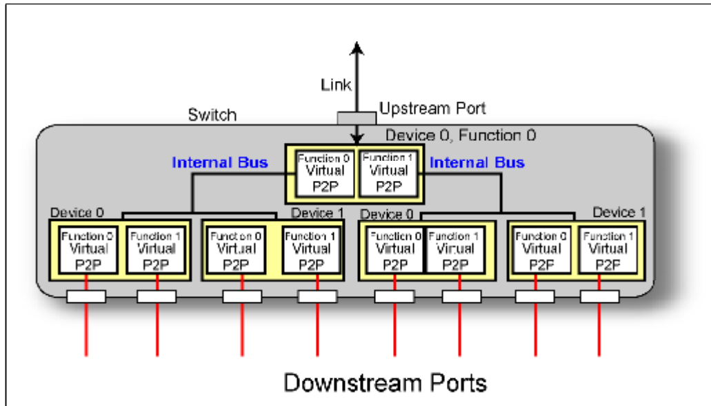
Figure 21-11: Second Example of a Multifunction Bridge In a Switch
