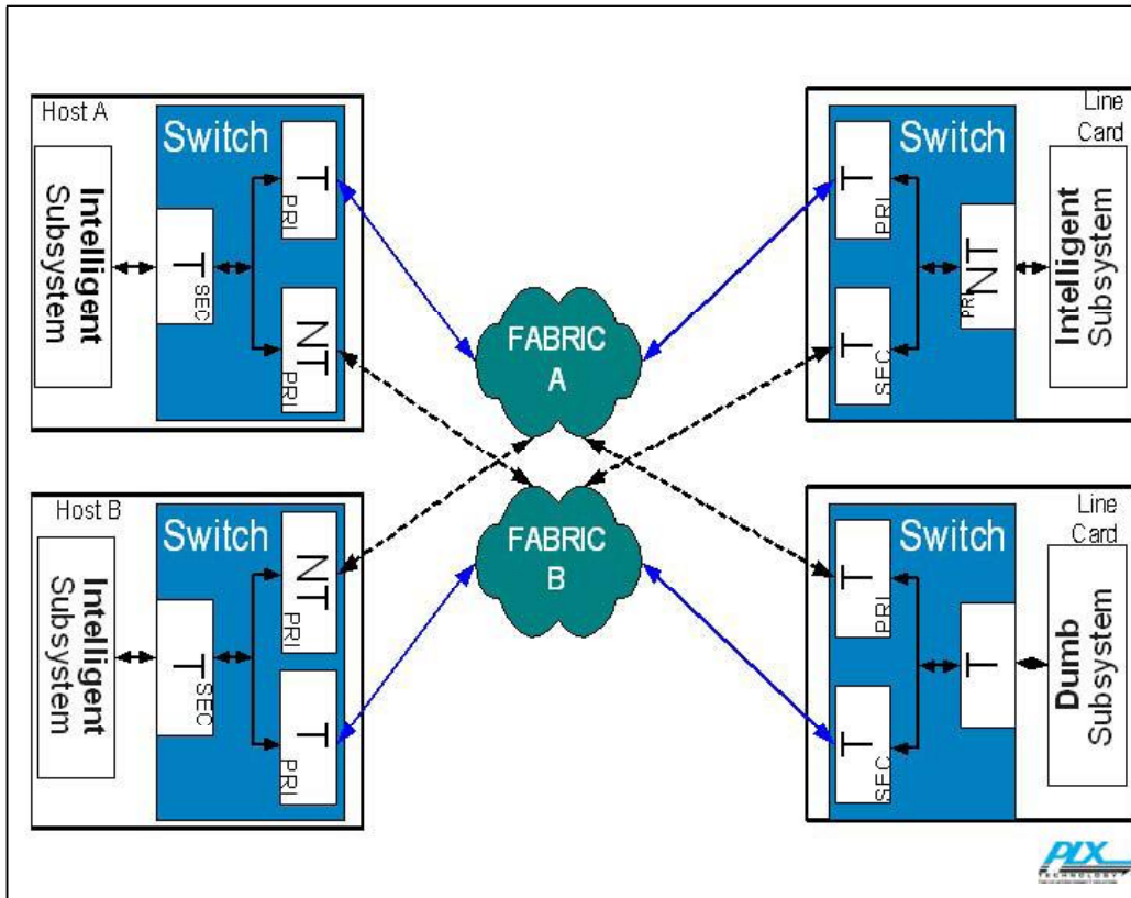
Figure C-7: Dual-Star Fabric
