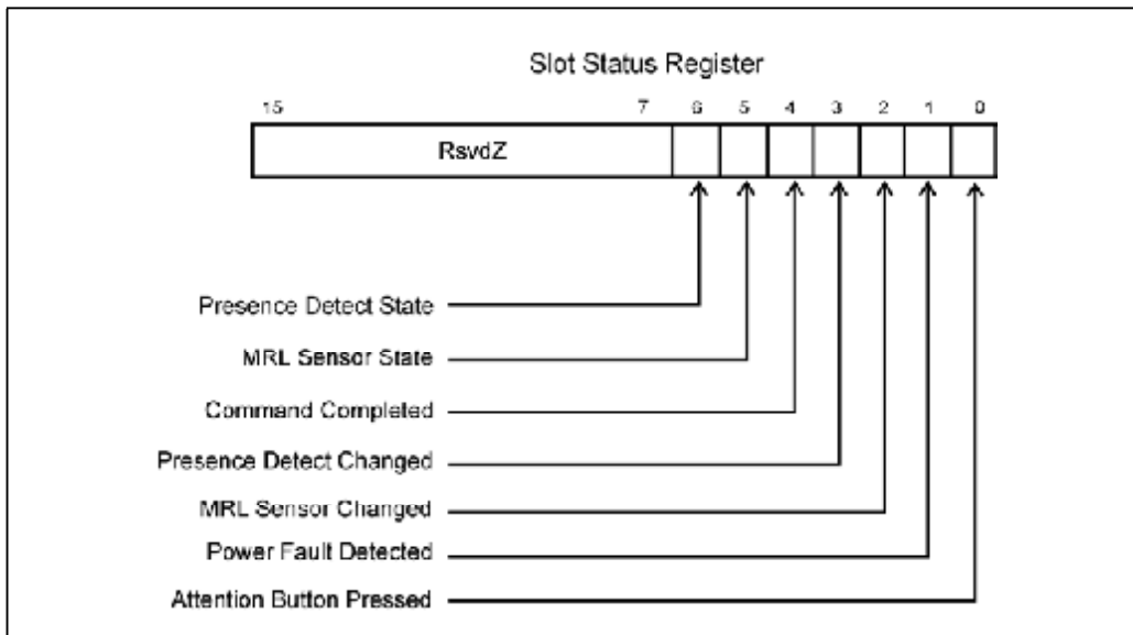
Figure 24-12: Slot Status Register
