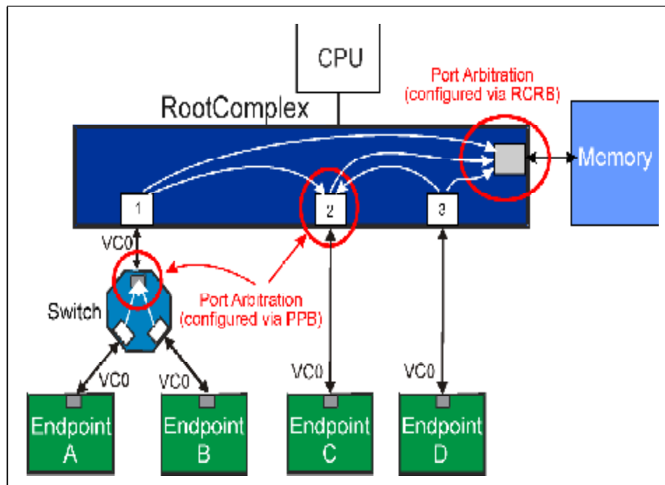
Figure 6-16: Port Arbitration Concept
