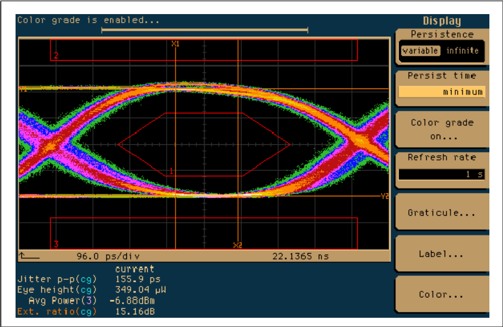
Figure 12-13: Screen Capture of a Normal Eye (With no De-emphasis Shown)
