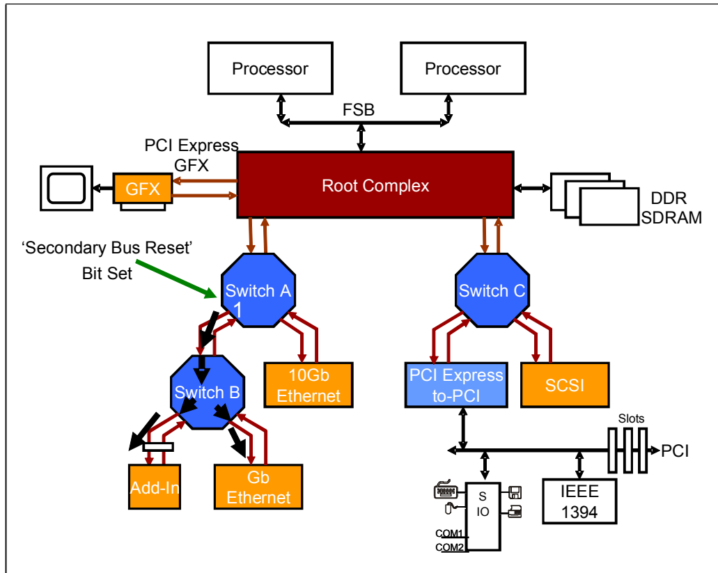
Figure 13-4: Switch Generates Hot Reset on One Downstream Port
