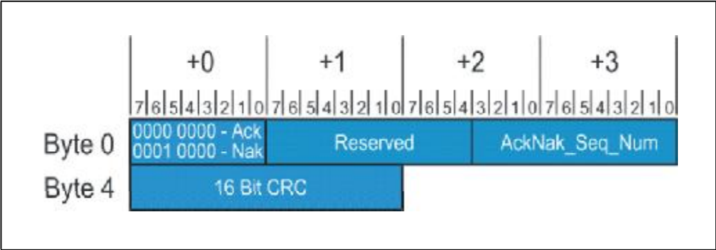
Figure 4-14: Ack Or Nak DLLP Packet Format
