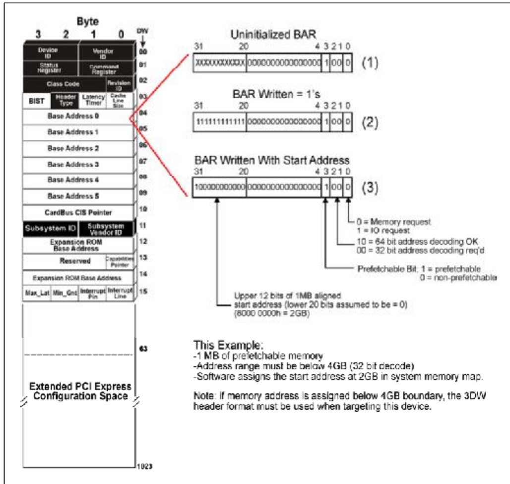
Figure 3-17: 32-Bit Prefetchable Memory BAR Set Up
