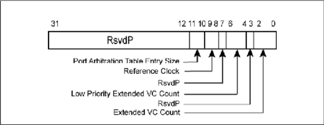
Figure 24-30: Port VC Capability Register 1 (Read-Only)
