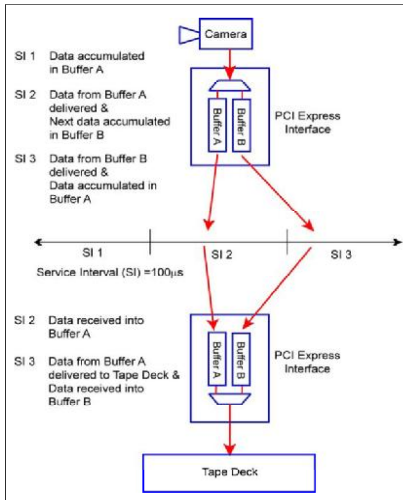
Figure 6-1: Example Application of Isochronous Transaction
