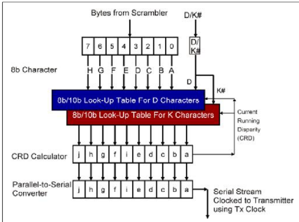
Figure 11-16: 8-bit to 10-bit (8b/10b) Encoder
