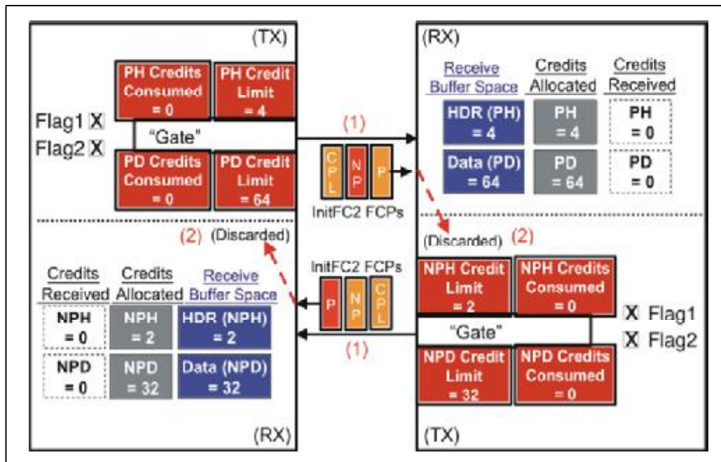
Figure 7-12: Device Confirm that Flow Control Initialization is Completed for a Given Buffer
