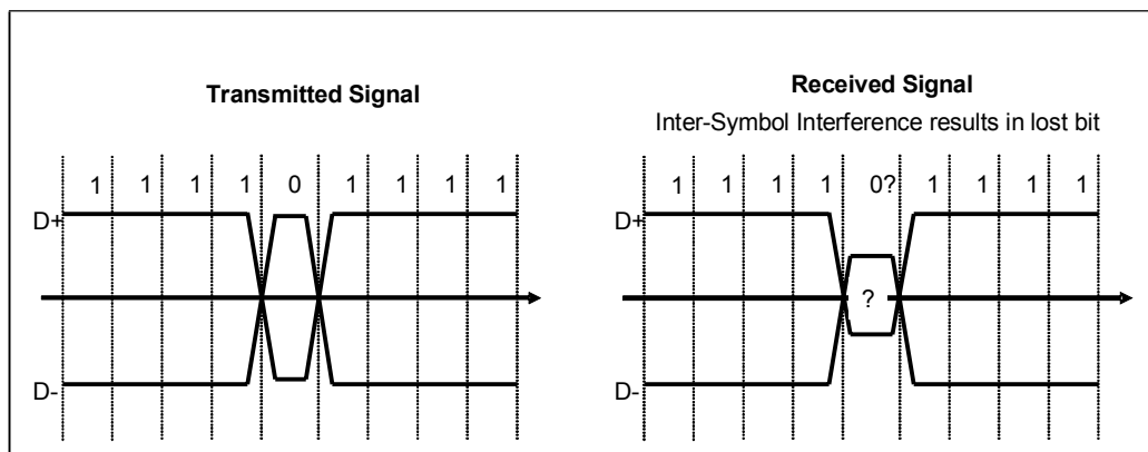
Figure 12-8: Problem of Inter-Symbol Interference
