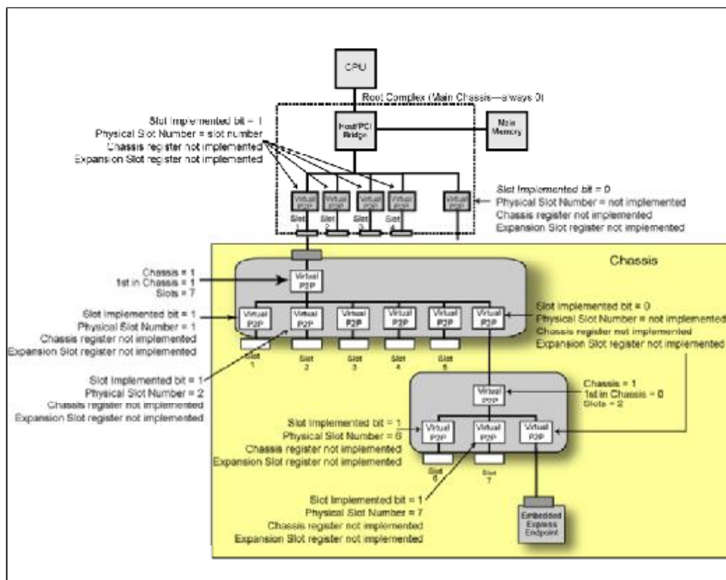
Figure 22-33: Chassis Example Two
