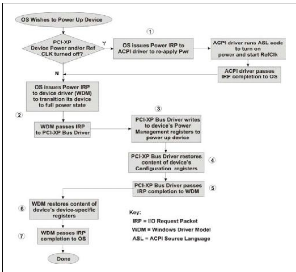
Figure 16-3: Example of OS Restoring a PCI Express Function To Full Power
