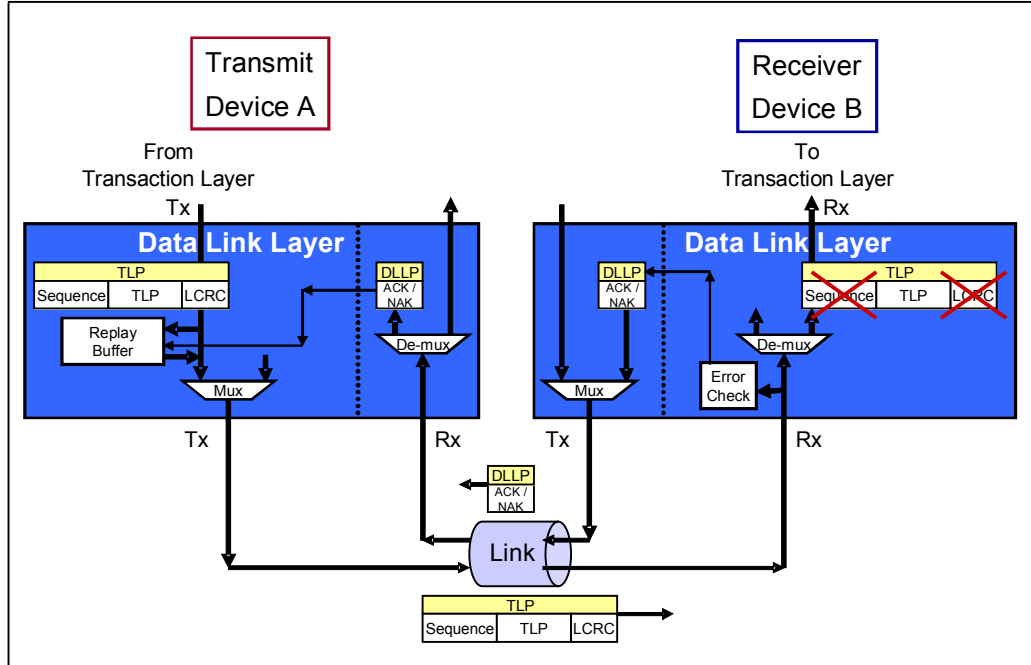
Figure 5-2: Overview of the ACK/NAK Protocol
