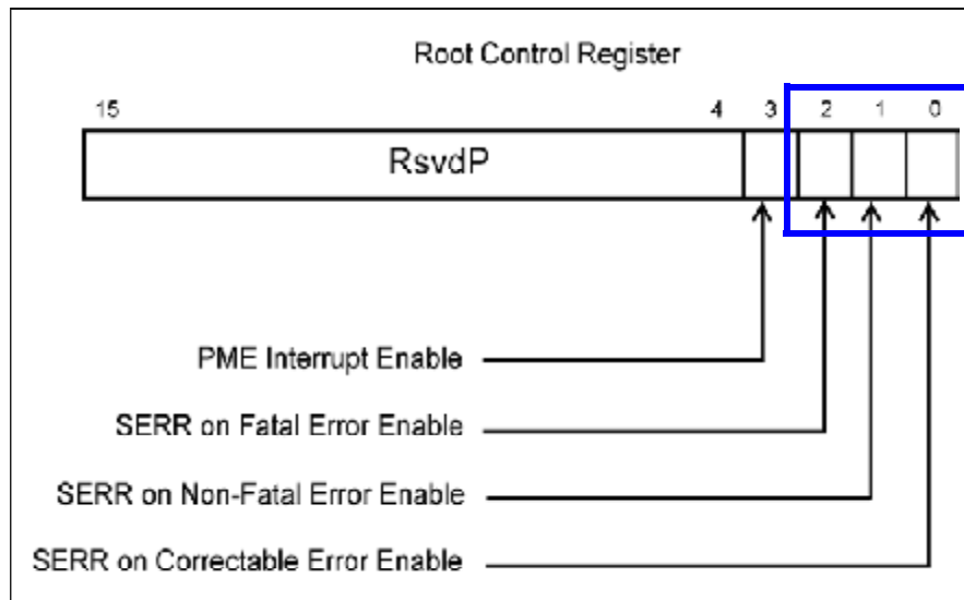
Figure 10-13: Root Control Register
