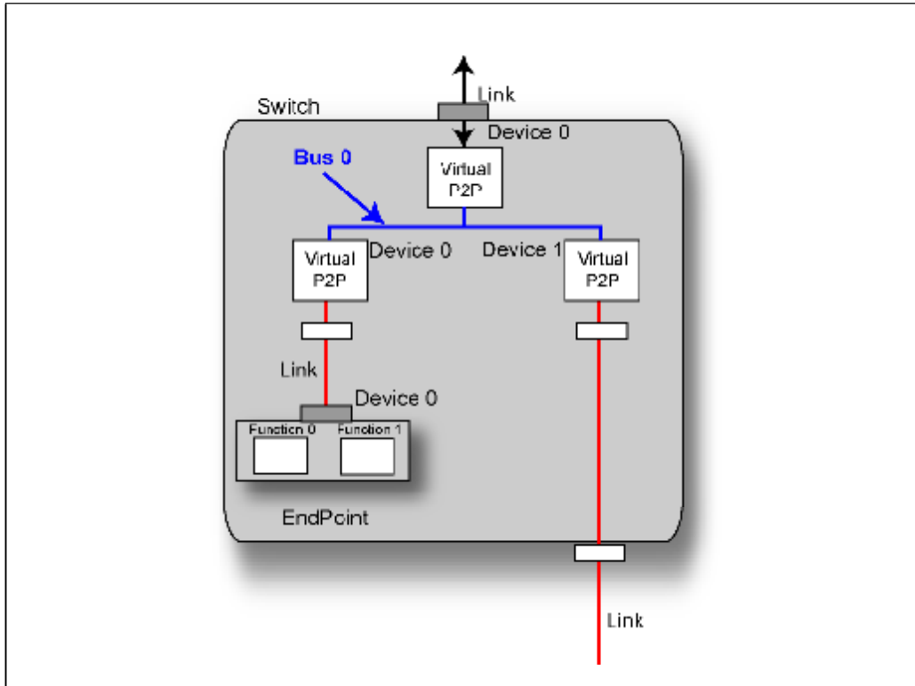
Figure 21-13: Embedded Switch Endpoint
