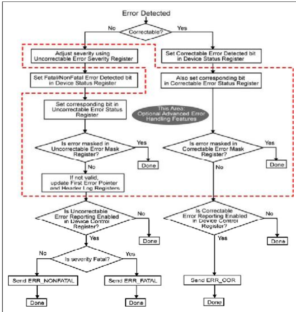
Figure 10-24: Error Handling Flow Chart
