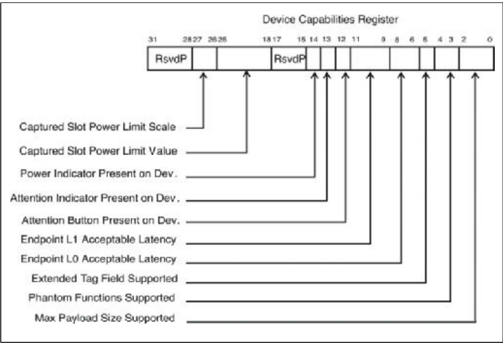
Figure 17-9: Hot-Plug Capability Bits for Server IO Modules
