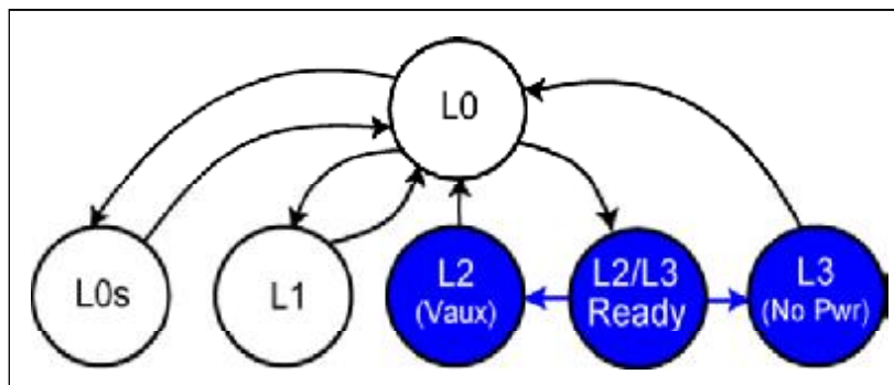
Figure 16-26: State Transitions from L2/L3 Ready When Power is Removed
