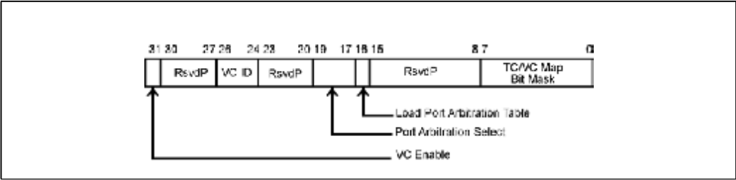
Figure 24-35: VC Resource Control Register (Read-Write)
