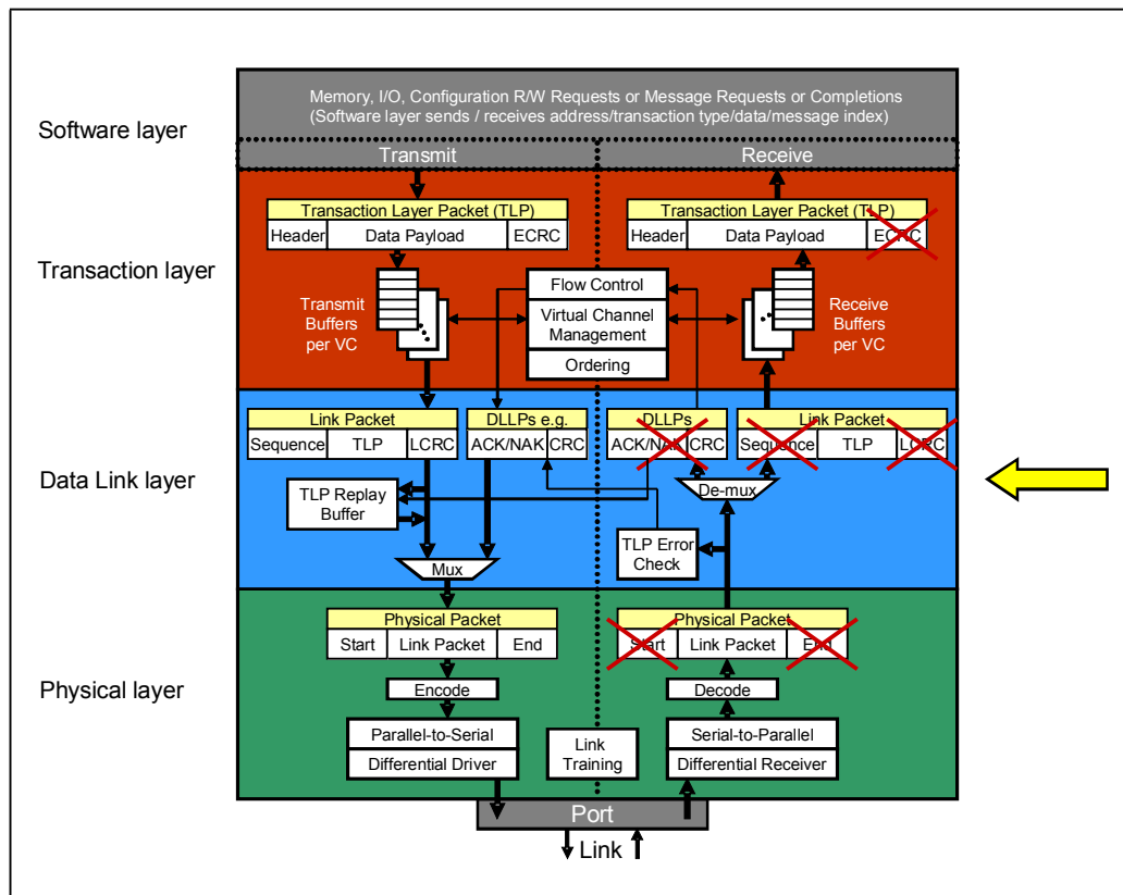
Figure 5-1: Data Link Layer
