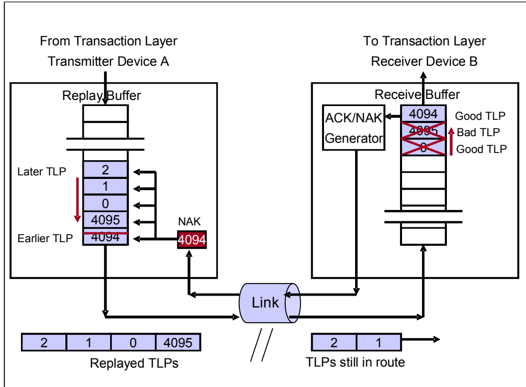
Figure 5-12: Example that Shows Receiver Behavior When It Receives Bad TLPs
