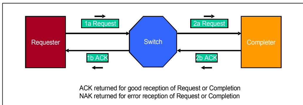
Figure 2-28: Posted Transaction on Link
