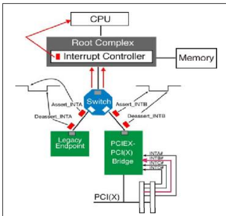
Figure 9-11: Legacy Devices use INTx Messages to Virtualize INTA#-INTD# Signal Transitions
