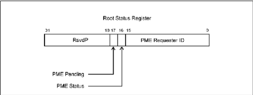
Figure 24-14: Root Status Register
