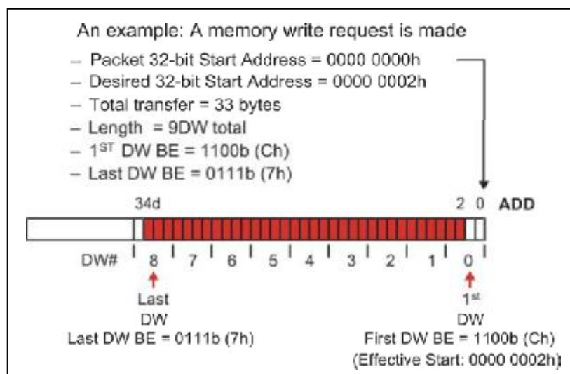
Figure 4-4: Using First DW and Last DW Byte Enable Fields
