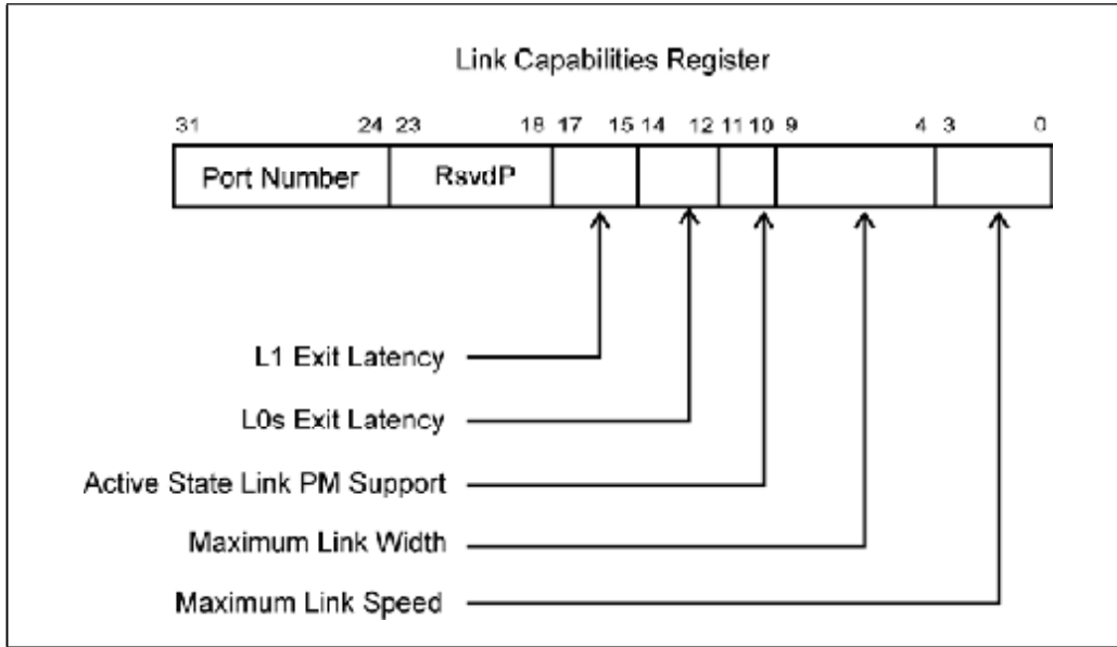
Figure 24-7: Link Capabilities Register
