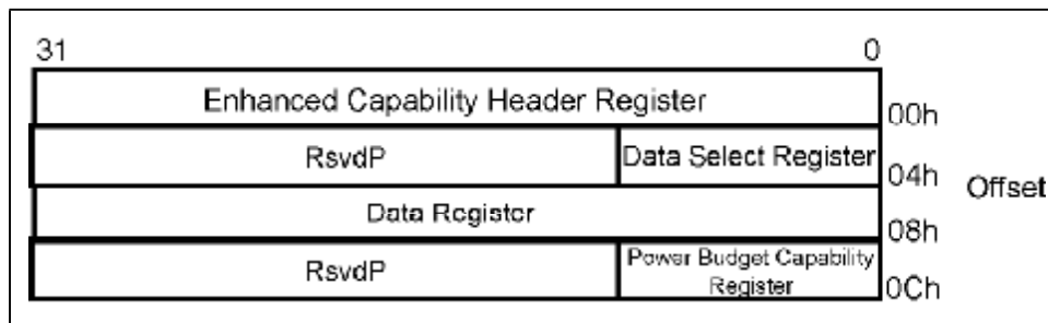
Figure 15-4: Power Budget Capability Registers
