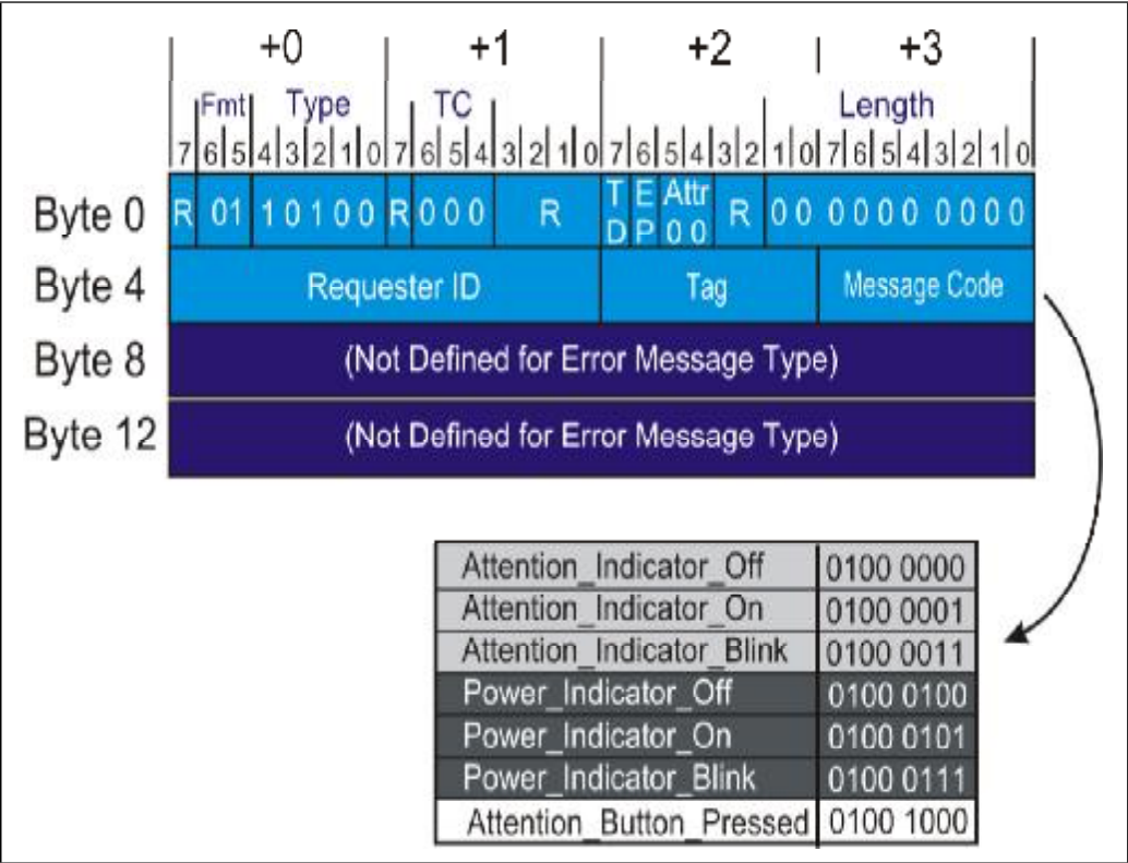
Figure 17-10: Hot Plug Message Format
