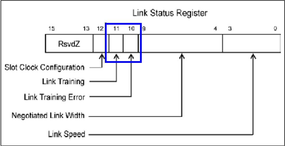
Figure 10-12: Link Retraining Status Bits within the Link Status Register
