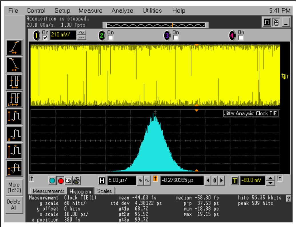
Figure A-20: Jitter Analysis of a Transceiver source clock—Acceptable (for a specific device)
