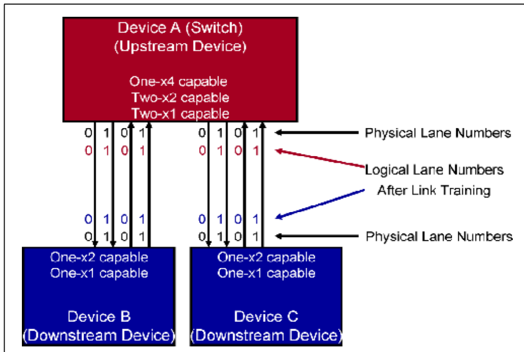
Figure 14-11: Example 2 Link Numbering and Lane Numbering
