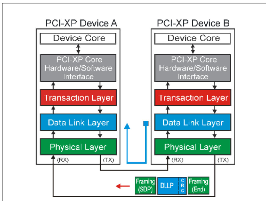
Figure 4-12: Data Link Layer Sends A DLLP
