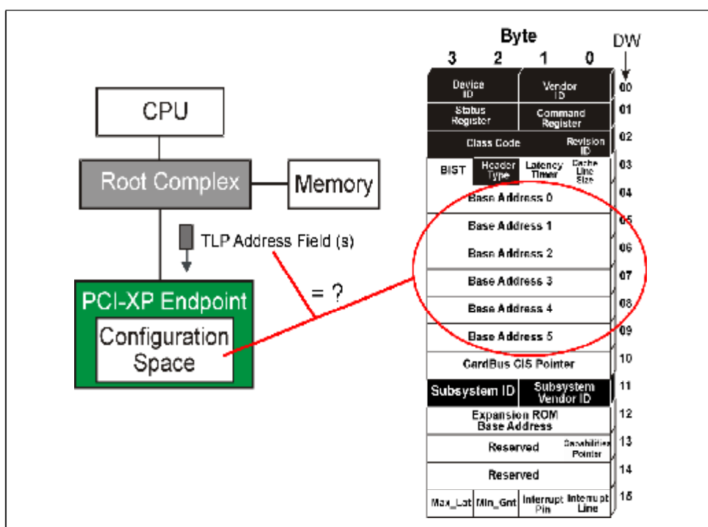
Figure 3-9: Endpoint Checks Routing Of An Inbound TLP Using Address Routing
