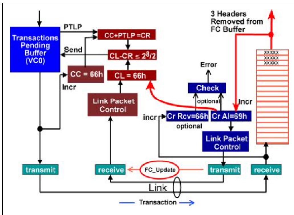
Figure 7-13: Flow Control Update Example
