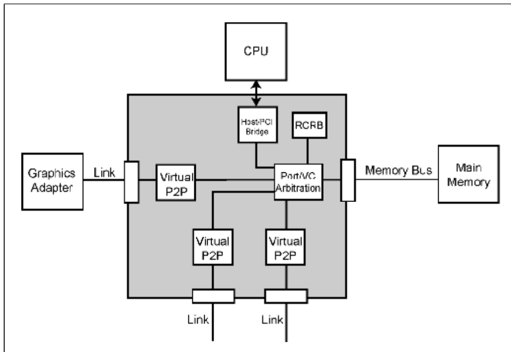
Figure 21-15: RCRB Example
