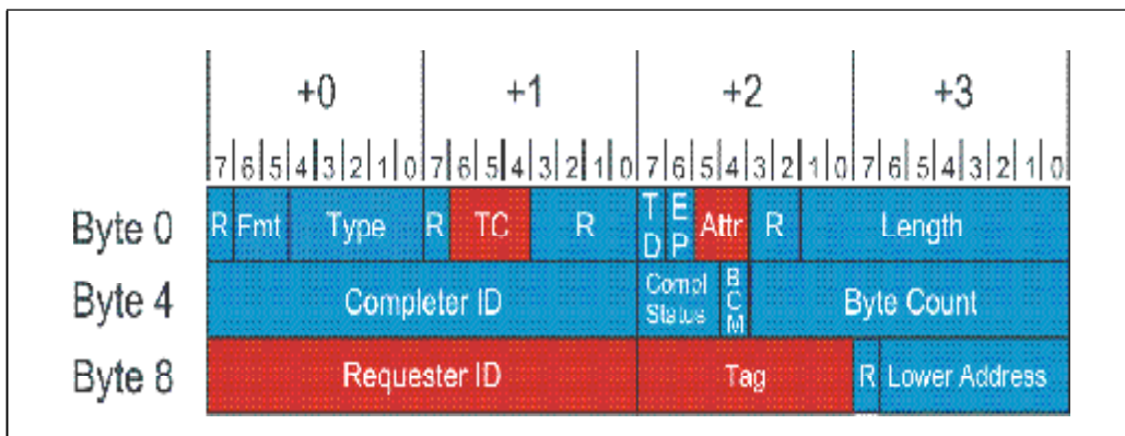
Figure 4-5: Transaction Descriptor Fields
