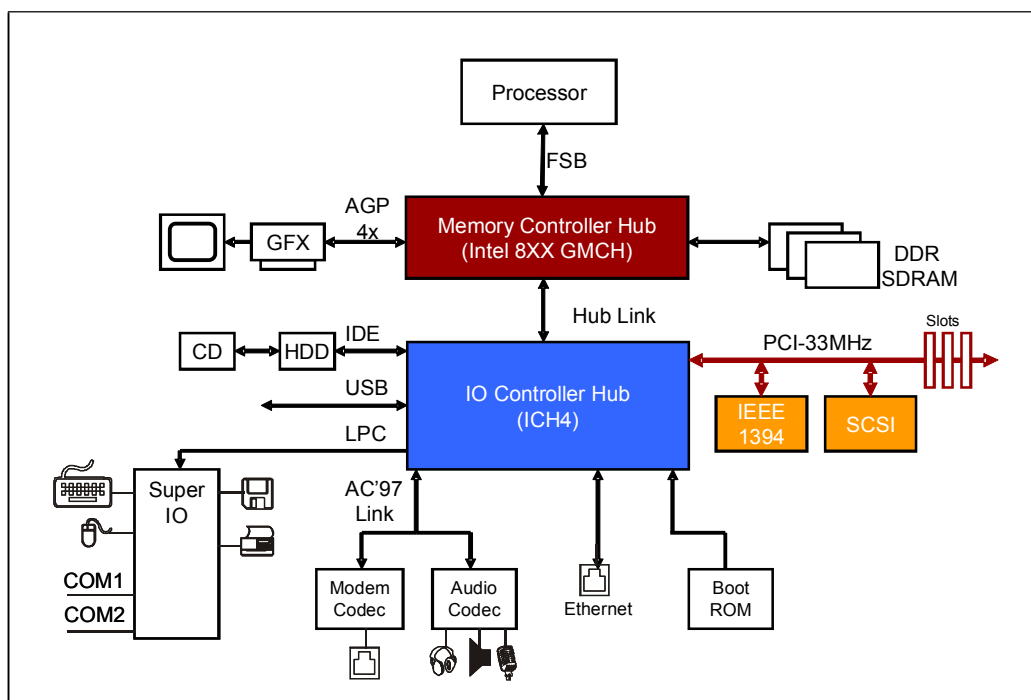
Figure 1-14: Latest Generation of PCI Chipsets
