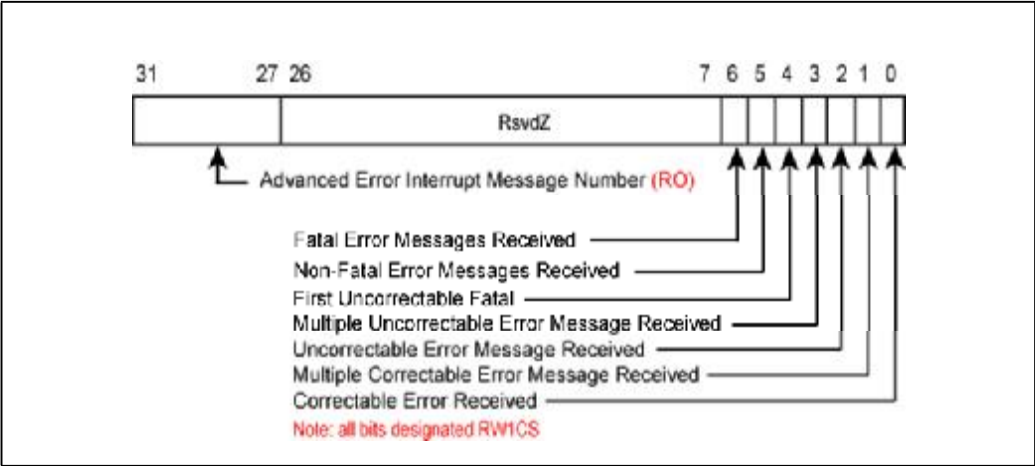
Figure 24-25: Advanced Error Root Error Status Register
