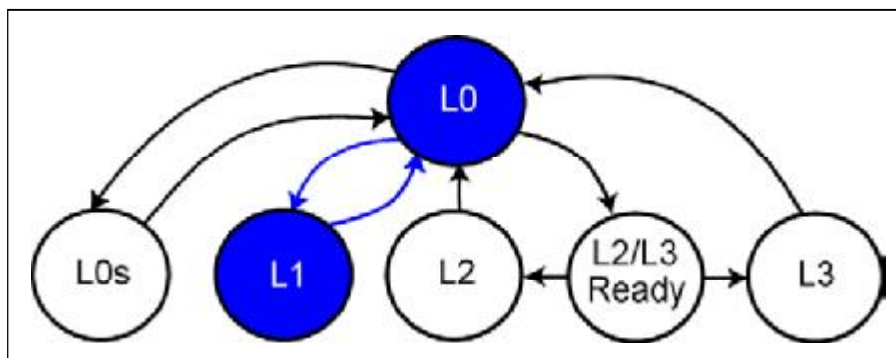
Figure 16-21: Devices Transition to L1 When Software Changes their Power Level from D0
