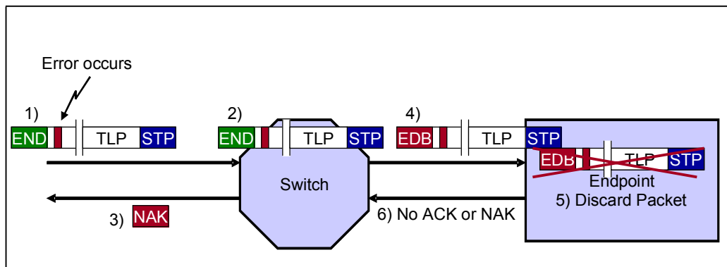
Figure 5-17: Switch Cut-Through Mode Showing Error Handling
