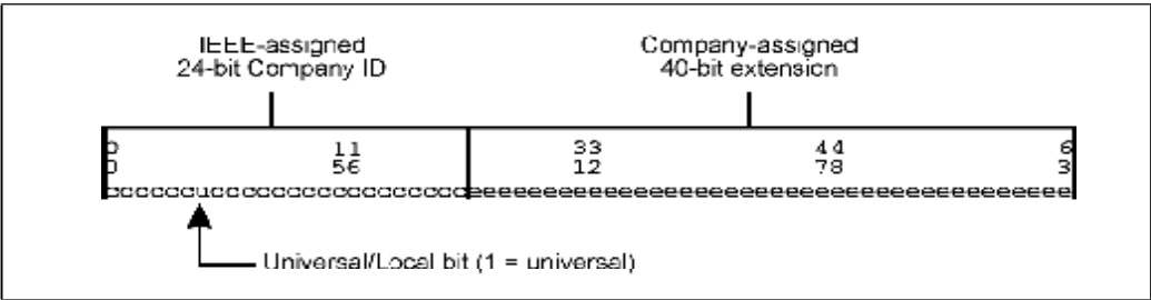
Figure 24-39: EUI-64 Format
