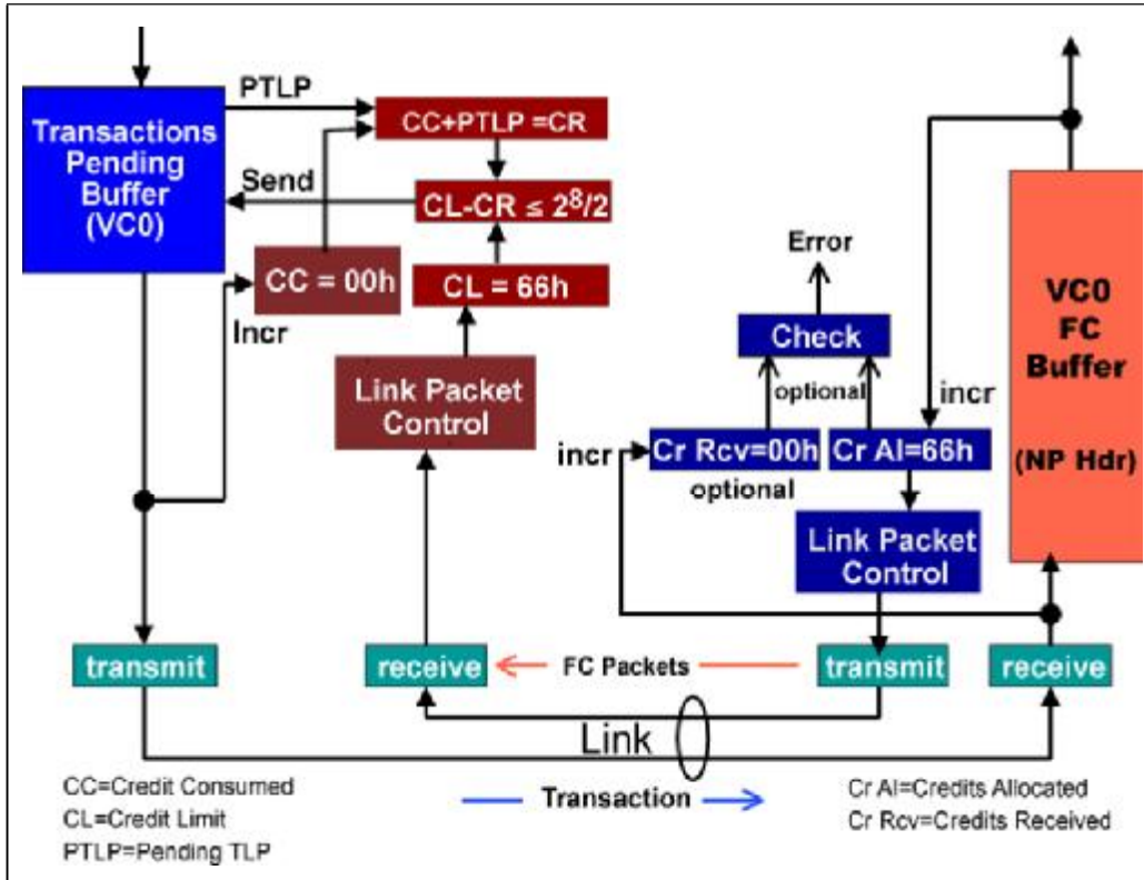
Figure 7-5: Flow Control Elements Following Initialization
