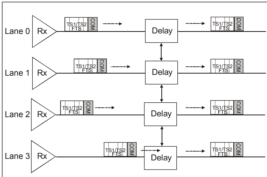
Figure 11-22: Receiver's Link De-Skew Logic
