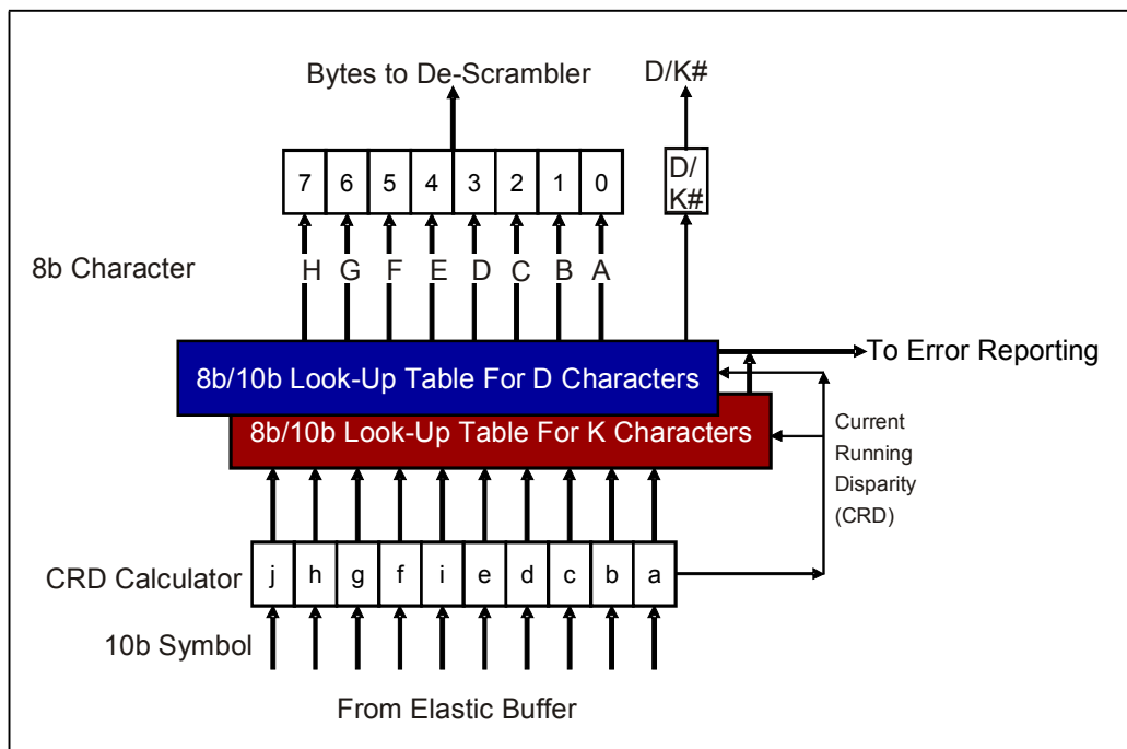
Figure 11-23: 8b/10b Decoder per Lane
