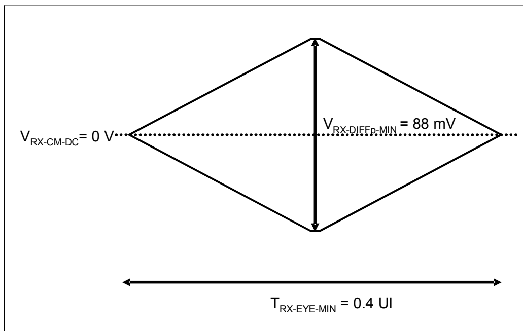
Figure 12-16: Receiver Eye Diagram
