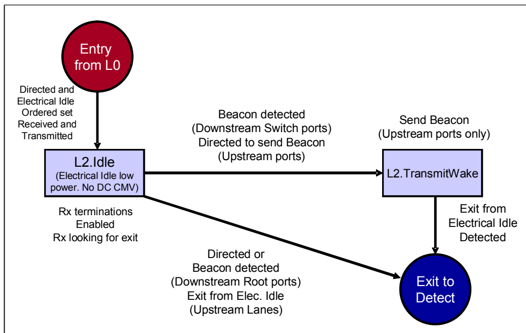
Figure 14-17: L2 State Machine
