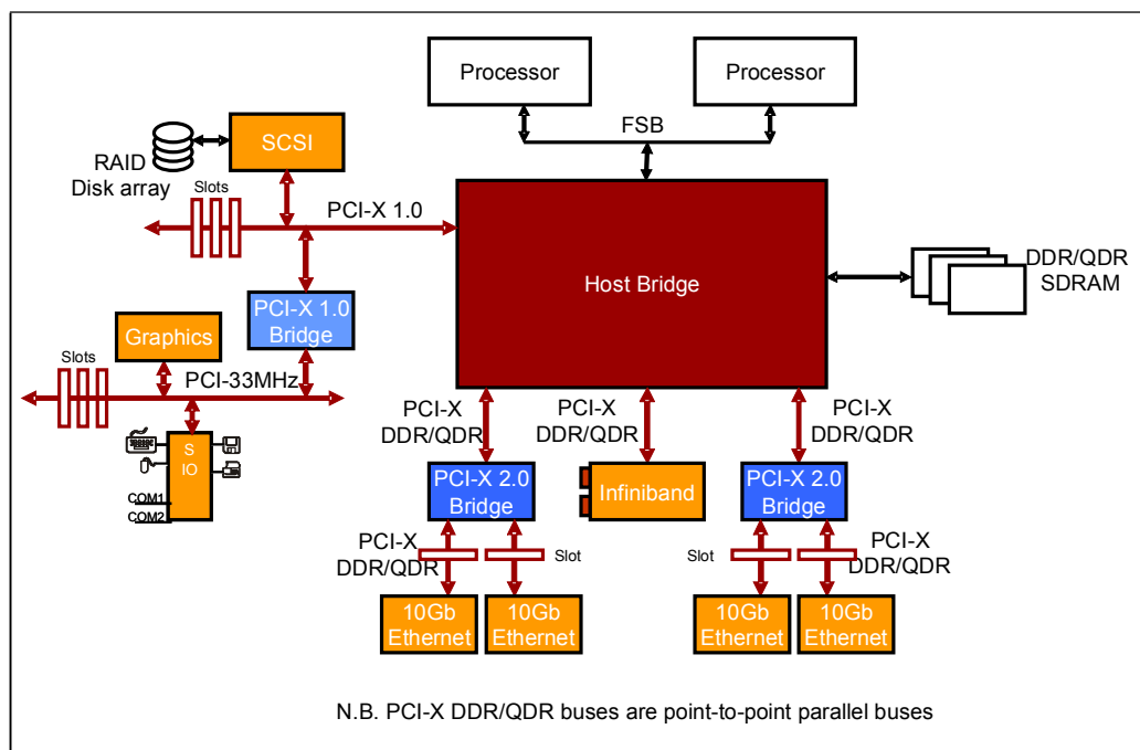
Figure 1-19: Hypothetical PCI-X 2.0 Bus Based Platform
