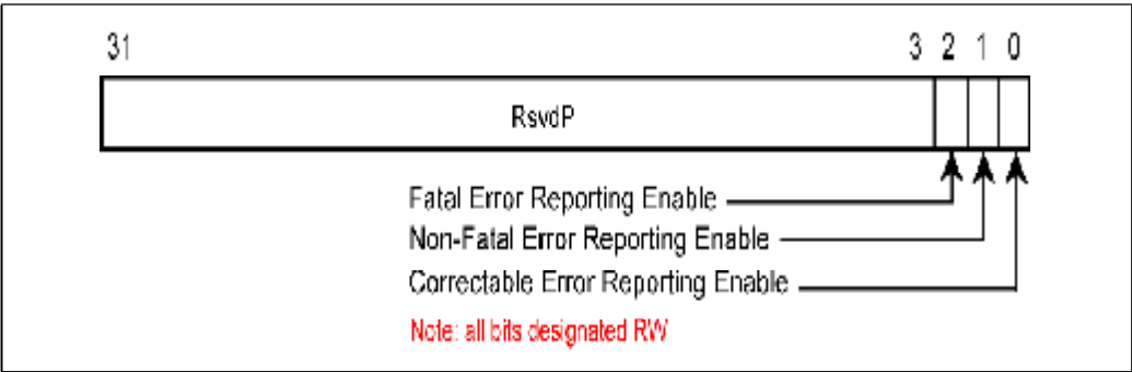
Figure 10-23: Advanced Root Error Command Register
