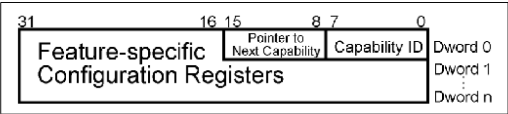
Figure 22-6: General Format of a New Capabilities List Entry
