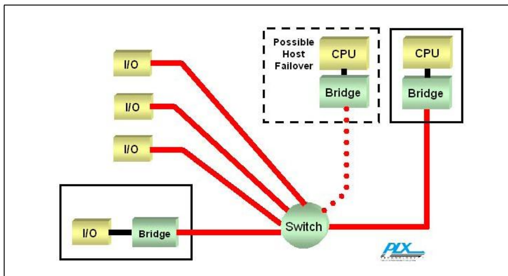
Figure B-5: PCI Express in a Storage System
