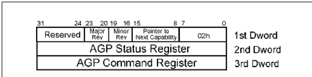
Figure 22-25: Format of the AGP Capability Register Set
