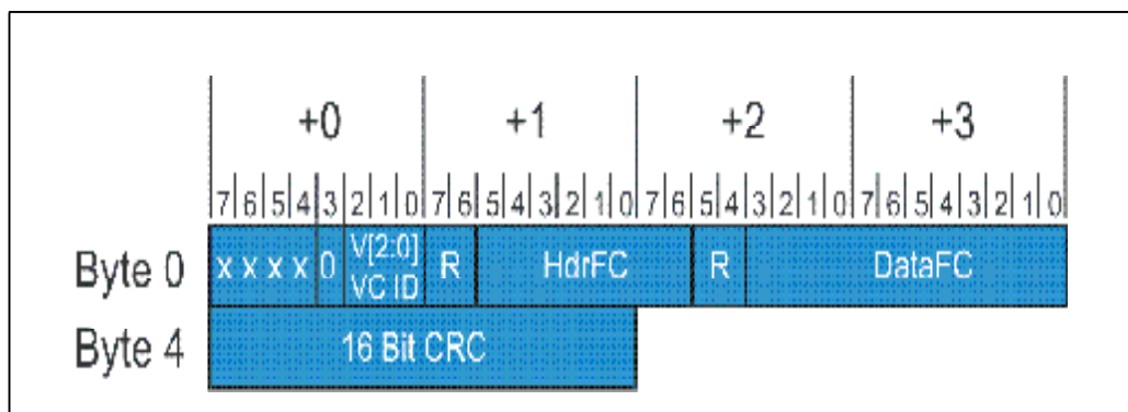
Figure 4-16: Flow Control DLLP Packet Format
