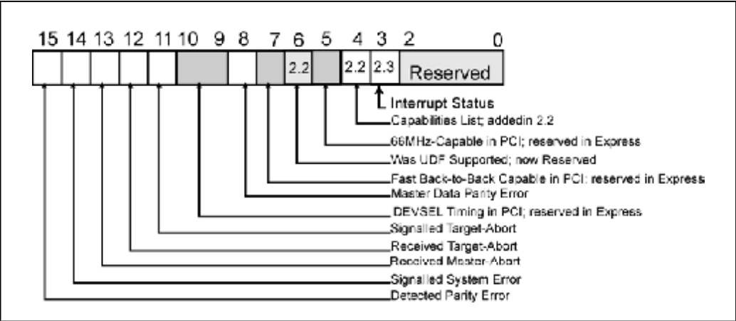
Figure 22-9: PCI Configuration Status Register
