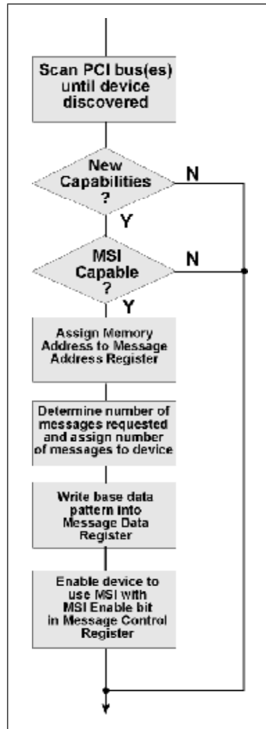
Figure 9-5: Device MSI Configuration Process
