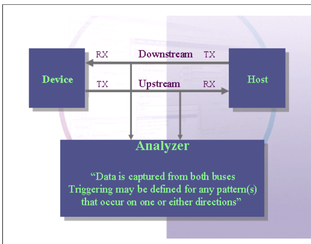
Figure A-3: PCI Express Dual-Simplex Bus
