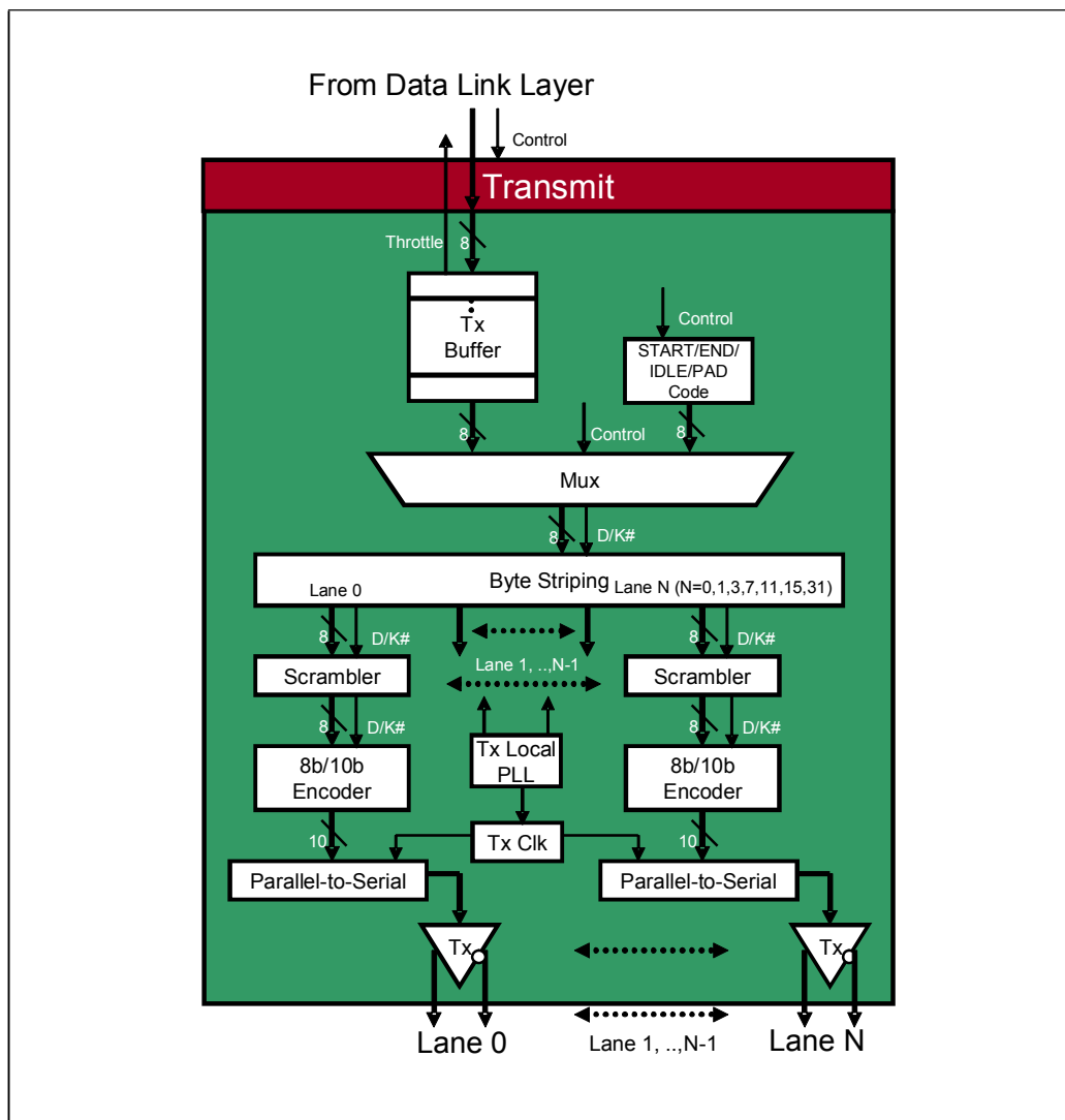
Figure 11-4: Physical Layer Transmit Logic Details
