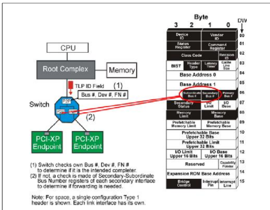
Figure 3-13: Switch Checks Routing Of An Inbound TLP Using ID Routing
