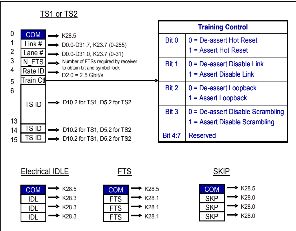
Figure 14-4: Five Ordered-Sets Used in the Link Training and Initialization Process
