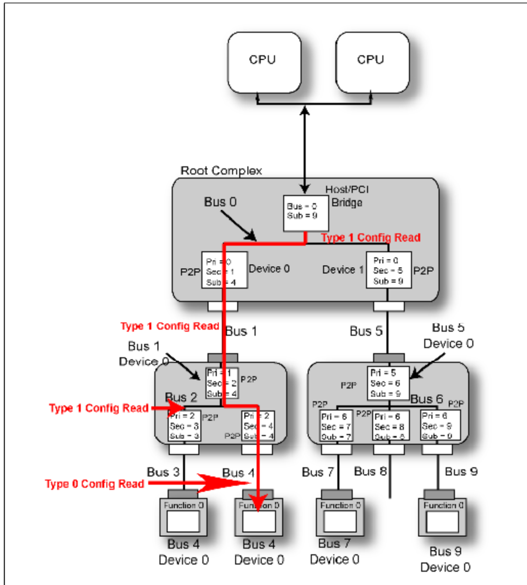
Figure 20-9: Example Configuration Access
