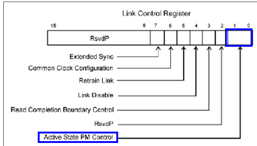
Figure 16-13: Active State PM Control Field
