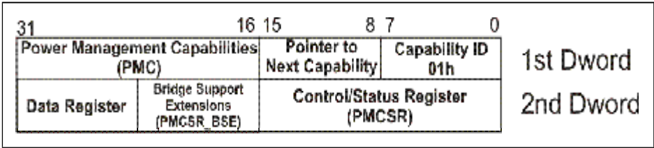
Figure 16-7: PCI Function’s PM Registers
