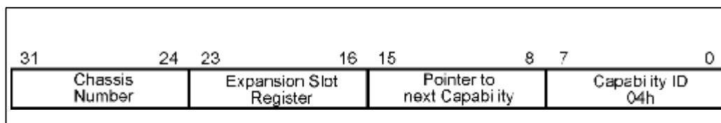
Figure 22-27: Chassis and Slot Number Registers
