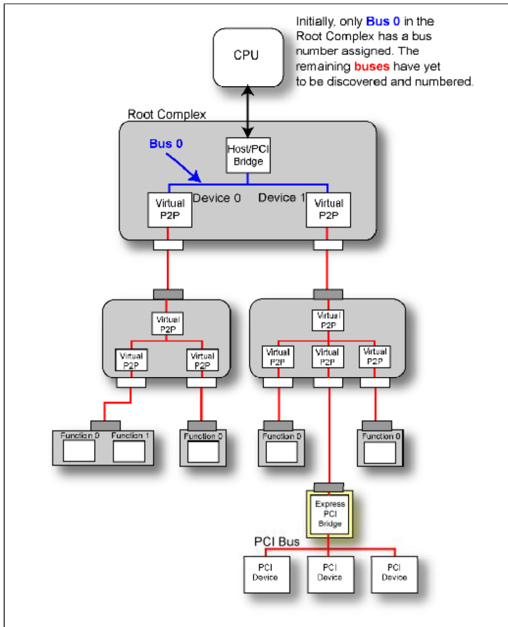
Figure 21-2: Example System Before Bus Enumeration
