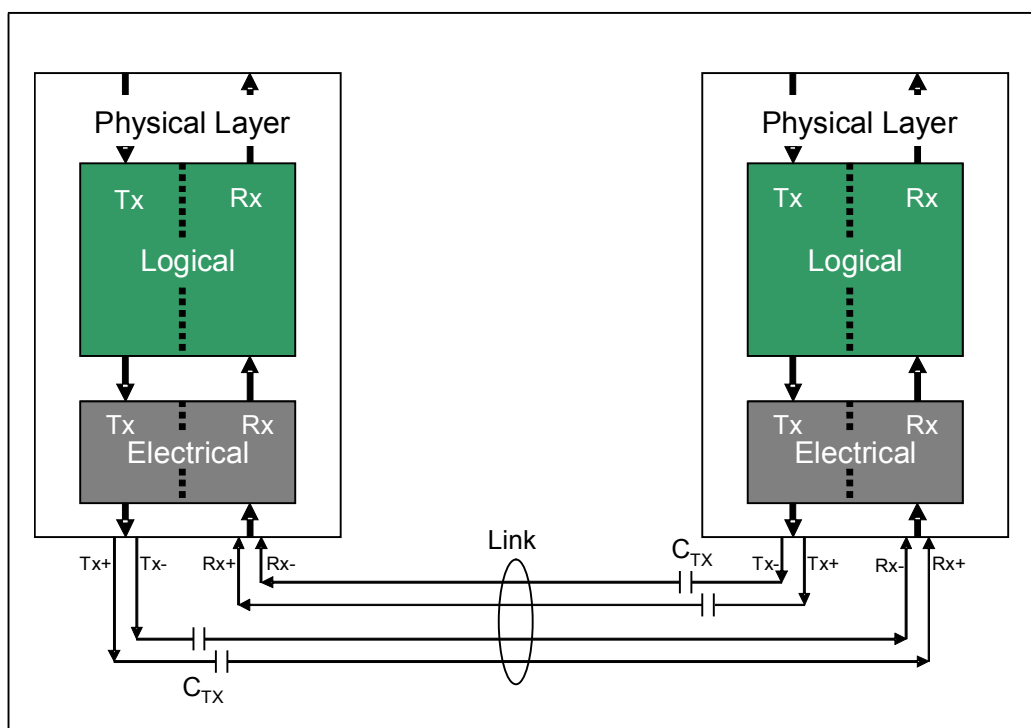
Figure 12-1: Electrical Sub-Block of the Physical Layer
