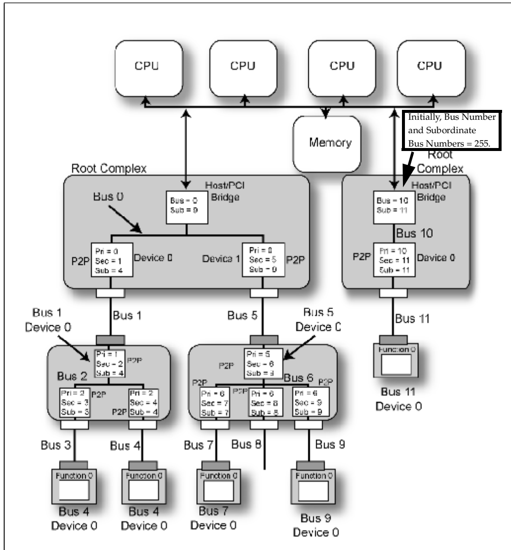
Figure 21-8: Peer Root Complexes
