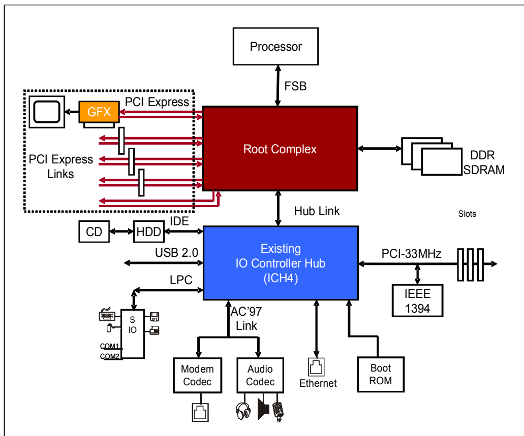
Figure 1-24: Another Low Cost PCI Express System
