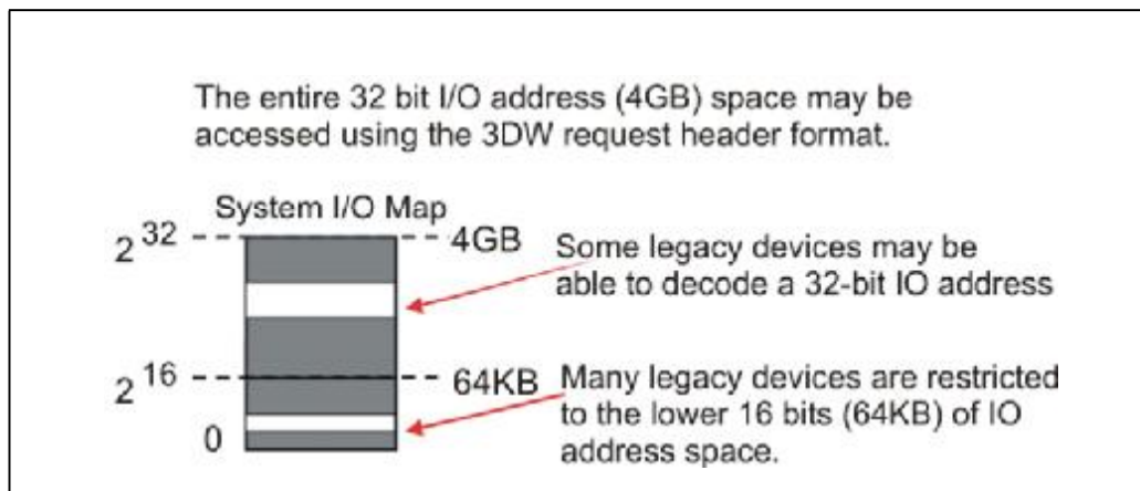
Figure 4-6: System IO Map
