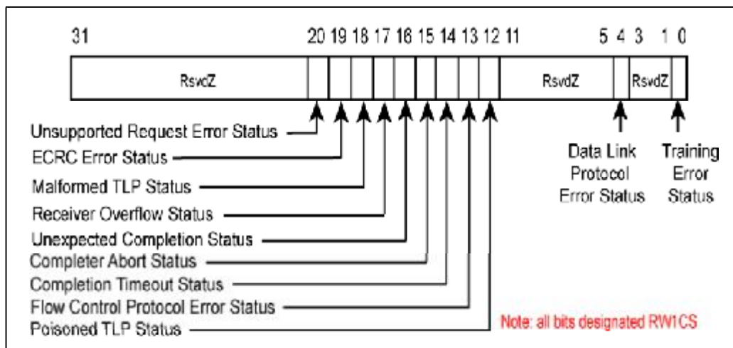
Figure 10-18: Advanced Uncorrectable Error Status Register
