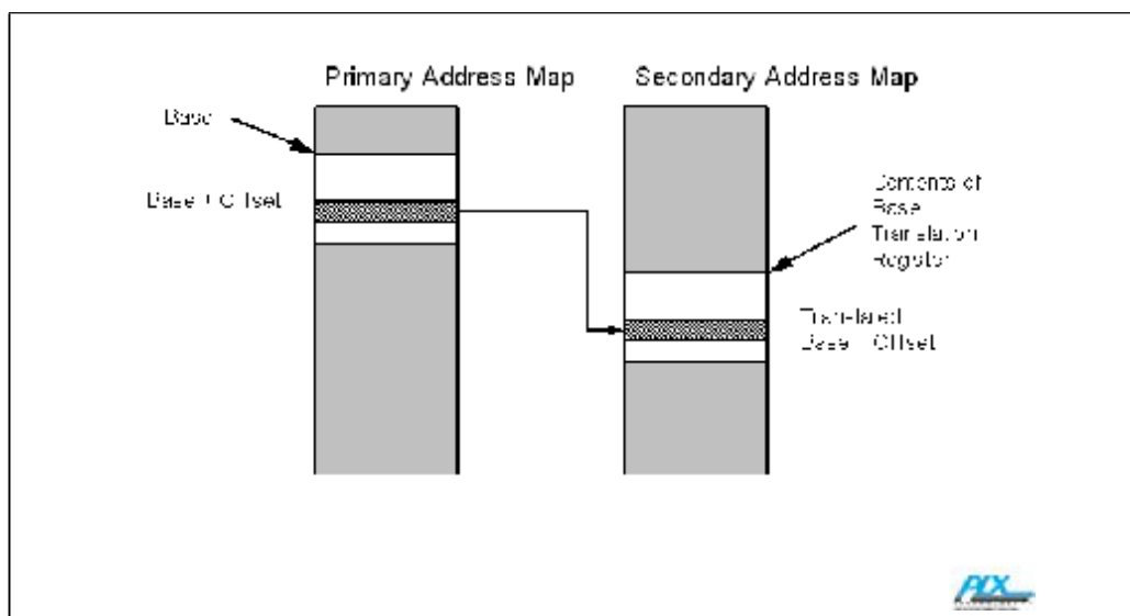
Figure C-8: Direct Address Translation
