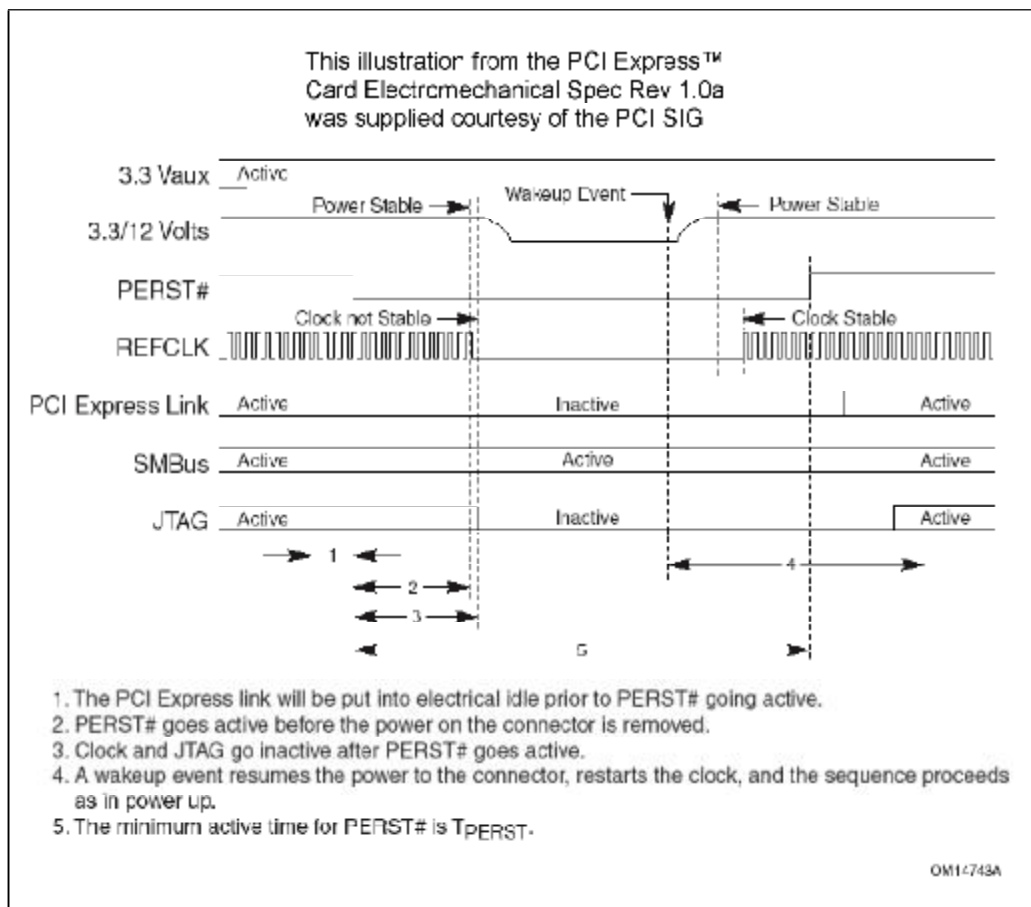
Figure 18-4: PERST# Timing During Power Management States
