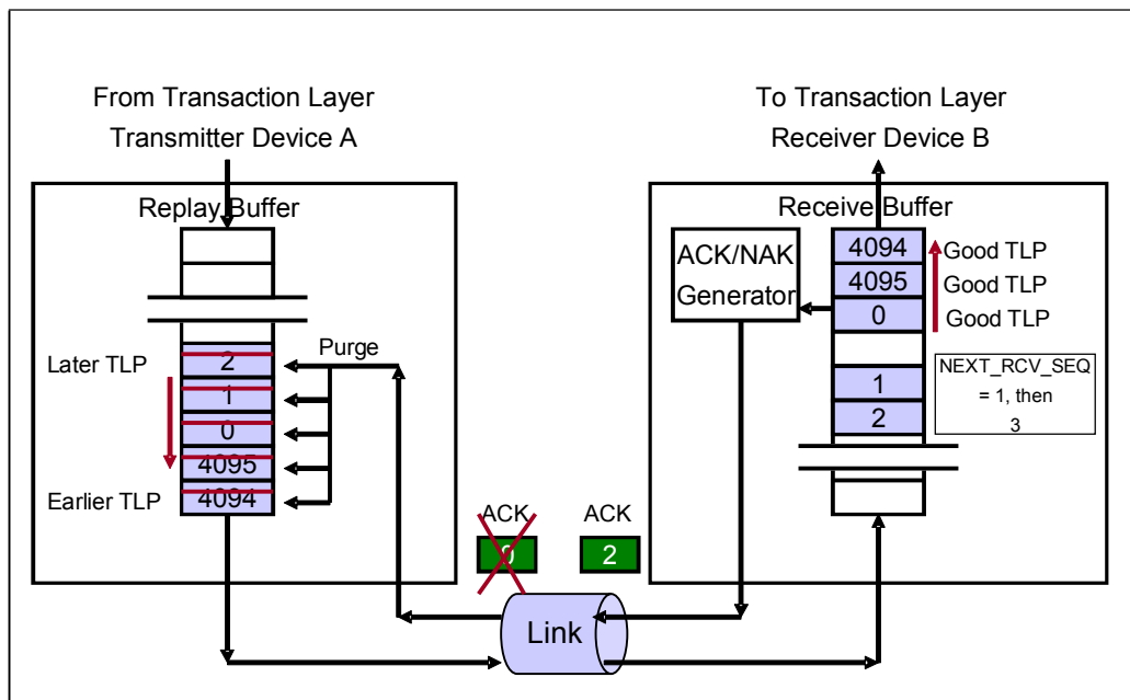
Figure 5-15: Lost ACK DLLP Handling
