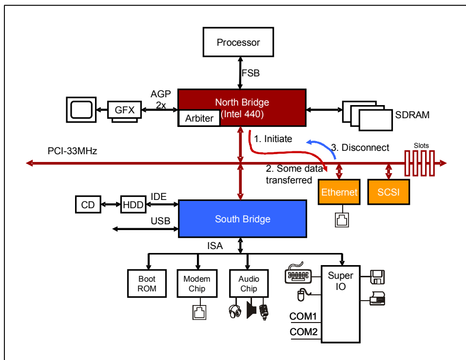
Figure 1-8: PCI Transaction Disconnect Mechanism
