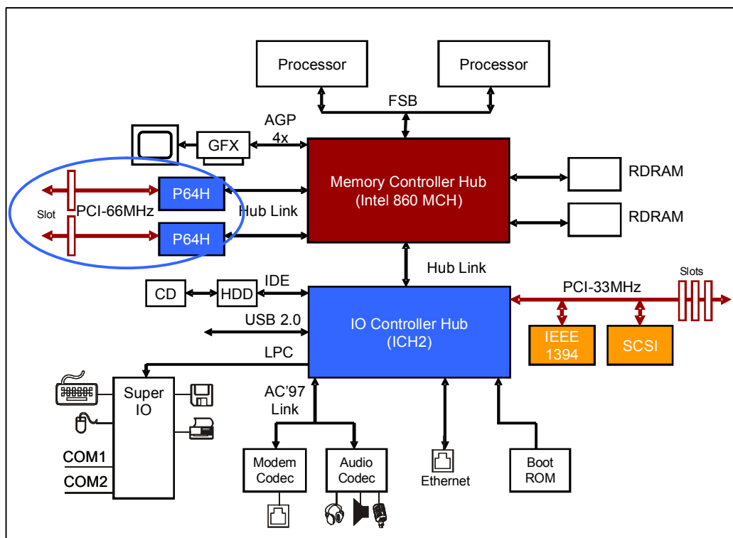
Figure 1-15: 66 MHz PCI Bus Based Platform
