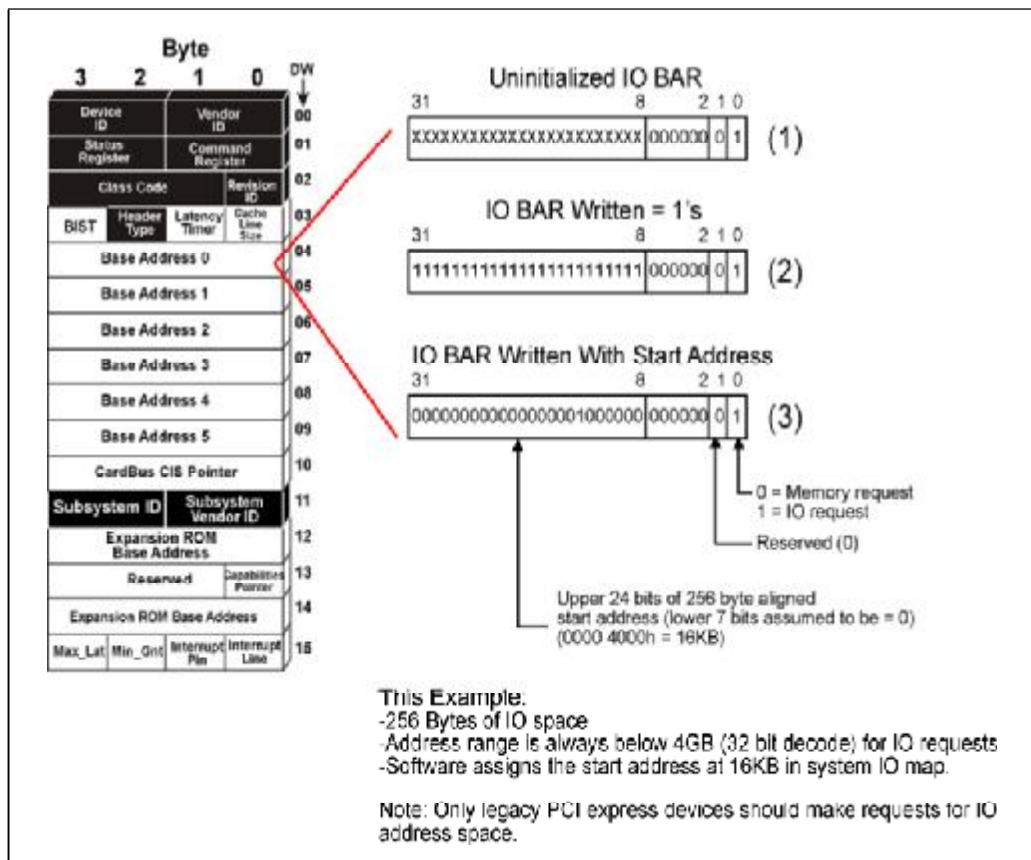
Figure 3-19: IO BAR Set Up
