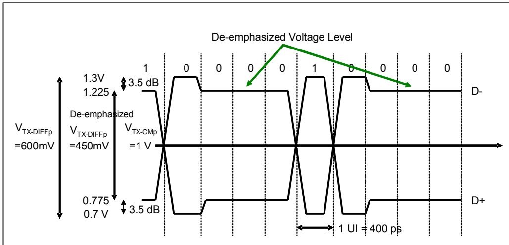
Figure 12-7: Transmission with De-emphasis
