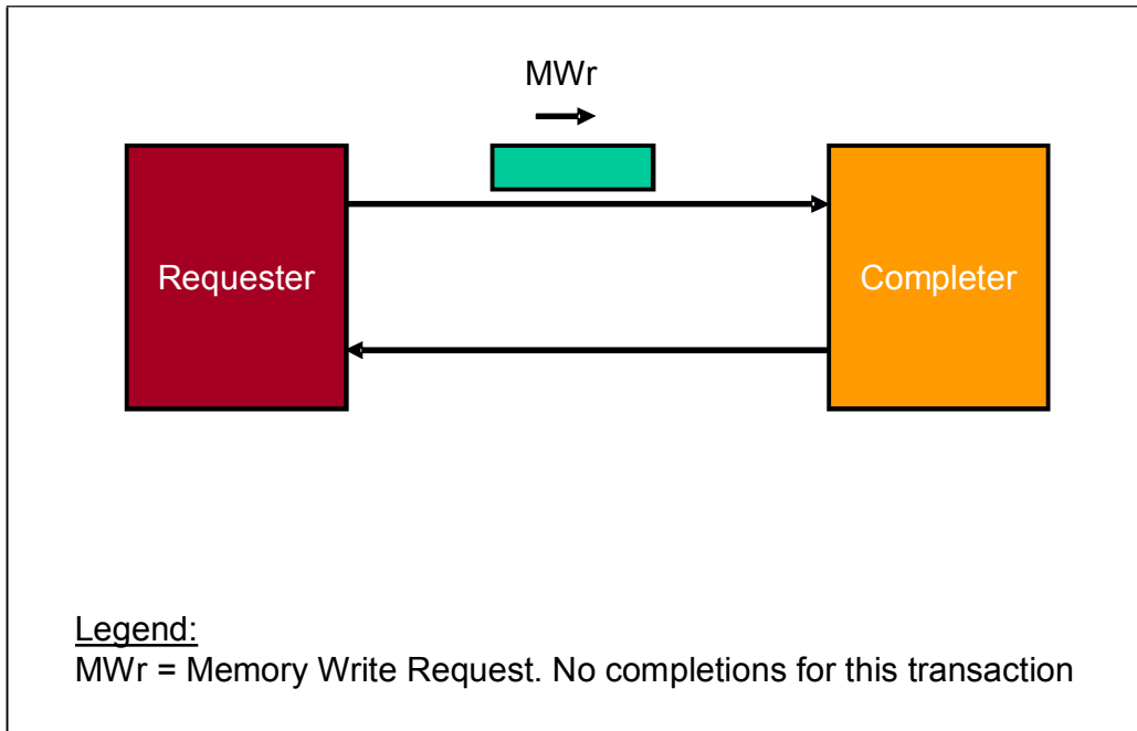
Figure 2-4: Posted Memory Write Transaction Protocol
