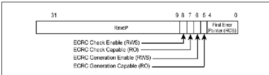
Figure 24-18: Advanced Error Capabilities and Control Register
