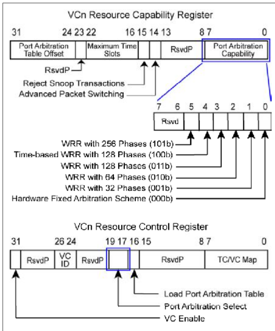
Figure 6-19: Software checks Port Arbitration Capabilities and Selects the Scheme to be Used.
