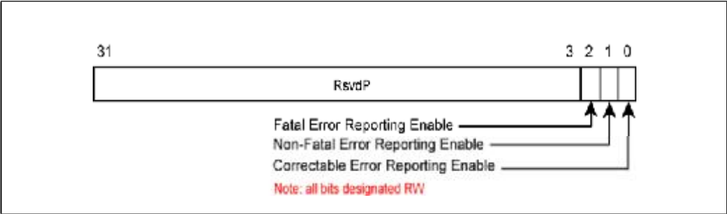
Figure 24-24: Advanced Error Root Error Command Register
