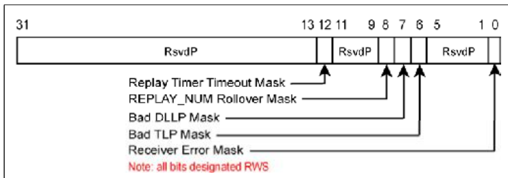
Figure 10-17: Advanced Correctable Error Mask Register
