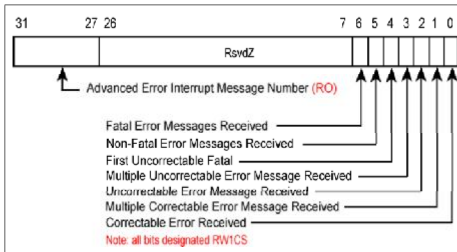
Figure 10-21: Root Error Status Register
