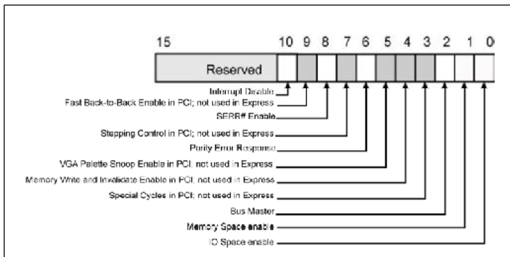
Figure 22-8: Command Register
