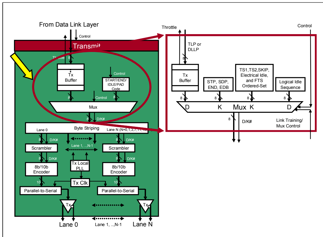
Figure 11-5: Transmit Logic Multiplexer
