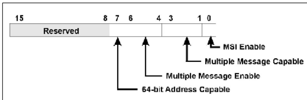
Figure 9-4: Message Control Register
