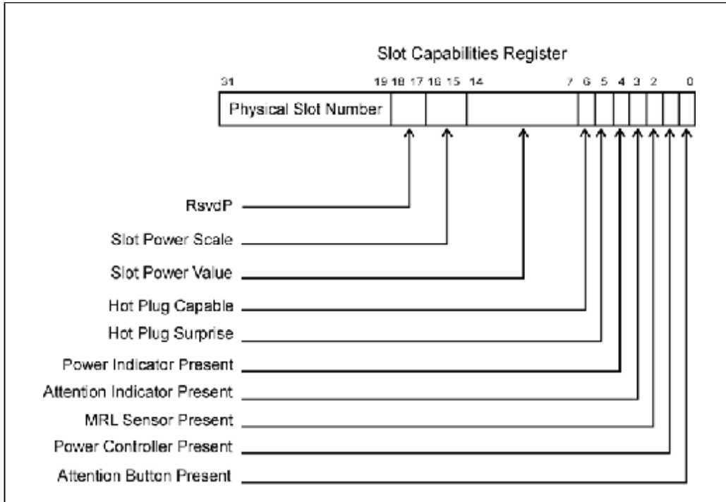
Figure 24-10: Slot Capabilities Register
