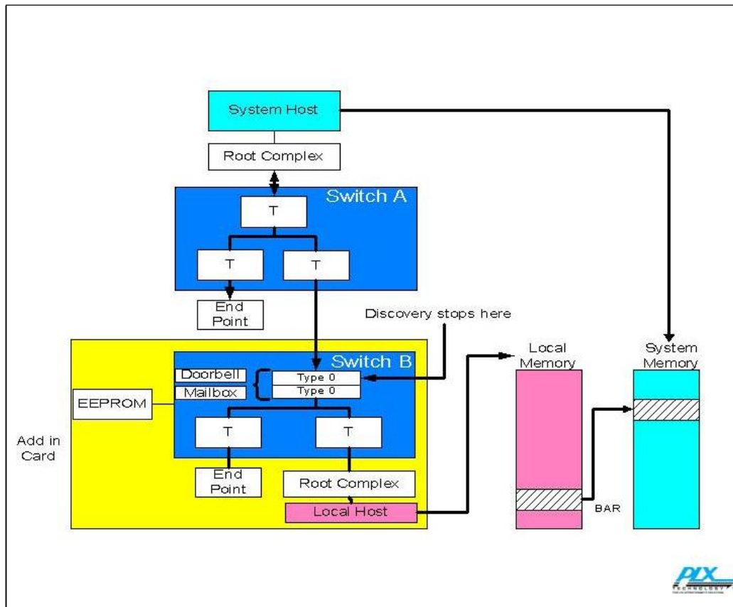
Figure C-4: Intelligent Adapters in PCI and PCI Express Systems
