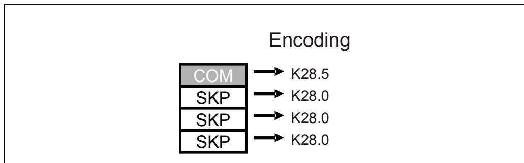
Figure 11-19: SKIP Ordered-Set
