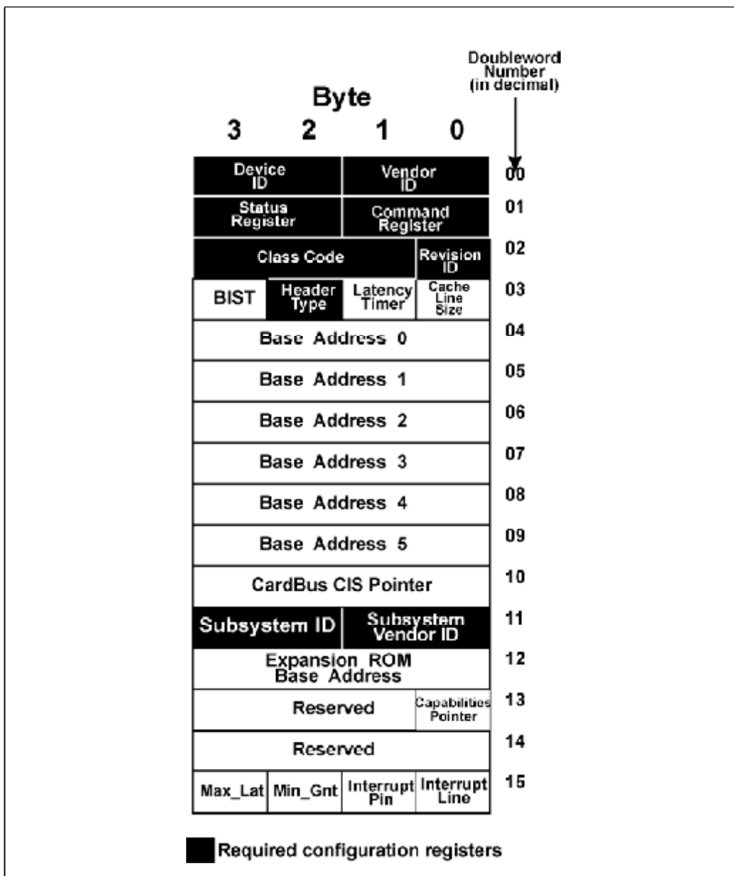
Figure 22-1: Header Type 0
