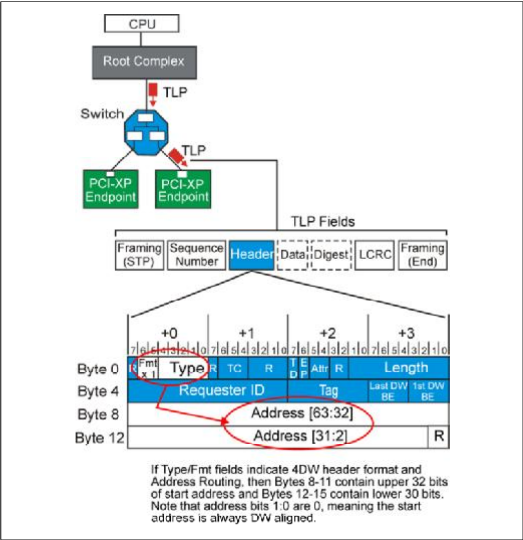
Figure 3-8: 4DW TLP Header Address Routing Fields
