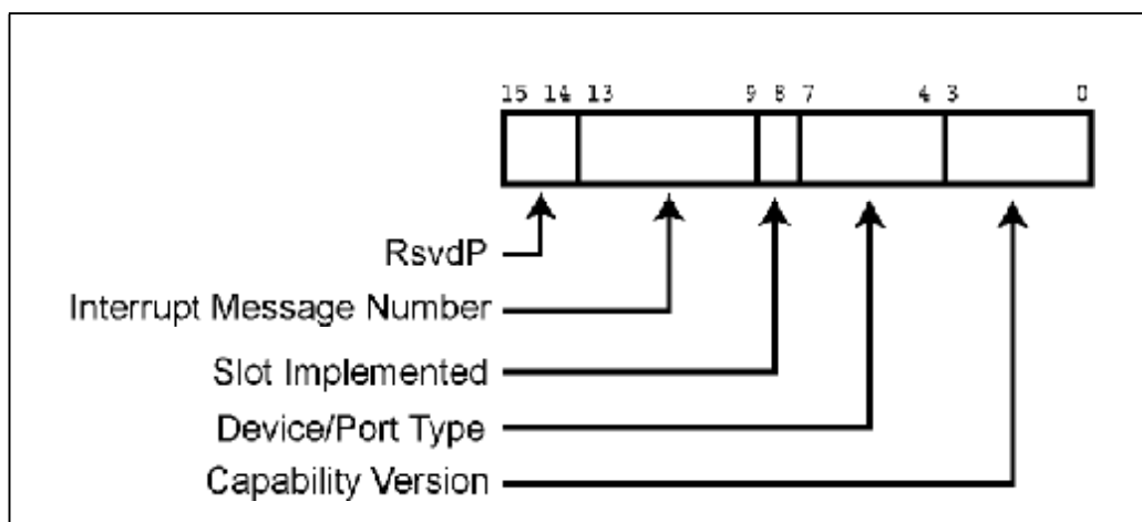
Figure 21-5: Capability Register
