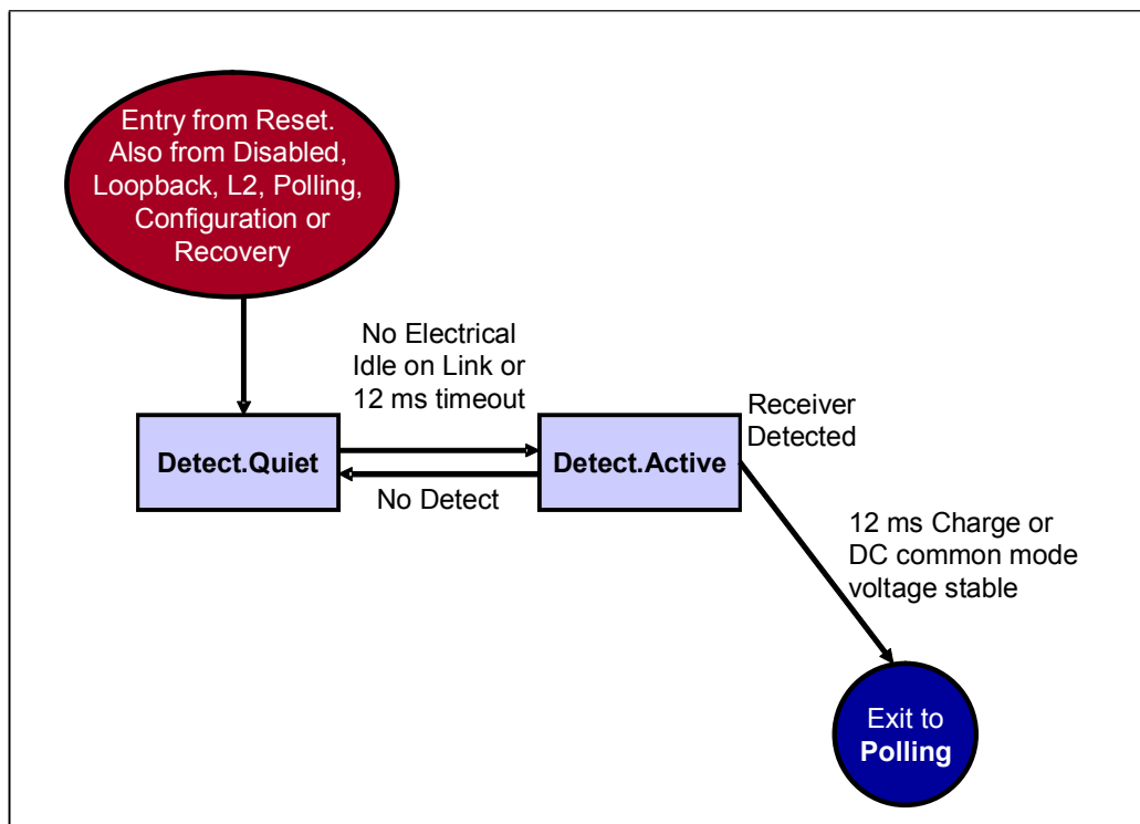
Figure 14-6: Detect State Machine
