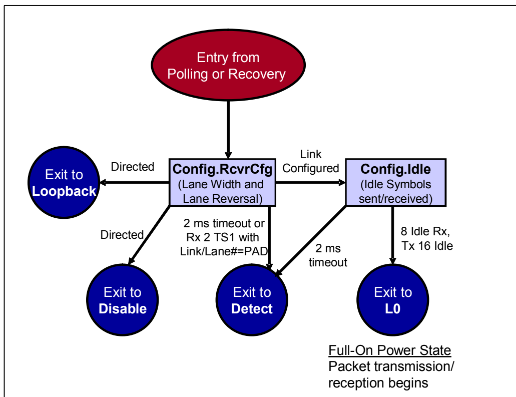
Figure 14-8: Configuration State Machine
