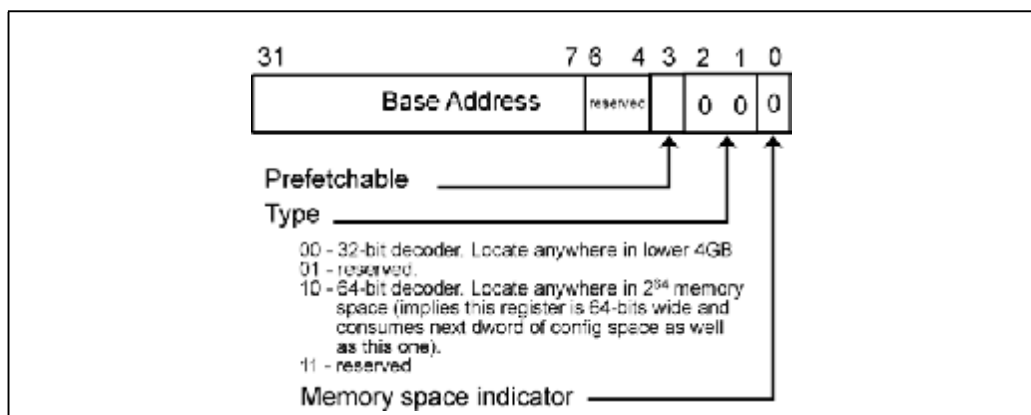
Figure 22-10: 32-Bit Memory Base Address Register Bit Assignment
