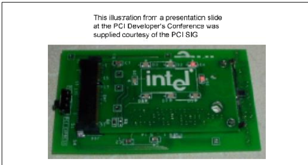
Figure 18-10: Mini PCI Express Add-in Card Photo 2
