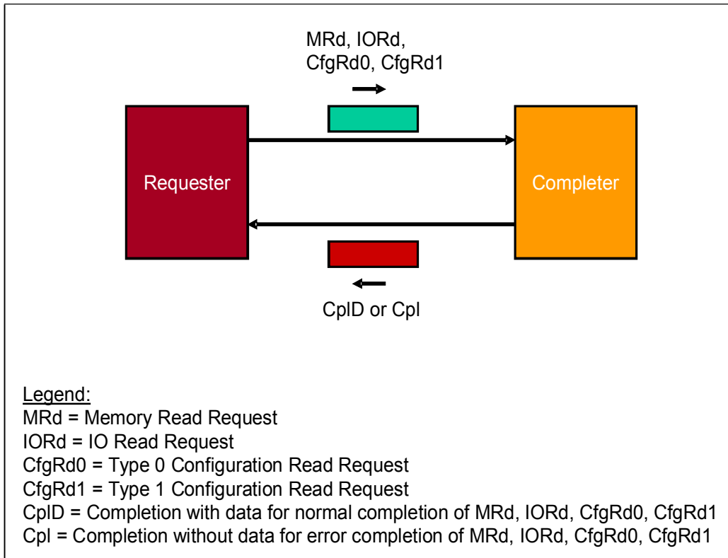
Figure 2-1: Non-Posted Read Transaction Protocol
