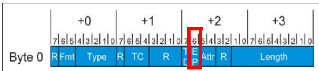
Figure 10-3: The Error/Poisoned Bit within Packet Headers
