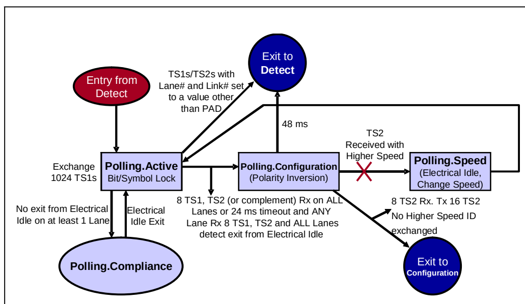
Figure 14-7: Polling State Machine
