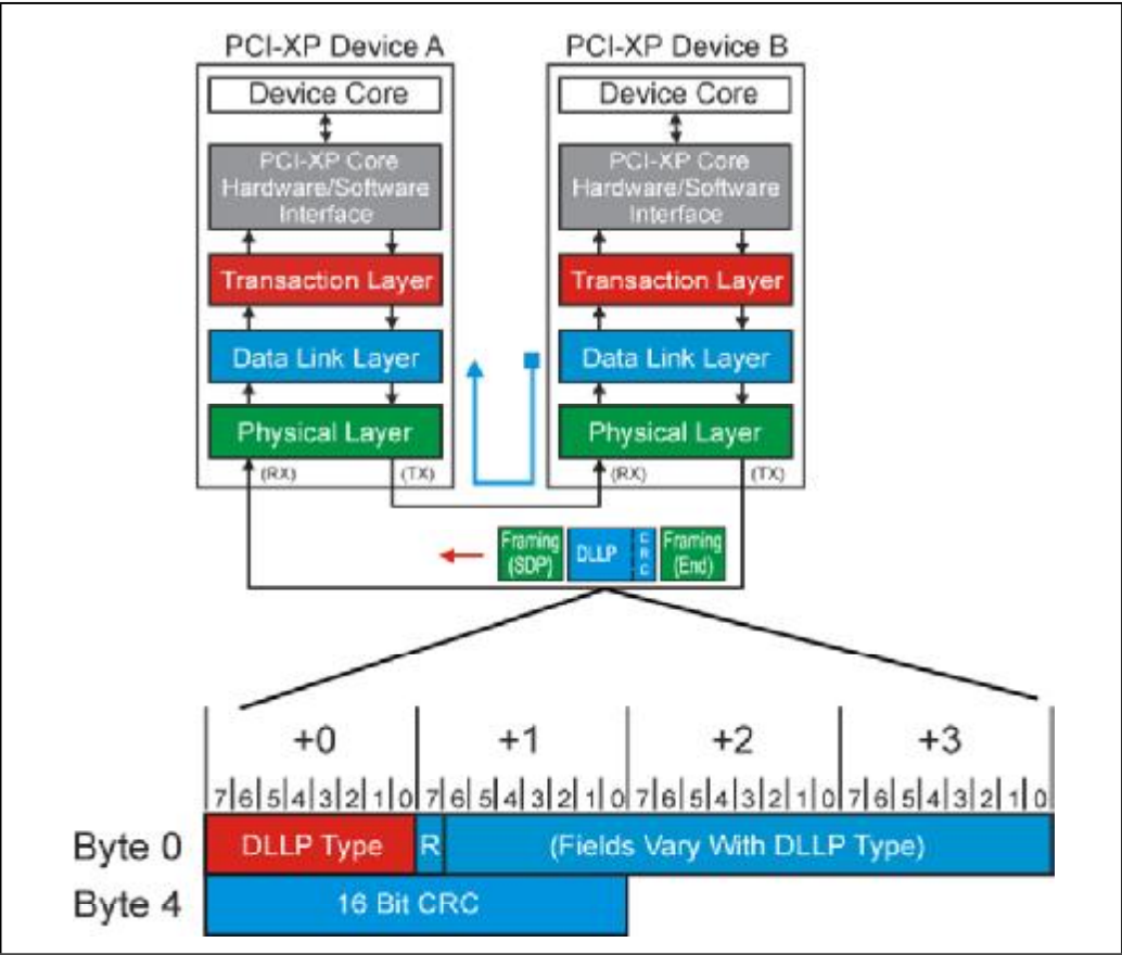
Figure 4-13: Generic Data Link Layer Packet Format
