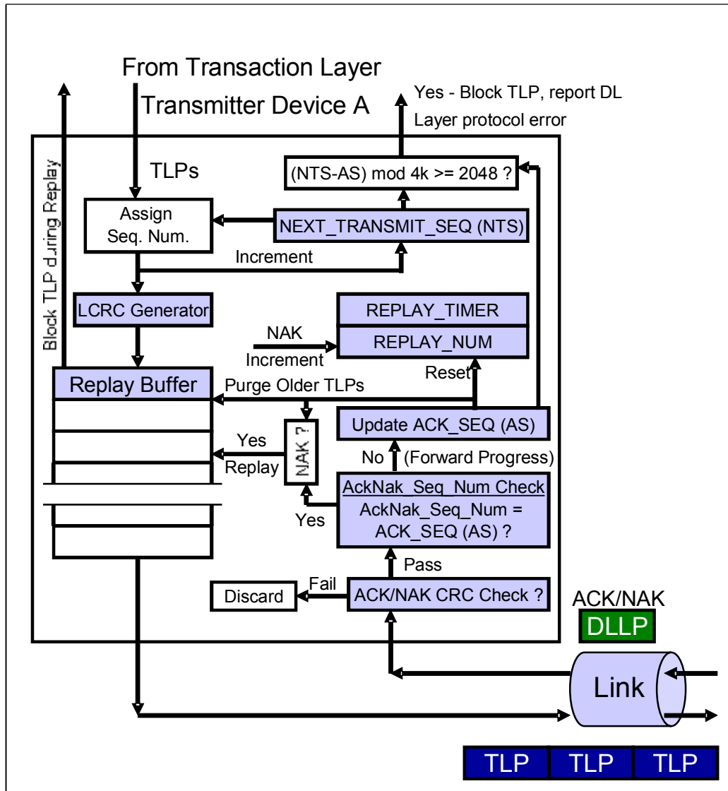
Figure 5-4: Transmitter Elements Associated with the ACK/NAK Protocol
