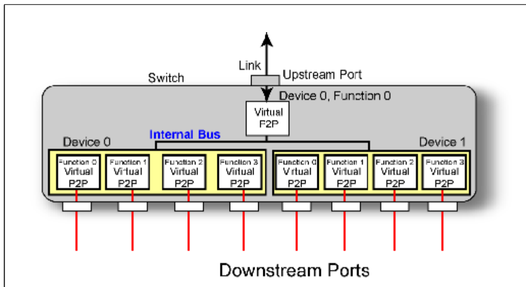
Figure 21-10: First Example of a Multifunction Bridge In a Switch
