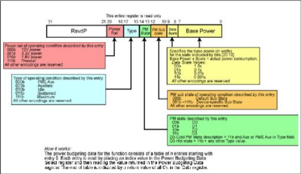
Figure 24-42: Power Budgeting Data Register
