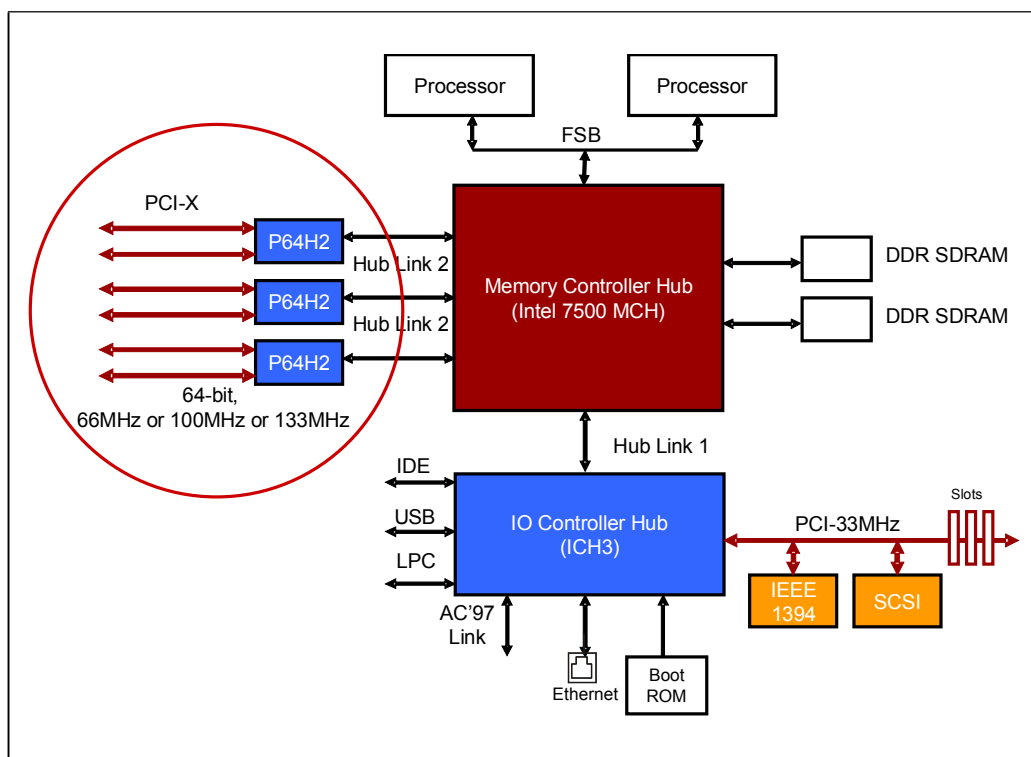
Figure 1-16: 66 MHz/133 MHz PCI-X Bus Based Platform
