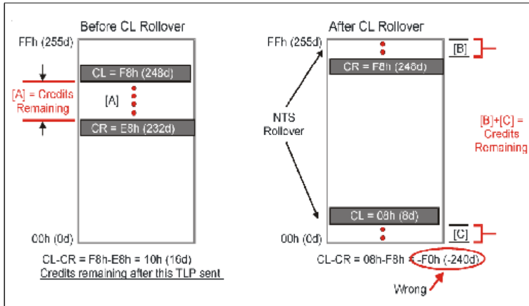
Figure 7-8: Flow Control Rollover Problem
