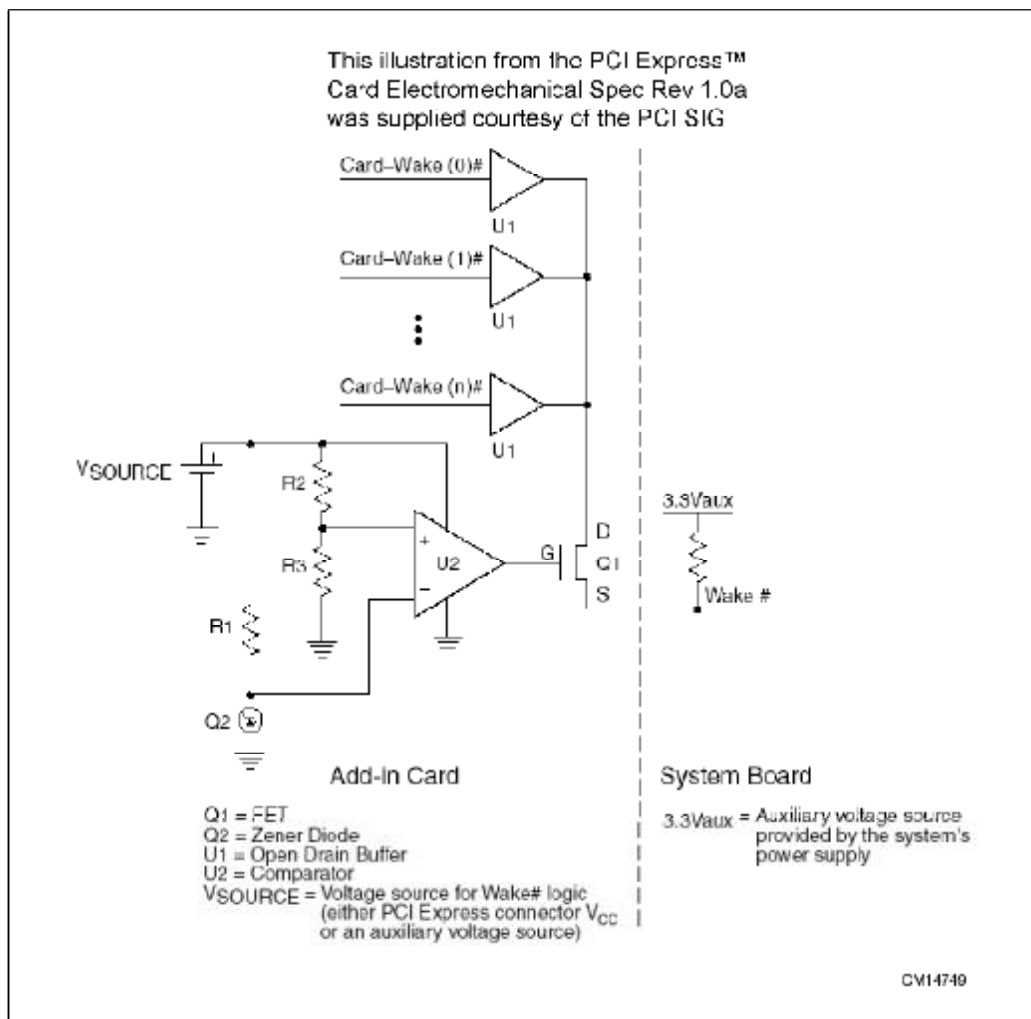
Figure 18-5: Example of WAKE# Circuit Protection
