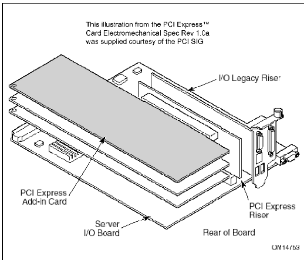
Figure 18-7: PCI Express Riser Card
