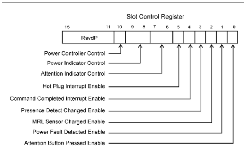
Figure 17-6: Slot Control Register Fields
