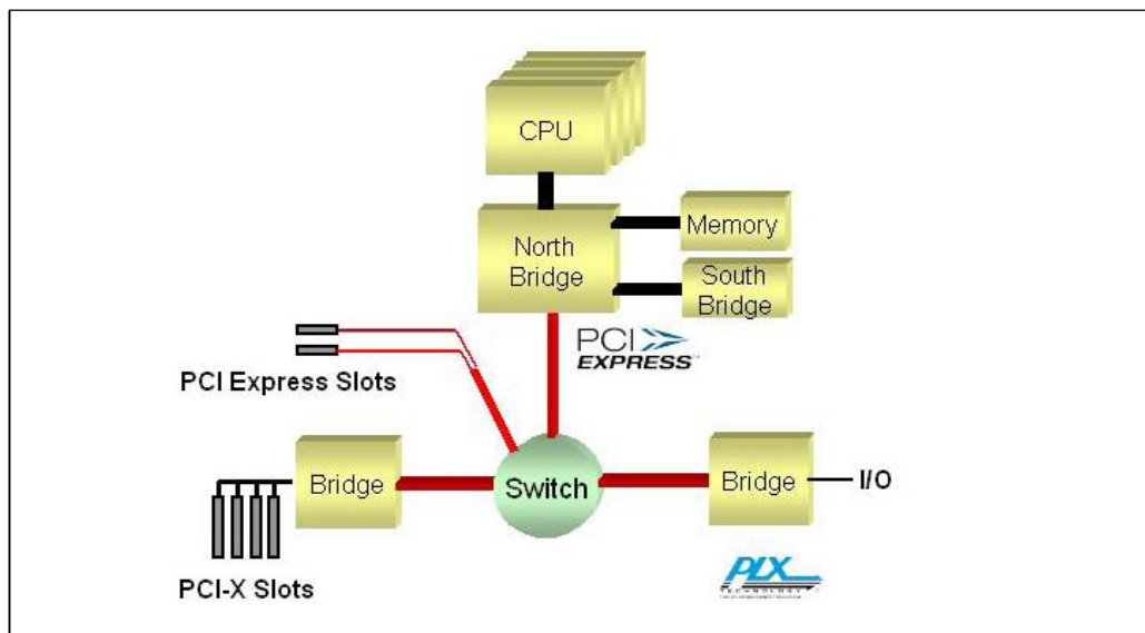
Figure B-3: PCI Express in a Server System
