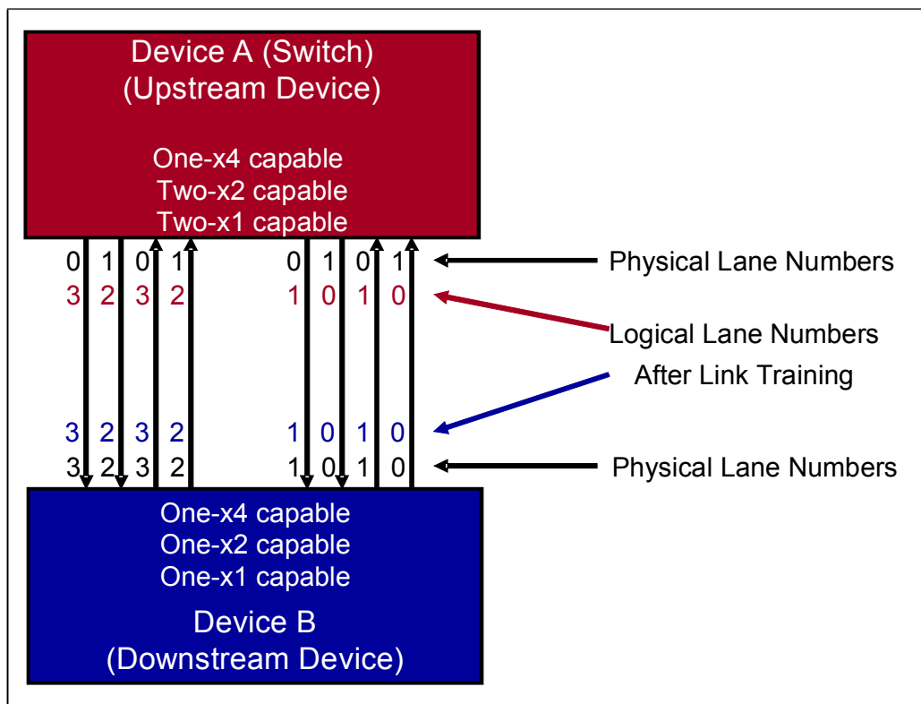
Figure 14-12: Example 3 Link Numbering and Lane Numbering
