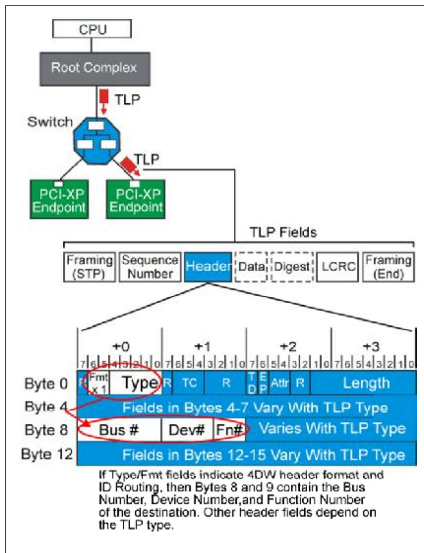
Figure 3-12: 4DW TLP Header ID Routing Fields
