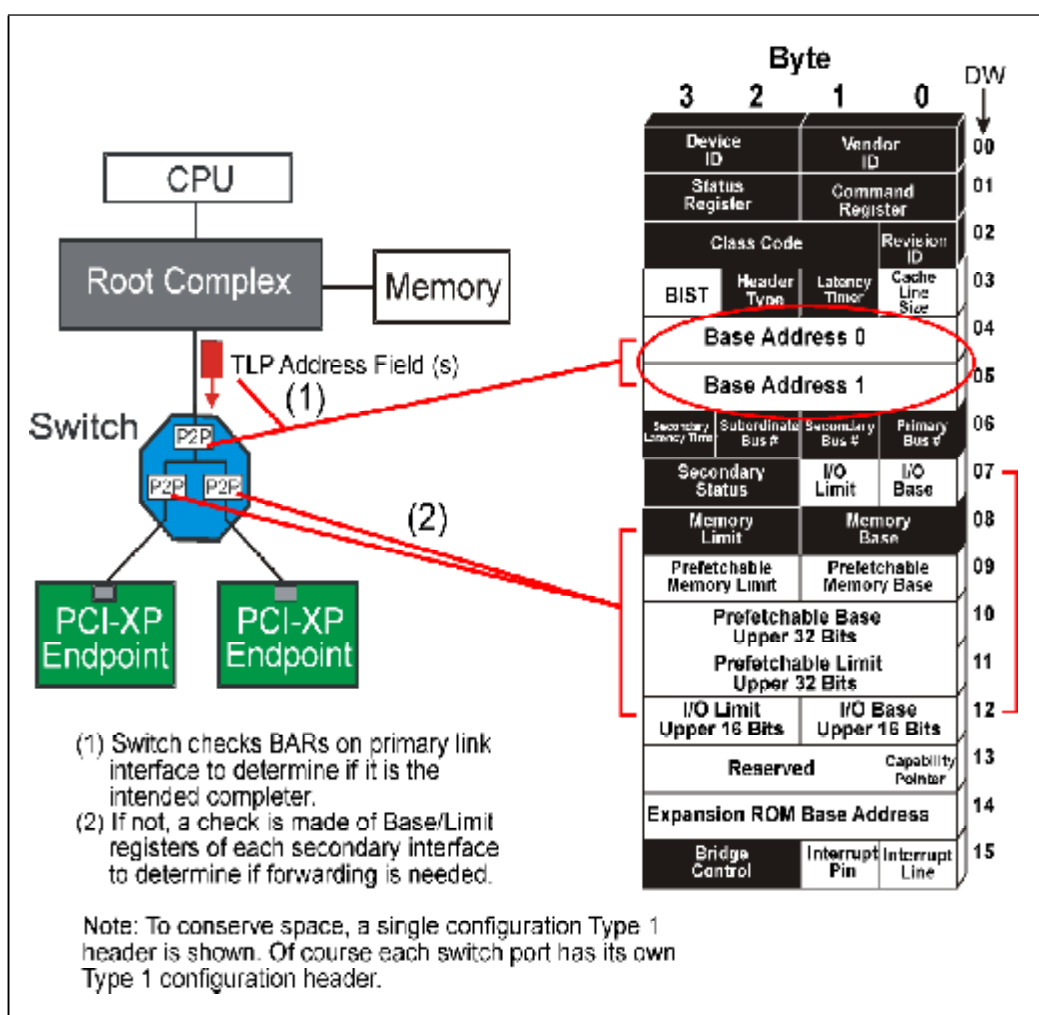
Figure 3-10: Switch Checks Routing Of An Inbound TLP Using Address Routing
