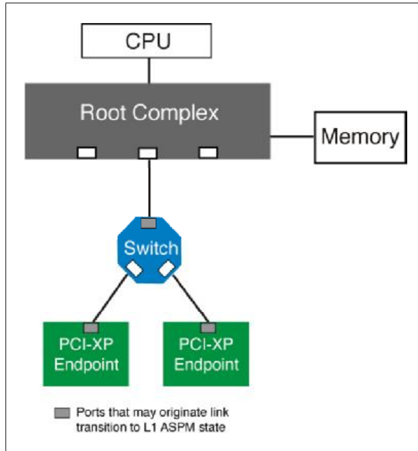
Figure 16-14: Ports that Initiate L1 ASPM Transitions
