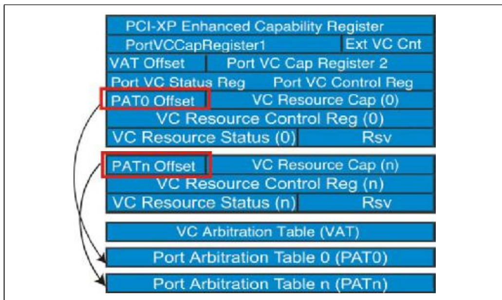
Figure 6-17: Port Arbitration Tables Needed for nEach VC
