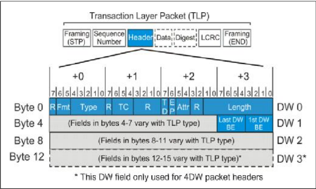
Figure 4-3: Generic TLP Header Fields
