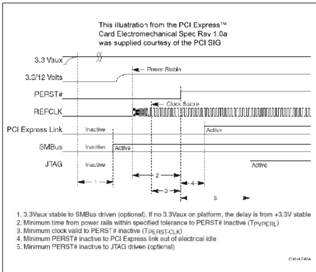
Figure 18-3: PERST Timing During Power Up
