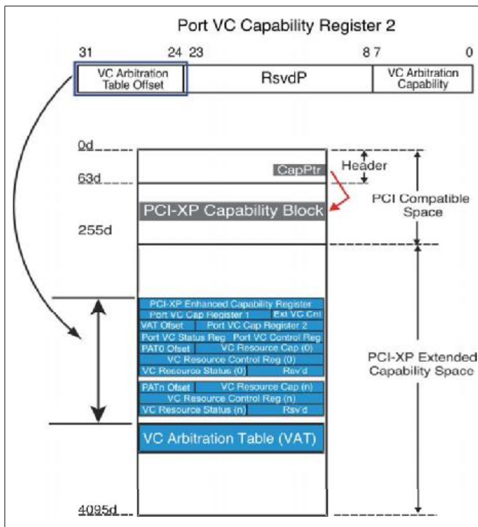
Figure 6-13: VC Arbitration Table Offset and Load VC Arbitration Table Fields
