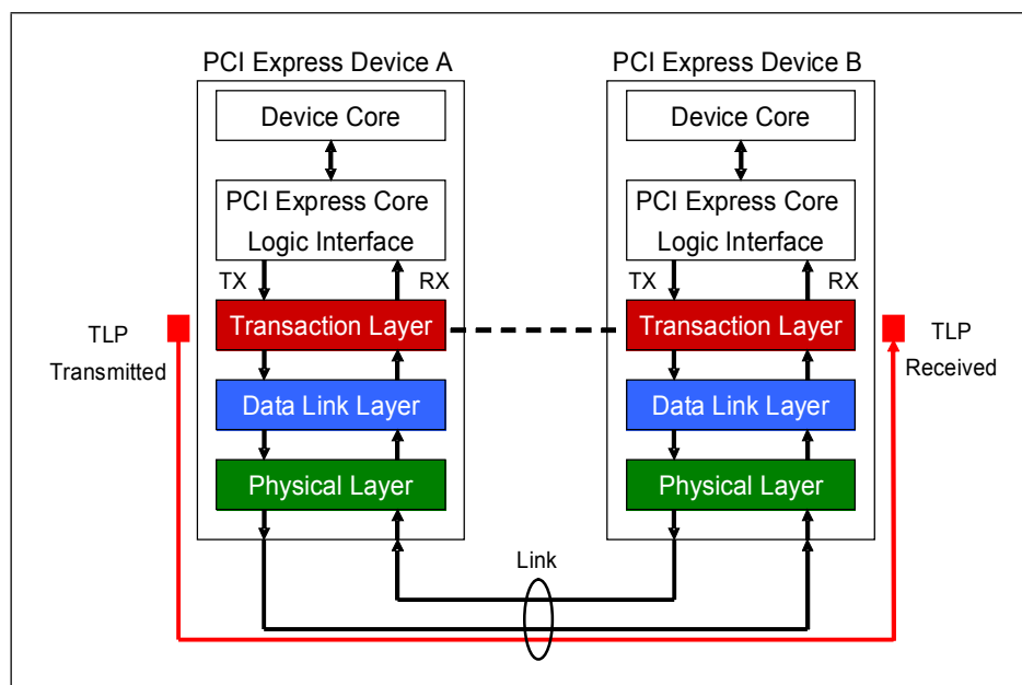
Figure 2-11: TLP Origin and Destination
