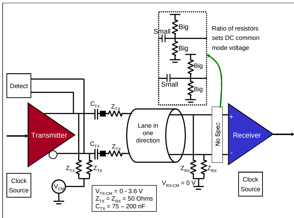
Figure 12-3: Receiver DC Common Mode Voltage Requirement
