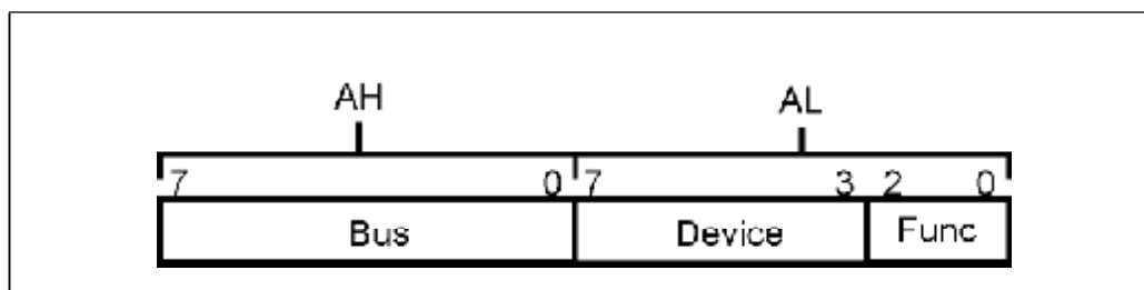
Figure 23-5: AX Contents On Entry To Initialization Code
