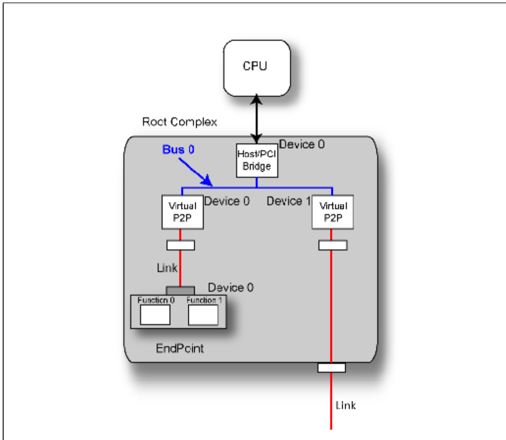
Figure 21-12: Embedded Root Endpoint
