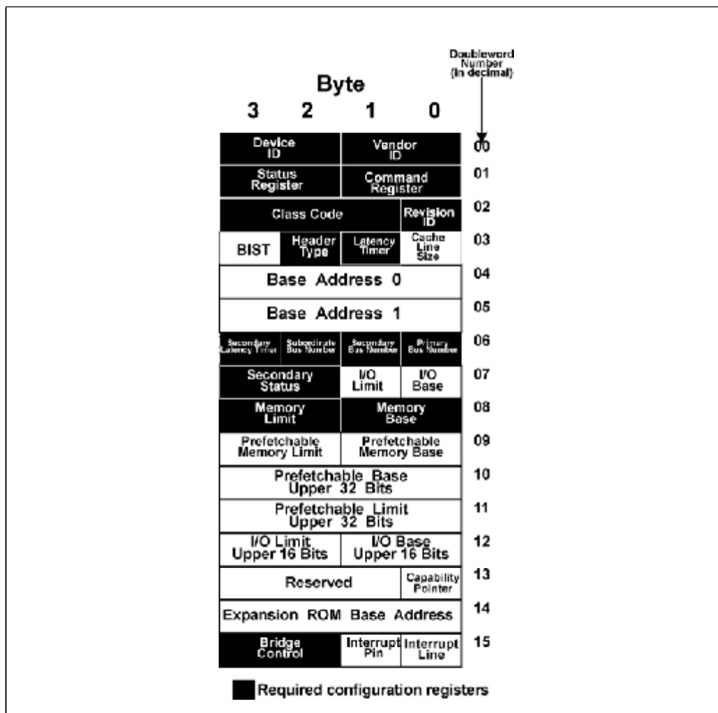
Figure 22-13: Header Type 1
