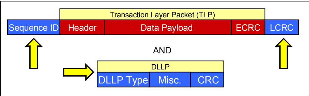
Figure 2-26: TLP and DLLP Structure at the Data Link Layer
