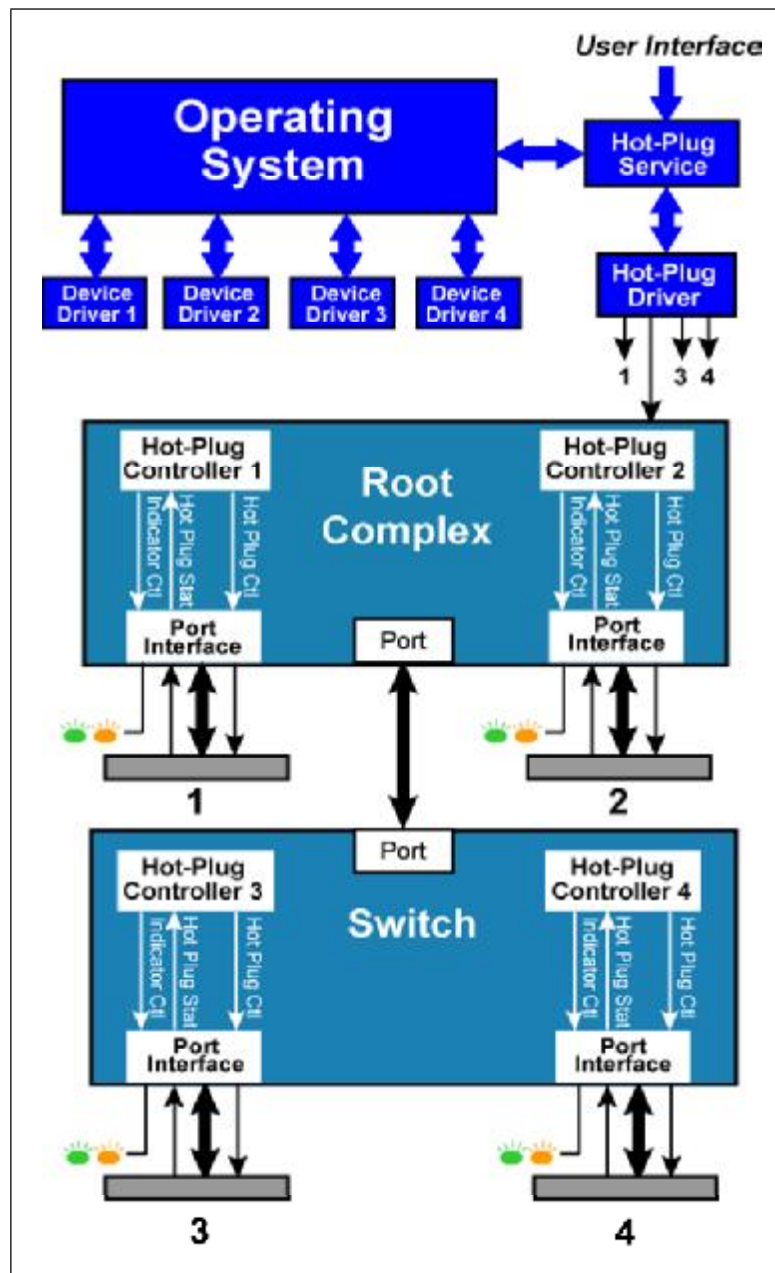
Figure 17-2: PCI Express Hot-Plug Hardware/Software Elements
