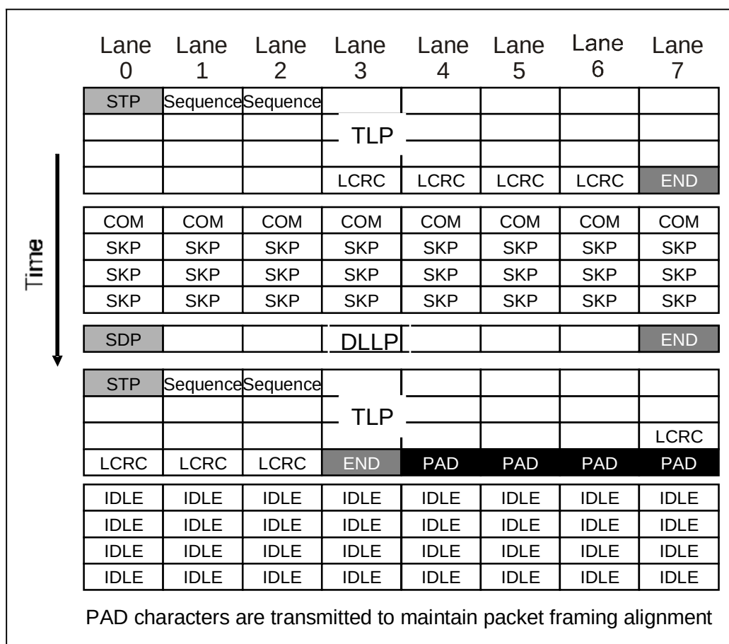
Figure 11-12: x8 Packet Format
