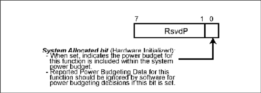
Figure 24-43: Power Budgeting Capability Register
