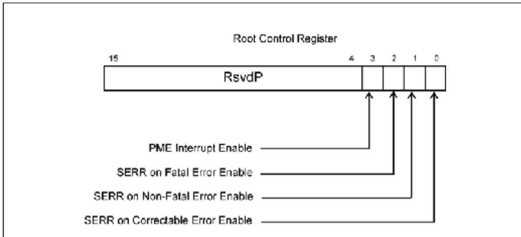
Figure 24-13: Root Control Register
