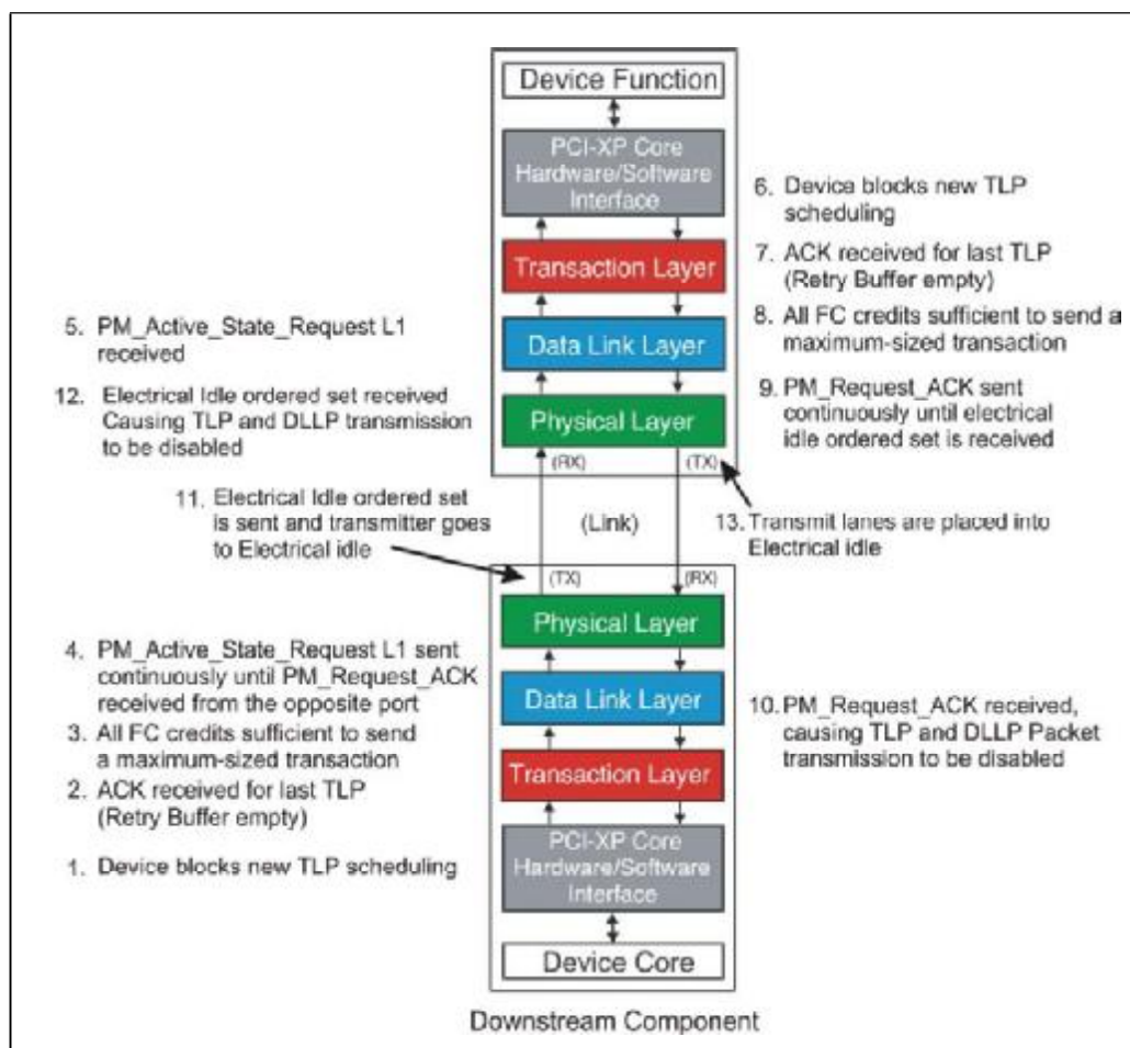
Figure 16-15: Negotiation Sequence Required to Enter L1 Active State PM
