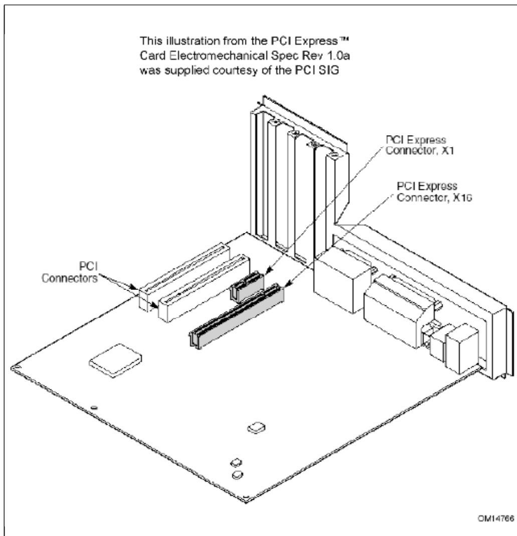
Figure 18-2: PCI Express Connectors on System Board
