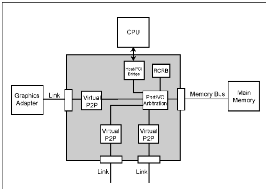
Figure 24-44: RCRB Example
