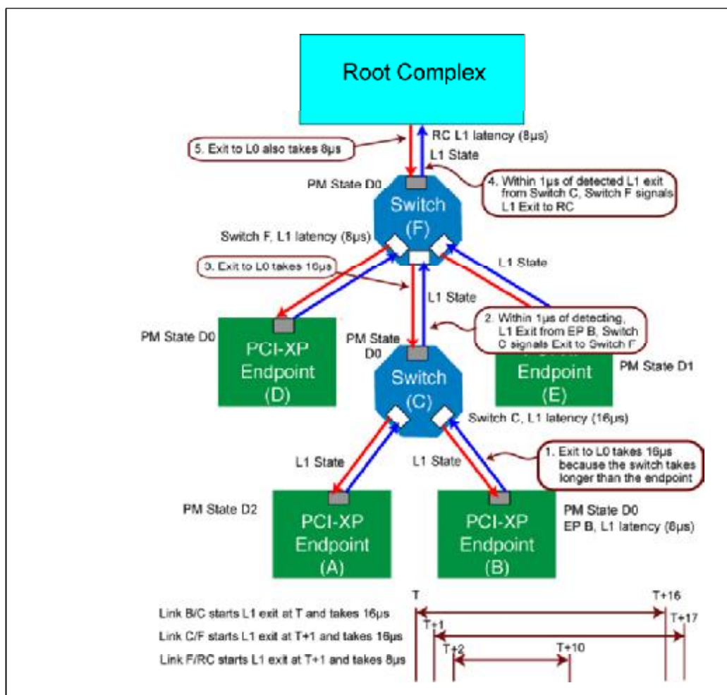
Figure 16-19: Example of Total L1 Latency
