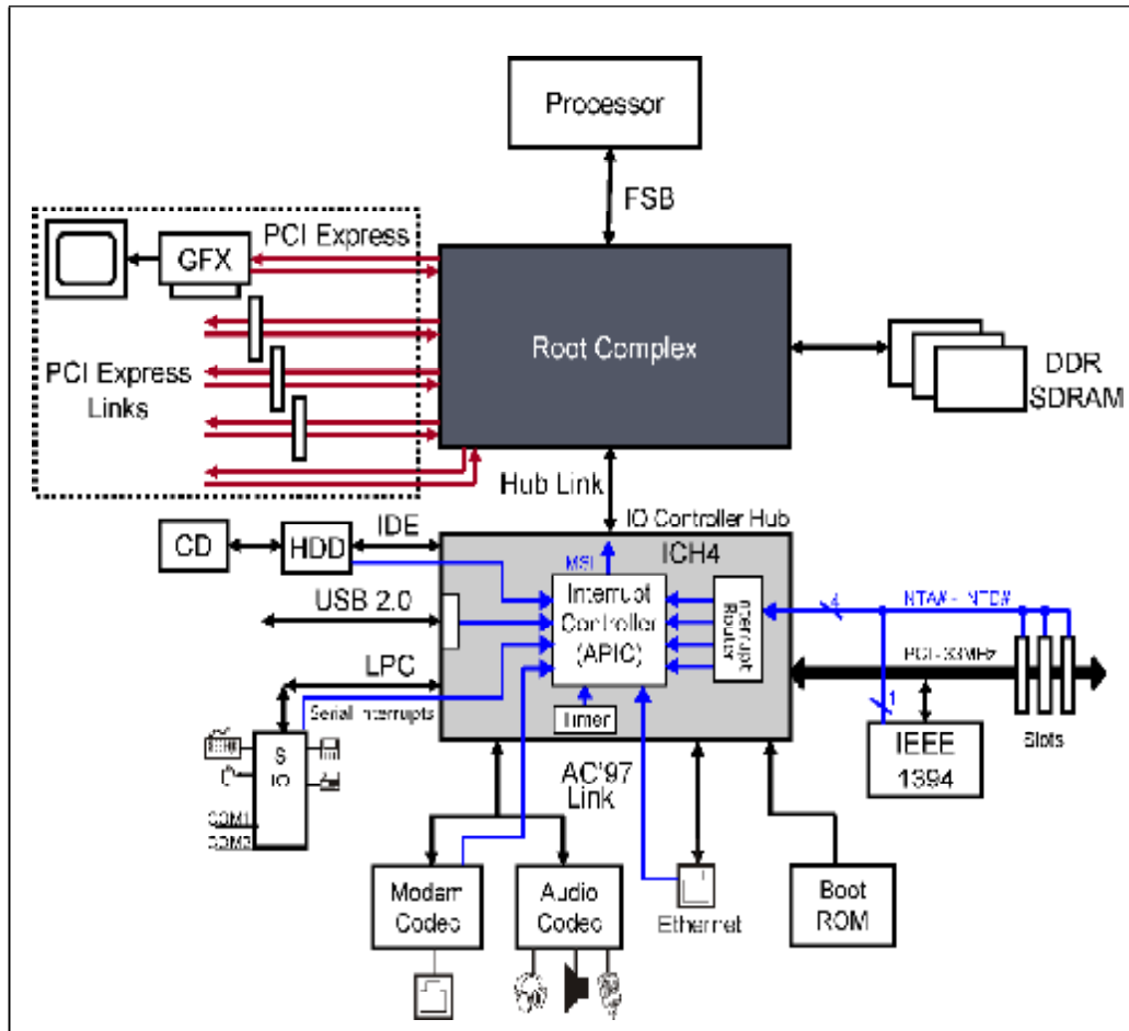
Figure 9-14: PCI Express System with PCI-Based IO Controller Hub
