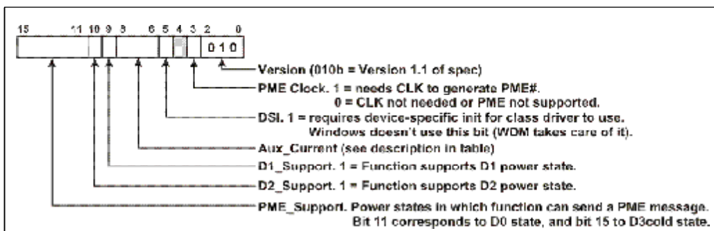
Figure 16-8: Power Management Capabilities (PMC) Register - Read Only
