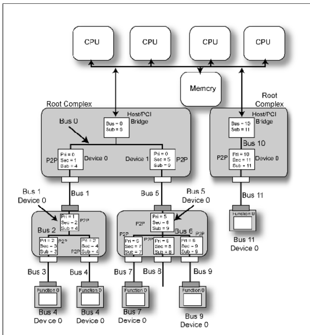
Figure 20-4: Peer Root Complexes
