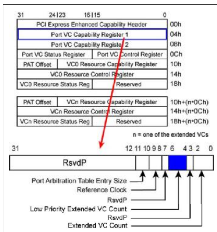
Figure 6-9: Low Priority Extended VC Count
