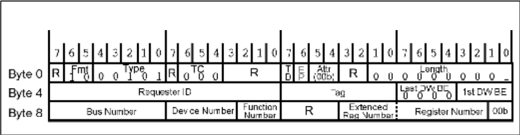
Figure 20-8: Type 1 Configuration Write Request Packet Header
