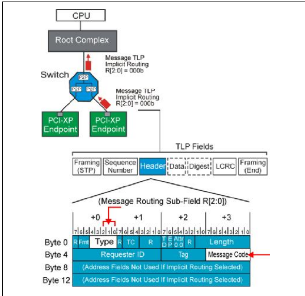
Figure 3-14: 4DW Message TLP Header Implicit Routing Fields
