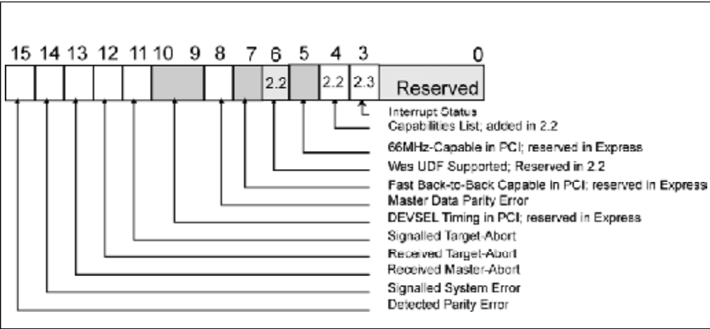
Figure 22-5: Status Register
