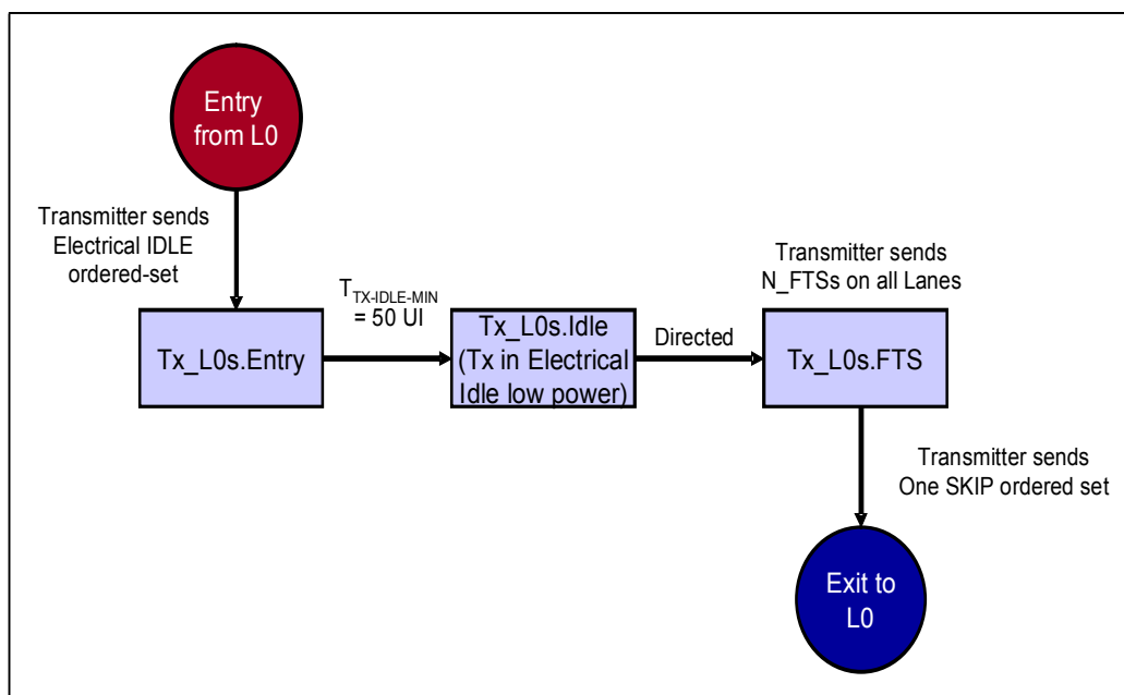
Figure 14-14: L0s Transmitter State Machine
