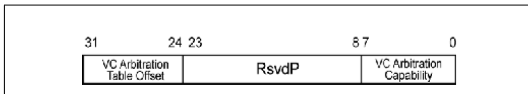
Figure 24-31: Port VC Capability Register 2 (Read-Only)
