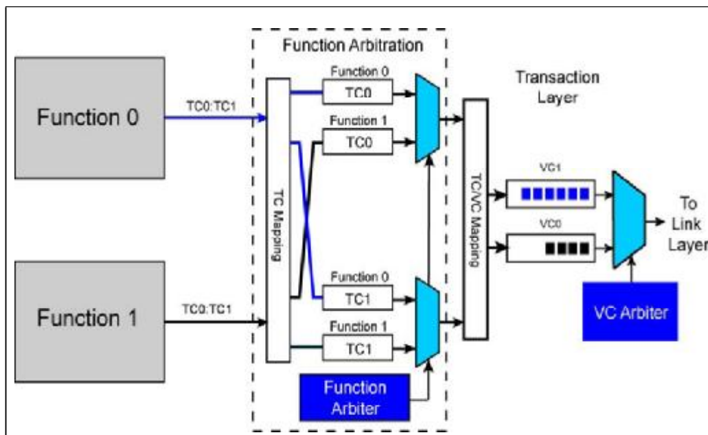
Figure 6-15: Example Multi-Function Endpoint Implementation with VC Arbitration
