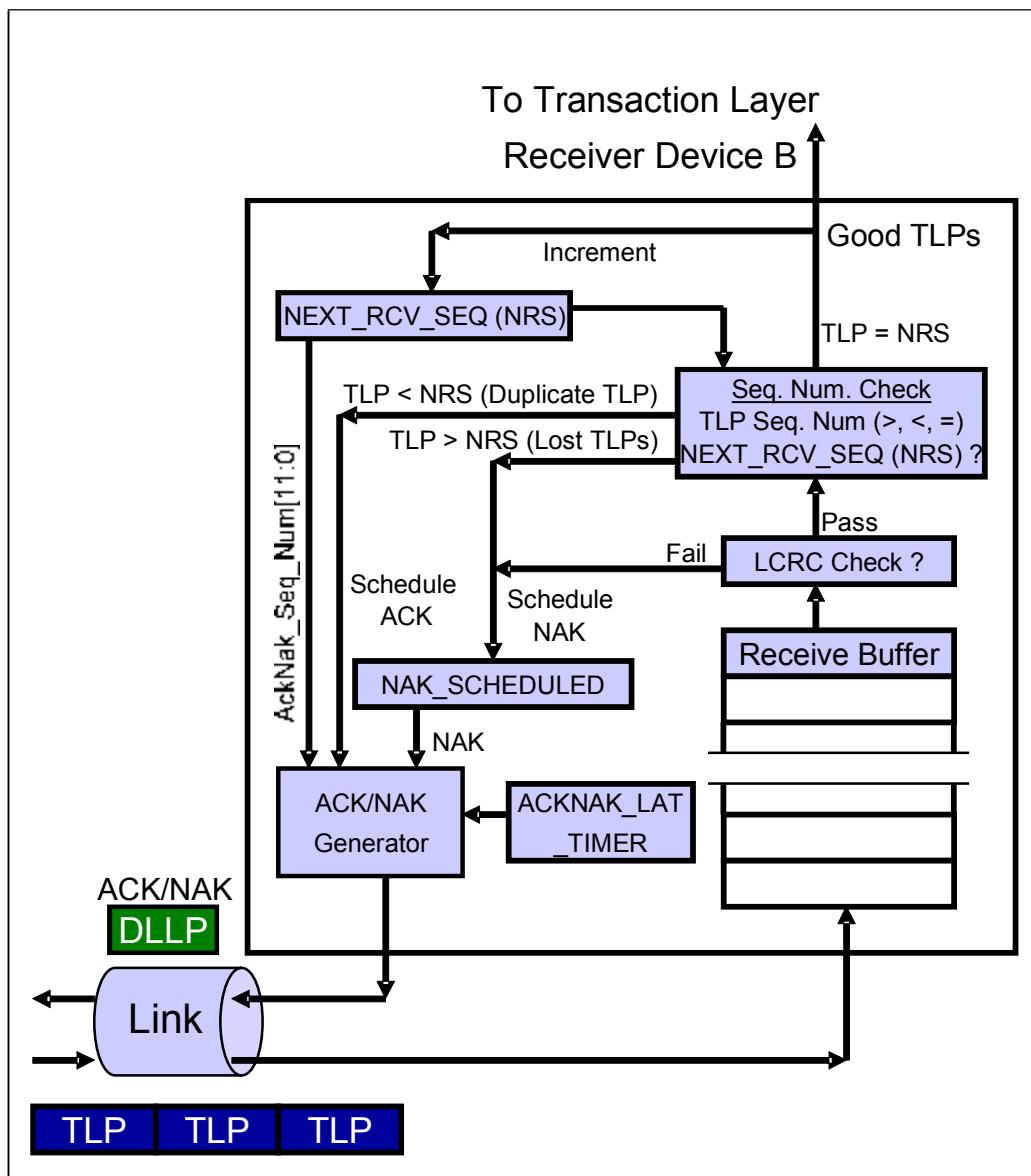
Figure 5-5: Receiver Elements Associated with the ACK/NAK Protocol
