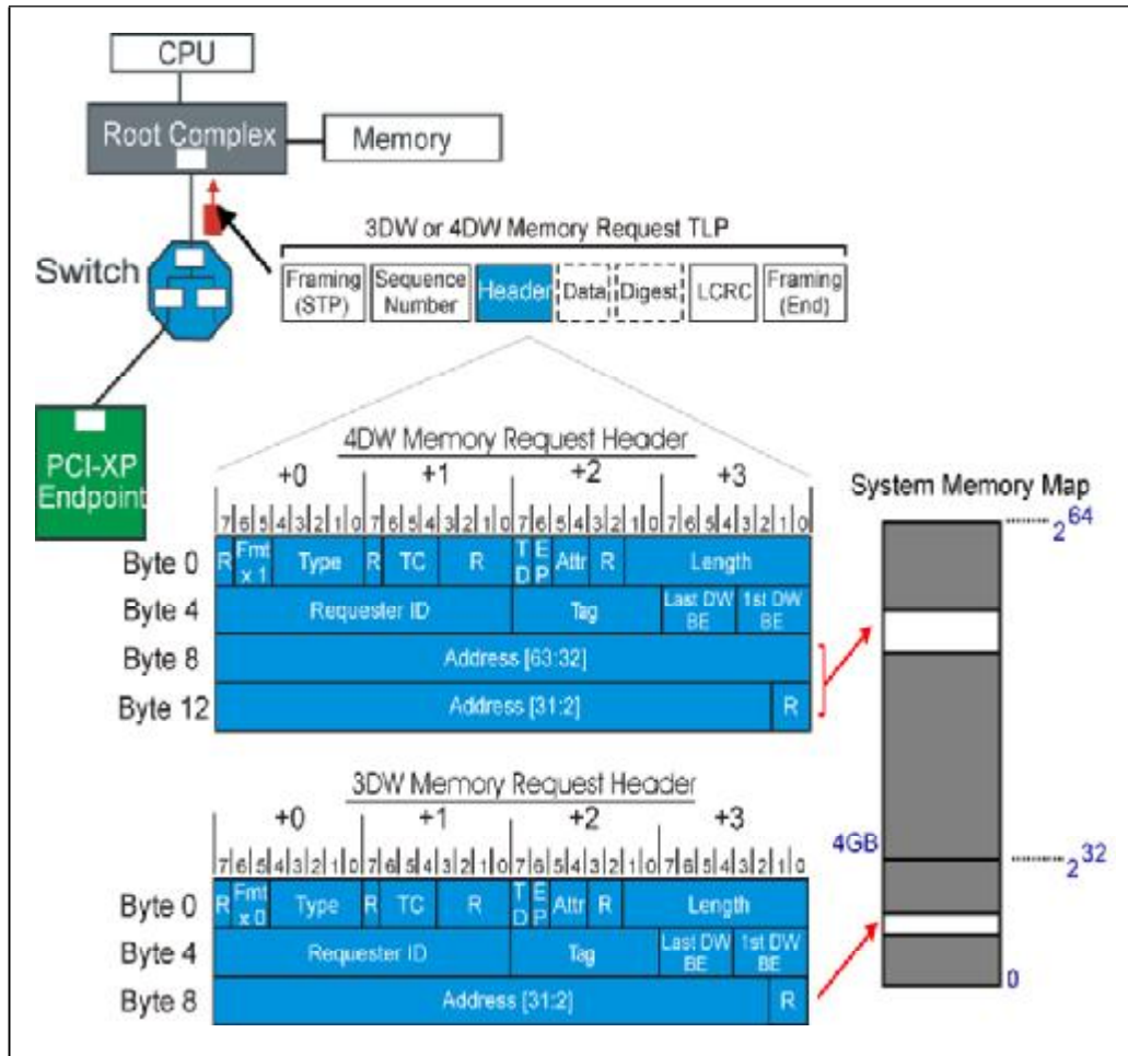
Figure 4-8: 3DW And 4DW Memory Request Header Formats
