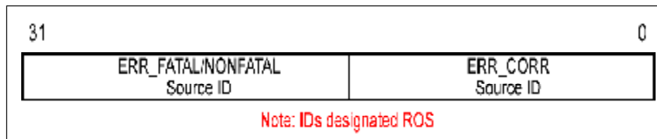
Figure 10-22: Advanced Source ID Register
