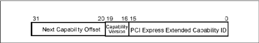
Figure 24-15: Enhanced Capability Header Register
