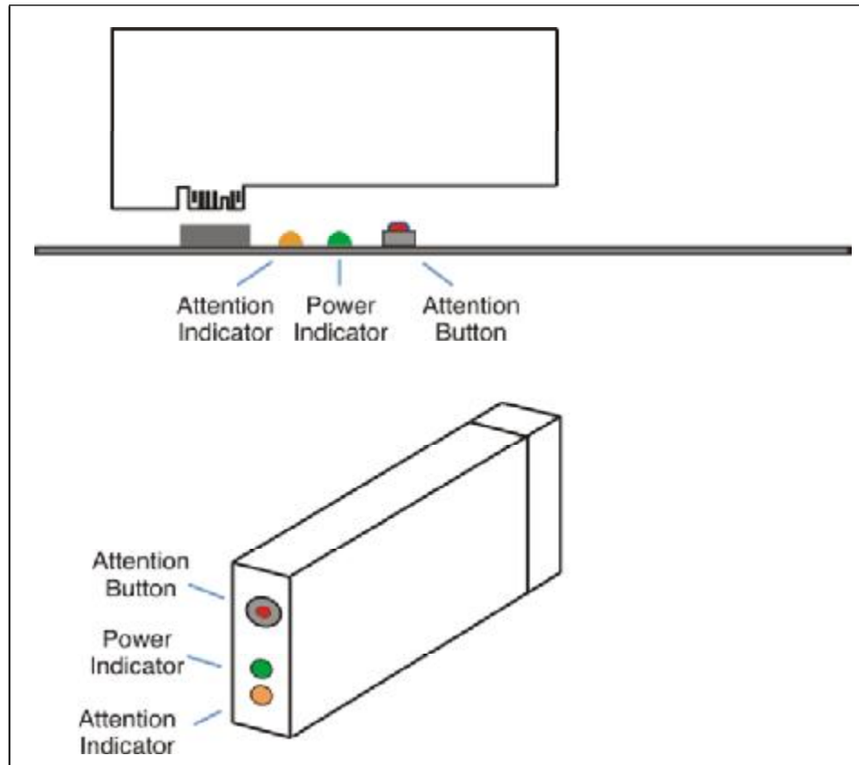
Figure 17-8: Location of Attention Button and Indicators
