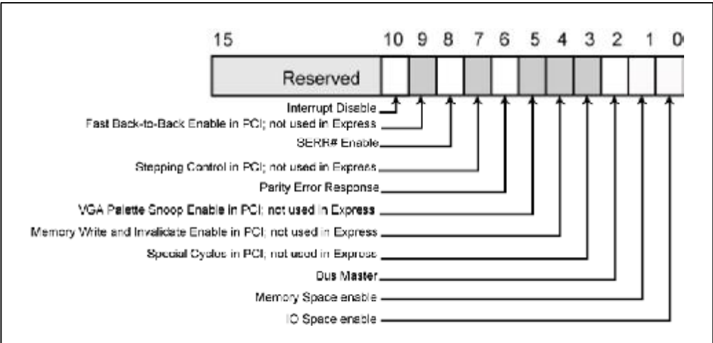
Figure 22-21: Command Register
