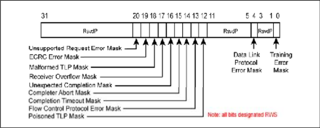
Figure 24-21: Advanced Error Uncorrectable Error Mask Register
