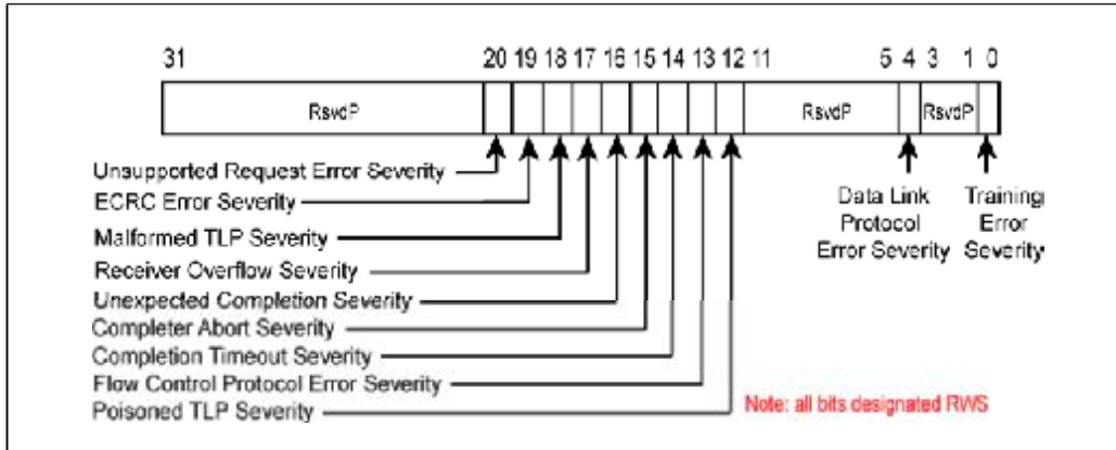
Figure 24-22: Advanced Error Uncorrectable Error Severity Register
