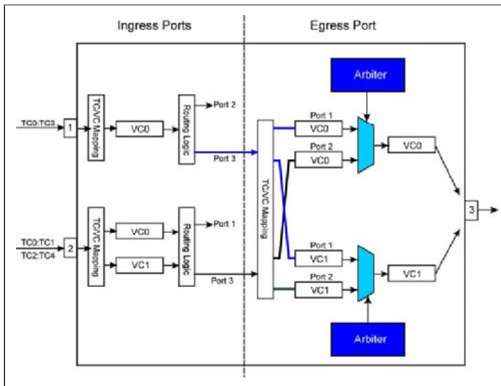
Figure 6-18: Port Arbitration Buffering
