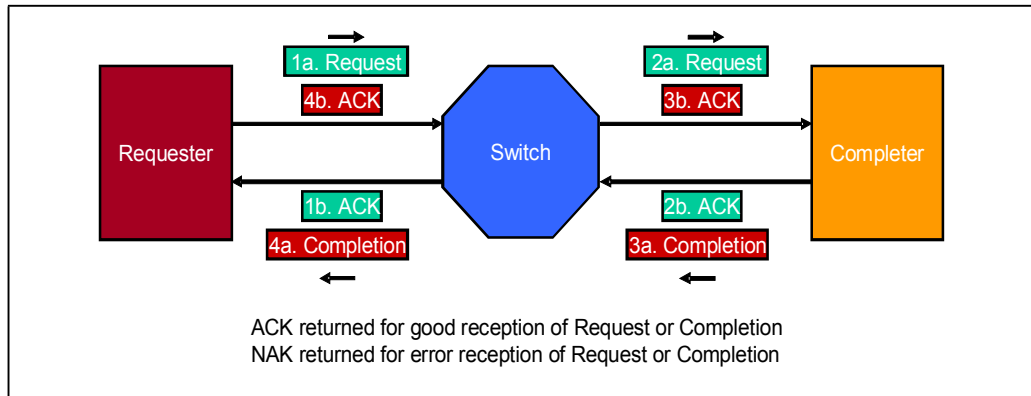
Figure 2-27: Non-Posted Transaction on Link
