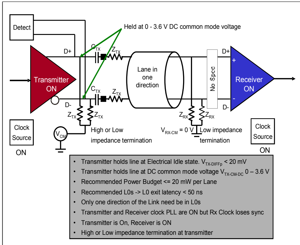
Figure 12-18: L0s Low Power Link State
