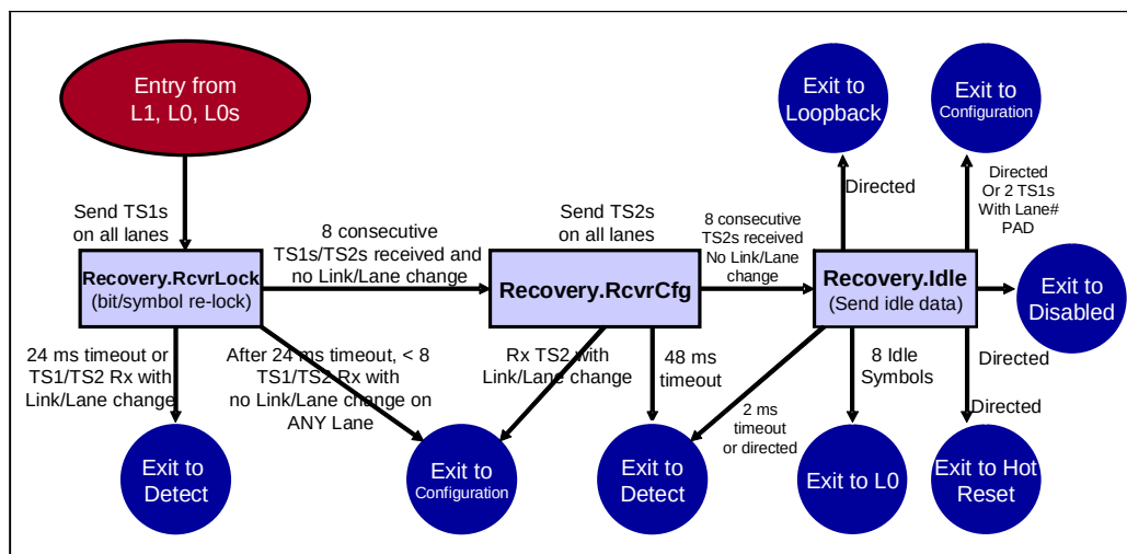
Figure 14-13: Recovery State Machine
