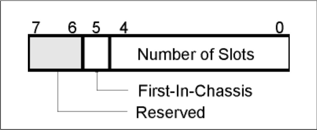
Figure 22-29: Expansion Slot Register
