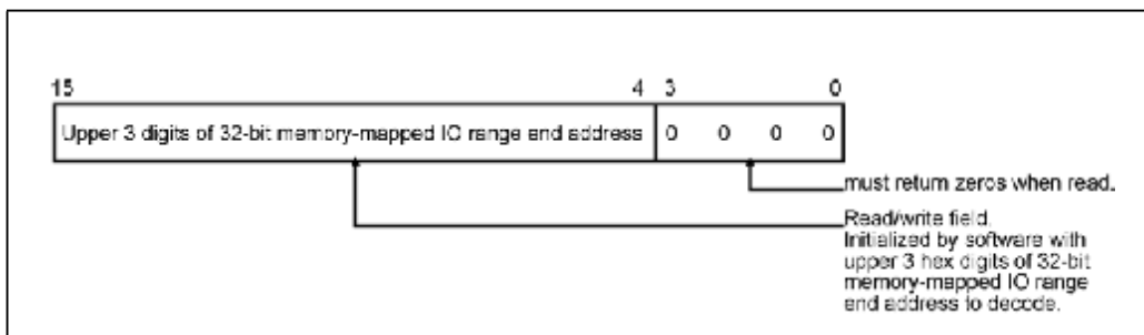
Figure 22-20: Memory-Mapped IO Limit Register
