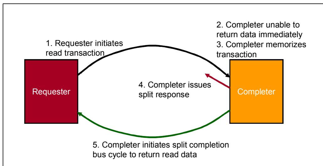
Figure 1-18: PCI-X Split Transaction Protocol
