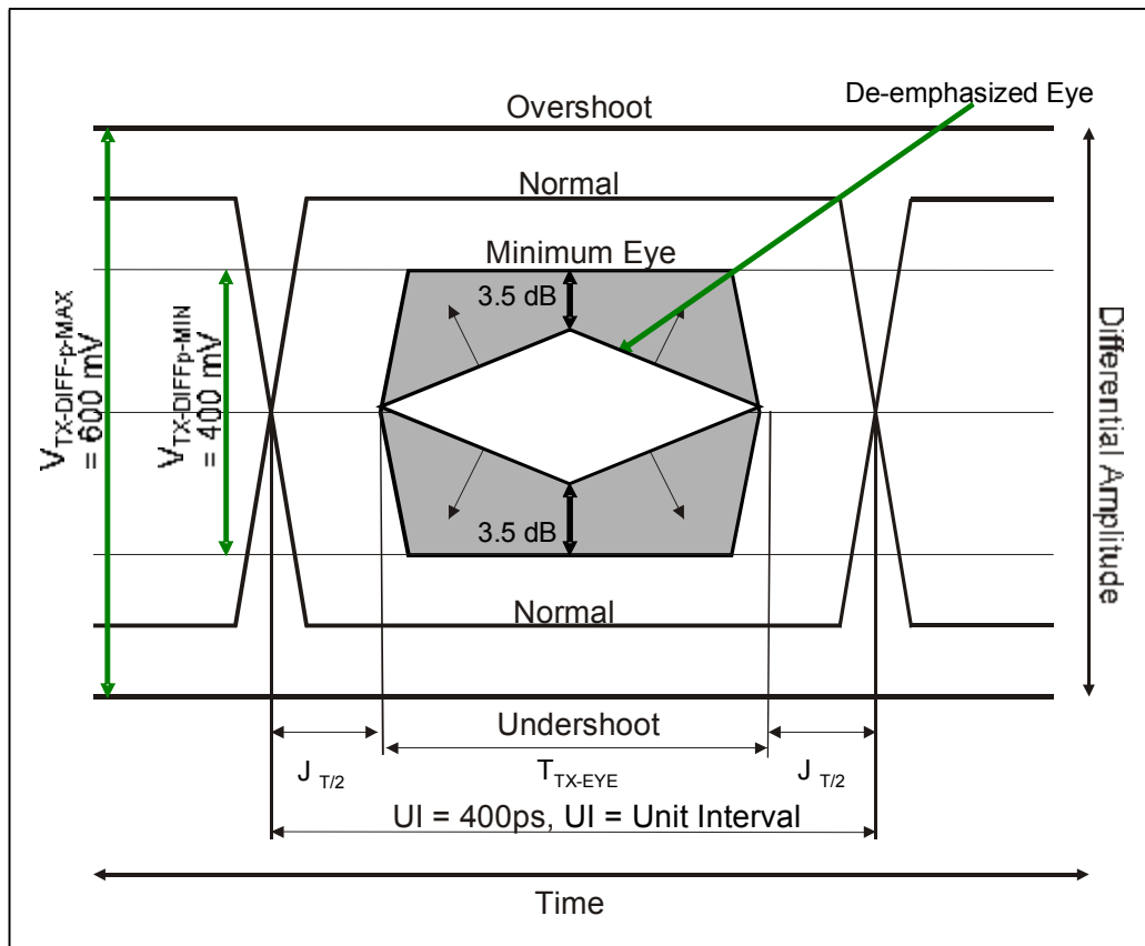
Figure 12-10: LVDS (Low-Voltage Differential Signal) Transmitter Eye Diagram
