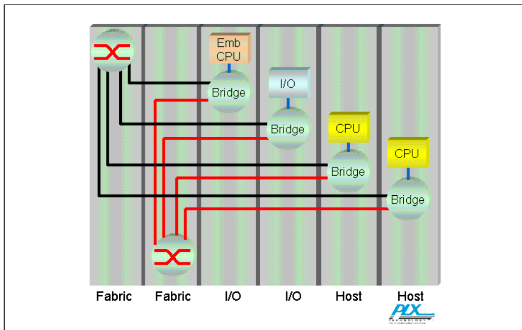
Figure B-6: PCI Express in Communications Systems
