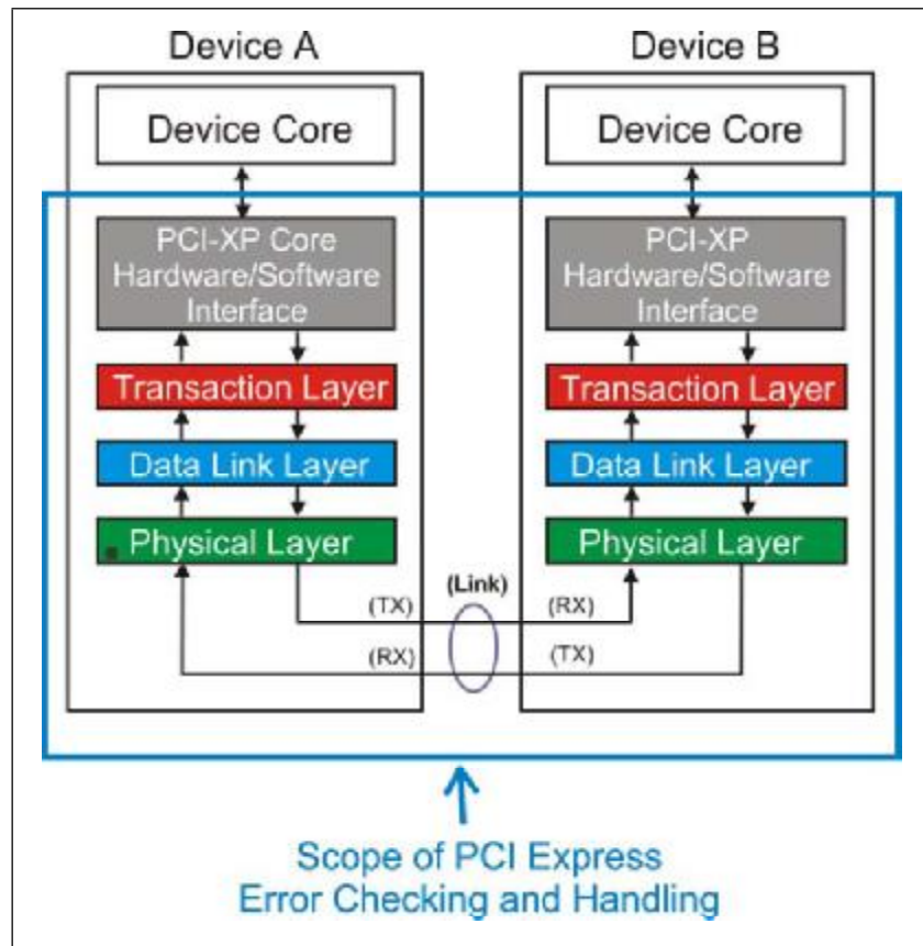
Figure 10-1: The Scope of PCI Express Error Checking and Reporting
