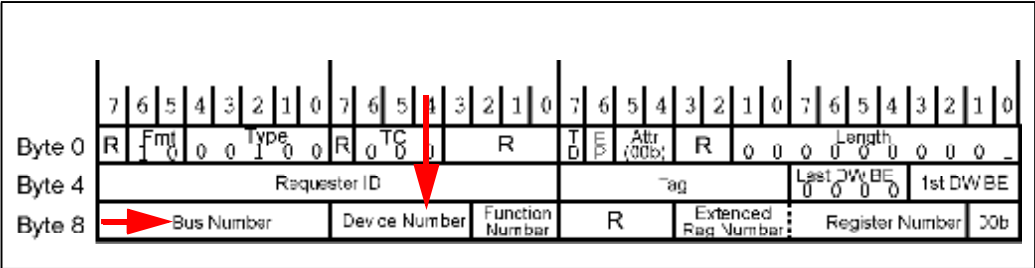
Figure 21-14: Type 0 Configuration Write Request Packet Header
