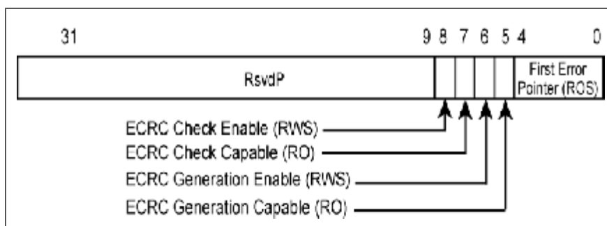
Figure 10-15: The Advanced Error Capability & Control Register
