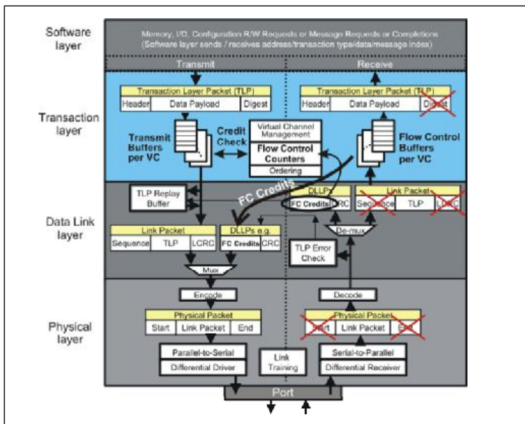
Figure 7-1: Location of Flow Control Logic
