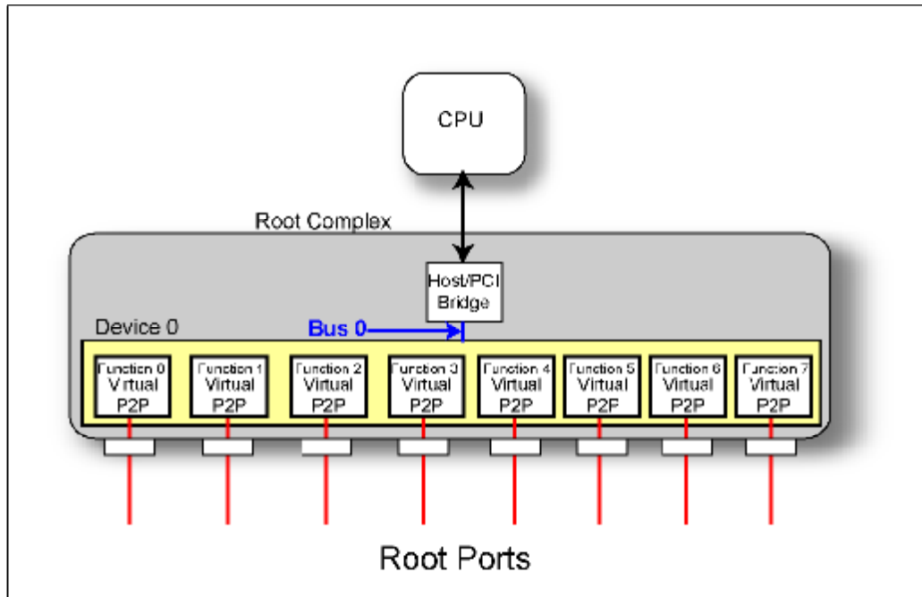
Figure 21-9: Multifunction Bridges in Root Complex
