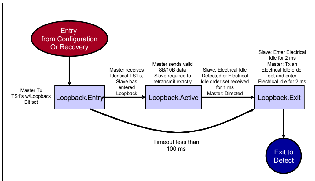
Figure 14-20: Loopback State Machine
