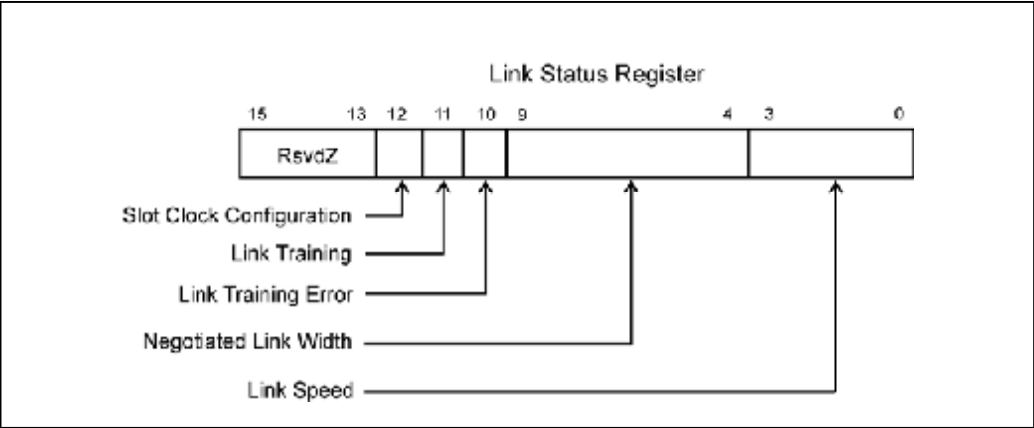
Figure 24-9: Link Status Register
