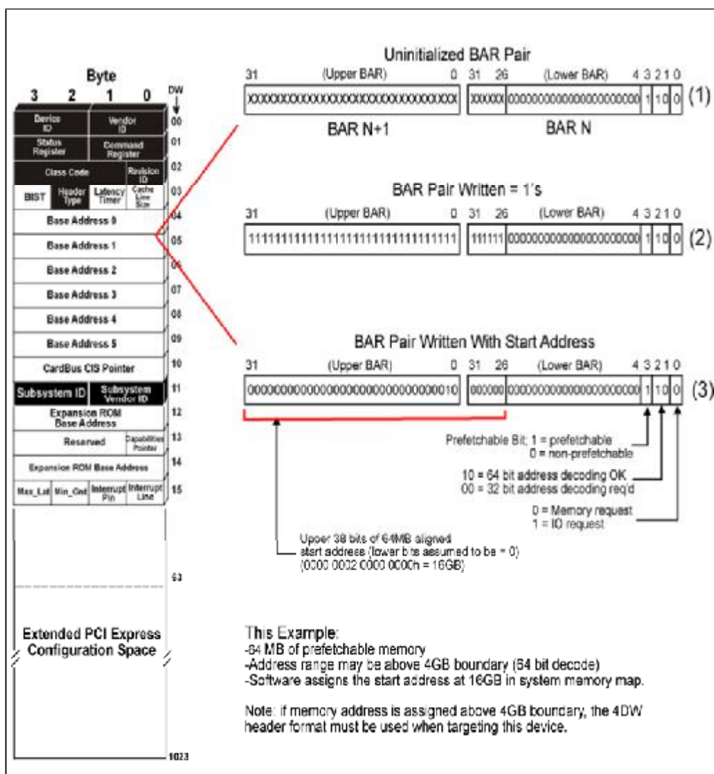
Figure 3-18: 64-Bit Prefetchable Memory BAR Set Up
