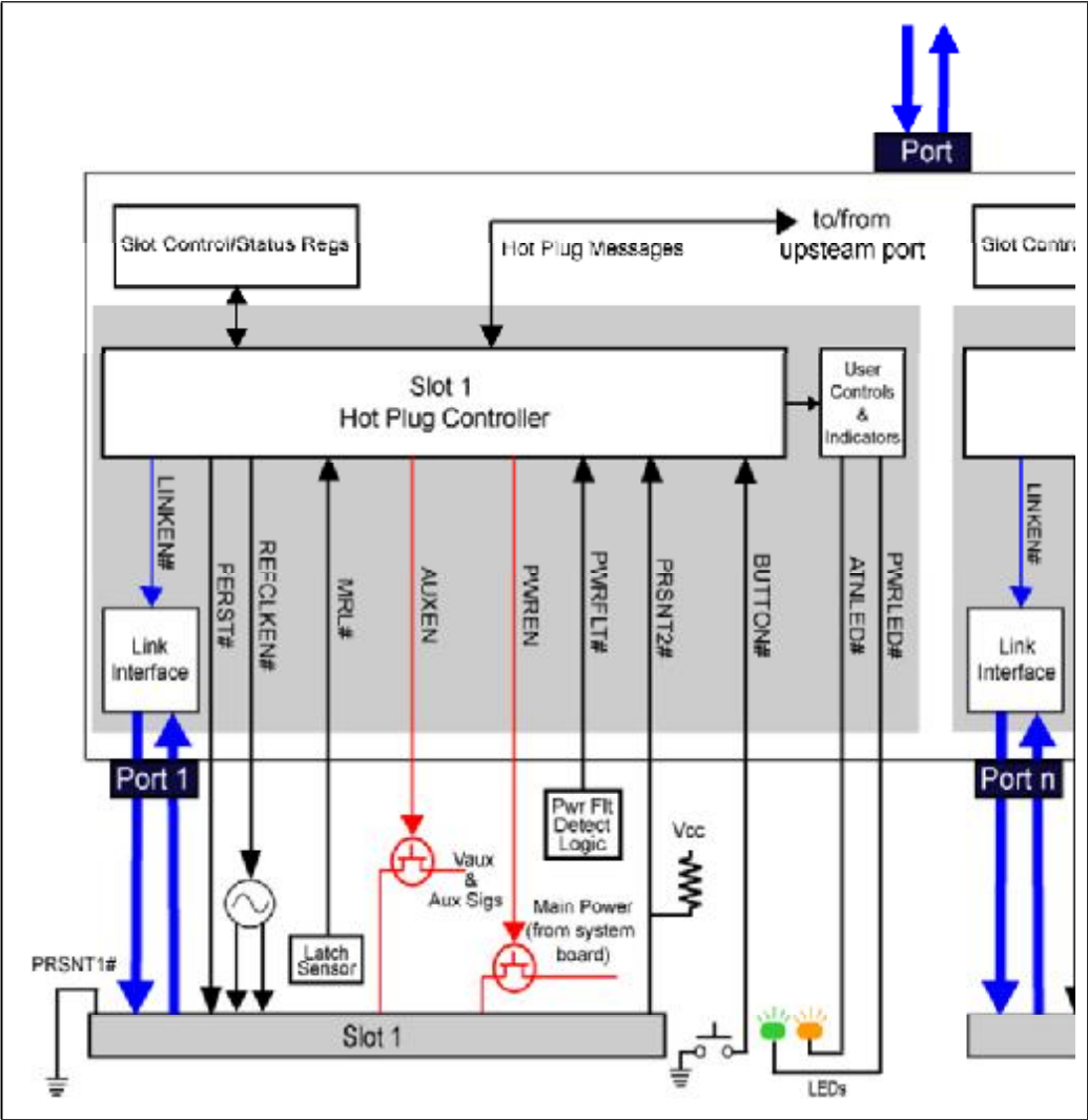
Figure 17-3: Hot Plug Control Functions within a Switch
