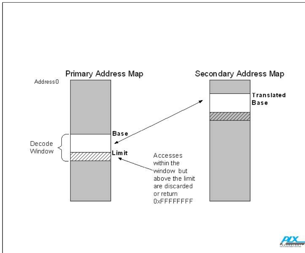
Figure C-10: Use of Limit Register
