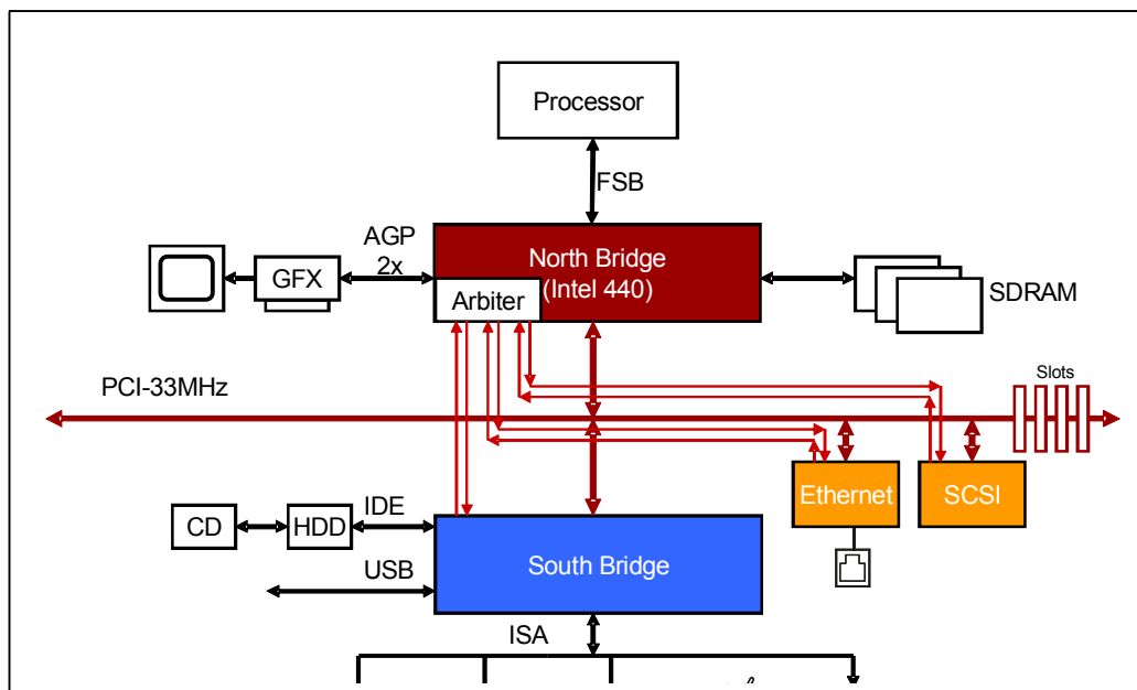
Figure 1-6: PCI Bus Arbitration
