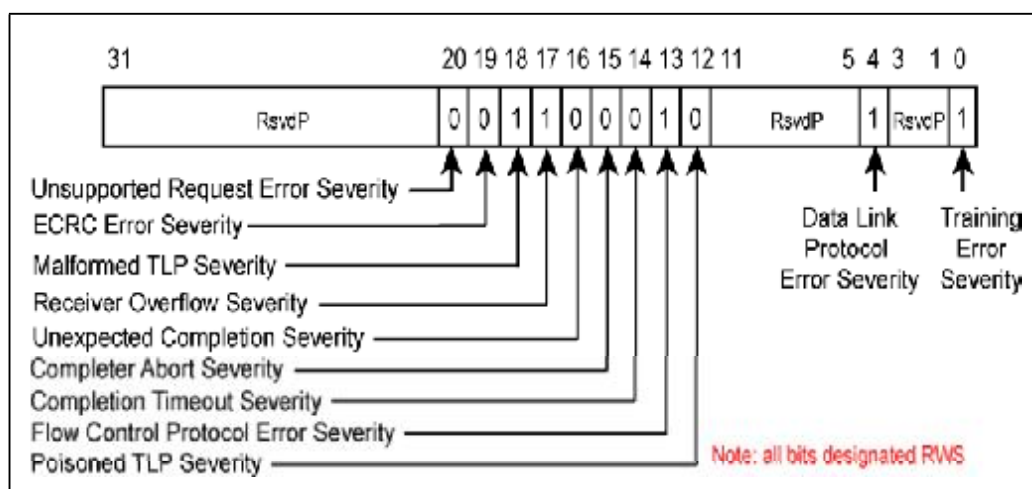
Figure 10-19: Advanced Uncorrectable Error Severity Register
