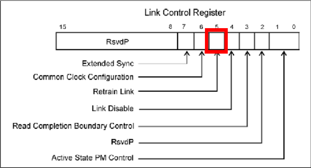
Figure 10-11: Link Control Register Allows Retraining of Link
