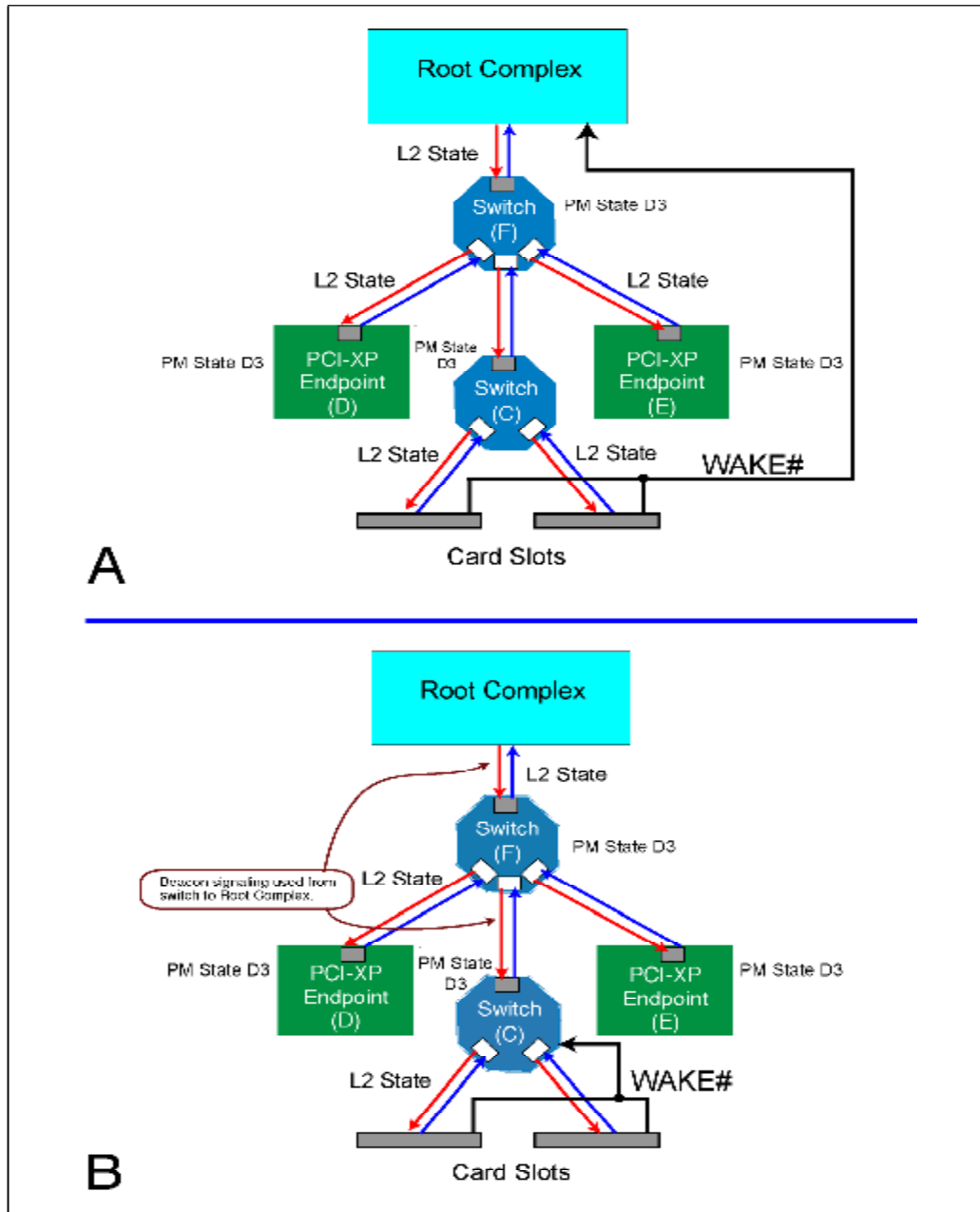
Figure 16-28: WAKE# Signal Implementations
