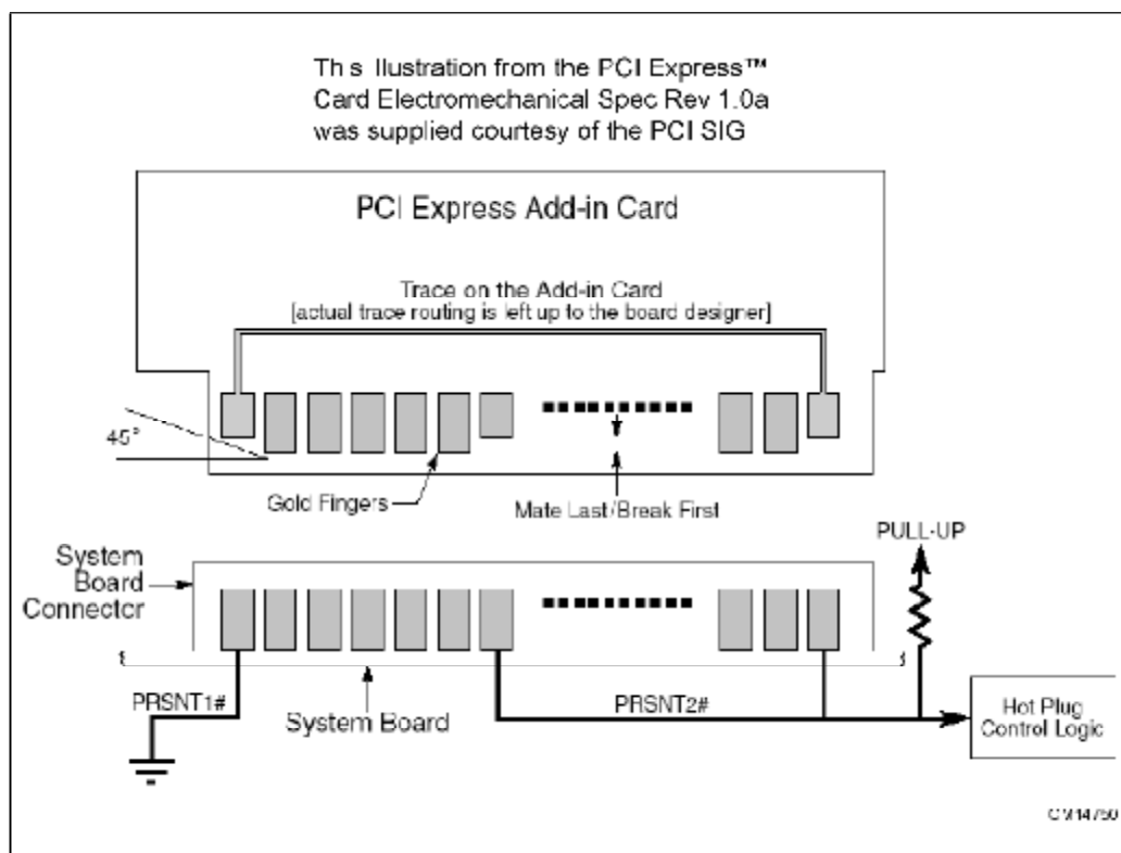
Figure 18-6: Presence Detect
