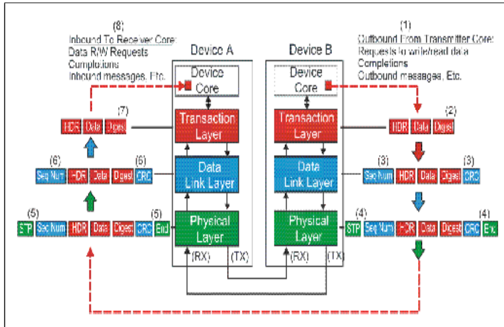
Figure 4-2: PCI Express Layered Protocol And TLP Assembly/Disassembly
