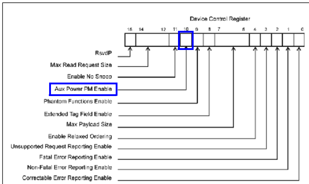
Figure 16-29: Auxiliary Current Enable for Devices Not Supporting PMEs
