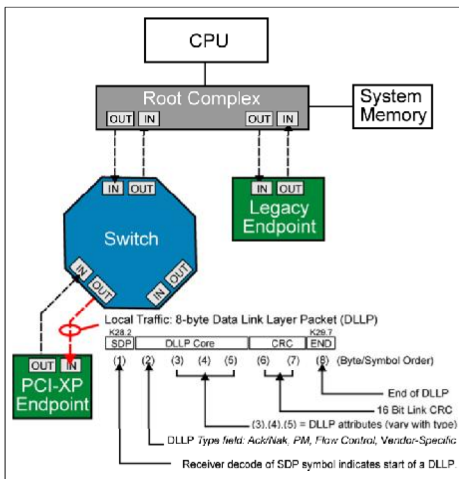
Figure 3-3: PCI Express Link Local Traffic: DLLPs
