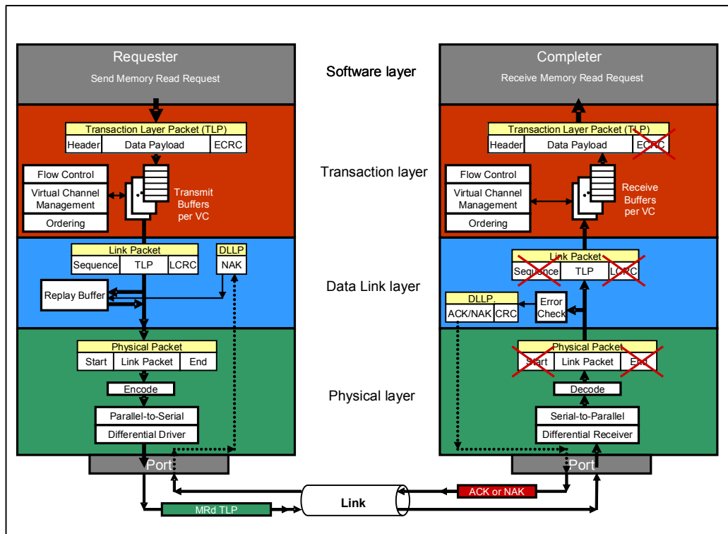
Figure 2-31: Memory Read Request Phase
