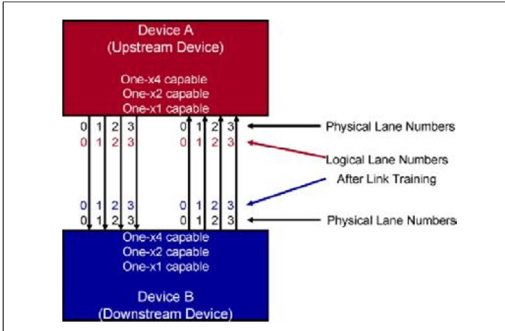
Figure 14-10: Example 1 Link Numbering and Lane Numbering
