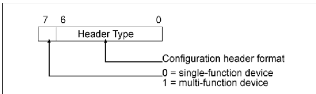
Figure 21-4: Header Type Register
