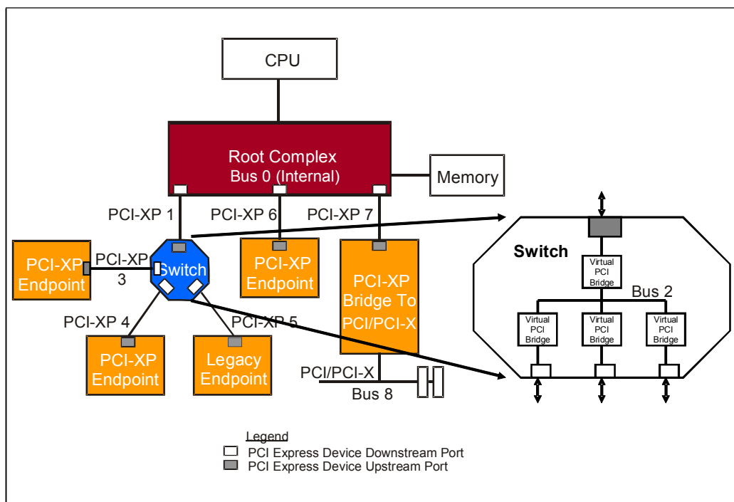
Figure 1-22: PCI Express Topology
