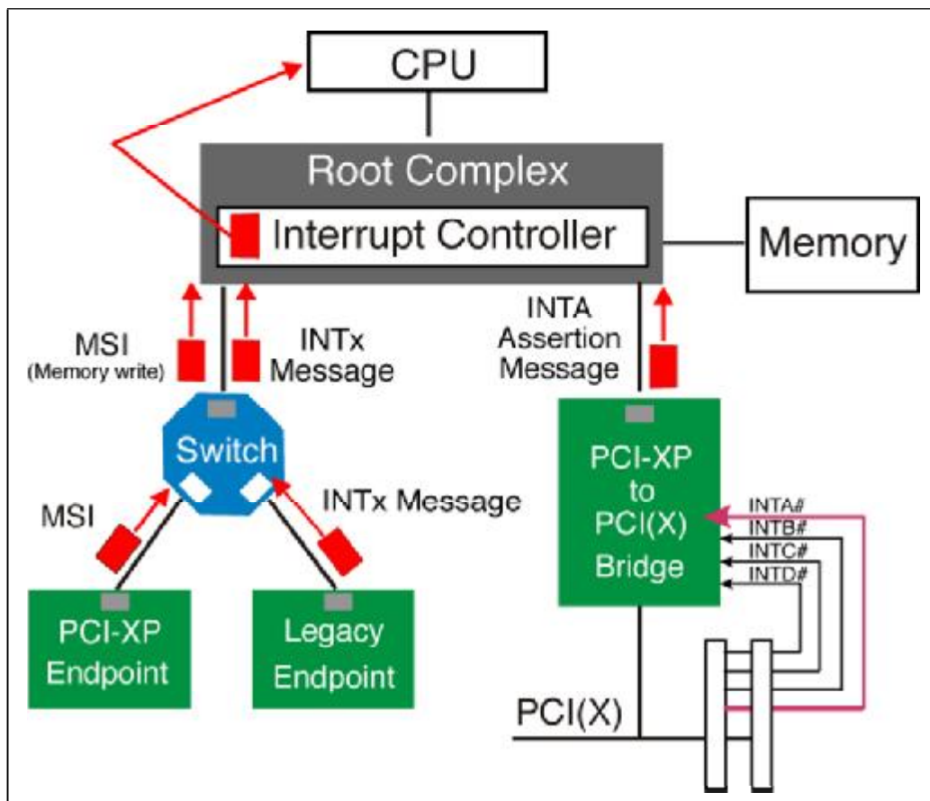
Figure 9-1: Native PCI Express and Legacy PCI Interrupt Delivery
