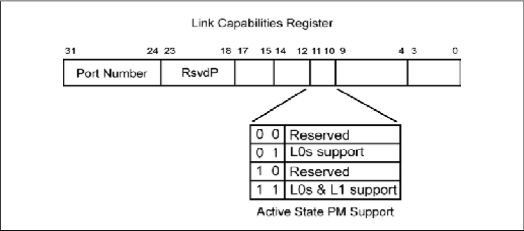
Figure 16-12: ASPM Support
