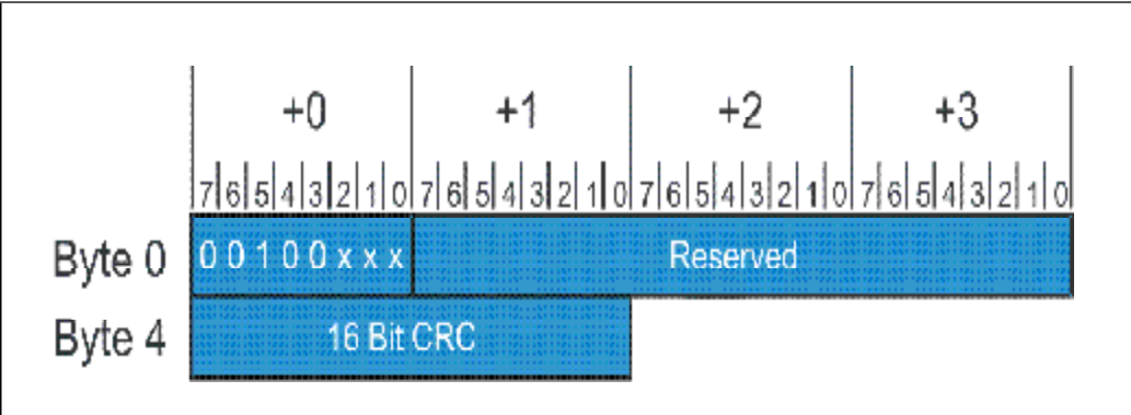
Figure 4-15: Power Management DLLP Packet Format
