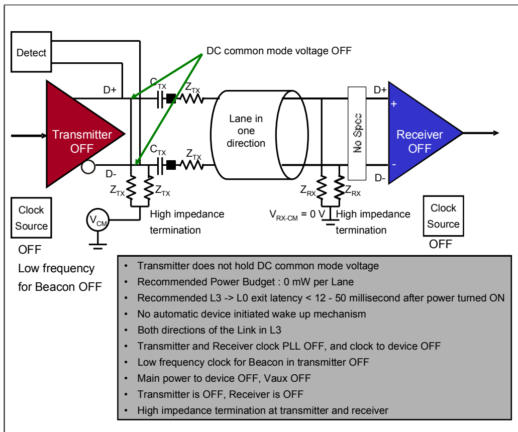
Figure 12-21: L3 Link Off State
