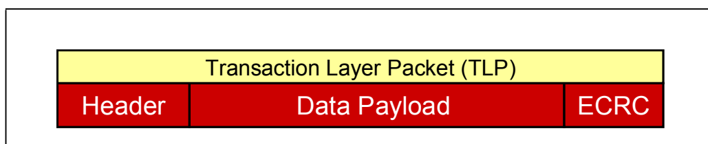
Figure 2-20: TLP Structure at the Transaction Layer
