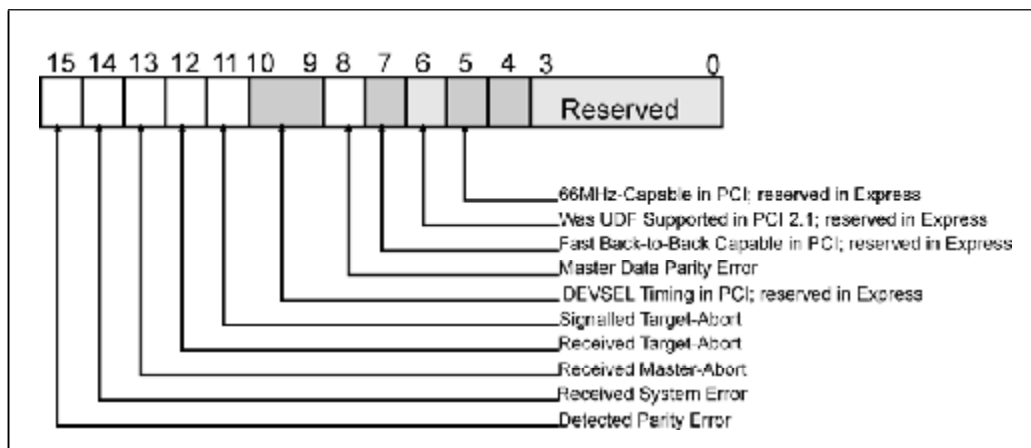
Figure 22-24: Secondary Status Register
