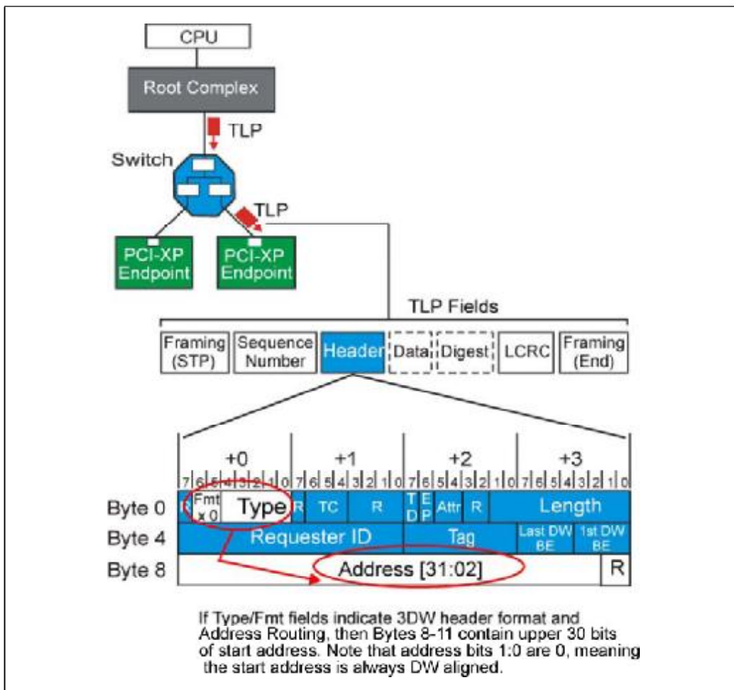
Figure 3-7: 3DW TLP Header Address Routing Fields
