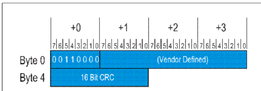
Figure 4-17: Vendor Specific DLLP Packet Format
