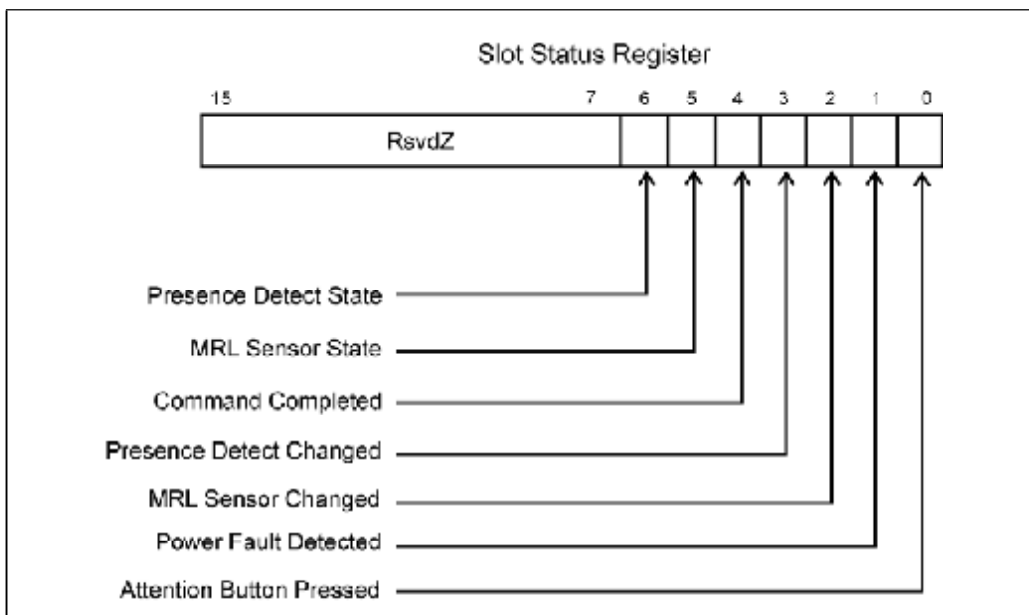
Figure 17-7: Slot Status Register Fields
