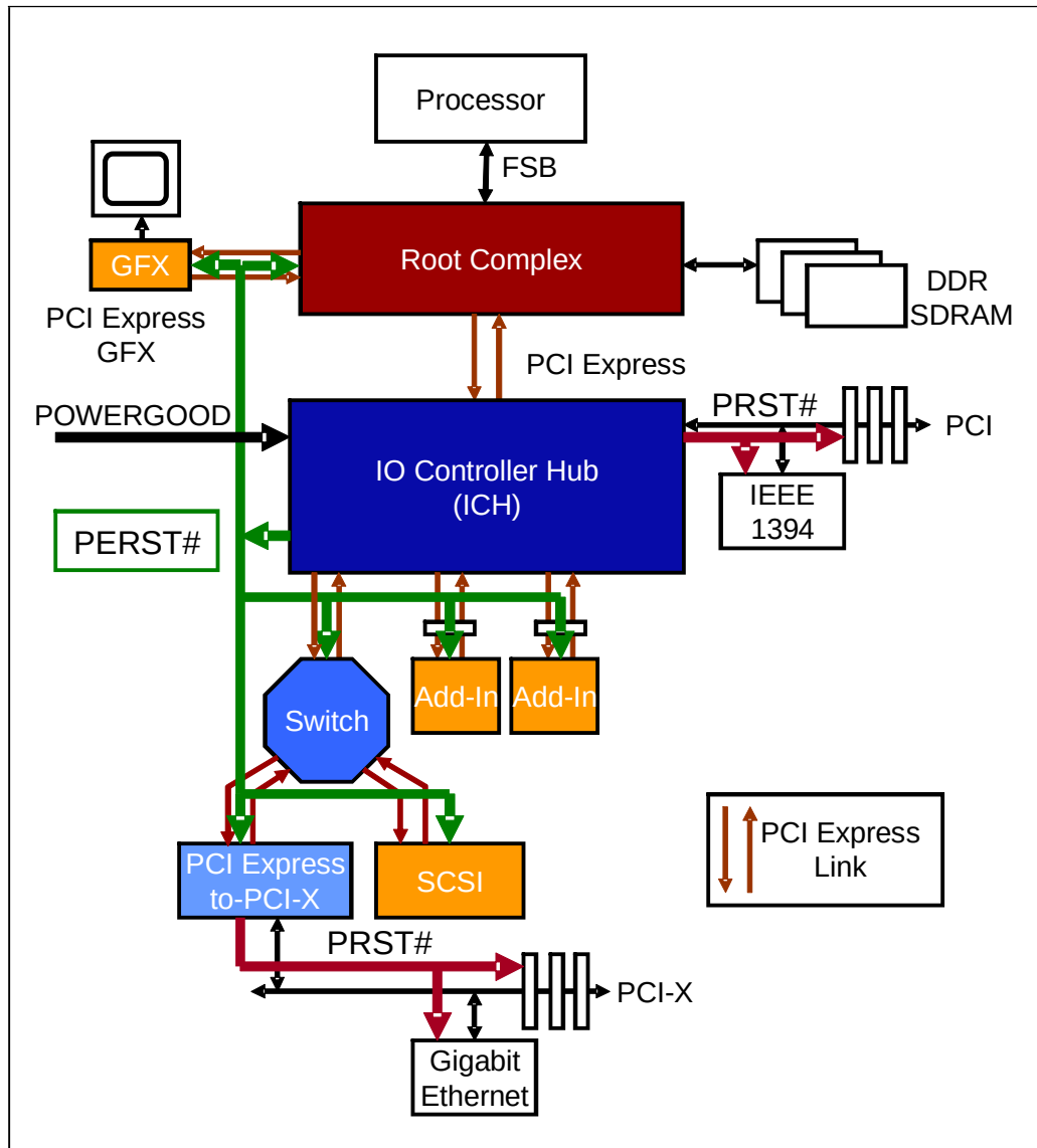
Figure 13-1: PERST# Generation
