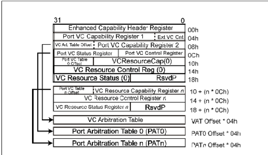
Figure 24-28: Virtual Channel Capability Register Set
