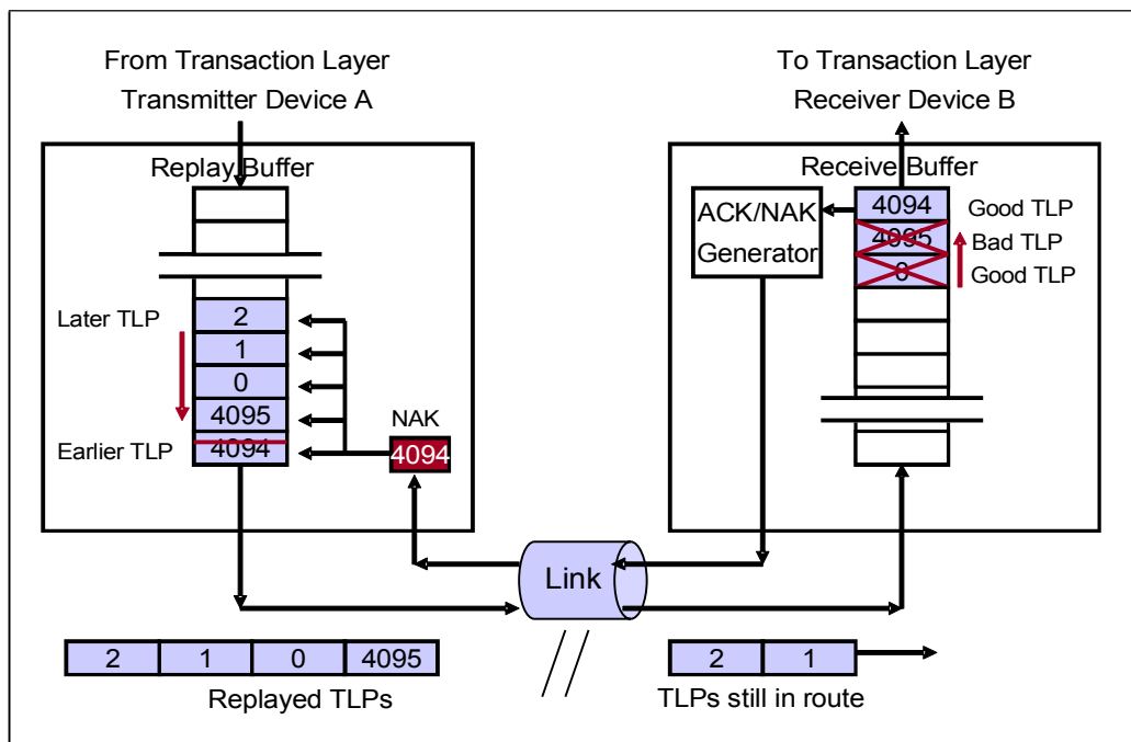
Figure 5-9: Example that Shows Transmitter Behavior on Receipt of a NAK DLLP
