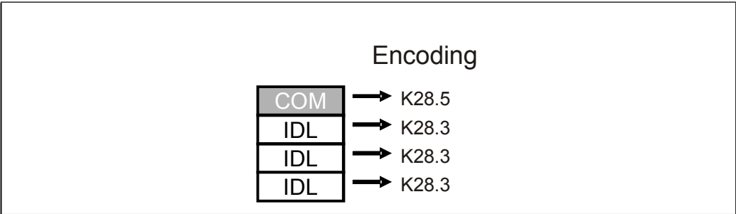
Figure 12-6: Electrical Idle Ordered-Set
