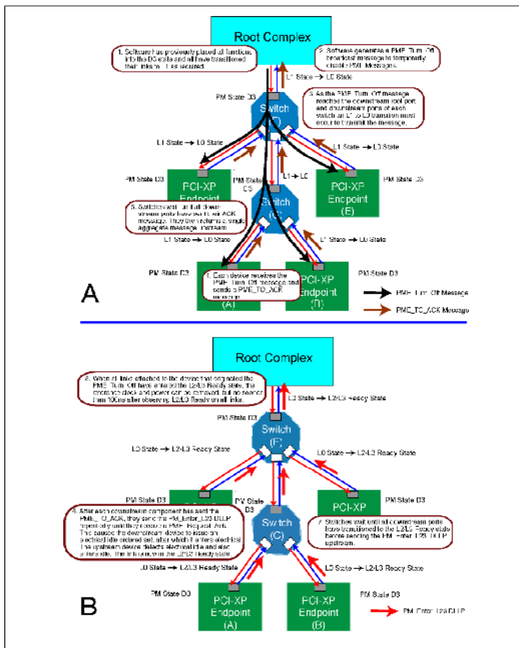
Figure 16-25: Negotiation for Entering L2/L3 Ready State
