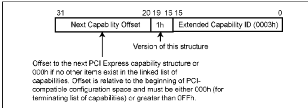
Figure 24-37: Device Serial Number Enhanced Capability Header
