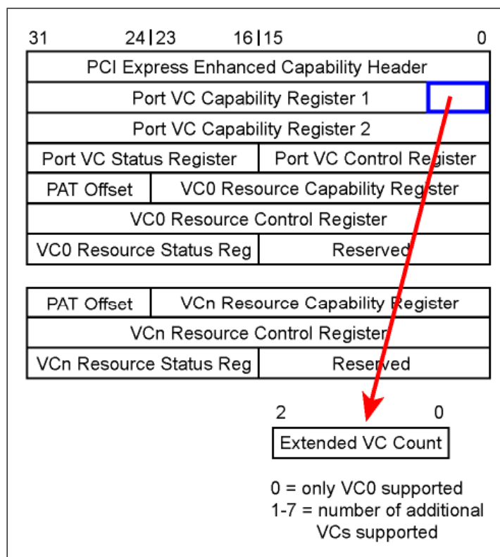
Figure 6-4: Extended VCs Supported Field
