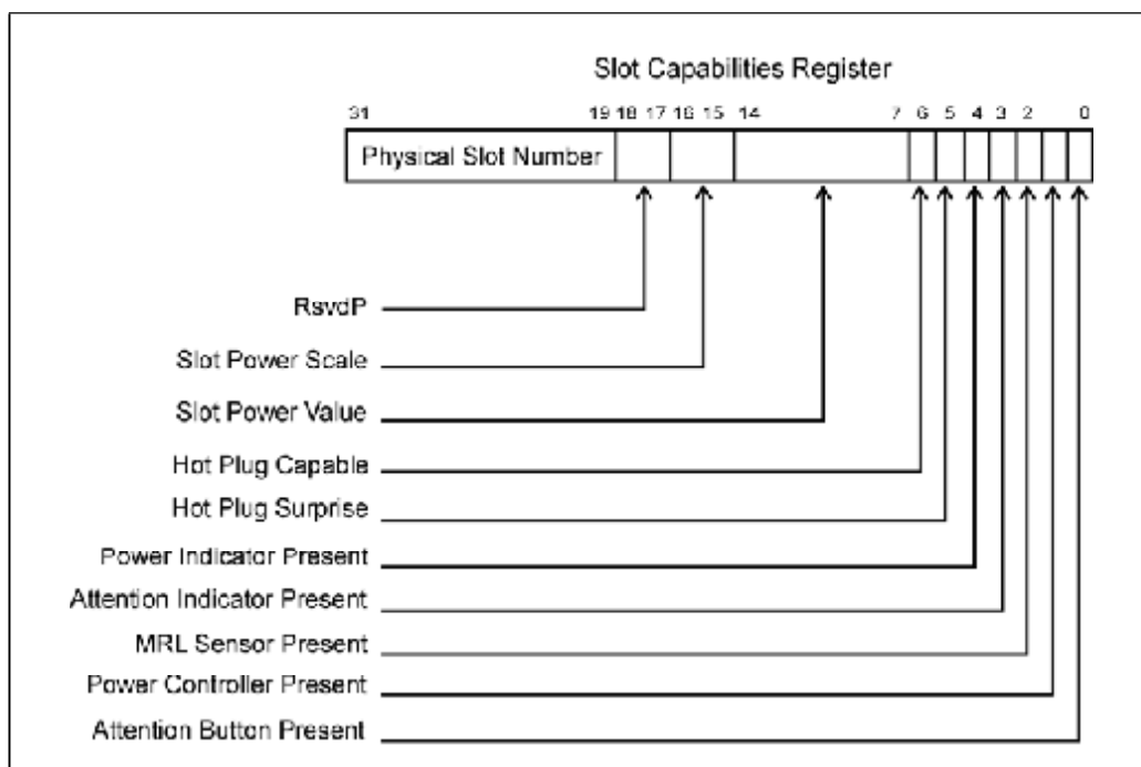
Figure 22-30: Slot Capability Register
