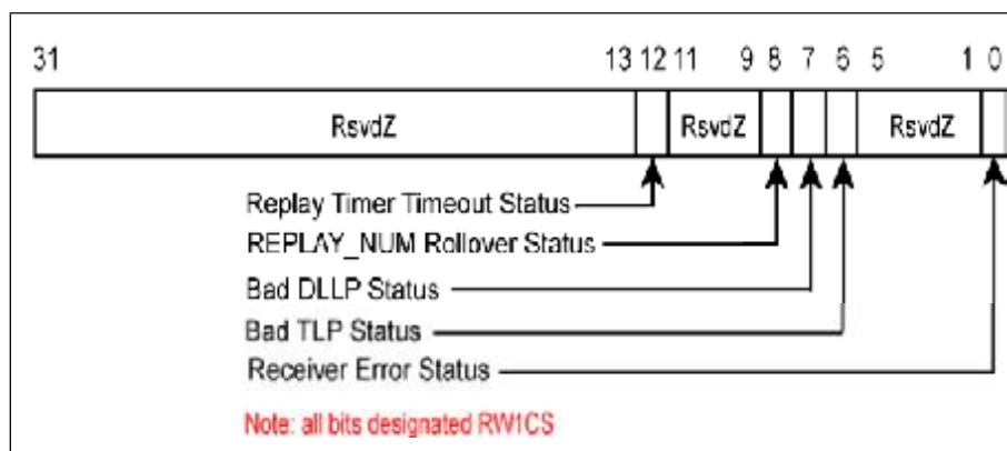
Figure 10-16: Advanced Correctable Error Status Register
