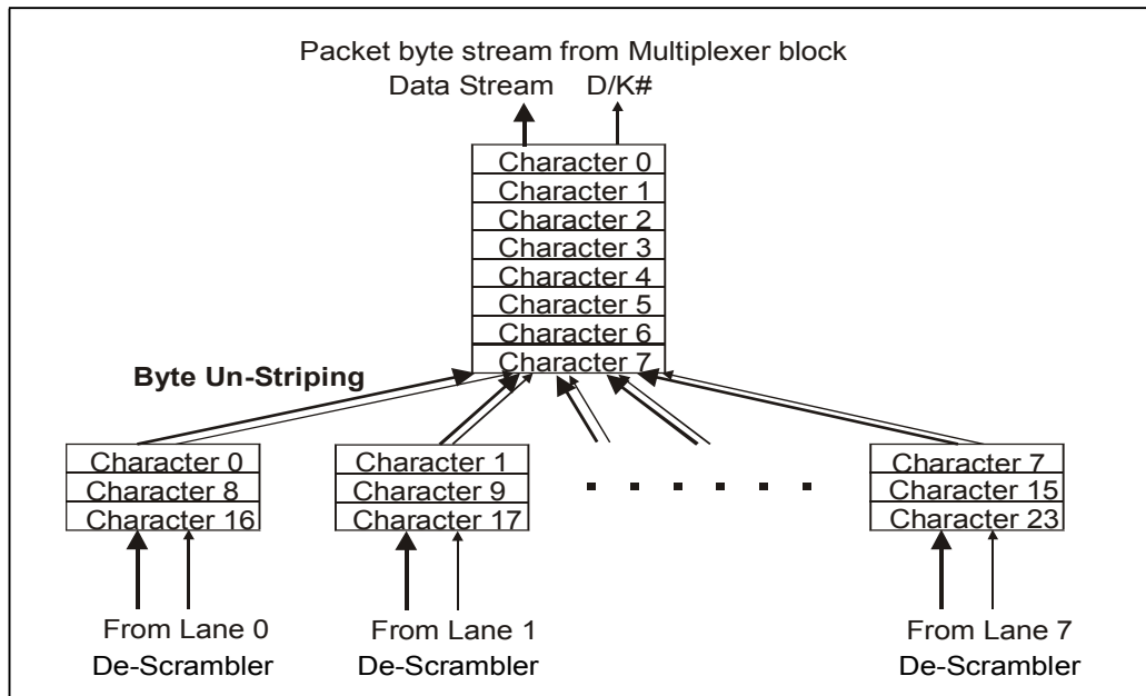
Figure 11-25: Example of x8 Byte Un-Striping
