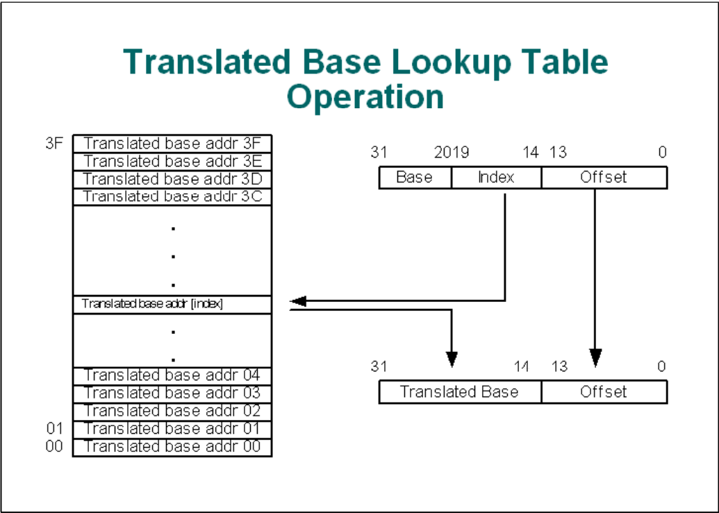
Figure C-9: Lookup Table Based Translation
