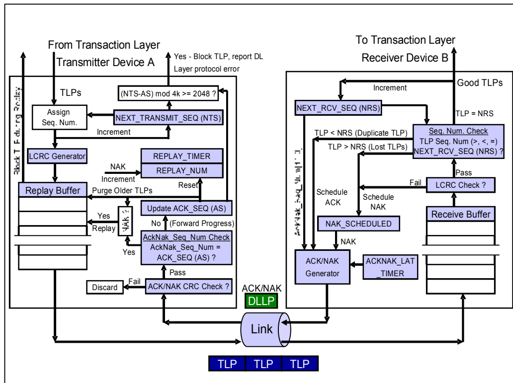
Figure 5-3: Elements of the ACK/NAK Protocol
