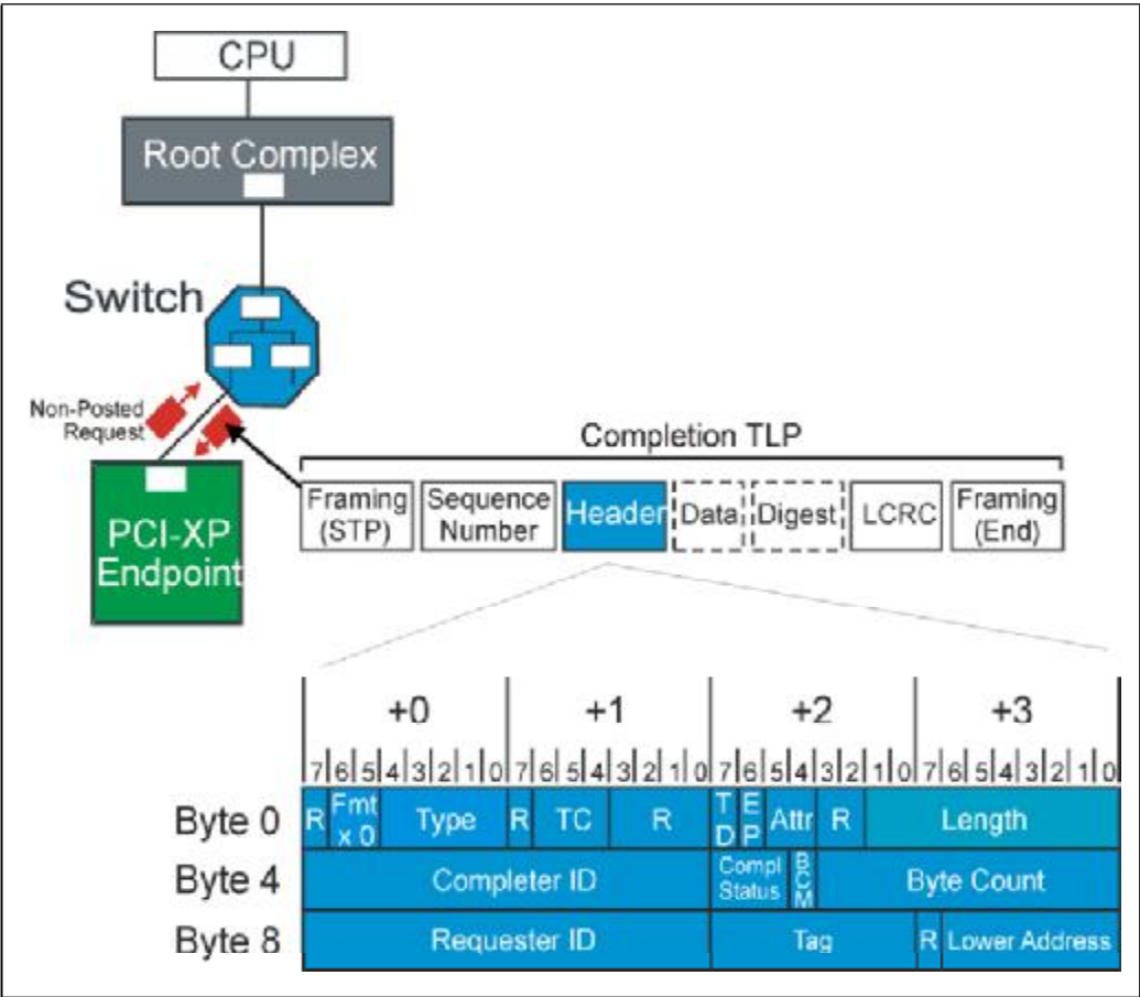
Figure 4-10: 3DW Completion Header Format
