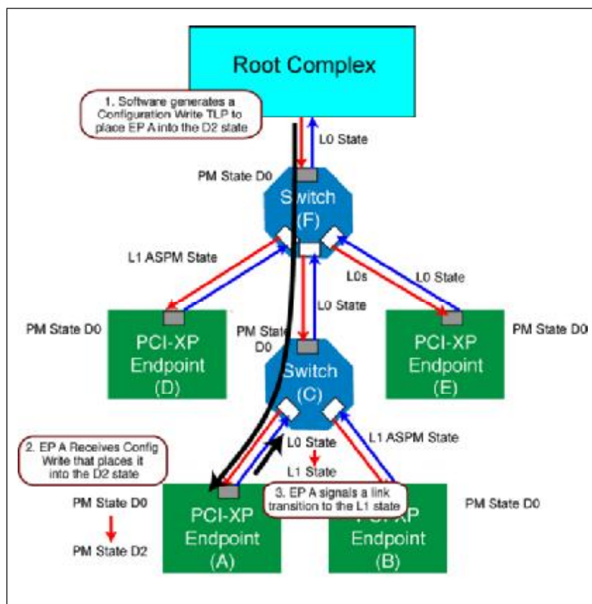
Figure 16-22: Software Placing a Device into a D2 State and Subsequent Transition to L1
