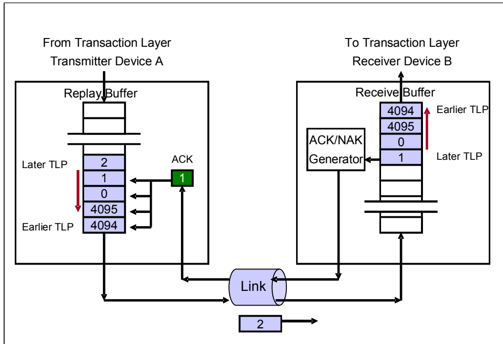
Figure 5-8: Example 2 that Shows Transmitter Behavior with Receipt of an ACK DLLP
