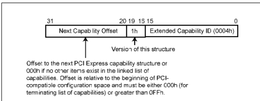
Figure 24-41: Power Budgeting Enhanced Capability Header
