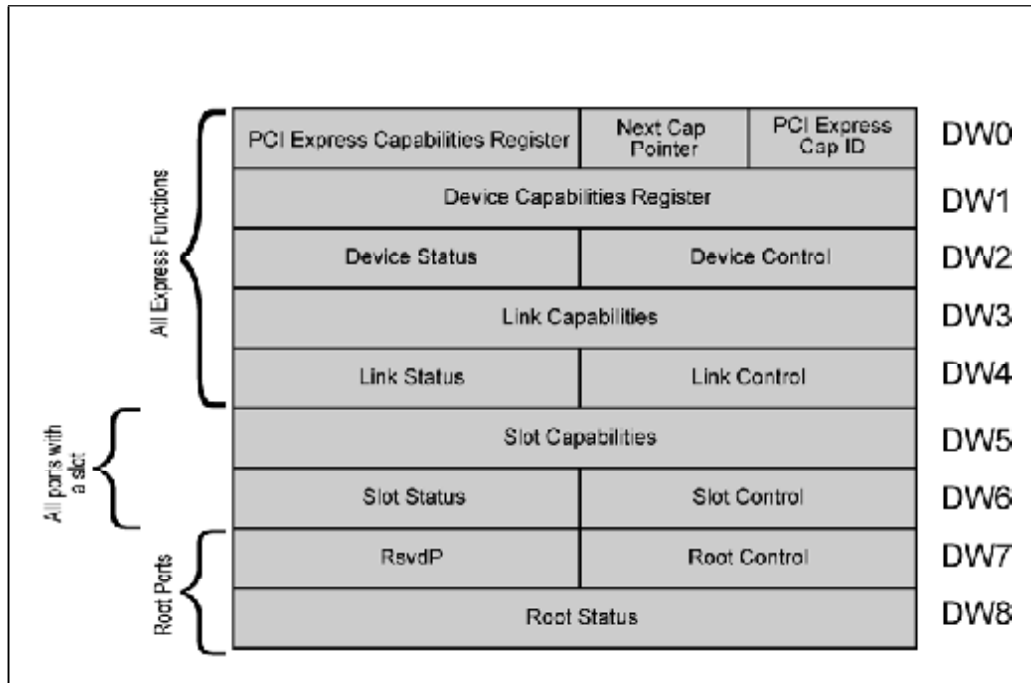
Figure 24-2: PCI Express Capability Register Set
