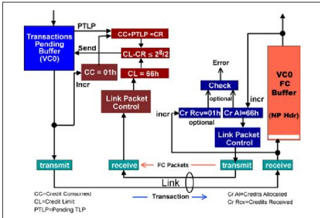
Figure 7-6: Flow Control Elements Following Delivery of First Transaction
