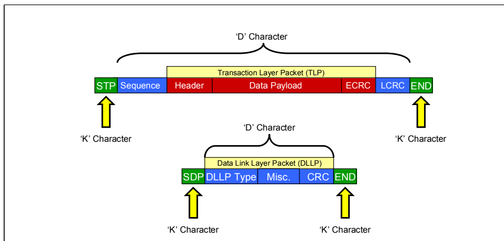
Figure 11-6: TLP and DLLP Packet Framing with Start and End Control Characters
