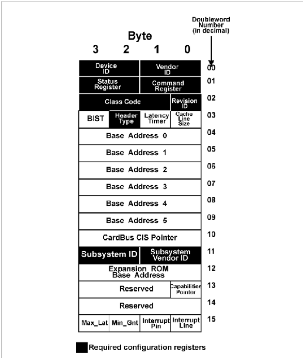
Figure 21-6: Header Type 0
