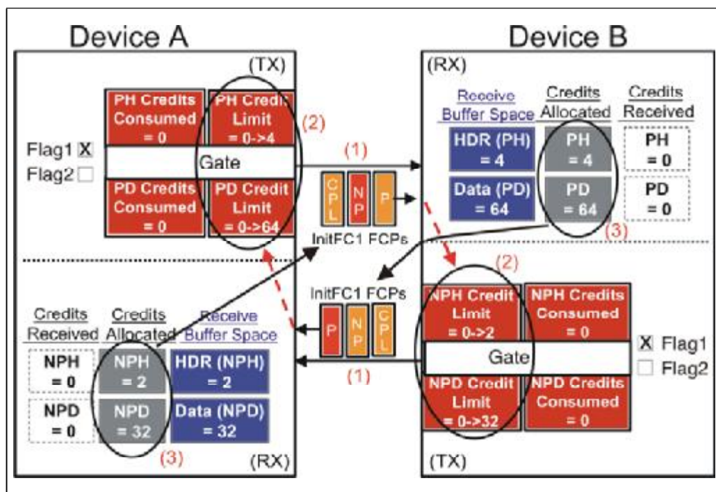
Figure 7-11: Devices Send and Initialize Flow Control Registers
