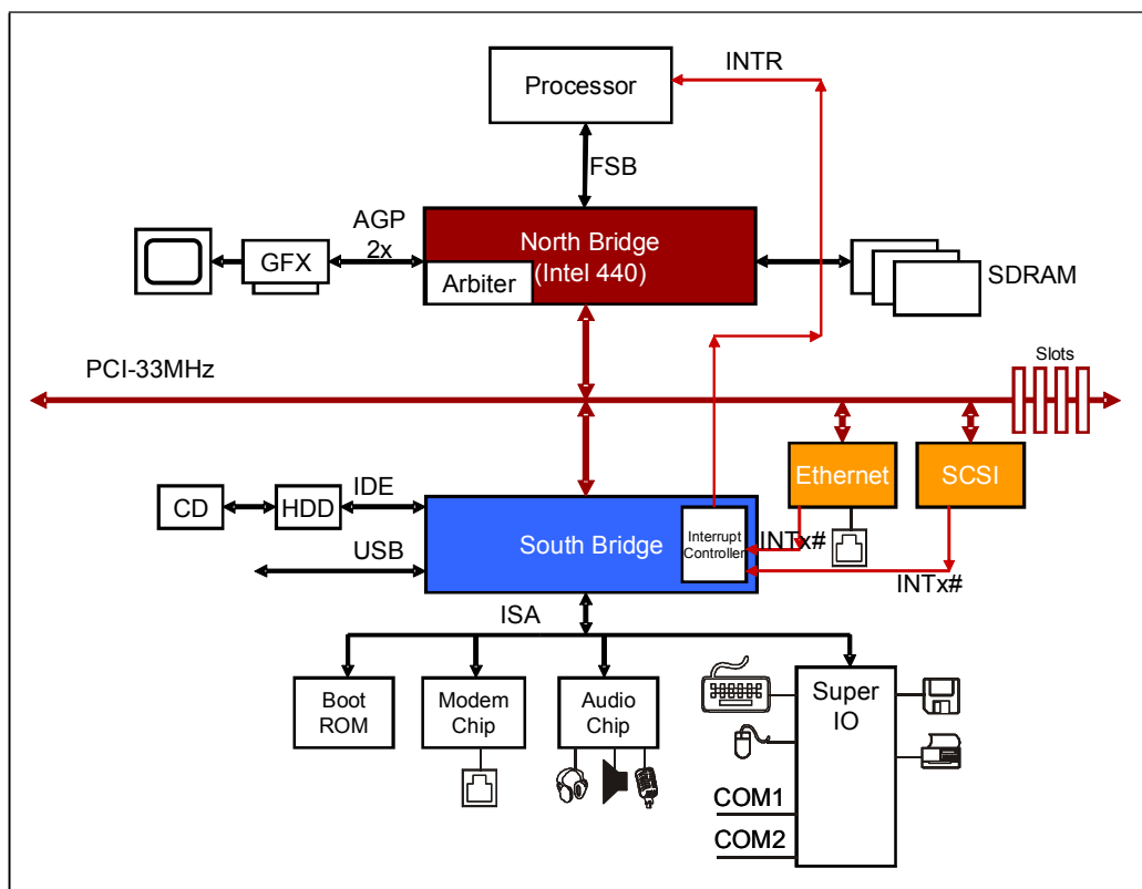
Figure 1-9: PCI Interrupt Handling
