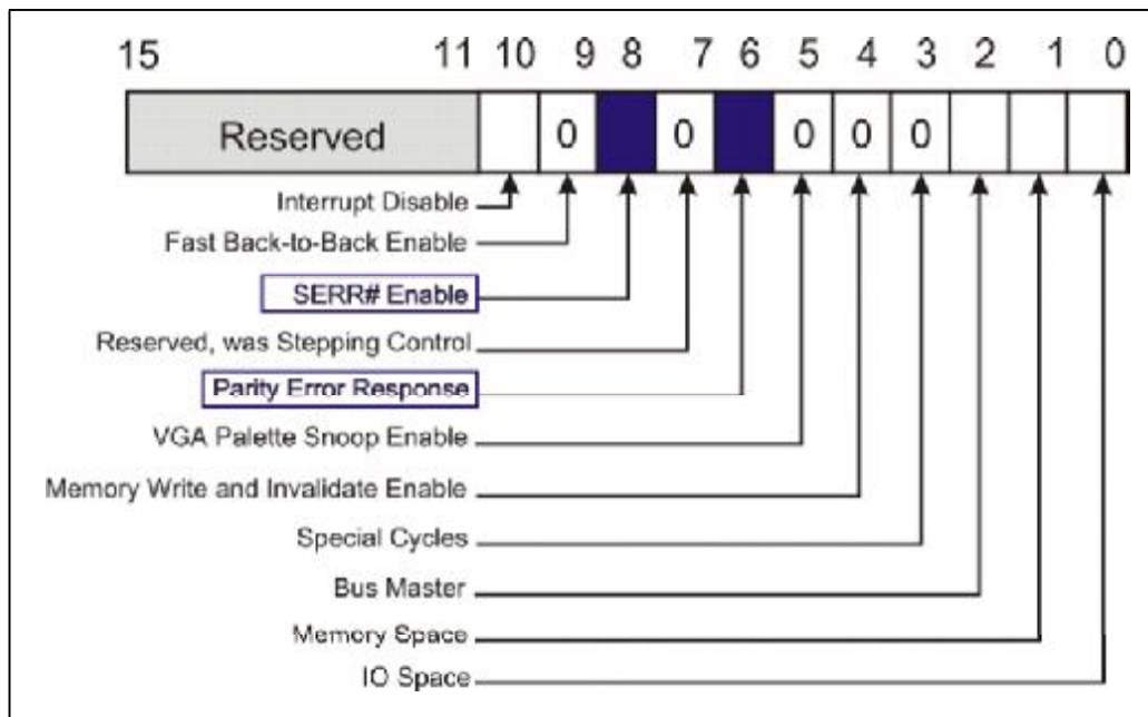
Figure 10-6: PCI-Compatible Configuration Command Register
