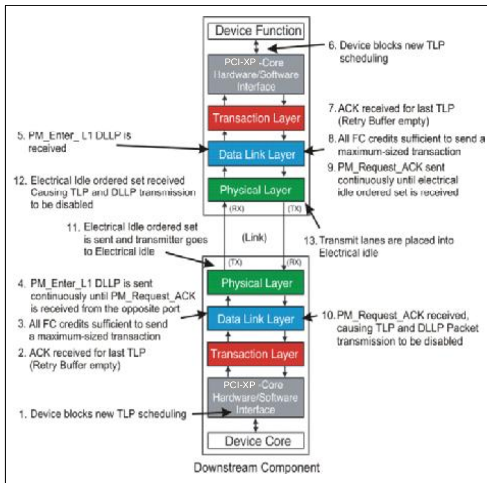
Figure 16-23: Procedure Used to Transition a Link from the L0 to L1 State
