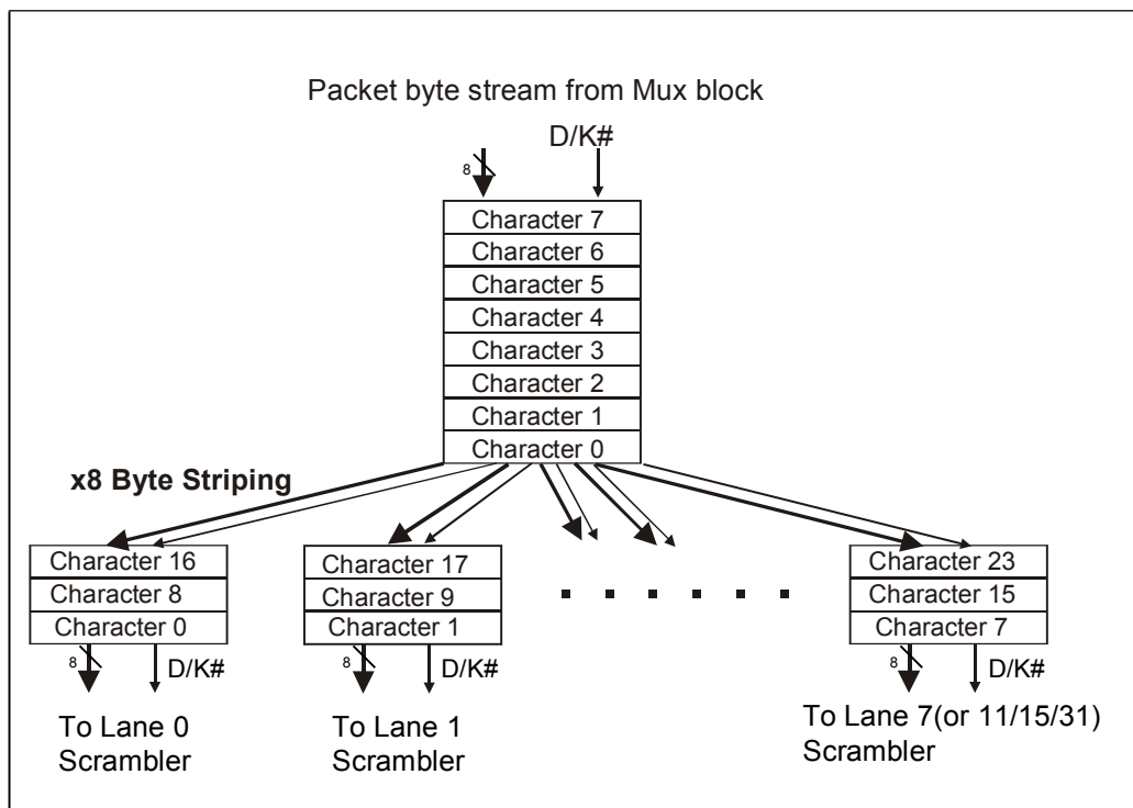
Figure 11-9: x8, x12, x16, x32 Byte Striping
