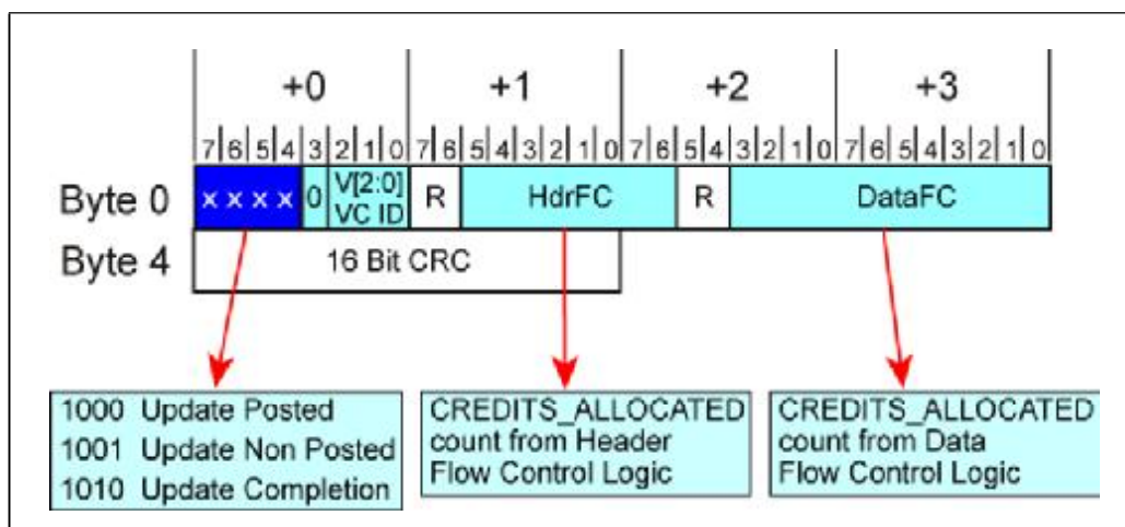
Figure 7-14: Update Flow Control Packet Format and Contents
