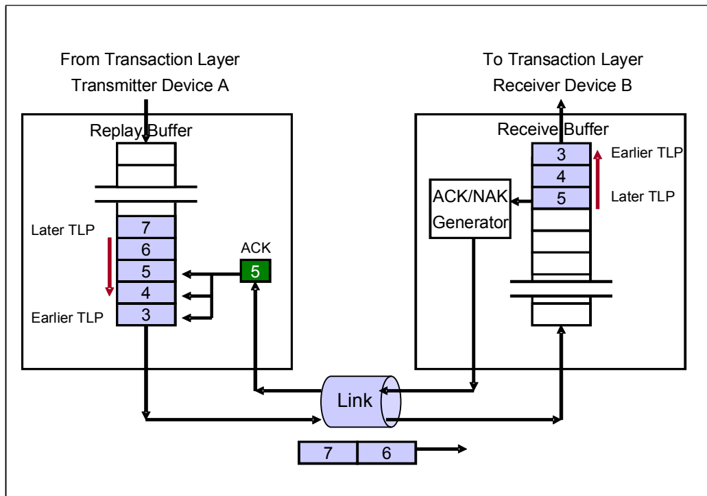
Figure 5-7: Example 1 that Shows Transmitter Behavior with Receipt of an ACK DLLP
