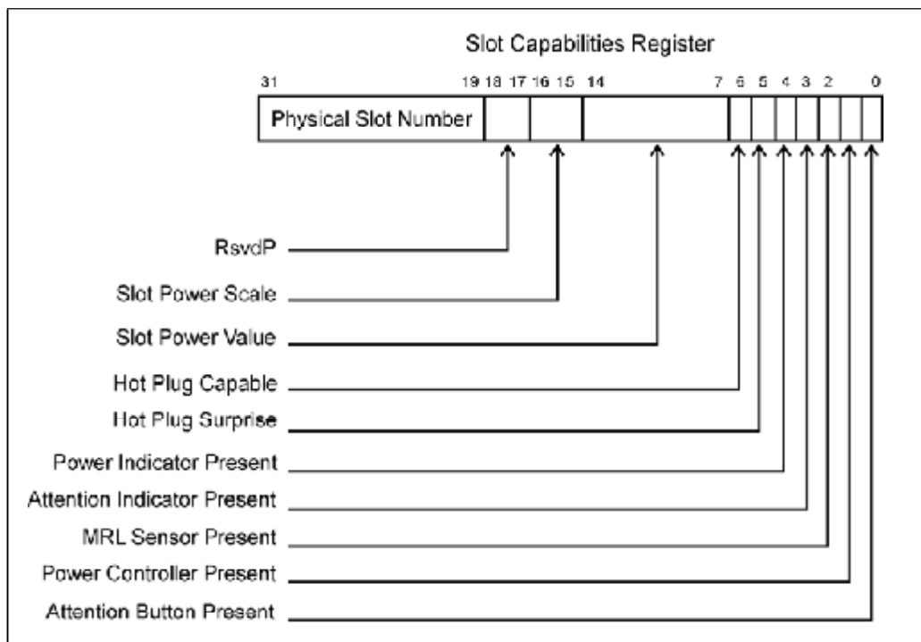
Figure 17-5: Attention Button and Hot Plug Indicators Present Bits
