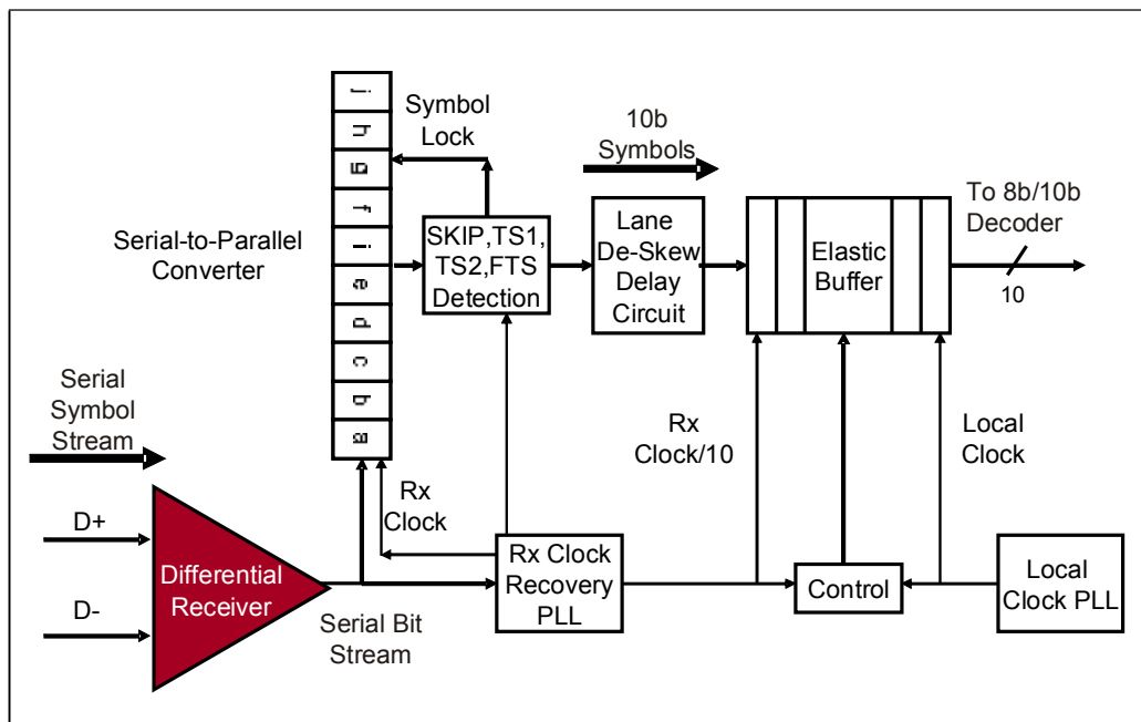
Figure 11-21: Receiver Logic's Front End Per Lane
