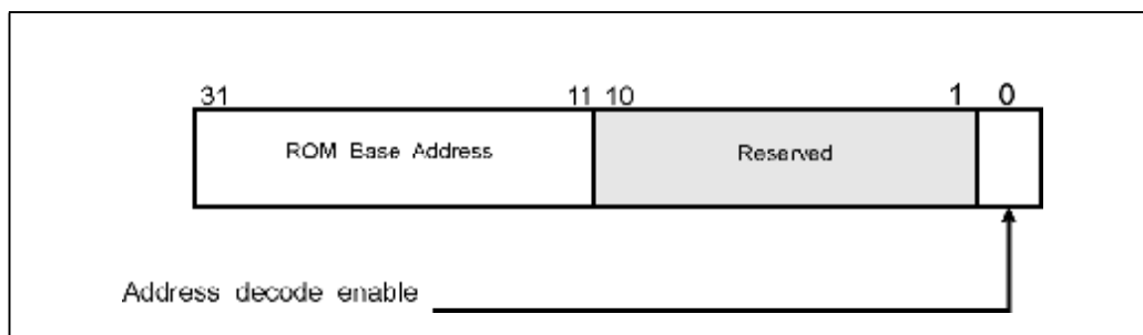
Figure 23-1: Expansion ROM Base Address Register Bit Assignment
