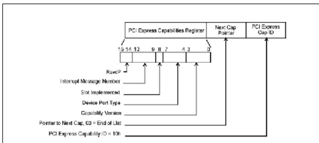
Figure 22-31: PCI Express Capabilities Register
