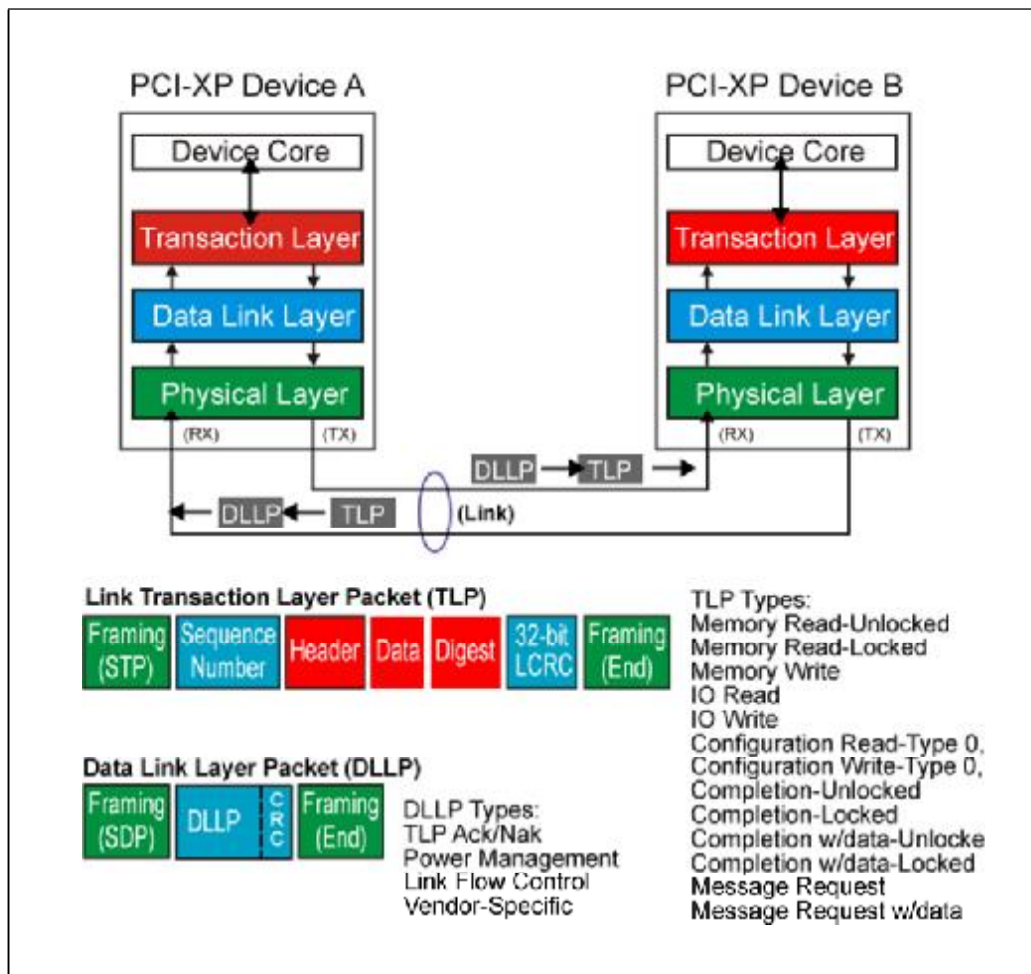
Figure 4-1: TLP And DLLP Packets
