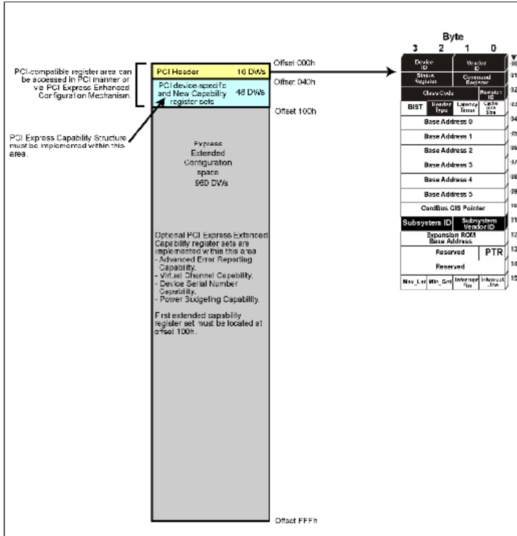
Figure 24-1: Function's Configuration Space Layout
