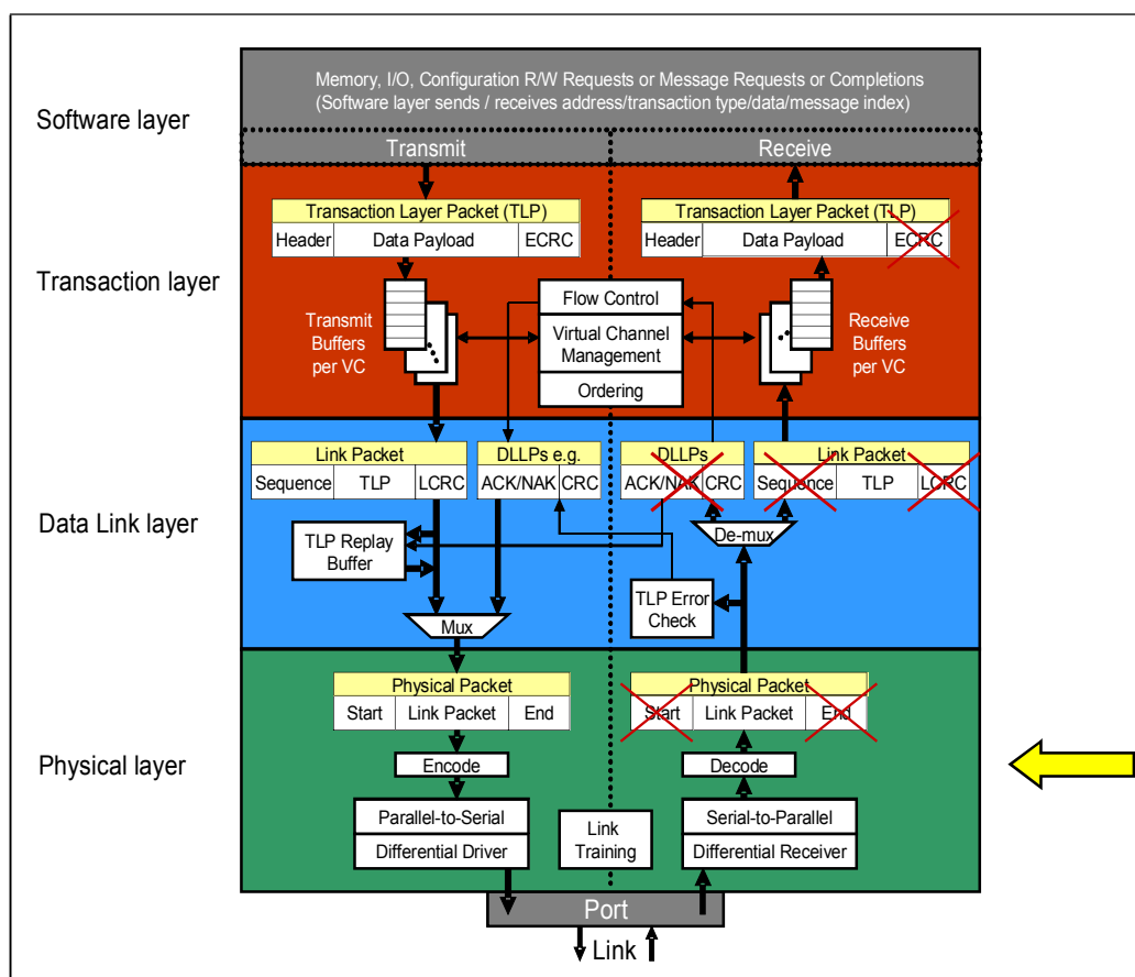
Figure 11-1: Physical Layer
