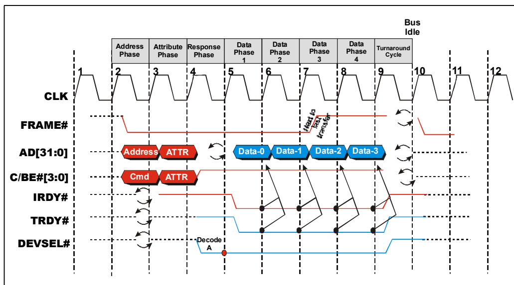
Figure 1-17: Example PCI-X Burst Memory Read Bus Cycle
