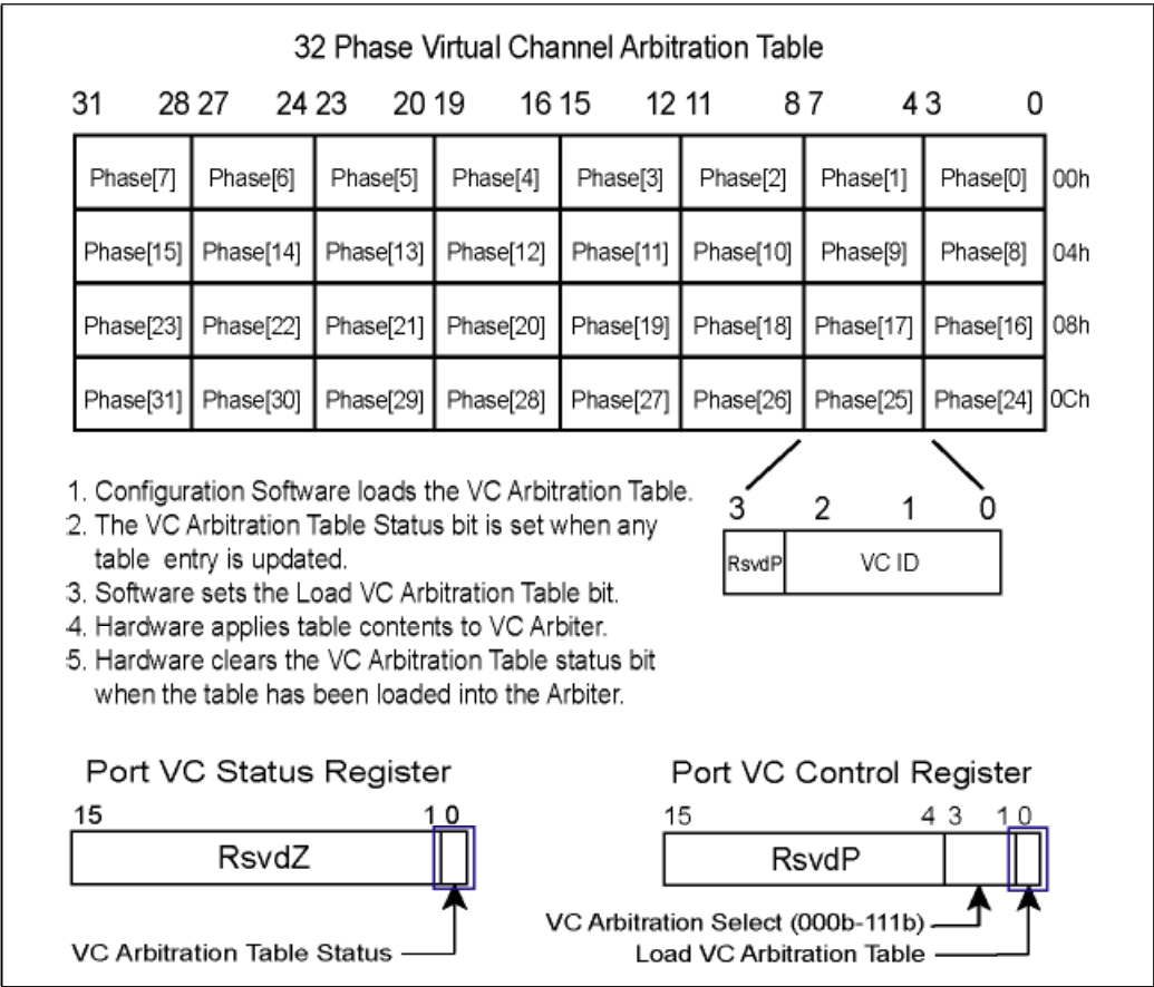
Figure 6-14: Loading the VC Arbitration Table Entries
