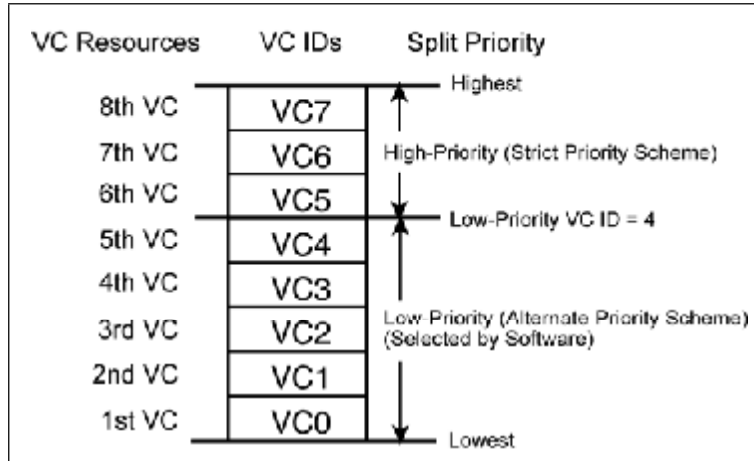
Figure 6-11: VC Arbitration with Low- and High-Priority Implementations
