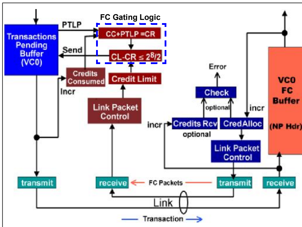
Figure 7-3: Flow Control Elements
