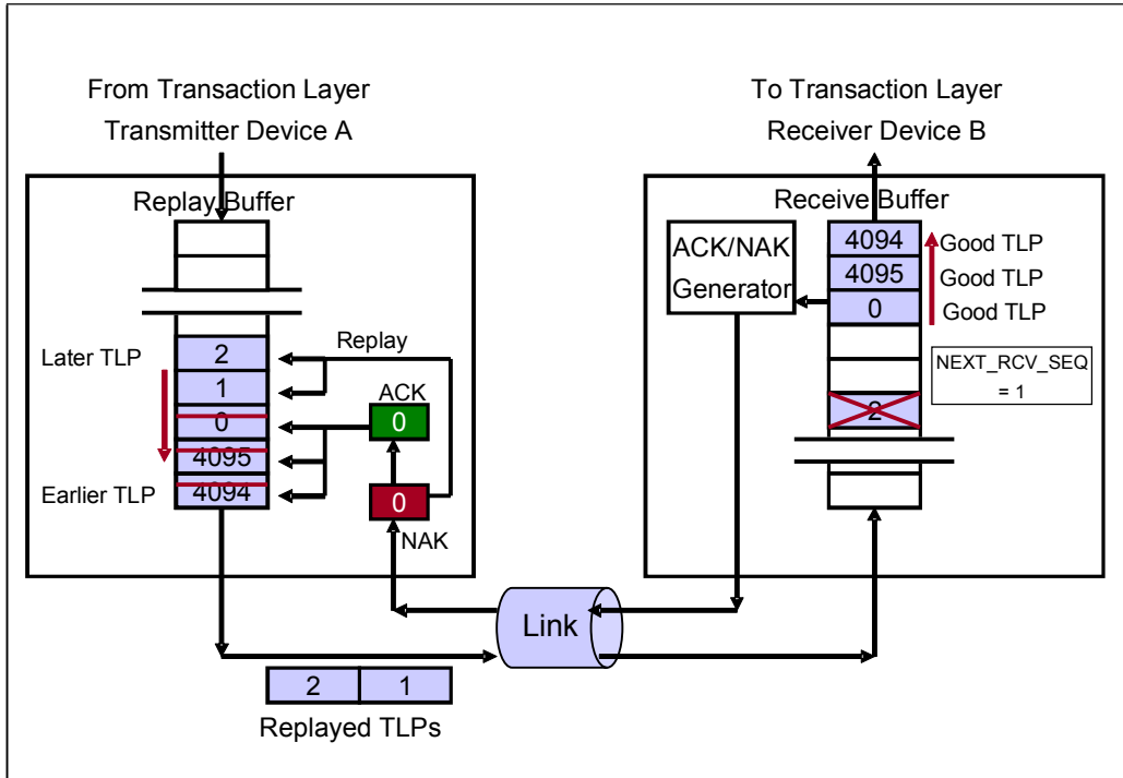
Figure 5-14: Lost TLP Handling
