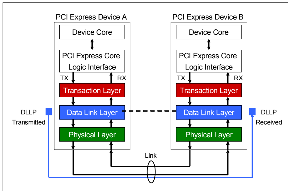
Figure 2-14: DLLP Origin and Destination
