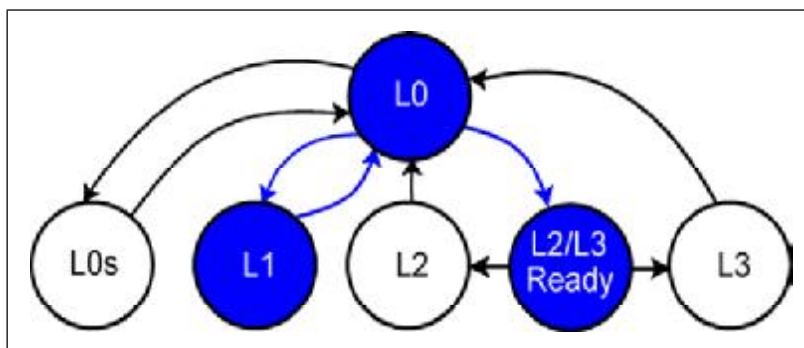
Figure 16-24: Link States Transitions Associated with Preparing Devices for Removal of the Reference Clock and Power
