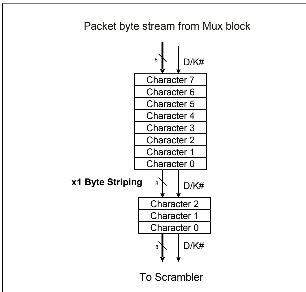
Figure 11-7: x1 Byte Striping
