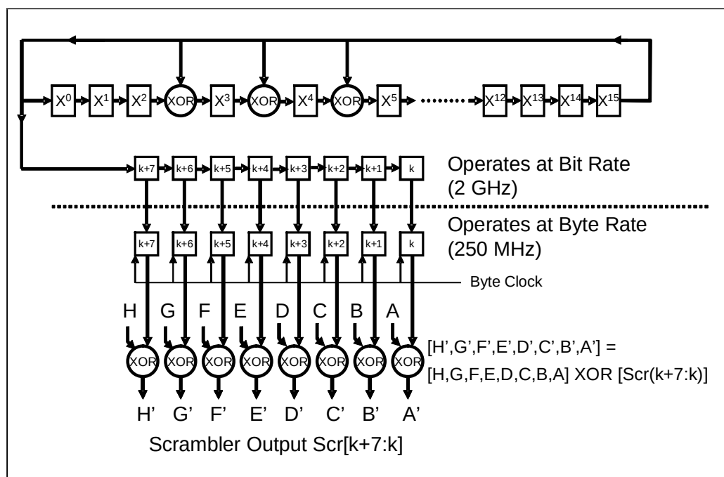
Figure 11-13: Scrambler
