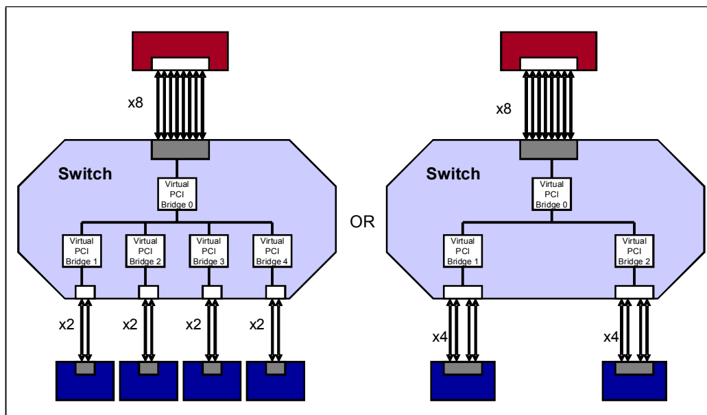
Figure 14-9: Combining Lanes to form Links
