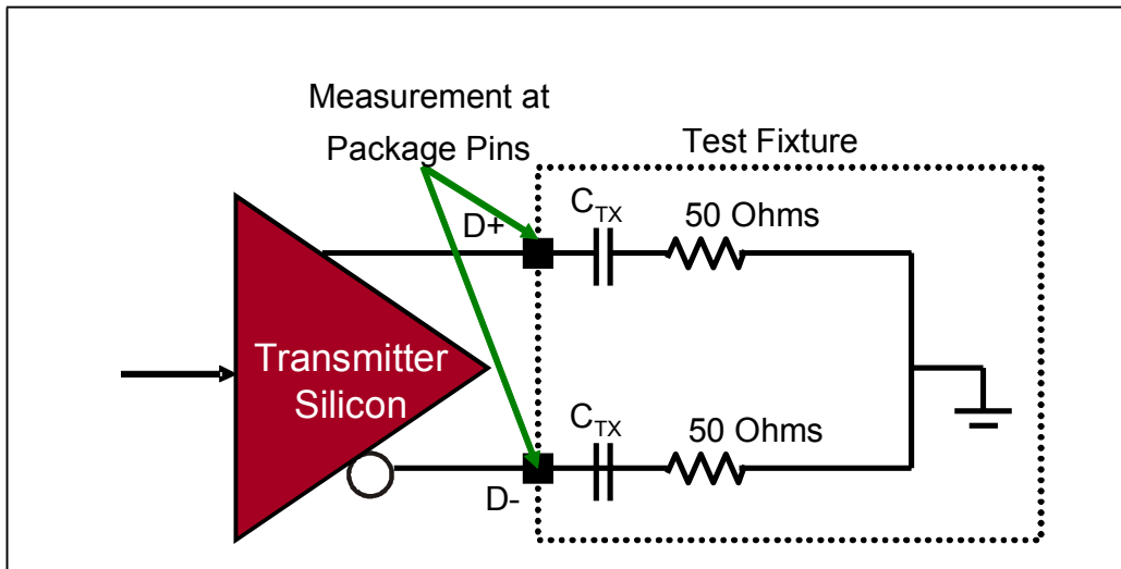
Figure 12-15: Compliance Test/Measurement Load
