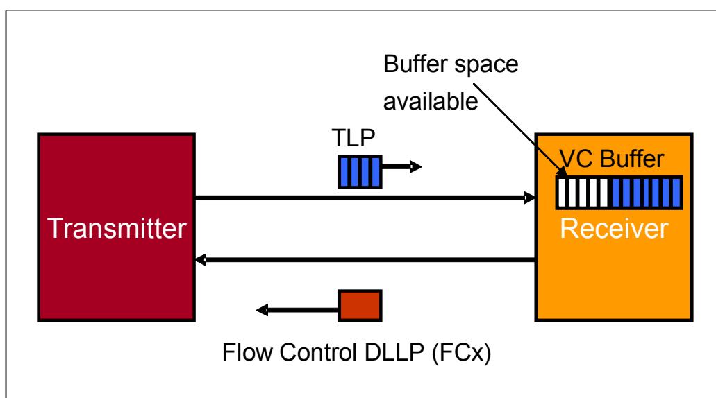
Figure 2-21: Flow Control Process
