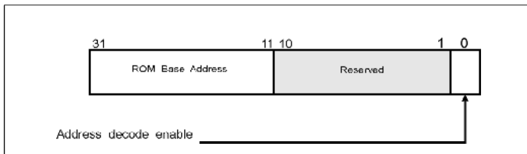
Figure 22-7: Expansion ROM Base Address Register Bit Assignment
