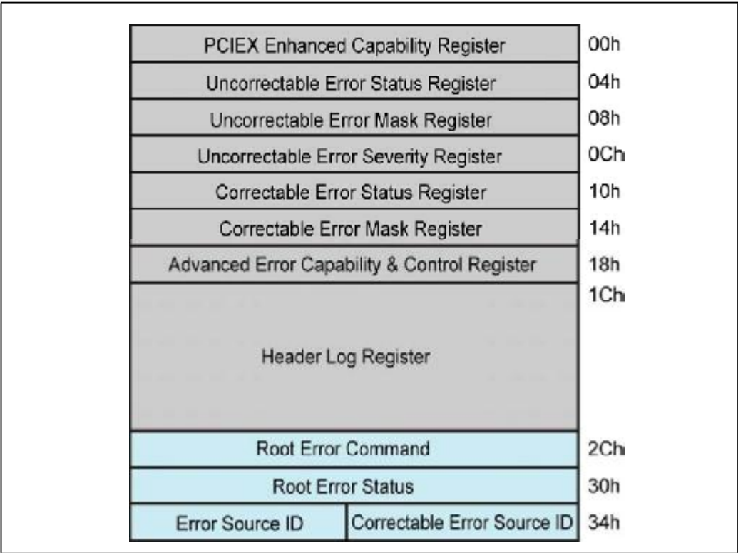
Figure 10-14: Advanced Error Capability Registers
