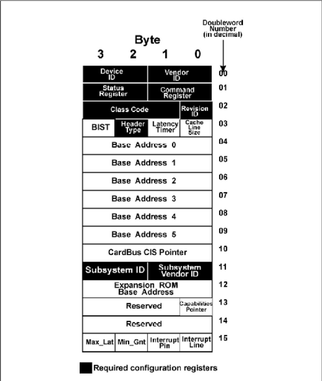
Figure 23-2: Header Type Zero Configuration Register Format
