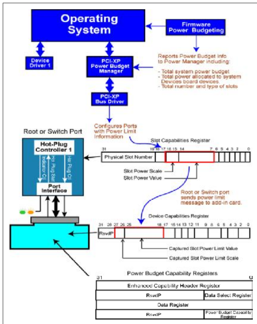
Figure 15-2: Elements Involved in Power Budget
