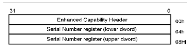
Figure 24-38: Device Serial Number Register
