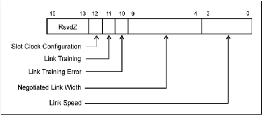
Figure 14-22: Link Status Register
