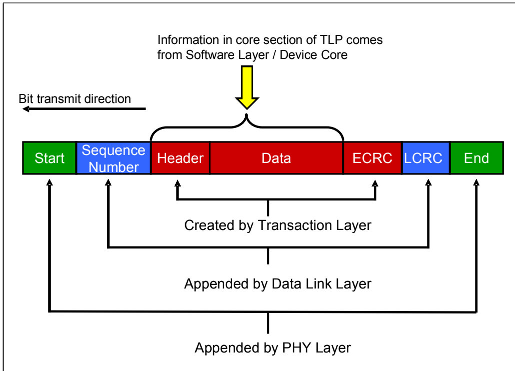
Figure 2-12: TLP Assembly
