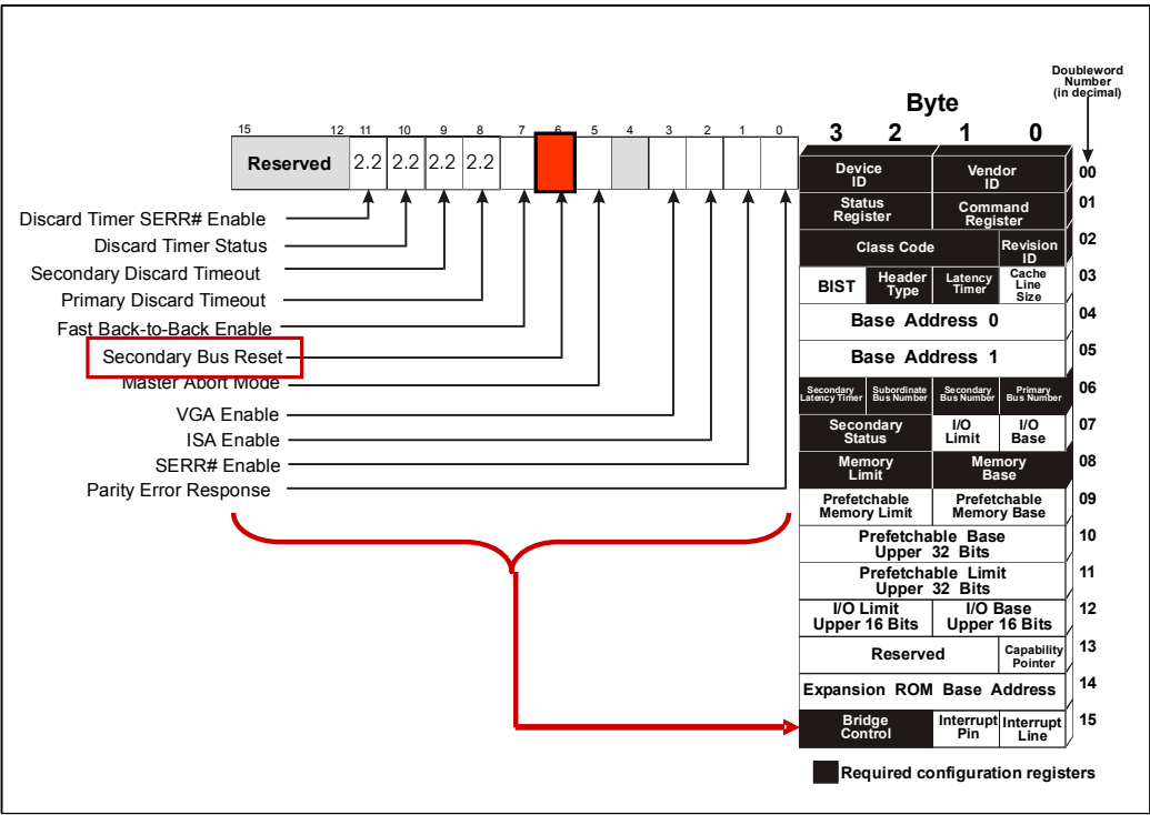
Figure 13-3: Secondary Bus Reset Register to Generate Hot Reset
