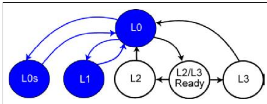
Figure 16-11: ASPM Link State Transitions
