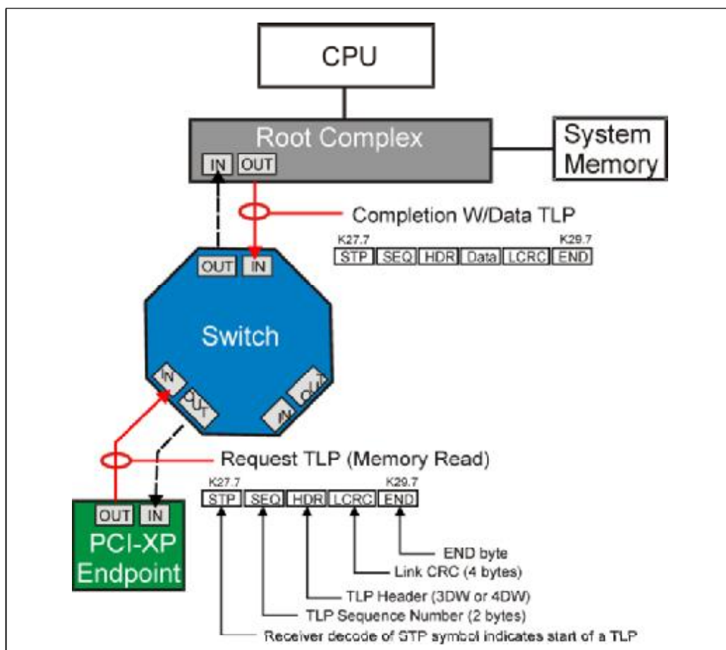
Figure 3-4: PCI Express Transaction Request And Completion TLPs
