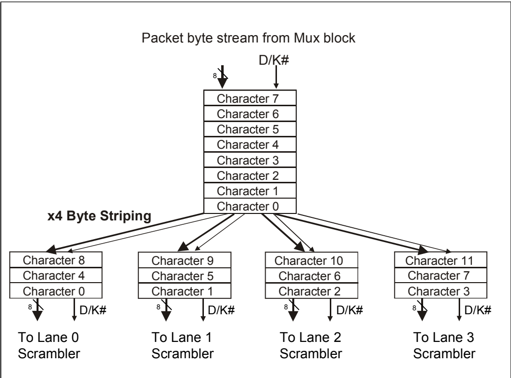
Figure 11-8: x4 Byte Striping
