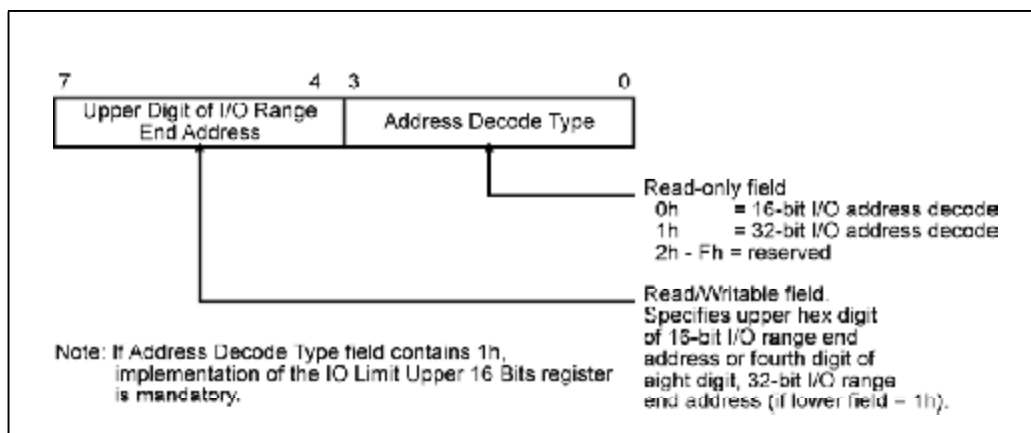
Figure 22-15: IO Limit Register
