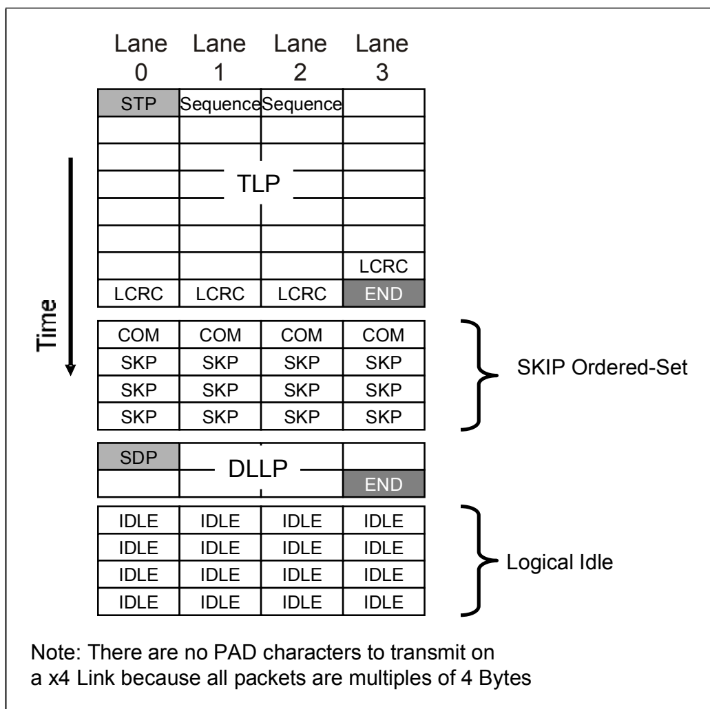
Figure 11-11: x4 Packet Format
