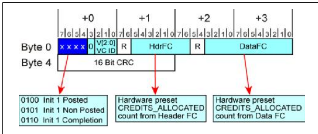
Figure 7-10: INIT1 Flow Control Packet Format and Contents
