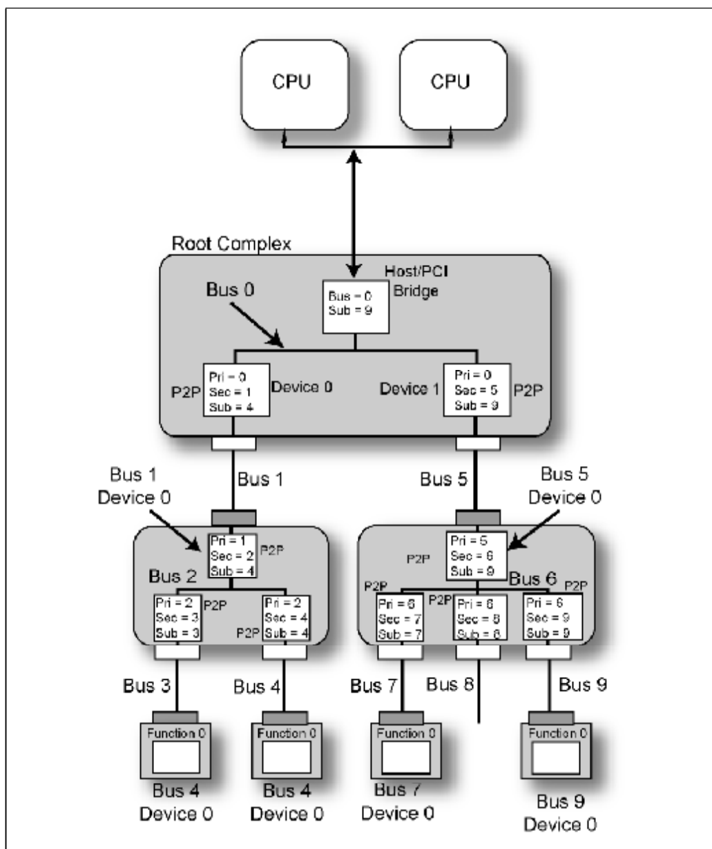
Figure 20-3: Example System
