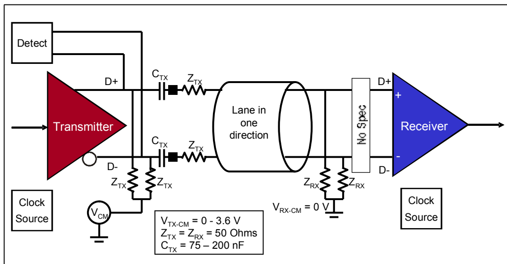
Figure 12-2: Differential Transmitter/Receiver
