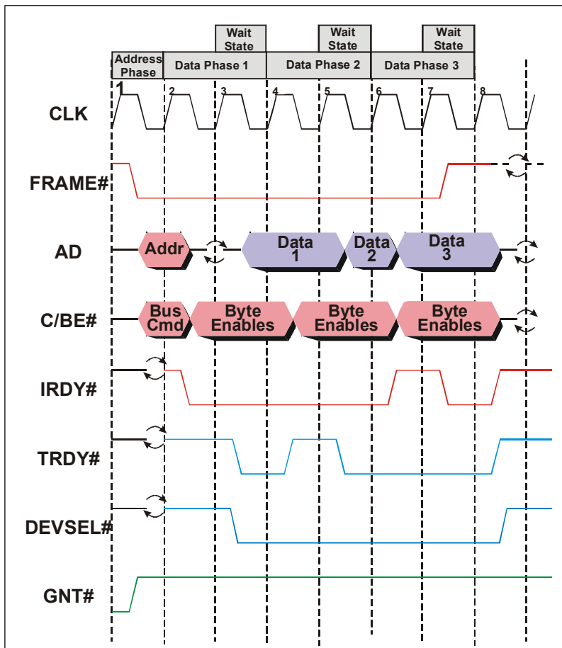
Figure 1-3: Typical PCI Burst Memory Read Bus Cycle
