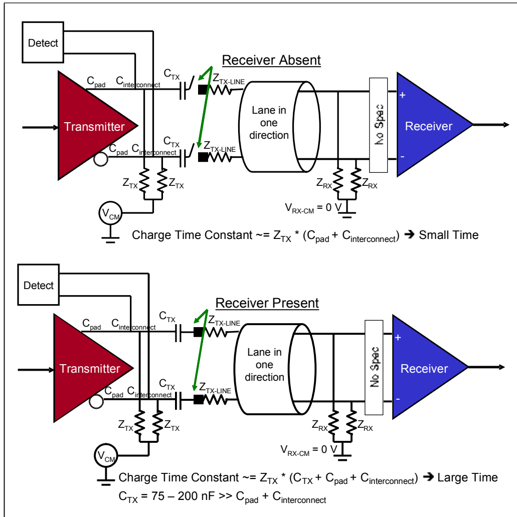
Figure 12-4: Receiver Detection Mechanism
