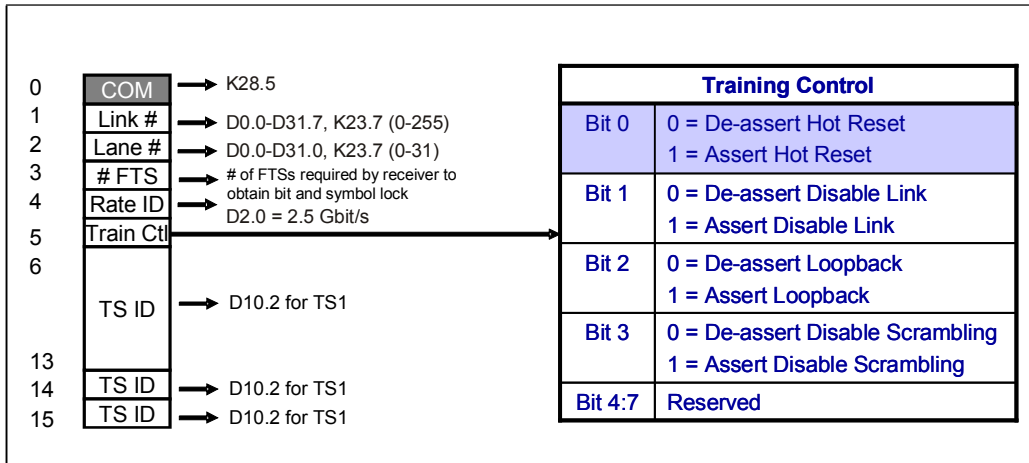
Figure 13-2: TS1 Ordered-Set Showing the Hot Reset Bit
