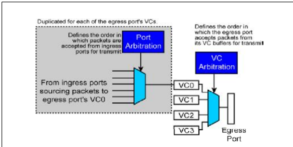
Figure 24-27: Port and VC Arbitration
