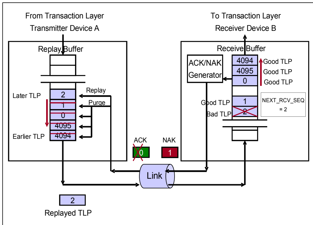
Figure 5-16: Lost ACK DLLP Handling
