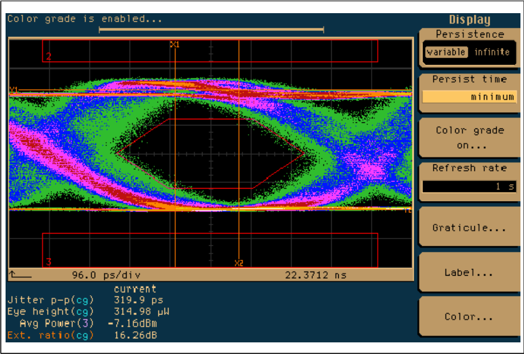
Figure 12-14: Screen Capture of a Bad Eye Showing Effect of Jitter, Noise and Signal Attenuation (With no De-emphasis Shown)
