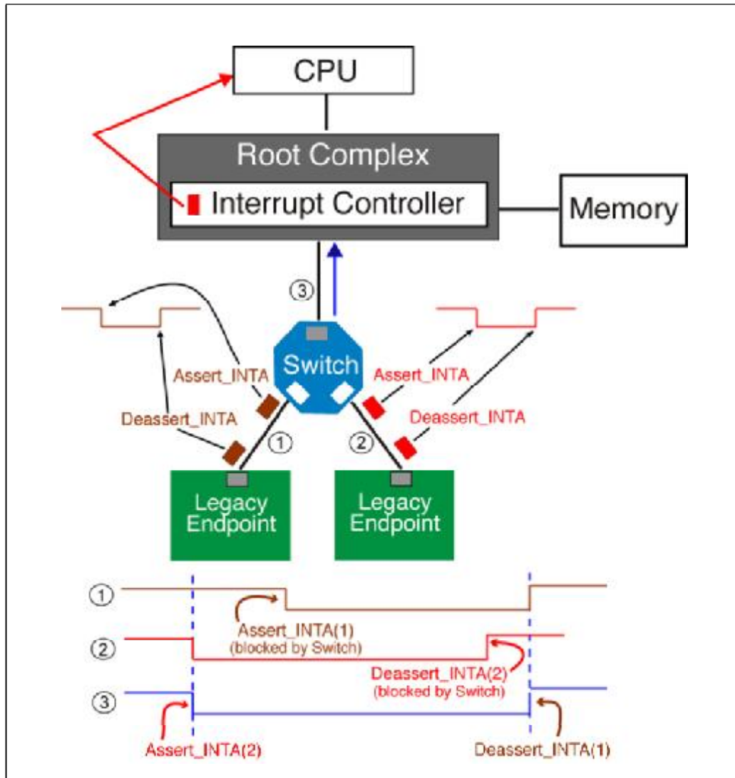
Figure 9-12: Switch Collapses INTx Message to Achieve Wired-OR Characteristics
