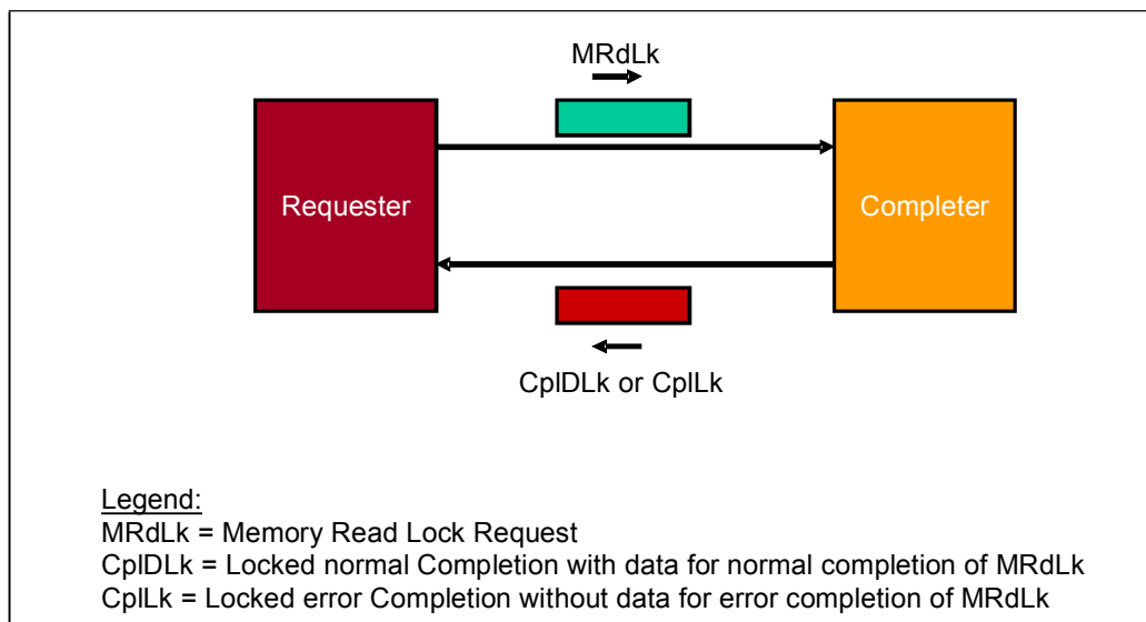
Figure 2-2: Non-Posted Locked Read Transaction Protocol
