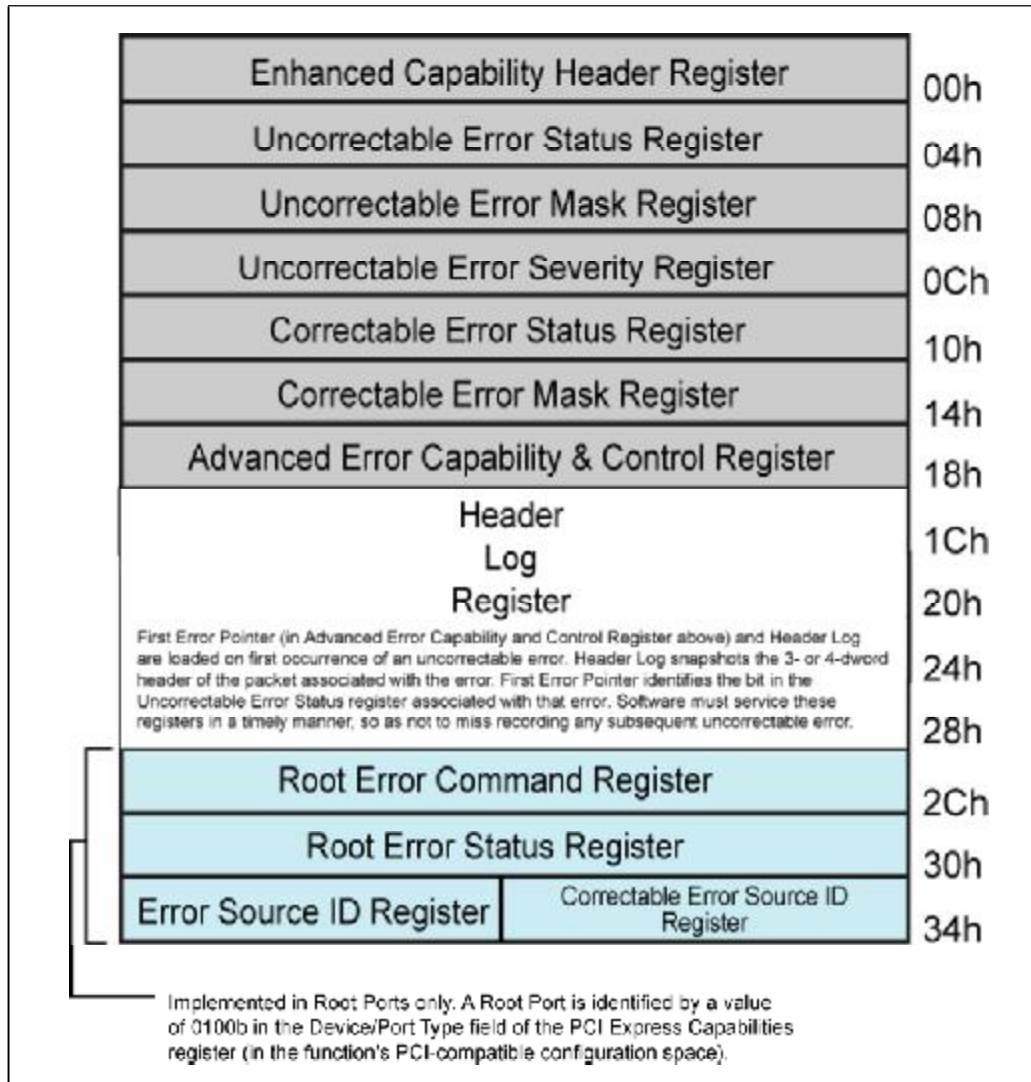
Figure 24-16: Advanced Error Reporting Capability Register Set
