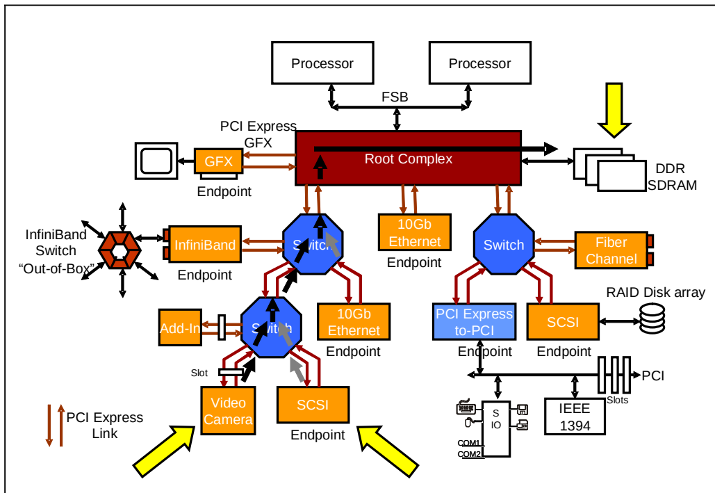
Figure 2-22: Example Showing QoS Capability of PCI Express
