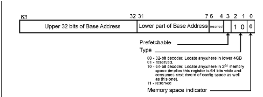
Figure 22-11: 64-Bit Memory Base Address Register Bit Assignment
