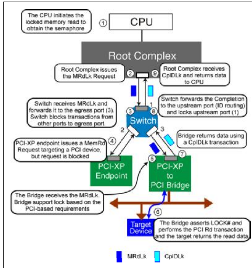
Figure E-1: Lock Sequence Begins with Memory Read Lock Request
