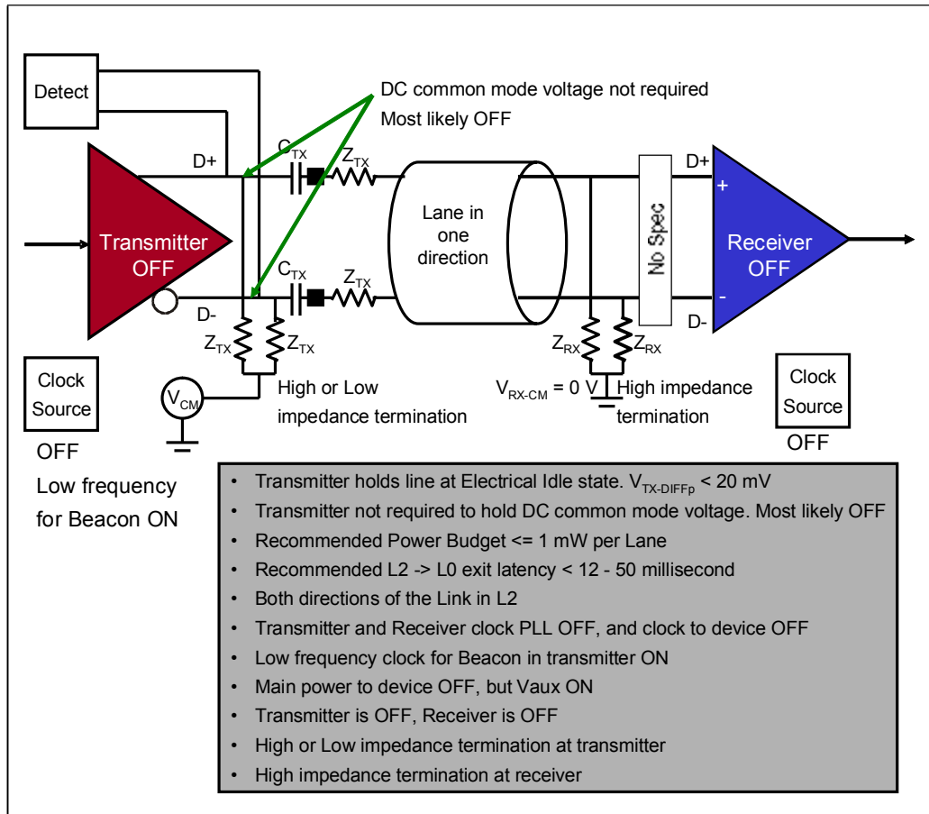
Figure 12-20: L2 Low Power Link State
