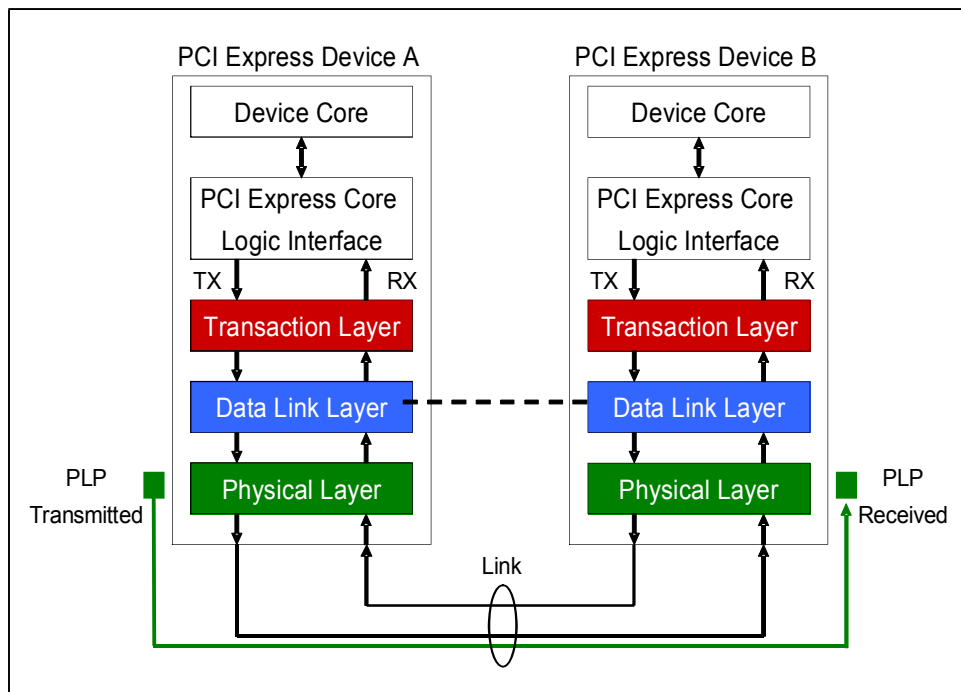
Figure 2-17: PLP Origin and Destination
