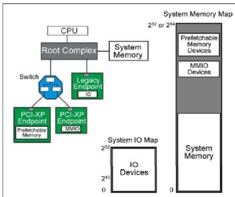
Figure 3-6: Generic System Memory And IO Address Maps
