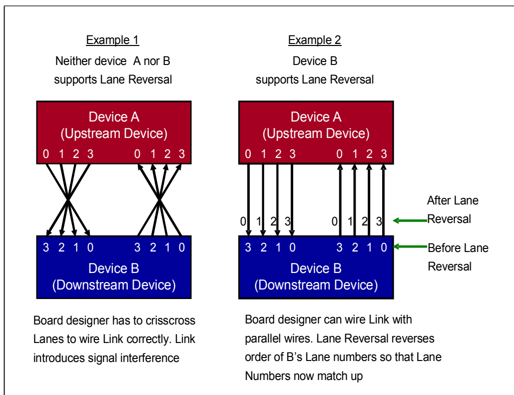
Figure 14-2: Example Showing Lane Reversal
