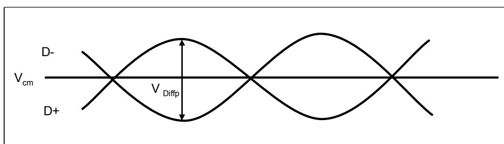
Figure 1-21: PCI Express Differential Signal
