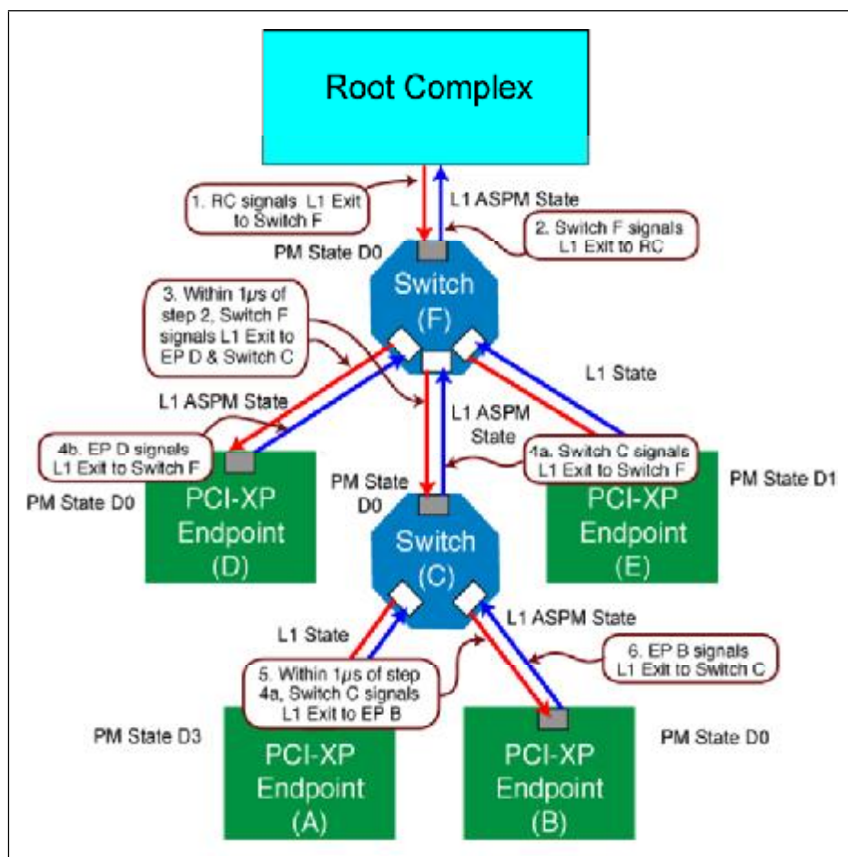
Figure 16-18: Switch Behavior When Upstream Component Signals L1 Exit
