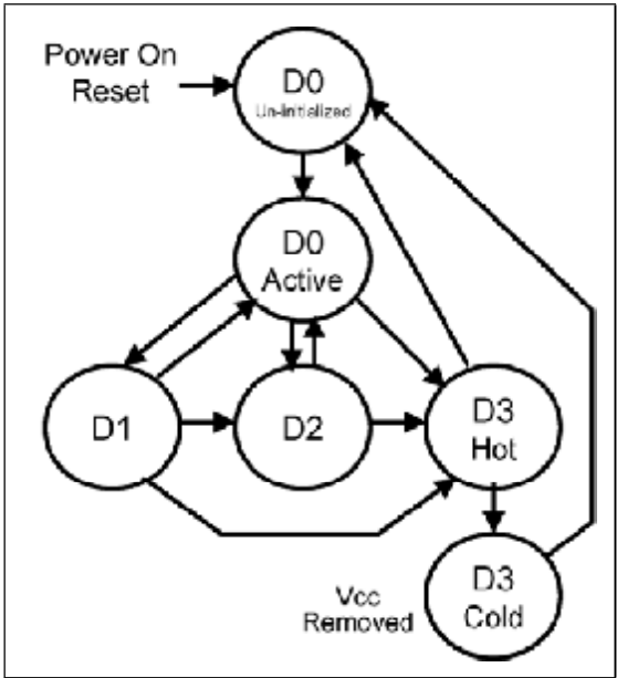
Figure 16-6: PCI Express Function Power Management State Transitions
