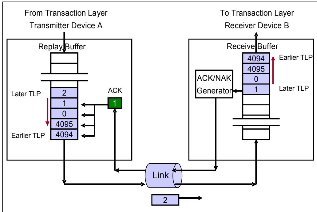
Figure 5-11: Example that Shows Receiver Behavior with Receipt of Good TLP
