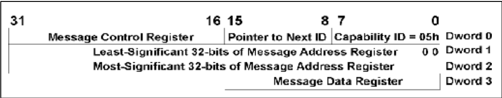
Figure 9-3: 32-bit MSI Capability Register Set Format
