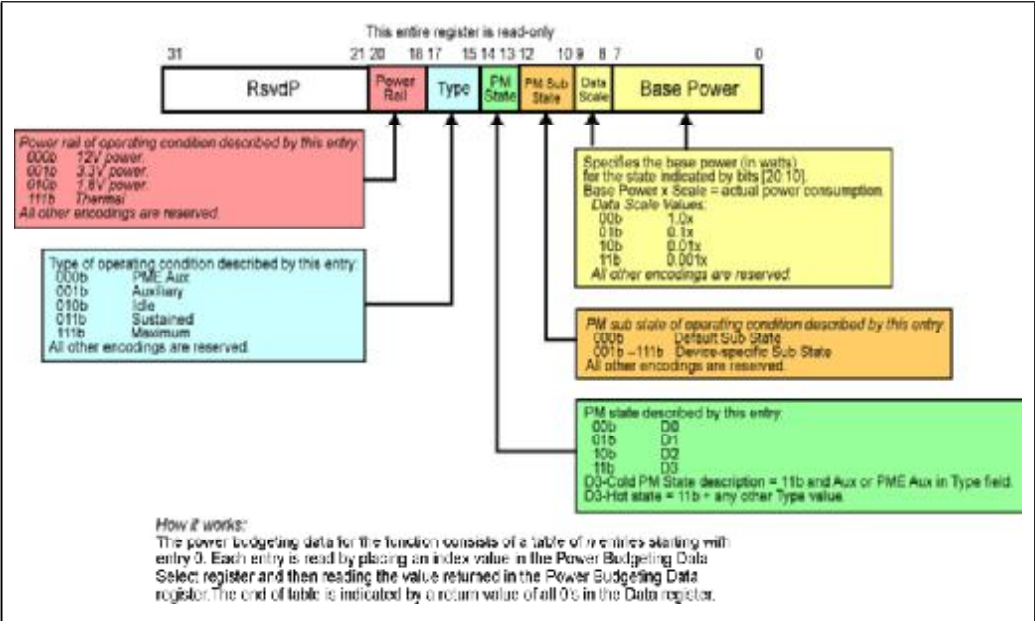
Figure 15-5: Power Budget Data Field Format and Definition
