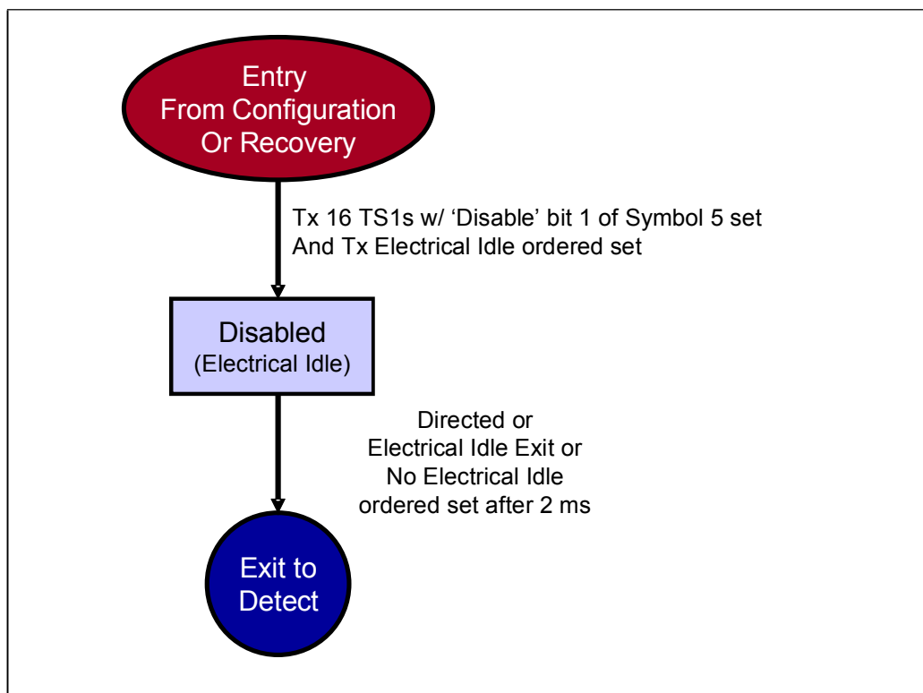
Figure 14-19: Disable State Machine
