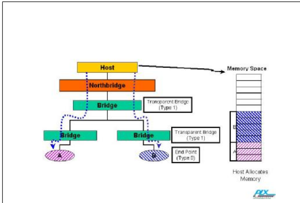
Figure C-1: Enumeration Using Transparent Bridges
