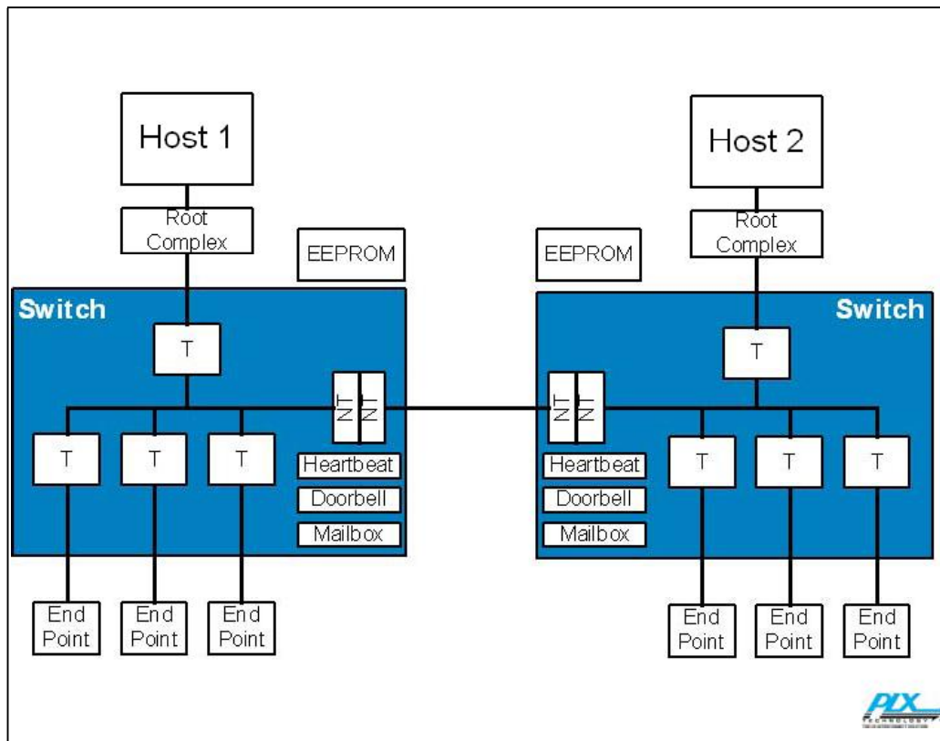
Figure C-6: Dual Host in a PCI and PCI Express System
