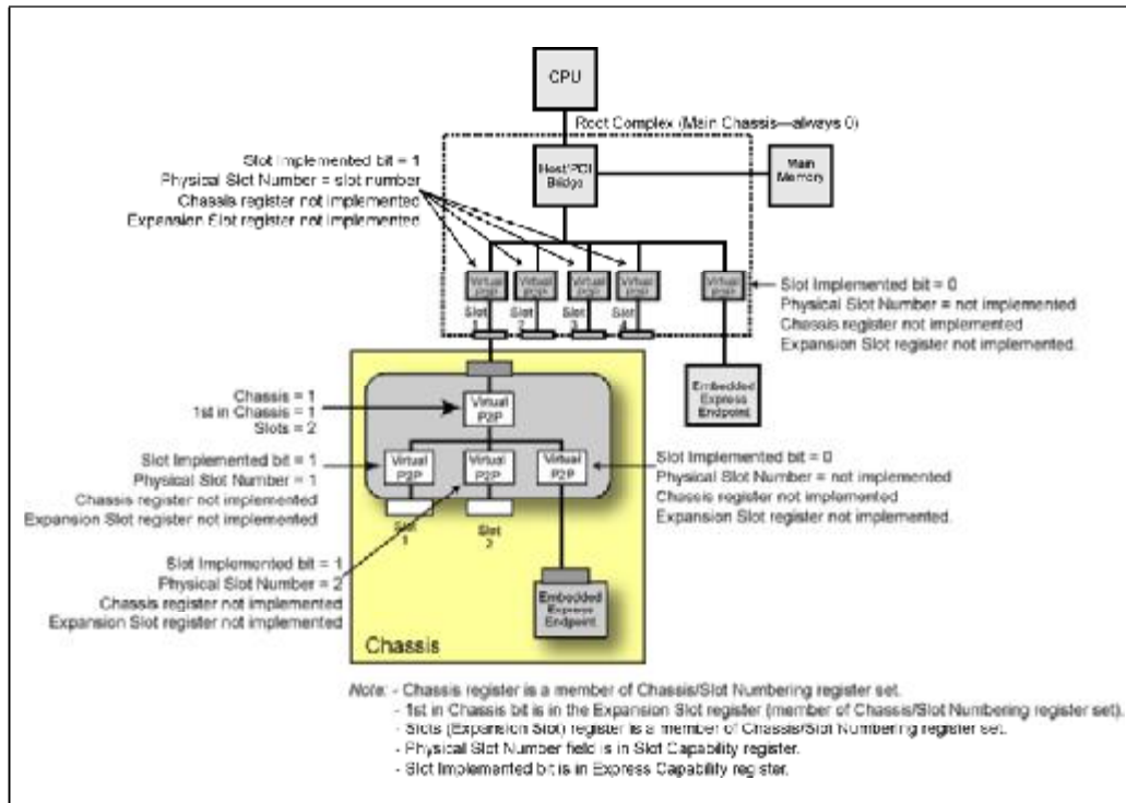
Figure 22-32: Chassis Example One
