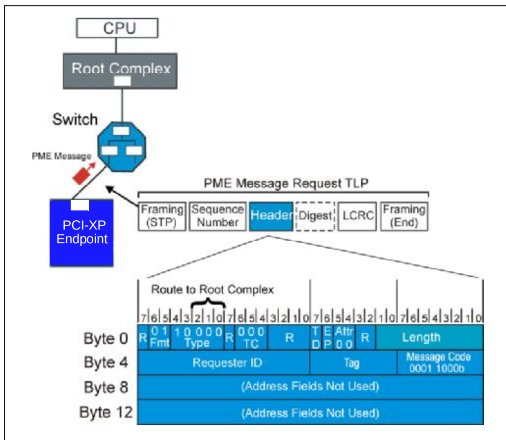
Figure 16-27: PME Message Format
