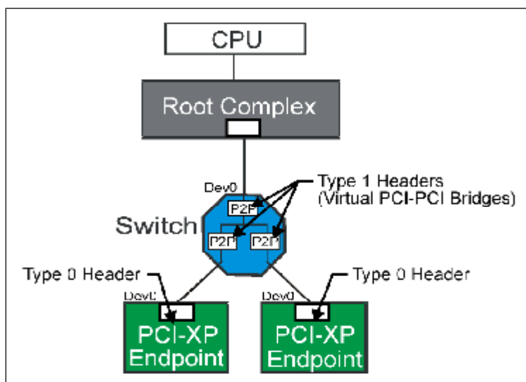
Figure 3-15: PCI Express Devices And Type 0 And Type 1 Header Use
