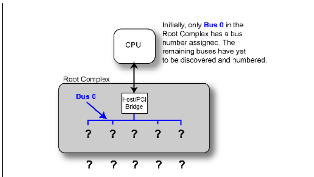
Figure 21-1: Topology View At Startup
