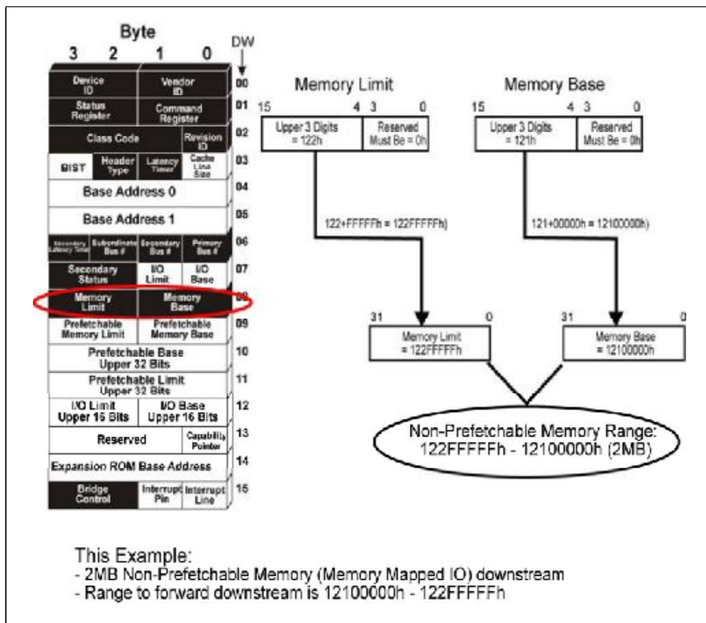
Figure 3-21: 2MB, 32-Bit Non-Prefetchable Base/Limit Register Set Up
