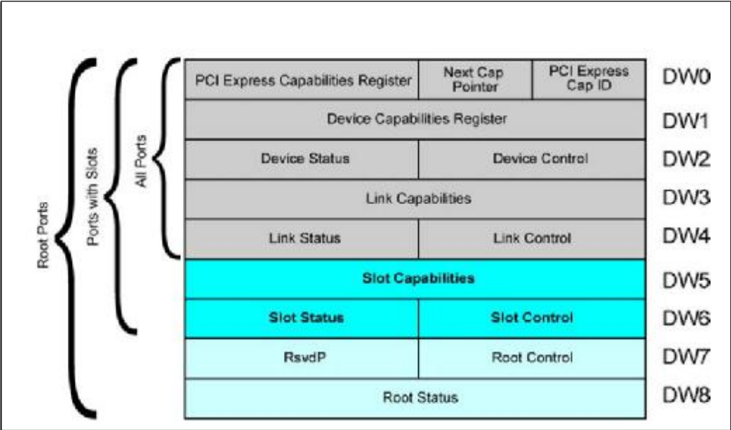
Figure 10-8: PCI Express Capability Register Set
