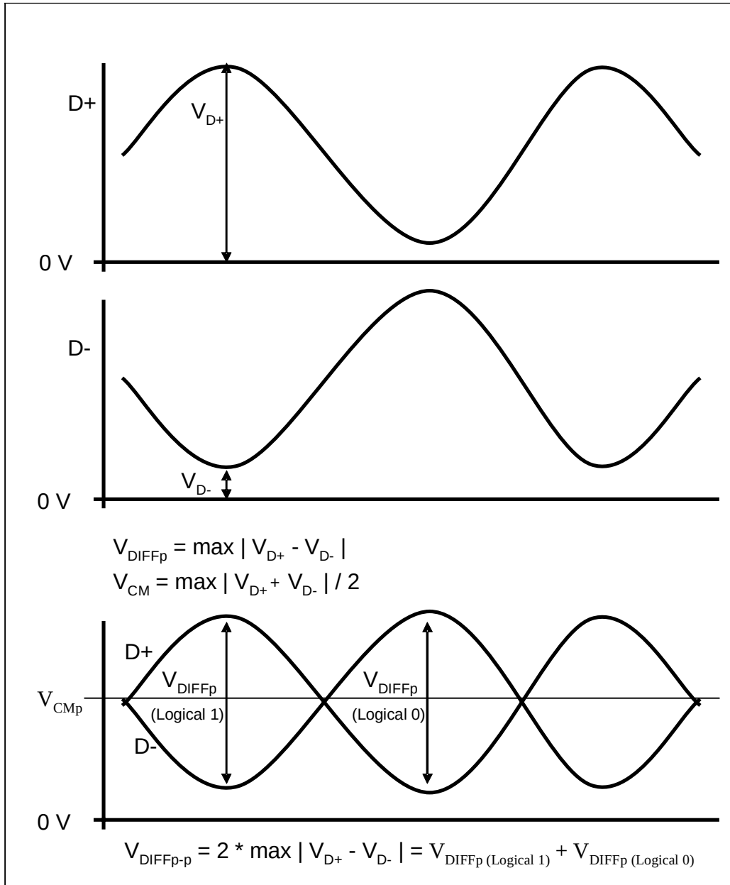
Figure 12-5: Pictorial Representation of Differential Peak-to-Peak and Differential Peak Voltages
