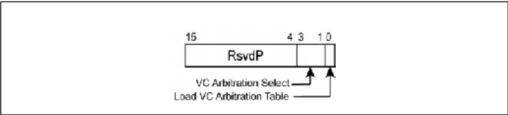
Figure 24-32: Port VC Control Register (Read-Write)
