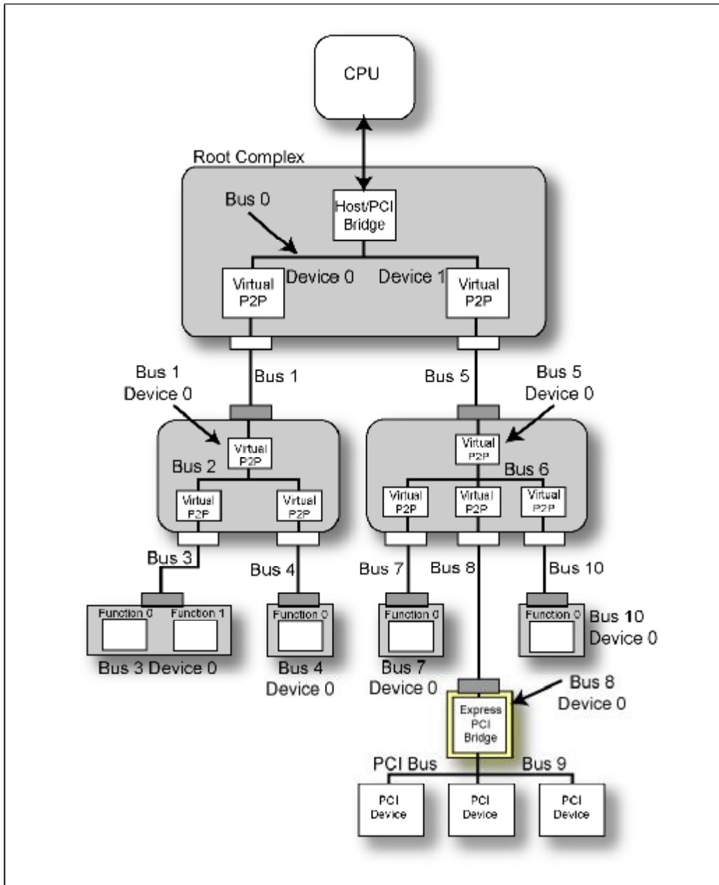
Figure 19-1: Example System
