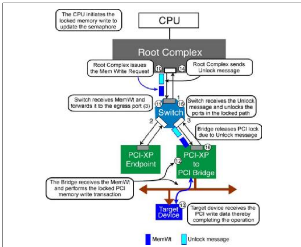
Figure E-2: Lock Completes with Memory Write Followed by Unlock Message
