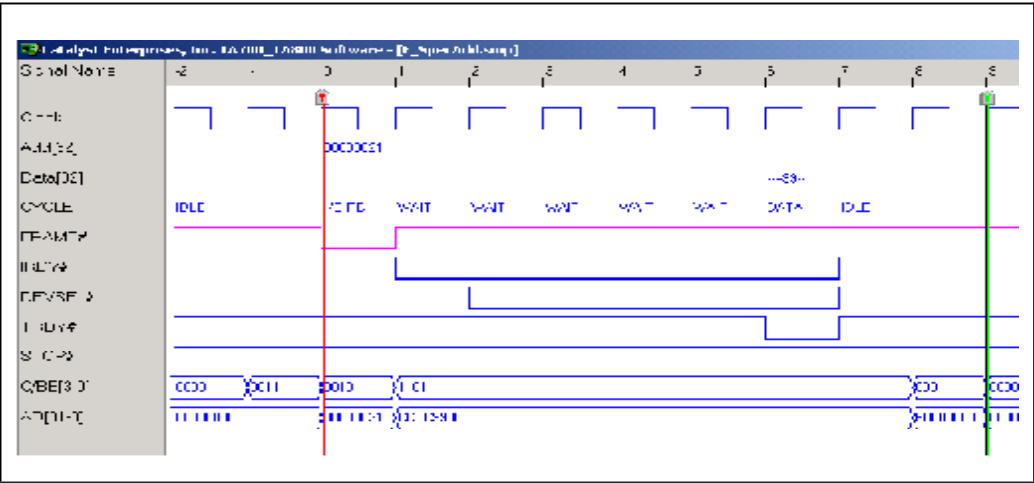
Figure A-1: PCI Parallel Bus Start and End of a Transaction Easily Identified
