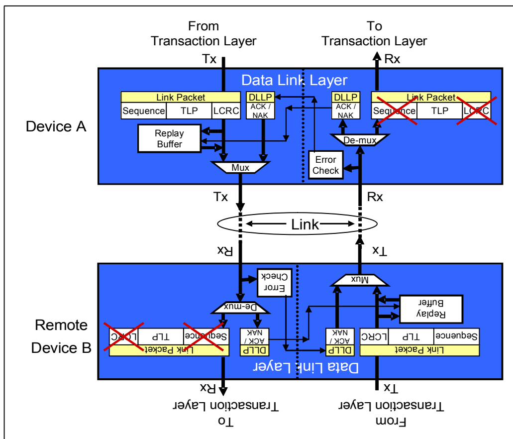
Figure 2-25: Data Link Layer Replay Mechanism
