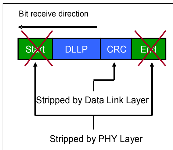
Figure 2-16: DLLP Disassembly
