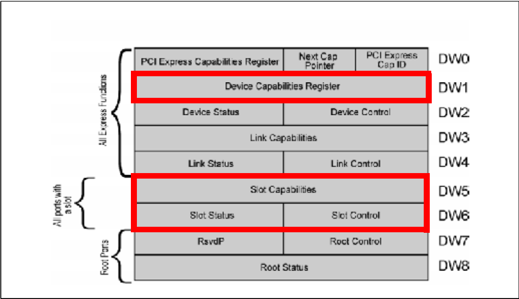
Figure 17-4: PCI Express Configuration Registers Used for Hot-Plug
