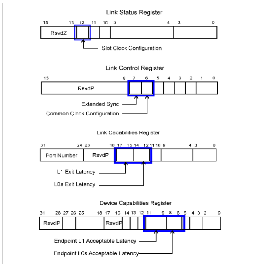
Figure 16-20: Config. Registers Used for ASPM Exit Latency Management and Reporting
