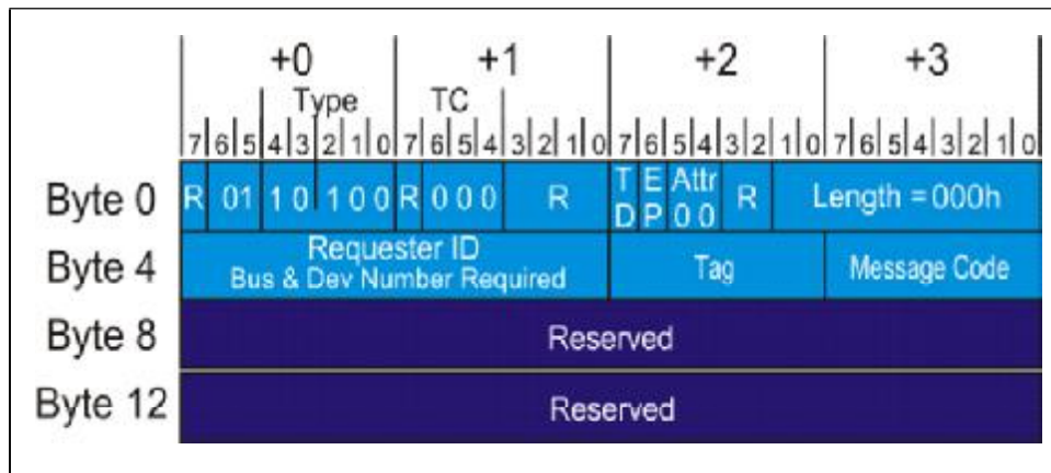
Figure 9-13: INTx Message Format and Types
