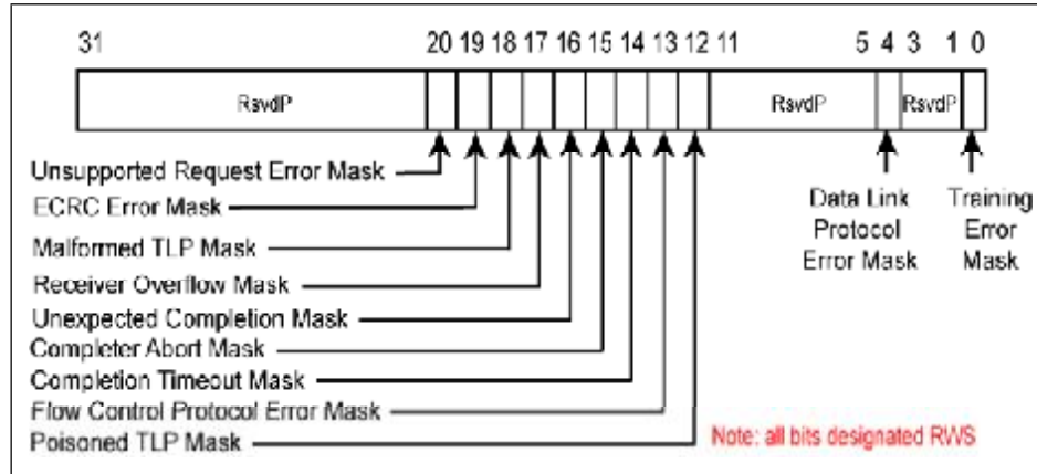
Figure 10-20: Advanced Uncorrectable Error Mask Register
