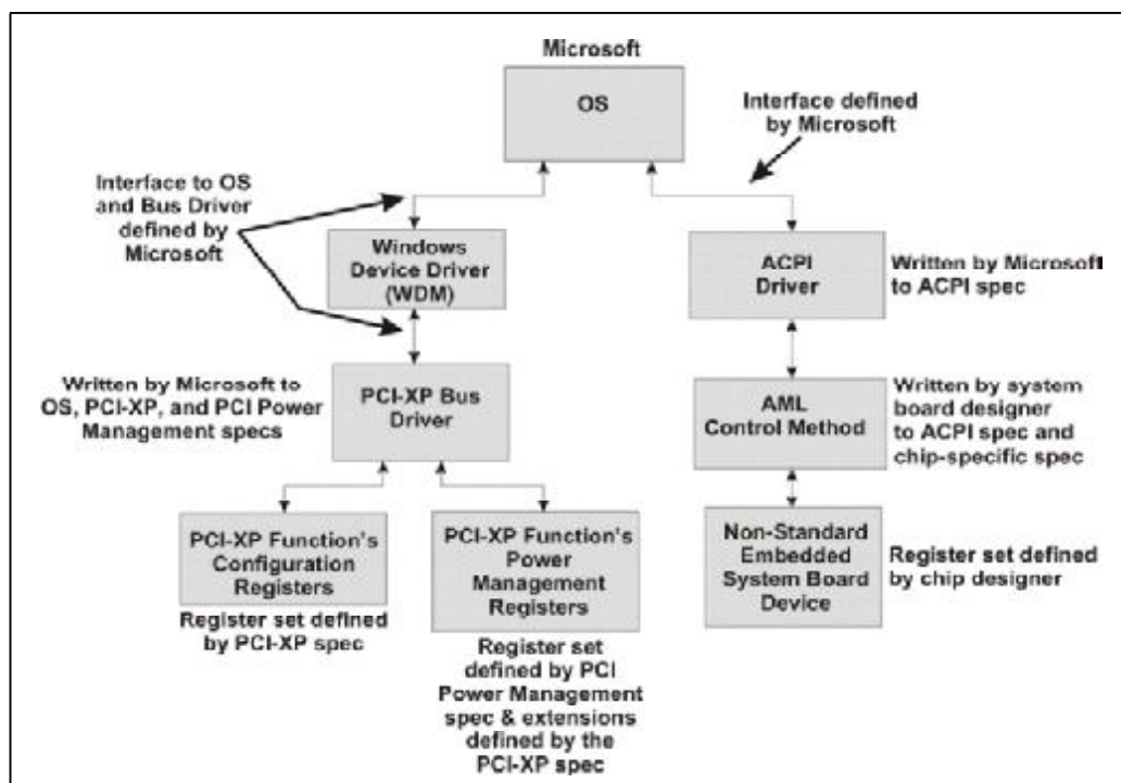
Figure 16-1: Relationship of OS, Device Drivers, Bus Driver, PCI Express Registers, and ACPI
