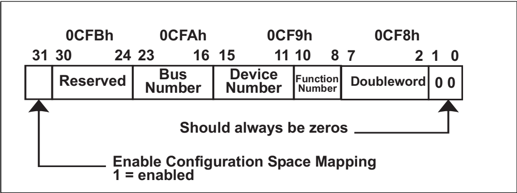
Figure 20-2: Configuration Address Port at 0CF8h
