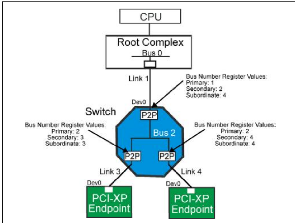
Figure 3-23: Bus Number Registers In A Switch
