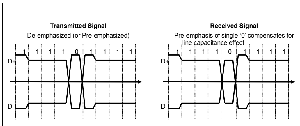
Figure 12-9: Solution is Pre-emphasis
