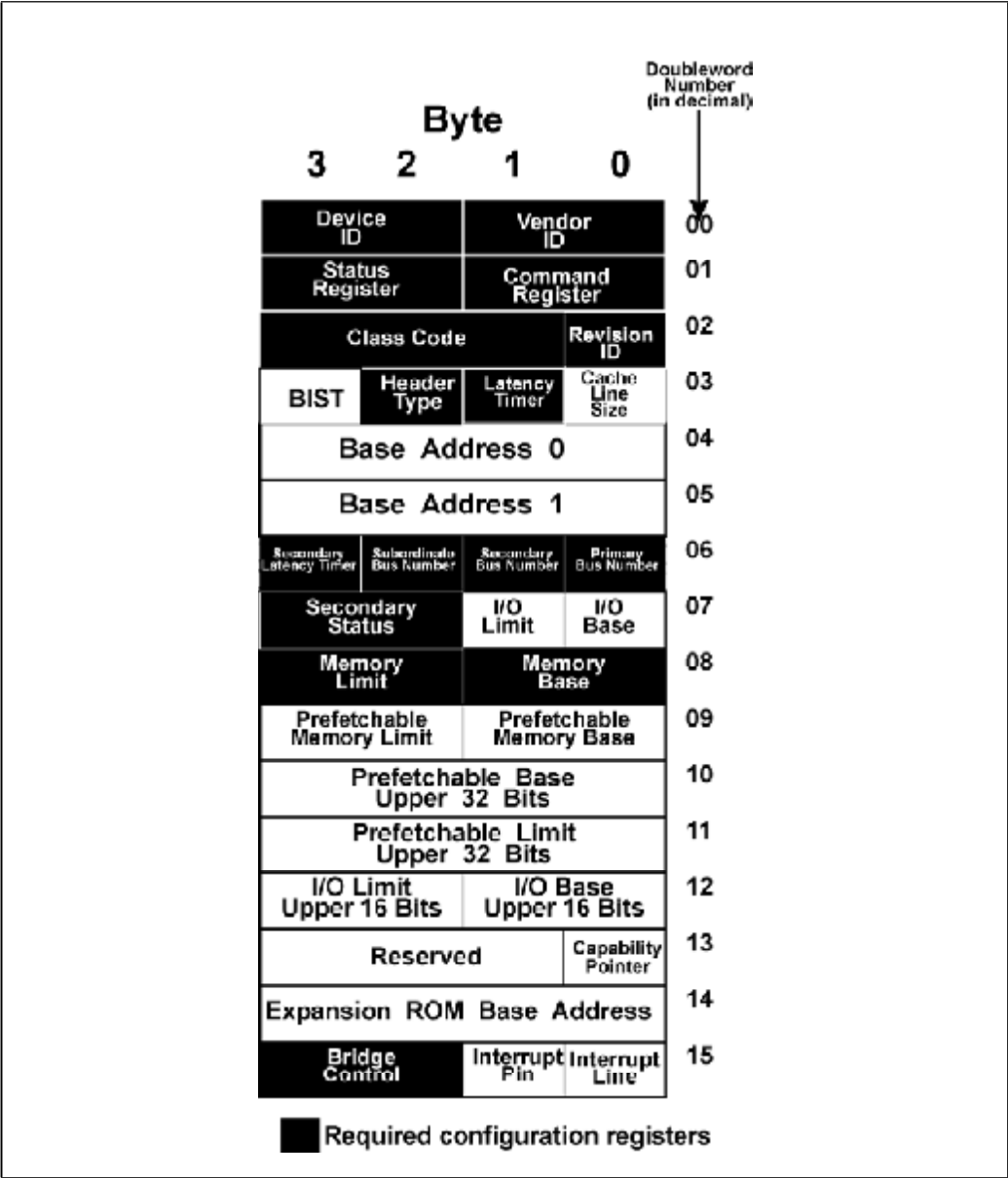
Figure 21-7: Header Type 1
