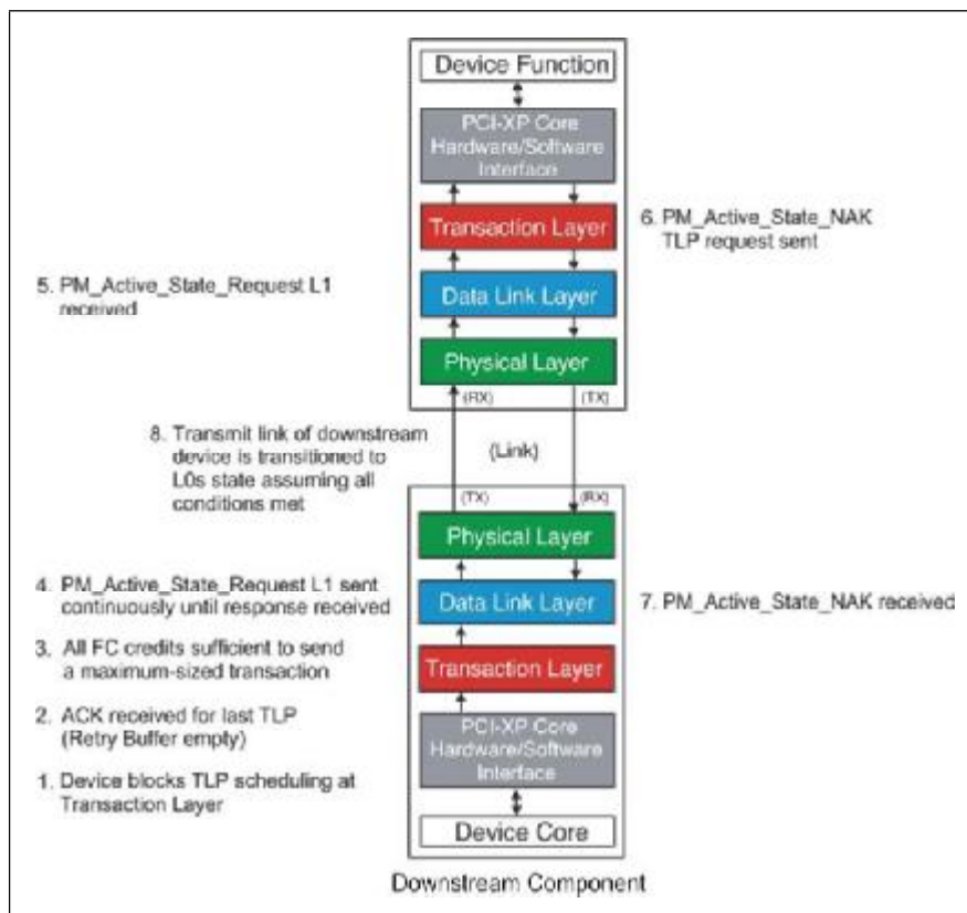
Figure 16-16: Negotiation Sequence Resulting in Rejection to Enter L1 ASPM State
