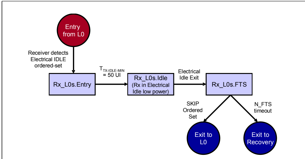
Figure 14-15: L0s Receiver State Machine
