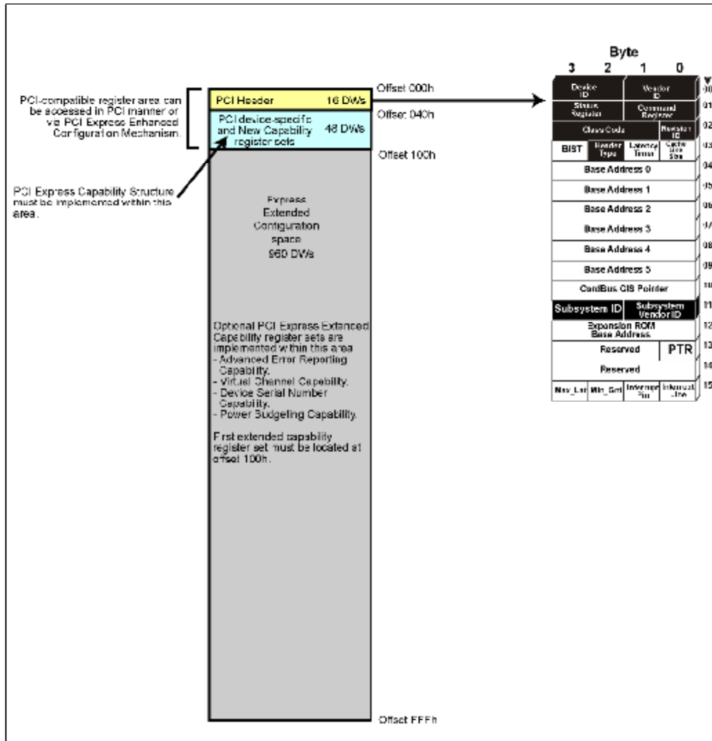
Figure 19-3: 4KB Configuration Space per PCI Express Function
