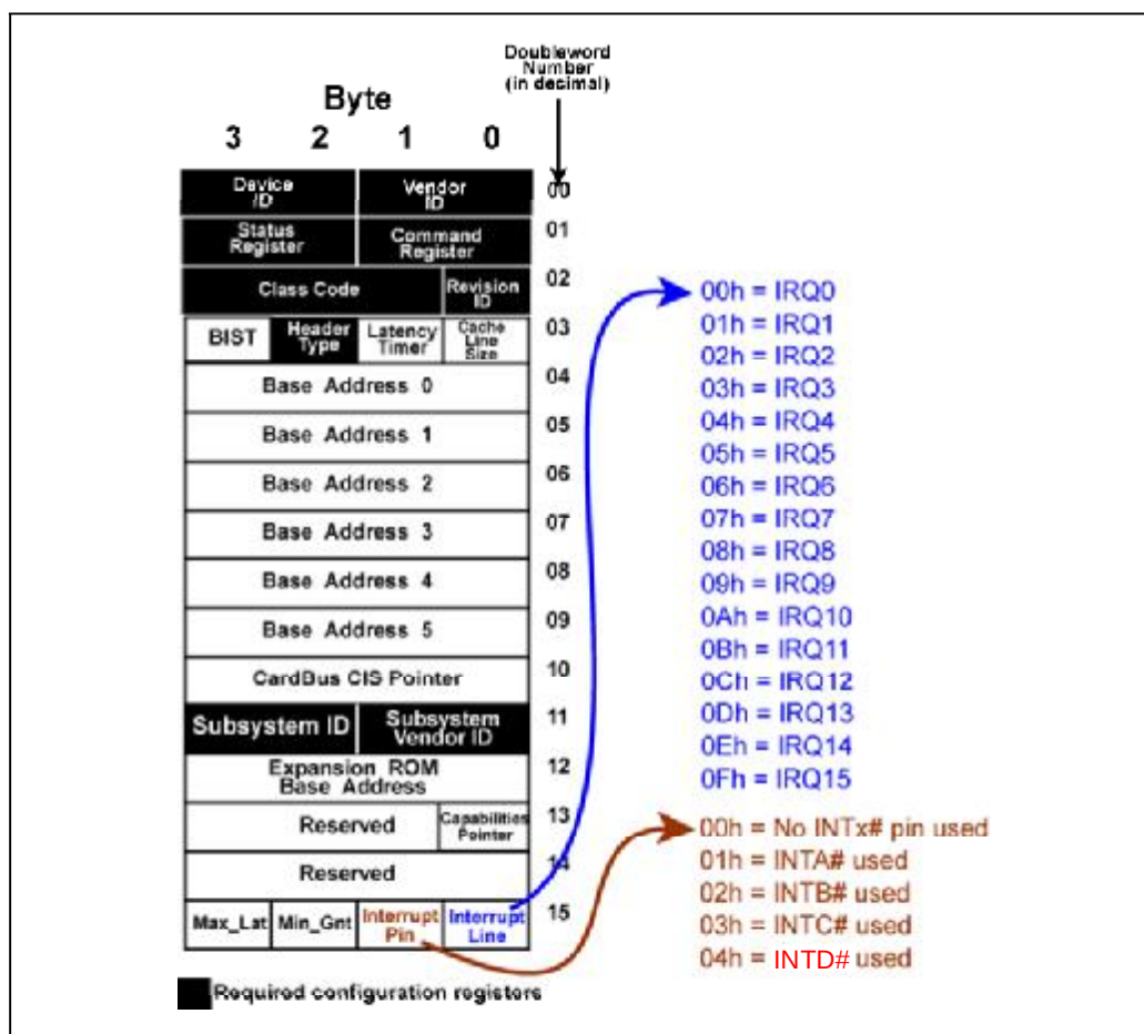
Figure 9-7: Interrupt Pin Register within PCI Configuration Header
