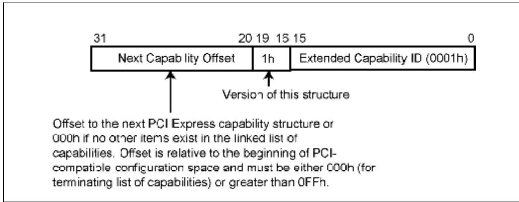
Figure 24-17: Advanced Error Reporting Enhanced Capability Header
