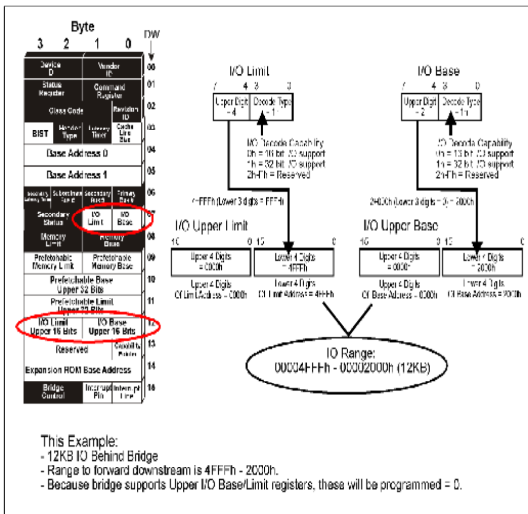
Figure 3-22: IO Base/Limit Register Set Up
