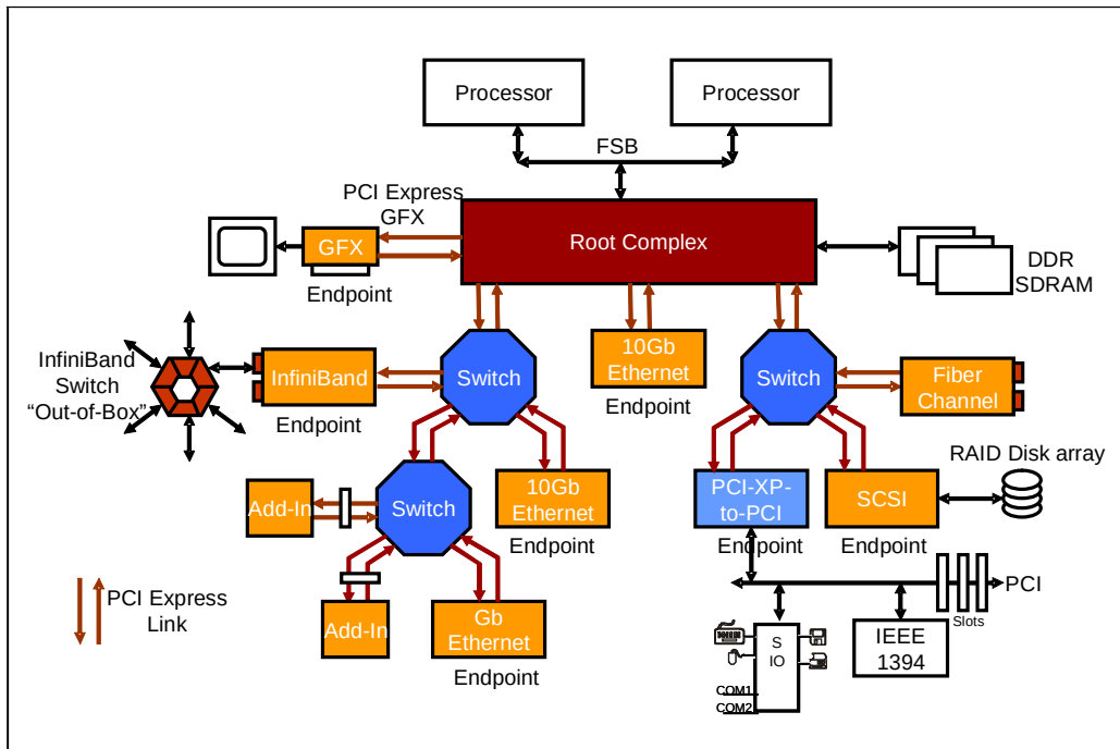
Figure 1-25: PCI Express High-End Server System
