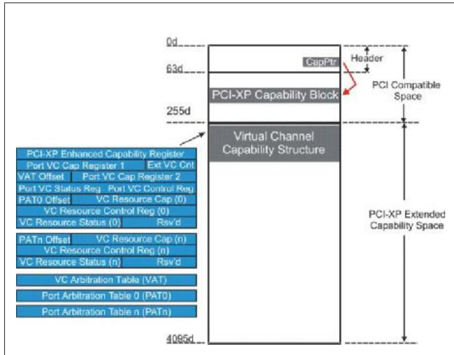
Figure 6-2: VC Configuration Registers Mapped in Extended Configuration Address Space
