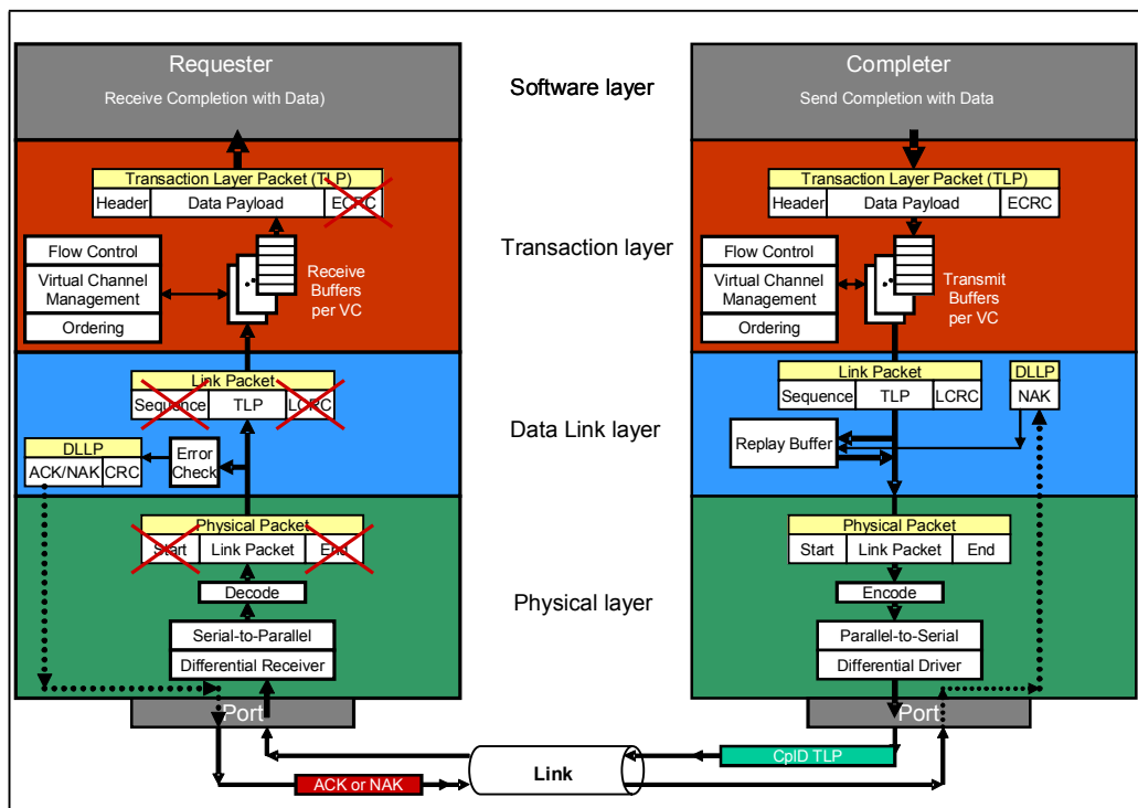
Figure 2-32: Completion with Data Phase
