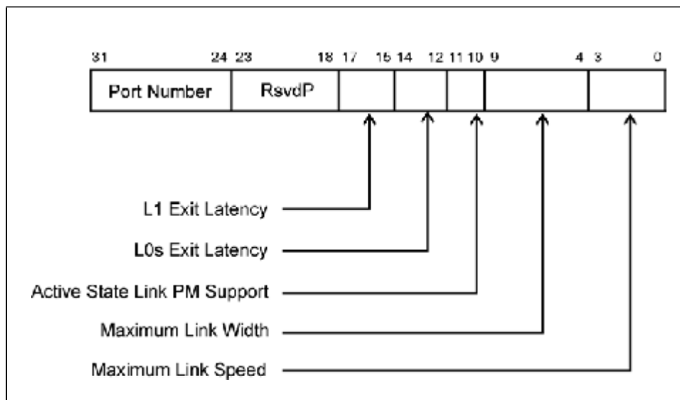
Figure 14-21: Link Capabilities Register
