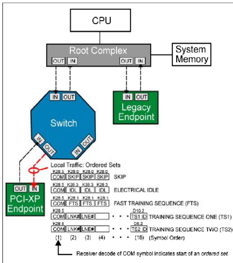
Figure 3-2: PCI Express Link Local Traffic: Ordered Sets
