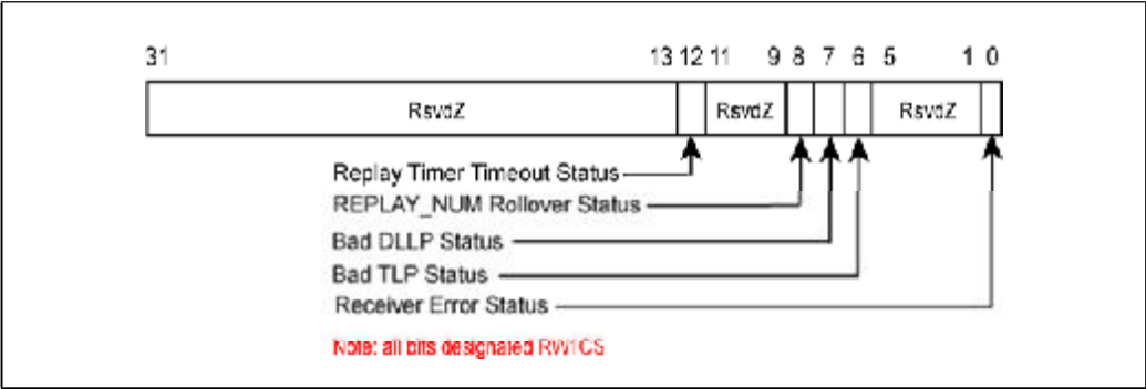
Figure 24-20: Advanced Error Correctable Error Status Register
