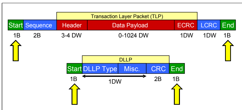
Figure 2-29: TLP and DLLP Structure at the Physical Layer
