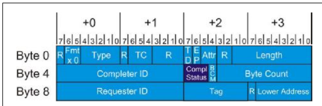
Figure 10-5: Completion Status Field within the Completion Header
