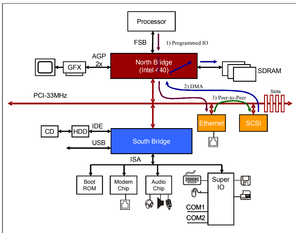
Figure 1-5: PCI Transaction Model
