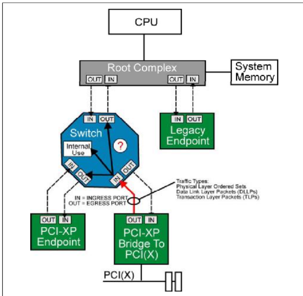
Figure 3-1: Multi-Port PCI Express Devices Have Routing Responsibilities
