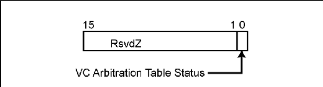
Figure 24-33: Port VC Status Register (Read-Only)
