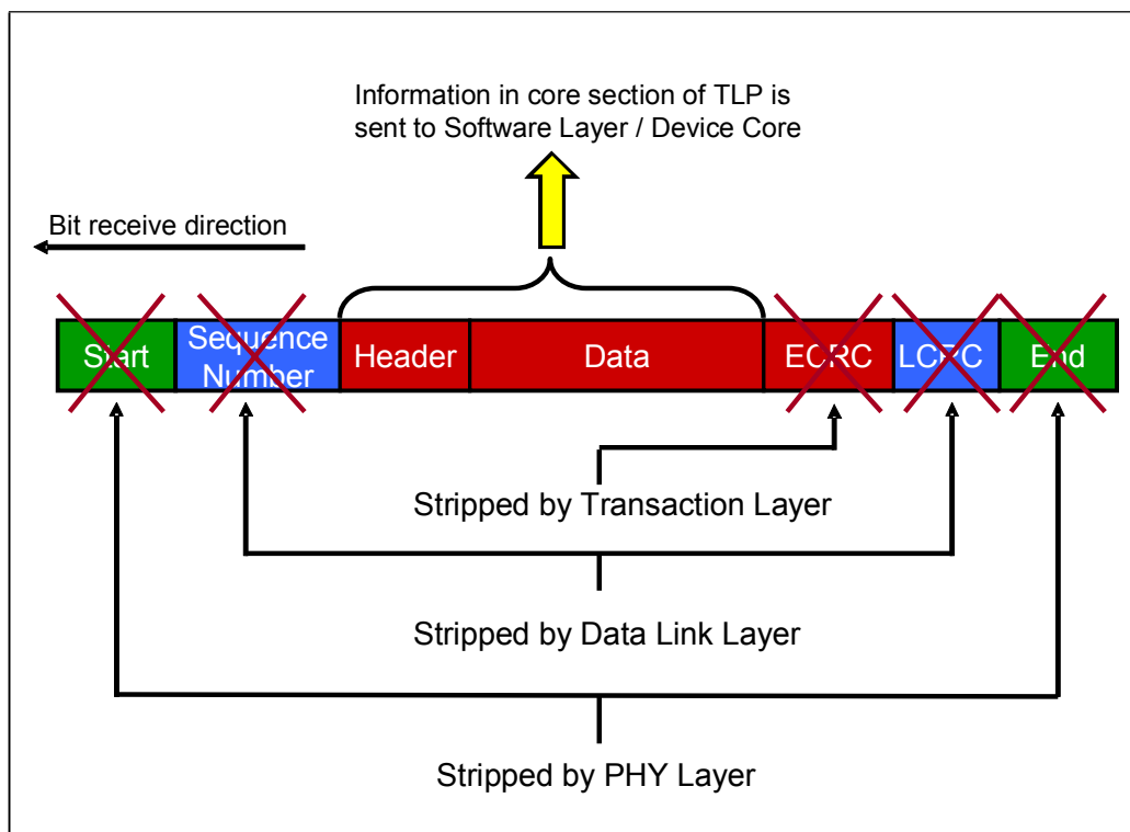
Figure 2-13: TLP Disassembly
