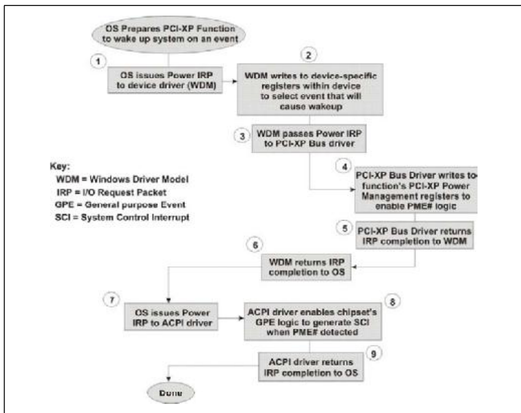
Figure 16-4: OS Prepares a Function To Cause System WakeUp On Device-Specific Event
