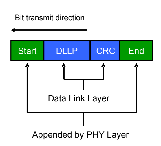
Figure 2-15: DLLP Assembly
