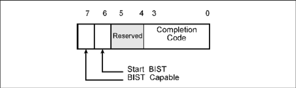
Figure 22-4: BIST Register Bit Assignment
