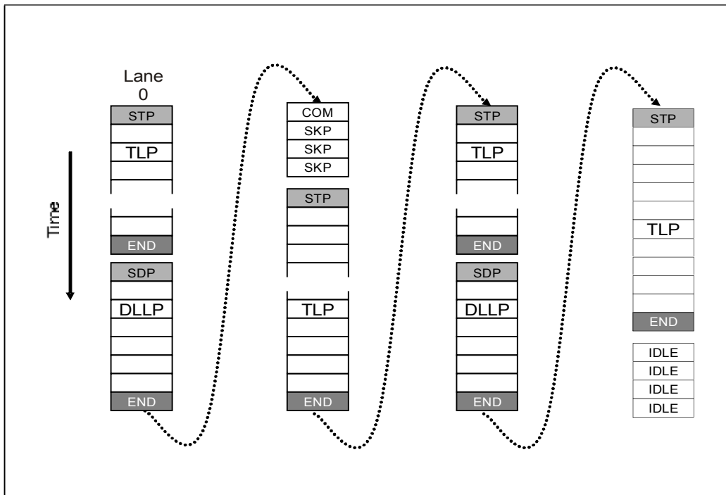
Figure 11-10: x1 Packet Format
