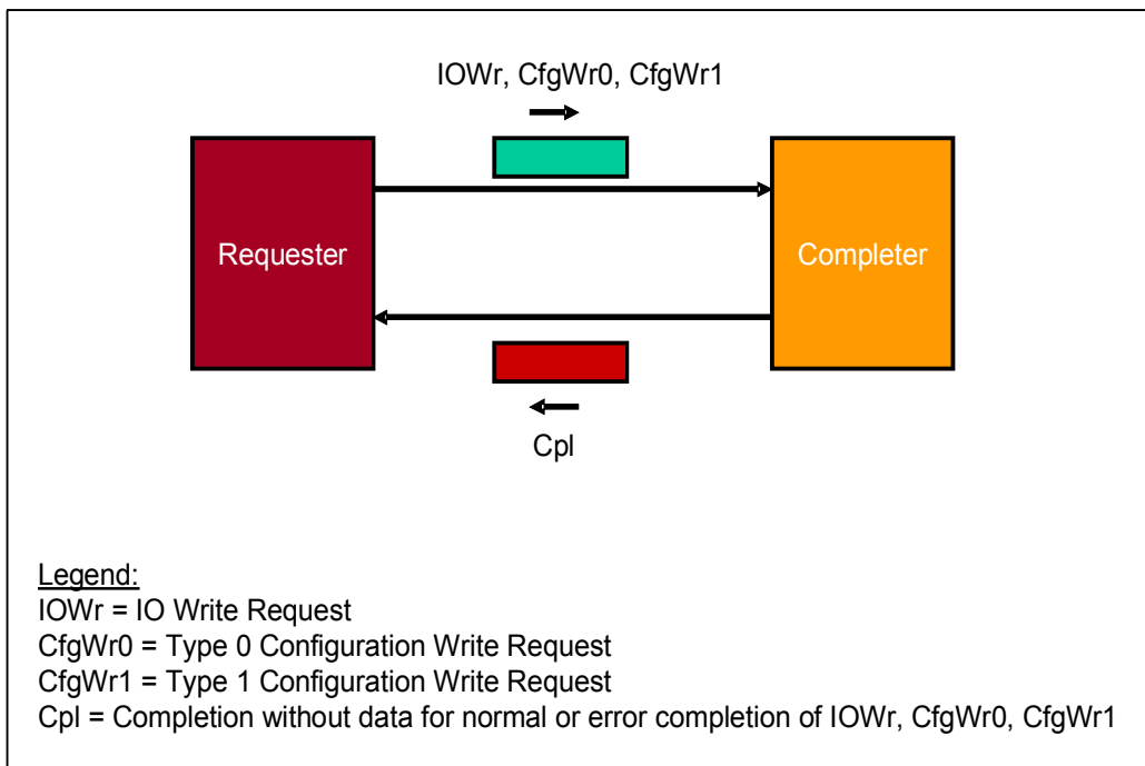
Figure 2-3: Non-Posted Write Transaction Protocol
