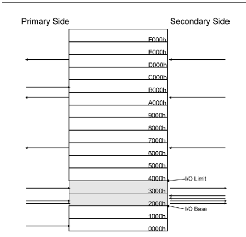
Figure 22-16: Example of IO Filtering Actions
