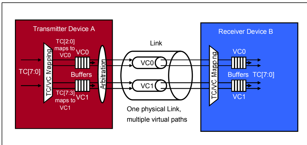
Figure 2-23: TC Numbers and VC Buffers
