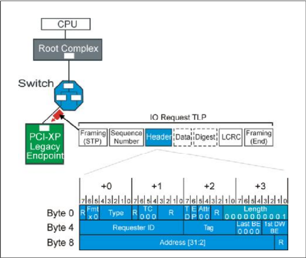
Figure 4-7: 3DW IO Request Header Format
