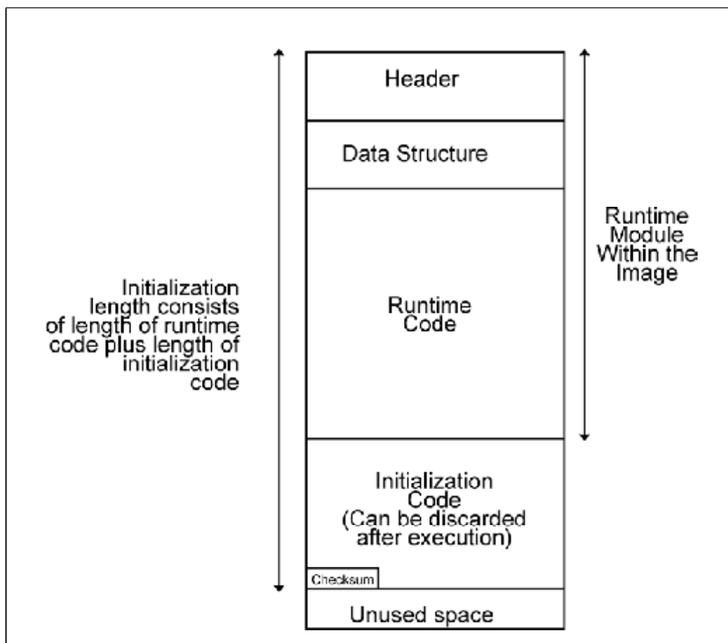
Figure 23-4: Code Image Format
