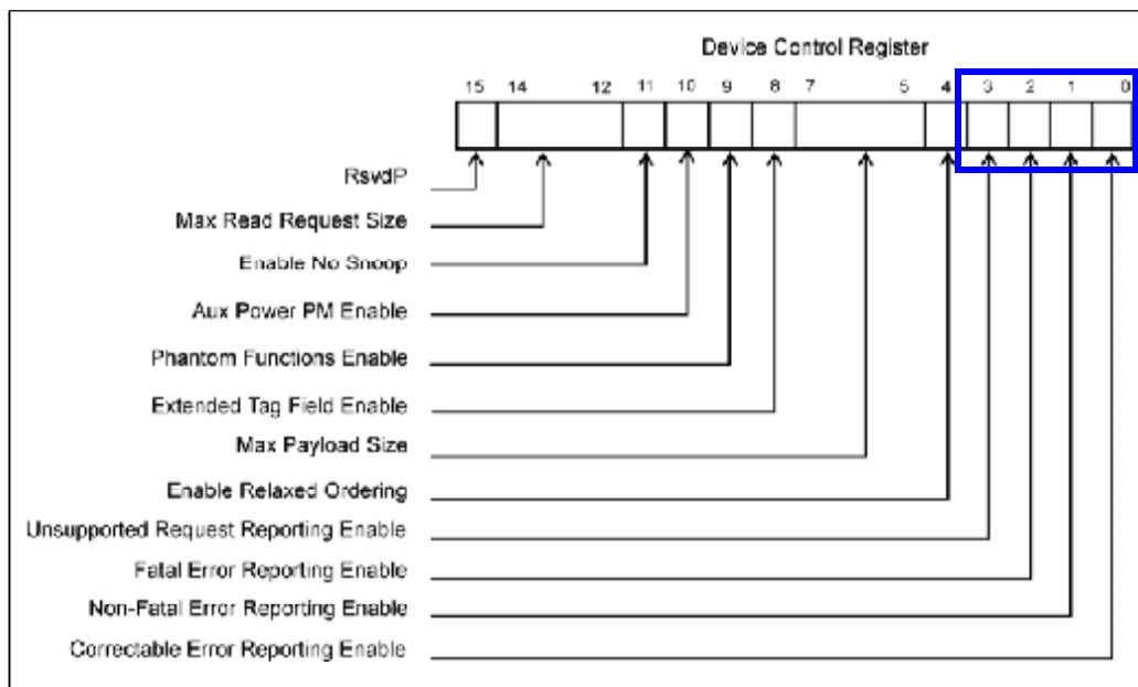
Figure 10-9: Device Control Register Bit Fields Related to Error Handling
