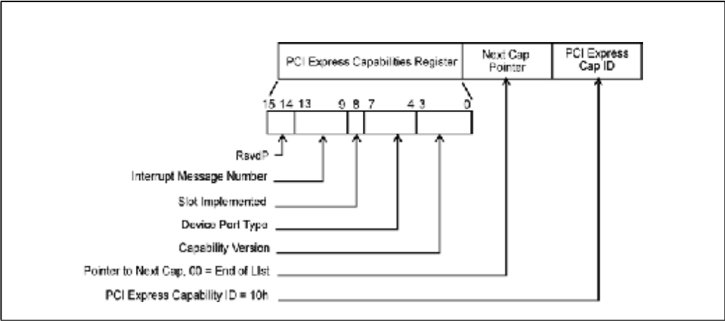
Figure 24-3: PCI Express Capabilities Register
