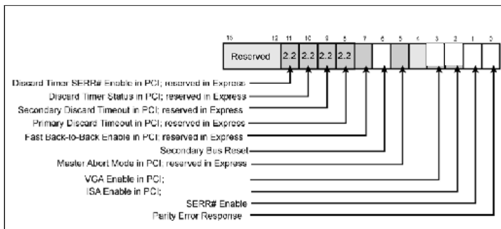
Figure 22-22: Bridge Control Register
