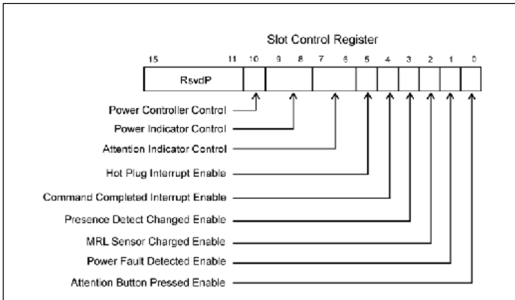
Figure 24-11: Slot Control Register
