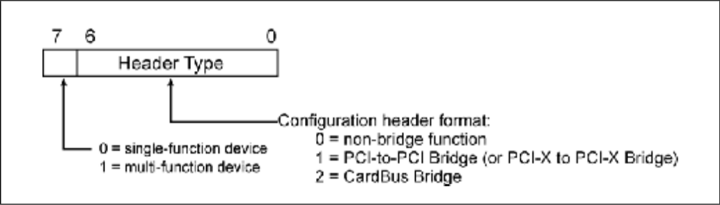
Figure 22-3: Header Type Register Bit Assignment
