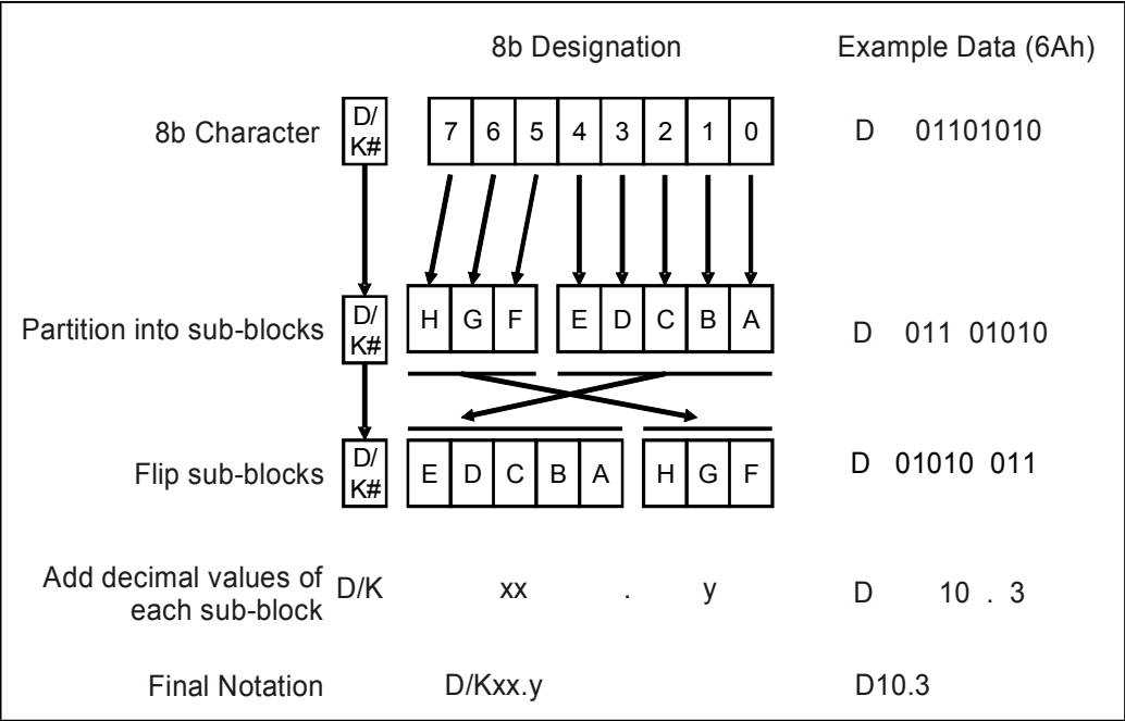
Figure 11-15: Preparing 8-bit Character for Encode
