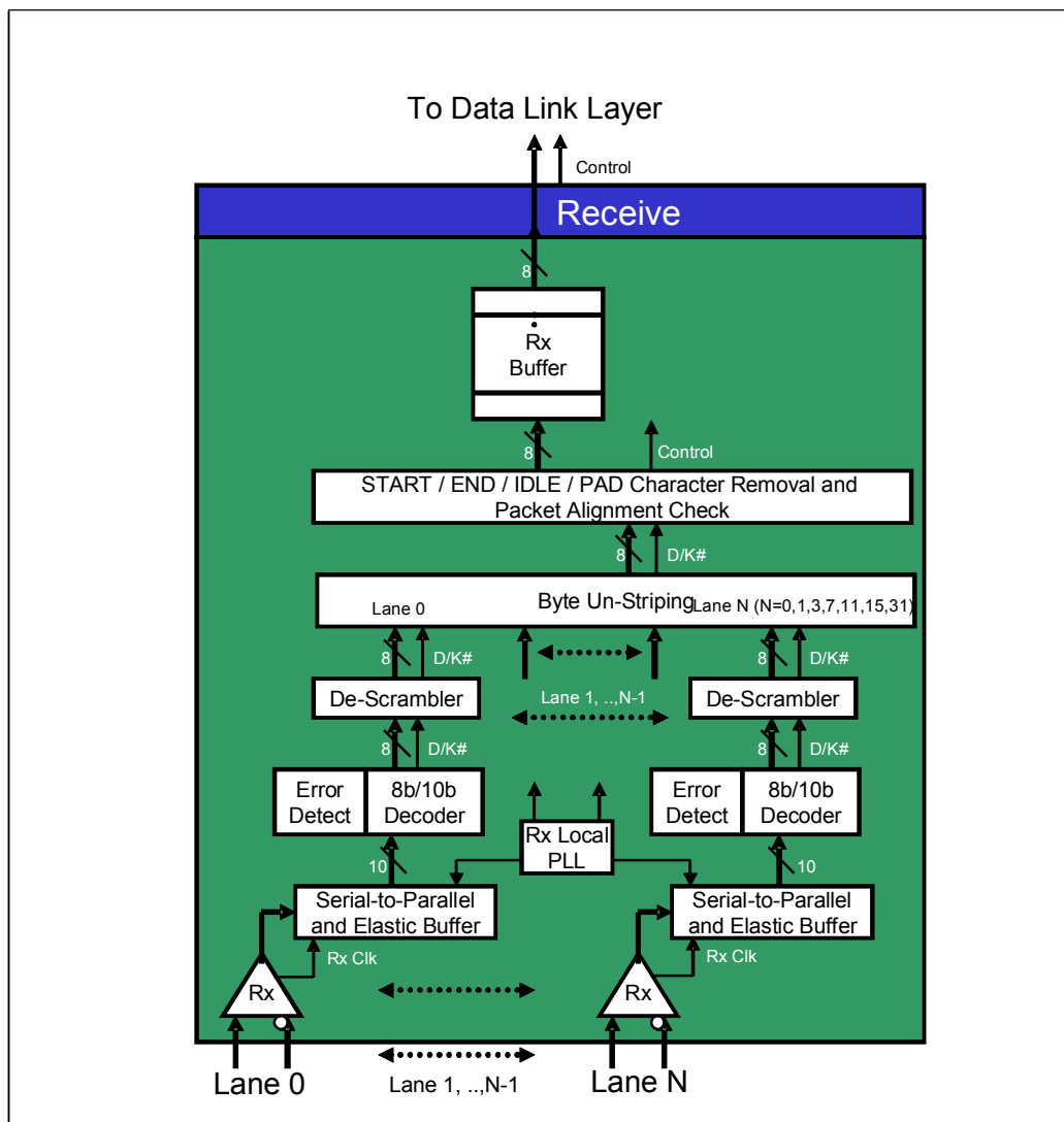
Figure 11-20: Physical Layer Receive Logic Details
