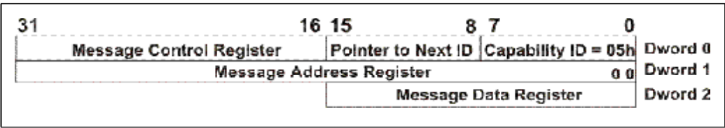
Figure 9-3: 32-bit MSI Capability Register Set Format
