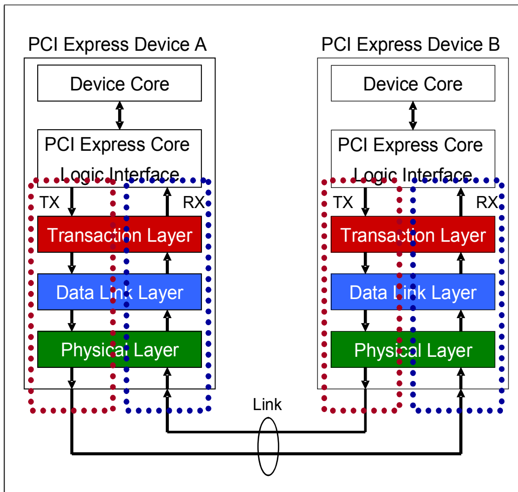
Figure 2-10: PCI Express Device Layers
