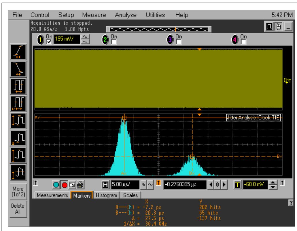
Figure A-21: Jitter analysis of a Transceiver source clock—Unacceptable (for a specific device)
