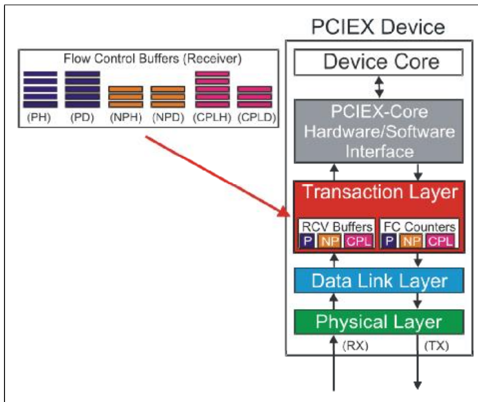
Figure 7-2: Flow Control Buffer Organization
